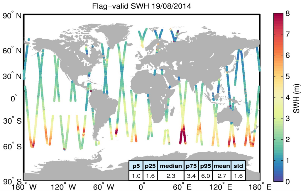
Figure 15. Geographical distribution of flag-valid SWH data over oceans and lakes for 19/08/2014. The statistical values shown in the table refer to the SWH in m and are calculated over all measurements shown in the figure.
