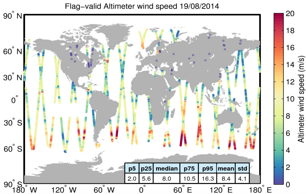
Figure 31. Geographical distribution of flag-valid wind data over oceans and lakes for 19/08/2014. The statistical values shown in the table refer to the wind in m/s and are calculated over all measurements shown in the figure.
