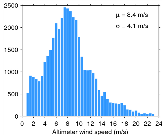
Figure 35. Histogram of science-valid wind over oceans and lakes for 19/08/2014. The mean ( \mu ) and standard deviation ( \sigma ) are also shown. Note that values larger than 24 m/s are excluded from the histogram for the sake of readability but not from the computation of \mu and \sigma .
