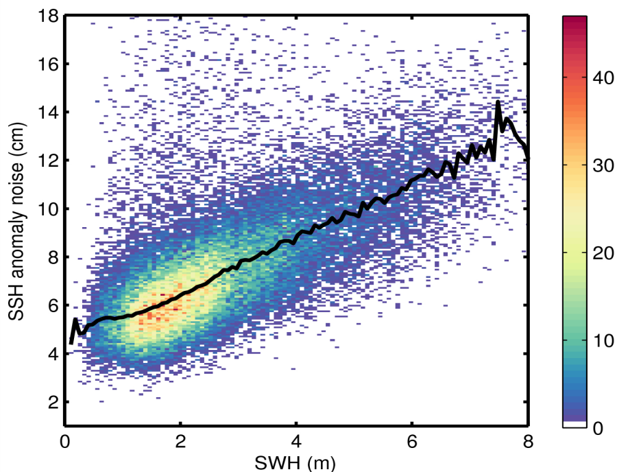
Figure 9. 2D histogram showing flag-valid SSH anomaly noise as a function of SWH for 19/08/2014. The black line denotes the median SSH anomaly as a function of SWH.
