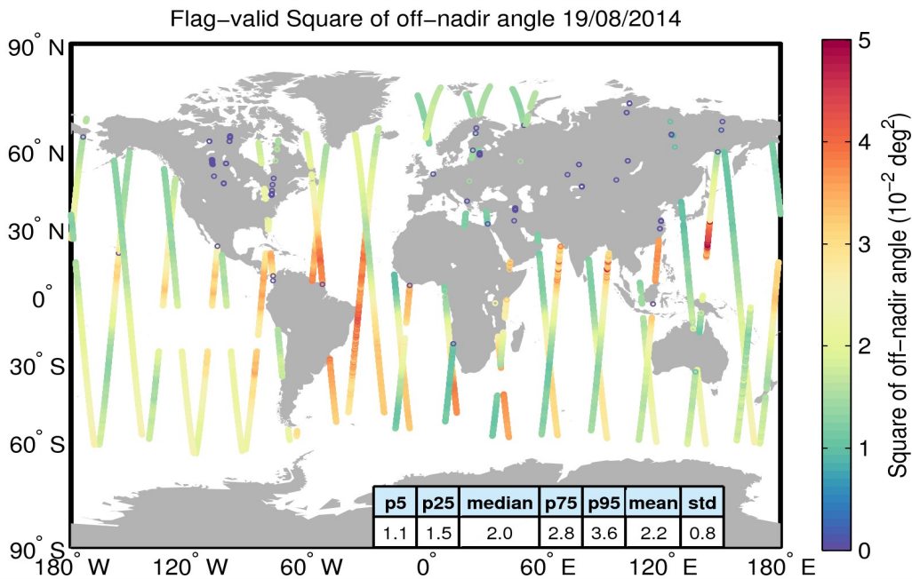
Figure 37. Geographical distribution of flag-valid mispointing data over oceans and lakes for 19/08/2014. The statistical values shown in the table refer to the mispointing in 10^{-2} \text{ deg}^2 and are calculated over all measurements shown in the figure.
