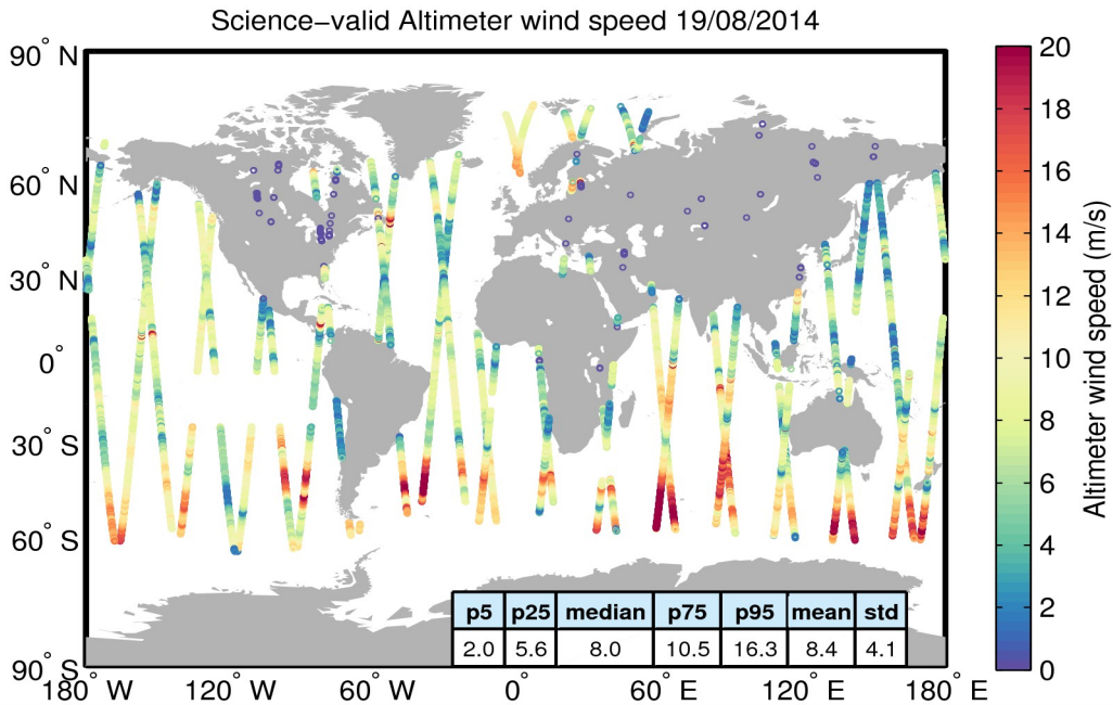
Figure 34. Geographical distribution of science-valid wind data over oceans and lakes for 19/08/2014. The statistical values shown in the table refer to the wind in m/s and are calculated over all measurements shown in the figure. Gray circles denote records that have been rejected based on the editing criteria described in Table 5.
