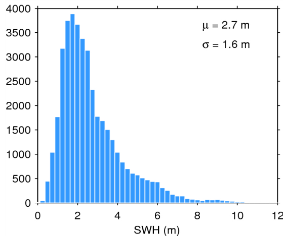
Figure 20. Histogram of science-valid SWH over oceans and lakes for 19/08/2014. The mean ( \mu ) and standard deviation ( \sigma ) are also shown. Note that values larger than 12 m are excluded from the histogram for the sake of readability but not from the computation of \mu and \sigma .
