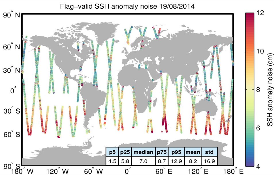
Figure 8. Geographical distribution of flag-valid 20-Hz SSH anomaly measurement noise over oceans and lakes for 19/08/2014. The statistical values shown in the table refer to the SSH anomaly noise and are calculated over all measurements shown in the figure.
