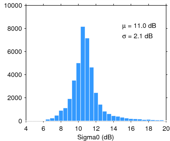
Figure 25. Histogram of flag-valid sigma0 over oceans and lakes for 19/08/2014. The mean ( \mu ) and standard deviation ( \sigma ) are also shown. Note that values outside [4 20] dB are excluded from the histogram for the sake of readability but not from the computation of \mu and \sigma .
