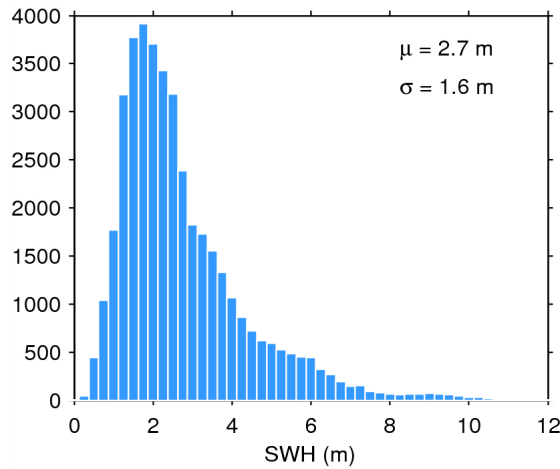
Figure 17. Histogram of flag-valid SWH over oceans and lakes for 19/08/2014. The mean ( \mu ) and standard deviation ( \sigma ) are also shown. Note that values larger than 12 m are excluded from the histogram for the sake of readability but not from the computation of \mu and \sigma .
