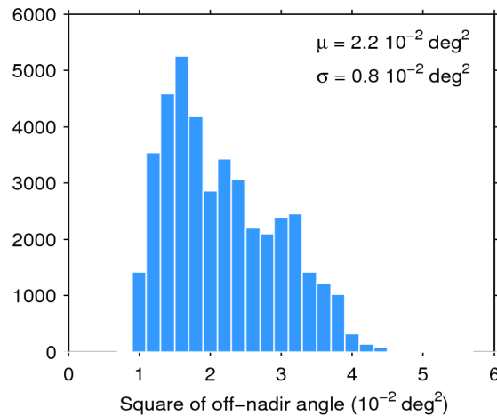
Figure 39. Histogram of flag-valid mispointing over oceans and lakes for 19/08/2014. The mean ( \mu ) and standard deviation ( \sigma ) are also shown. Note that values than 6 \cdot 10^{-2} \text{ deg}^2 are excluded from the histogram for the sake of readability but not from the computation of \mu and \sigma .
