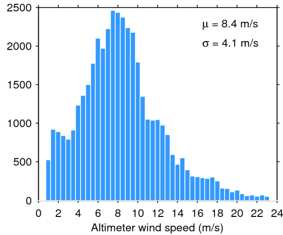
Figure 33. Histogram of flag-valid wind over oceans and lakes for 19/08/2014. The mean ( \mu ) and standard deviation ( \sigma ) are also shown. Note that values larger than 24 m/s are excluded from the histogram for the sake of readability but not from the computation of \mu and \sigma .
