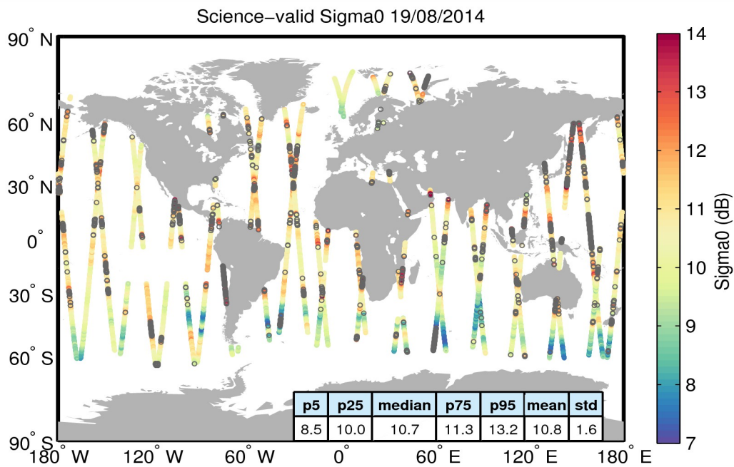
Figure 27. Geographical distribution of science-valid sigma0 data over oceans and lakes for 19/08/2014. The statistical values shown in the table refer to the sigma0 in dB and are calculated over all measurements shown in the figure. Gray circles denote records that have been rejected based on the editing criteria described in Table 4.
