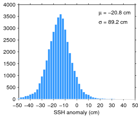
Figure 7. Histogram of flag-valid SSH anomaly over oceans and lakes for 19/08/2014. The mean ( \mu ) and standard deviation ( \sigma ) are also shown. Note that values outside [-50 50] cm are excluded from the histogram for the sake of readability but not from the computation of \mu and \sigma .
