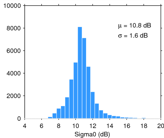
Figure 28. Histogram of science-valid sigma0 over oceans and lakes for 19/08/2014. The mean ( \mu ) and standard deviation ( \sigma ) are also shown. Note that values outside [4 20] dB are excluded from the histogram for the sake of readability but not from the computation of \mu and \sigma .
