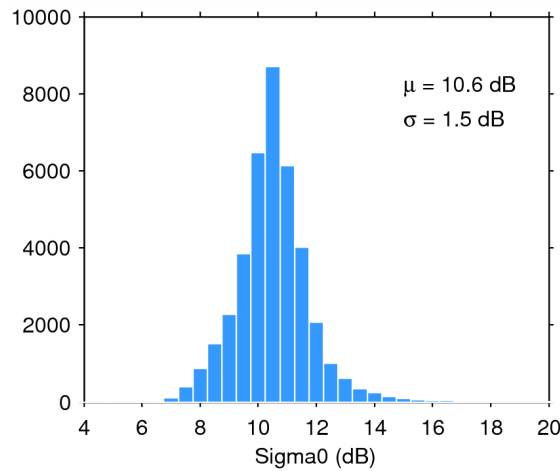
Figure 28. Histogram of science-valid sigma0 over oceans and lakes for 09/08/2014. The mean ( \mu ) and standard deviation ( \sigma ) are also shown. Note that values outside [4 20] dB are excluded from the histogram for the sake of readability but not from the computation of \mu and \sigma .
