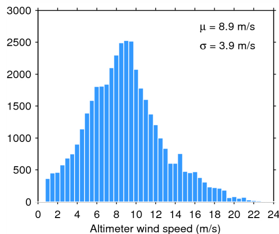
Figure 35. Histogram of science-valid wind over oceans and lakes for 09/08/2014. The mean ( \mu ) and standard deviation ( \sigma ) are also shown. Note that values larger than 24 m/s are excluded from the histogram for the sake of readability but not from the computation of \mu and \sigma .
