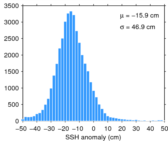
Figure 7. Histogram of flag-valid SSH anomaly over oceans and lakes for 09/08/2014. The mean ( \mu ) and standard deviation ( \sigma ) are also shown. Note that values outside [-50 50] cm are excluded from the histogram for the sake of readability but not from the computation of \mu and \sigma .
