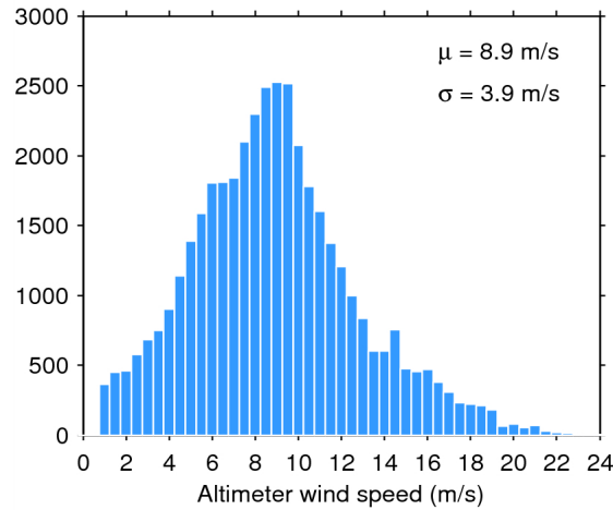
Figure 33. Histogram of flag-valid wind over oceans and lakes for 09/08/2014. The mean ( \mu ) and standard deviation ( \sigma ) are also shown. Note that values larger than 24 m/s are excluded from the histogram for the sake of readability but not from the computation of \mu and \sigma .
