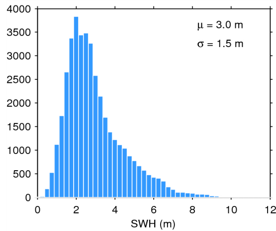
Figure 17. Histogram of flag-valid SWH over oceans and lakes for 09/08/2014. The mean ( \mu ) and standard deviation ( \sigma ) are also shown. Note that values larger than 12 m are excluded from the histogram for the sake of readability but not from the computation of \mu and \sigma .
