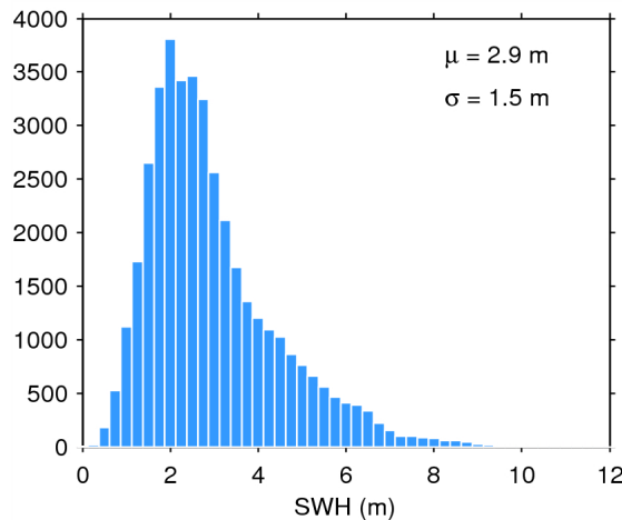
Figure 20. Histogram of science-valid SWH over oceans and lakes for 09/08/2014. The mean ( \mu ) and standard deviation ( \sigma ) are also shown. Note that values larger than 12 m are excluded from the histogram for the sake of readability but not from the computation of \mu and \sigma .
