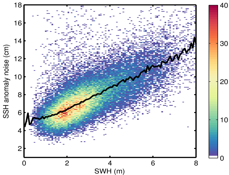
Figure 9. 2D histogram showing flag-valid SSH anomaly noise as a function of SWH for 09/08/2014. The black line denotes the median SSH anomaly as a function of SWH.
