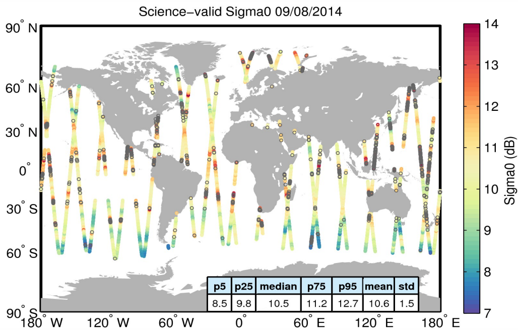
Figure 27. Geographical distribution of science-valid sigma0 data over oceans and lakes for 09/08/2014. The statistical values shown in the table refer to the sigma0 in dB and are calculated over all measurements shown in the figure. Gray circles denote records that have been rejected based on the editing criteria described in Table 4.
