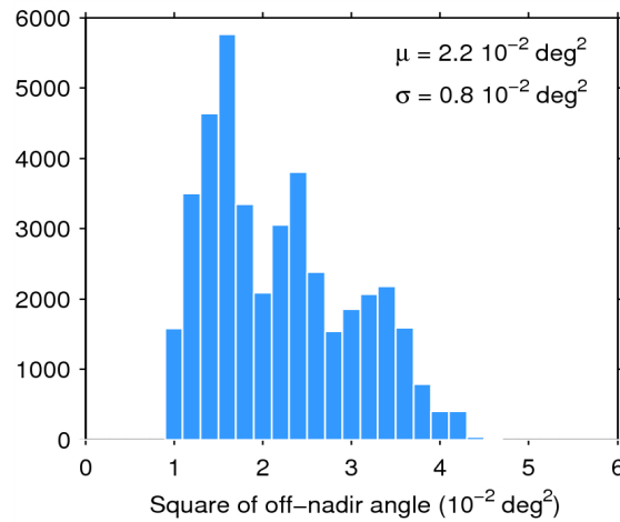
Figure 39. Histogram of flag-valid mispointing over oceans and lakes for 09/08/2014. The mean ( \mu ) and standard deviation ( \sigma ) are also shown. Note that values than 6 \cdot 10^{-2} \text{ deg}^2 are excluded from the histogram for the sake of readability but not from the computation of \mu and \sigma .
