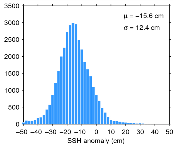
Figure 11. Histogram of science-valid SSH anomaly over oceans and lakes for 09/08/2014. The mean ( \mu ) and standard deviation ( \sigma ) are also shown. Note that values outside [-50 50] cm are excluded from the histogram for the sake of readability but not from the computation of \mu and \sigma .
