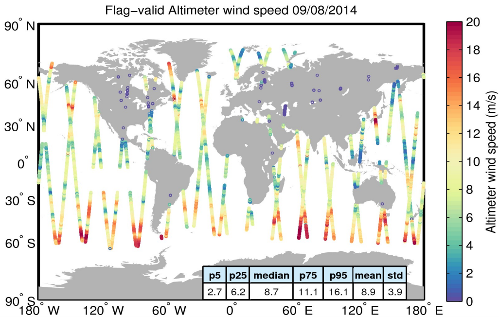
Figure 31. Geographical distribution of flag-valid wind data over oceans and lakes for 09/08/2014. The statistical values shown in the table refer to the wind in m/s and are calculated over all measurements shown in the figure.
