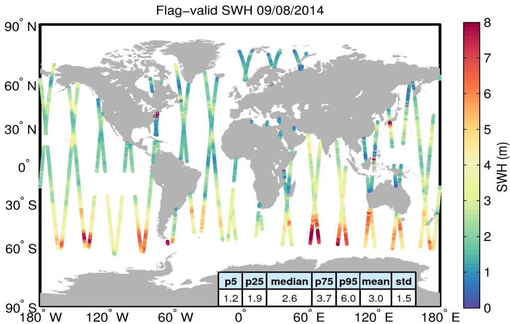
Figure 15. Geographical distribution of flag-valid SWH data over oceans and lakes for 09/08/2014. The statistical values shown in the table refer to the SWH in m and are calculated over all measurements shown in the figure.
