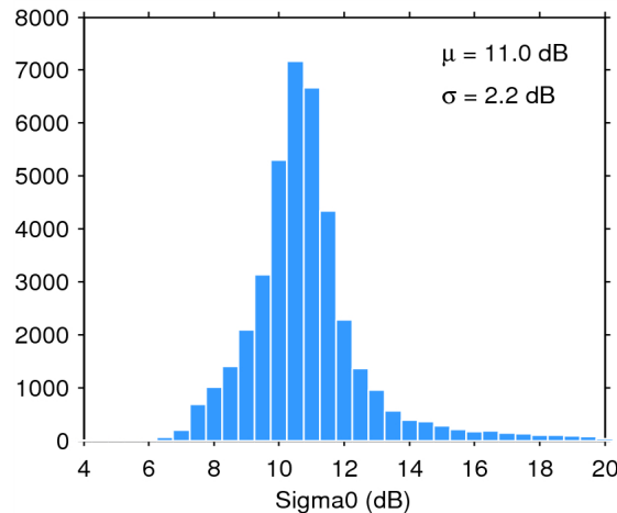
Figure 25. Histogram of flag-valid sigma0 over oceans and lakes for 31/07/2014. The mean ( \mu ) and standard deviation ( \sigma ) are also shown. Note that values outside [4 20] dB are excluded from the histogram for the sake of readability but not from the computation of \mu and \sigma .
