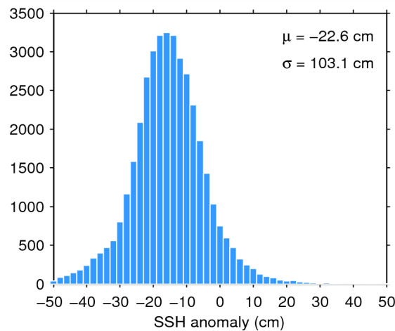
Figure 7. Histogram of flag-valid SSH anomaly over oceans and lakes for 31/07/2014. The mean ( \mu ) and standard deviation ( \sigma ) are also shown. Note that values outside [-50\ 50] cm are excluded from the histogram for the sake of readability but not from the computation of \mu and \sigma .
