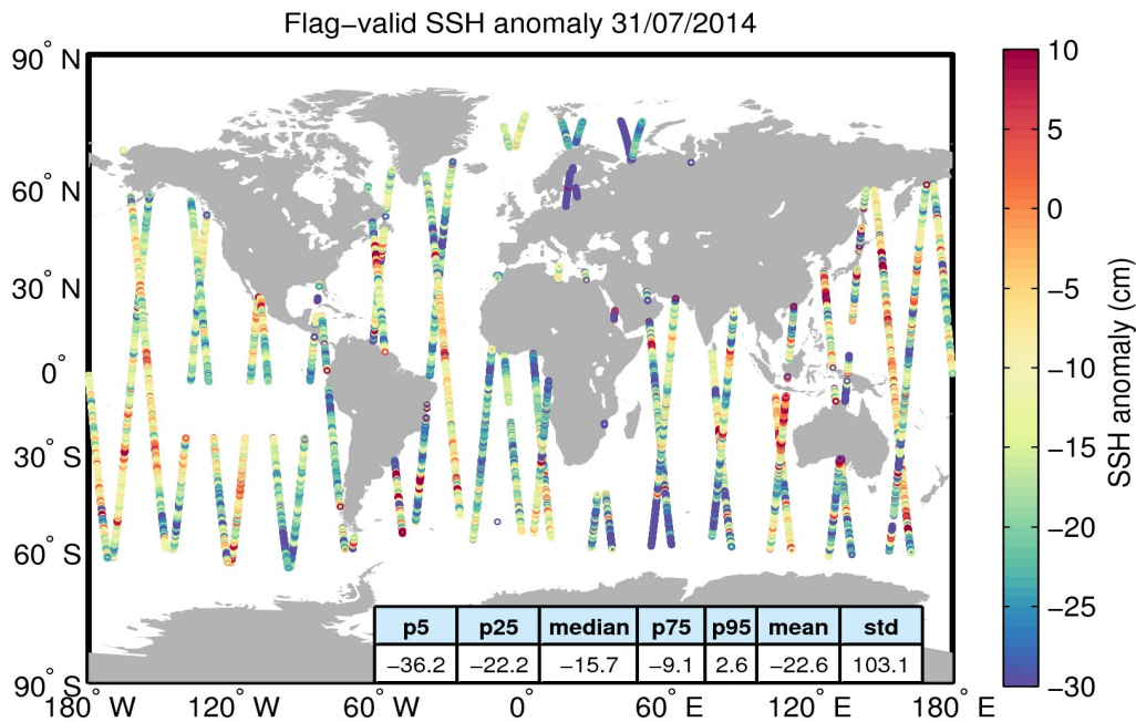
Figure 5. Geographical distribution of flag-valid 1-Hz SSH anomaly data over oceans and lakes for 31/07/2014. The statistical values shown in the table refer to the SSH anomaly in cm and are calculated over all measurements shown in the figure.
