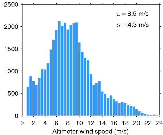
Figure 33. Histogram of flag-valid wind over oceans and lakes for 31/07/2014. The mean ( \mu ) and standard deviation ( \sigma ) are also shown. Note that values larger than 24 m/s are excluded from the histogram for the sake of readability but not from the computation of \mu and \sigma .
