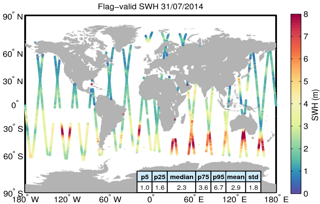
Figure 15. Geographical distribution of flag-valid SWH data over oceans and lakes for 31/07/2014. The statistical values shown in the table refer to the SWH in m and are calculated over all measurements shown in the figure.
