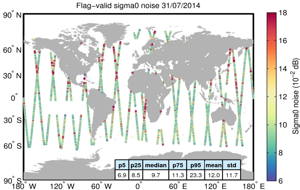
Figure 26. Geographical distribution of flag-valid 20-Hz sigma0 measurement noise over oceans and lakes for 31/07/2014. The statistical values shown in the table refer to the sigma0 noise and are calculated over all measurements shown in the figure.
