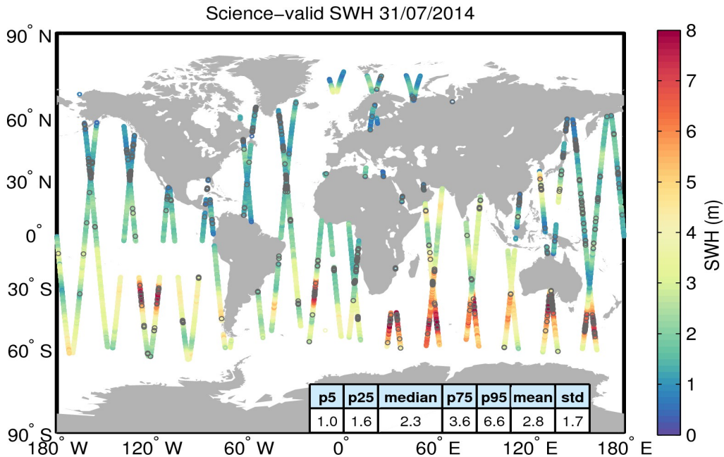
Figure 19. Geographical distribution of science-valid SWH data over oceans and lakes for 31/07/2014. The statistical values shown in the table refer to the SWH in m and are calculated over all measurements shown in the figure. Gray circles denote records that have been rejected based on the editing criteria described in Table 3.
