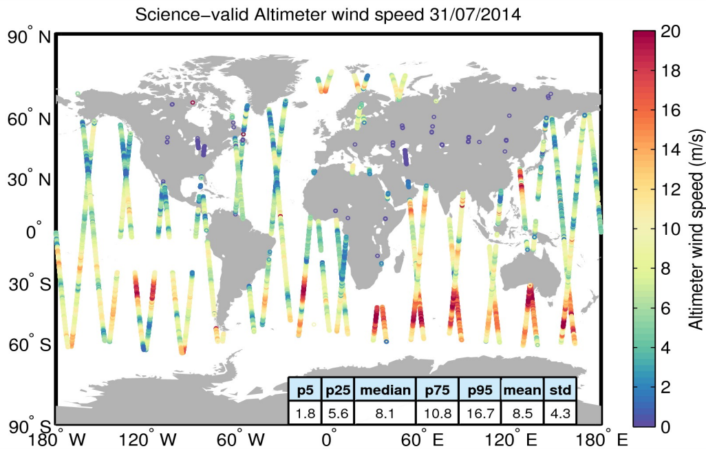
Figure 34. Geographical distribution of science-valid wind data over oceans and lakes for 31/07/2014. The statistical values shown in the table refer to the wind in m/s and are calculated over all measurements shown in the figure. Gray circles denote records that have been rejected based on the editing criteria described in Table 5.
