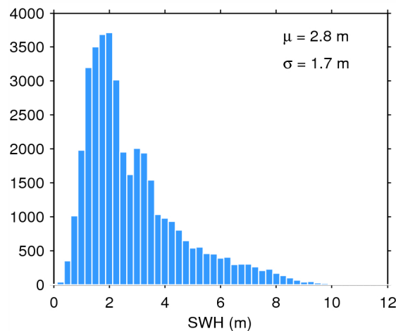
Figure 20. Histogram of science-valid SWH over oceans and lakes for 31/07/2014. The mean ( \mu ) and standard deviation ( \sigma ) are also shown. Note that values larger than 12 m are excluded from the histogram for the sake of readability but not from the computation of \mu and \sigma .
