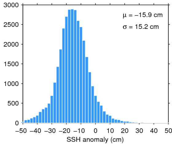
Figure 11. Histogram of science-valid SSH anomaly over oceans and lakes for 31/07/2014. The mean ( \mu ) and standard deviation ( \sigma ) are also shown. Note that values outside [-50 50] cm are excluded from the histogram for the sake of readability but not from the computation of \mu and \sigma .
