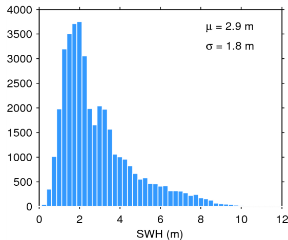
Figure 17. Histogram of flag-valid SWH over oceans and lakes for 31/07/2014. The mean ( \mu ) and standard deviation ( \sigma ) are also shown. Note that values larger than 12 m are excluded from the histogram for the sake of readability but not from the computation of \mu and \sigma .
