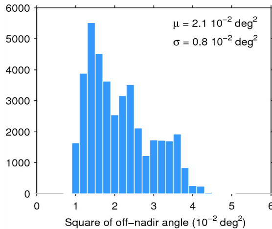
Figure 39. Histogram of flag-valid mispointing over oceans and lakes for 31/07/2014. The mean ( \mu ) and standard deviation ( \sigma ) are also shown. Note that values than 6 \cdot 10^{-2} \text{ deg}^2 are excluded from the histogram for the sake of readability but not from the computation of \mu and \sigma .
