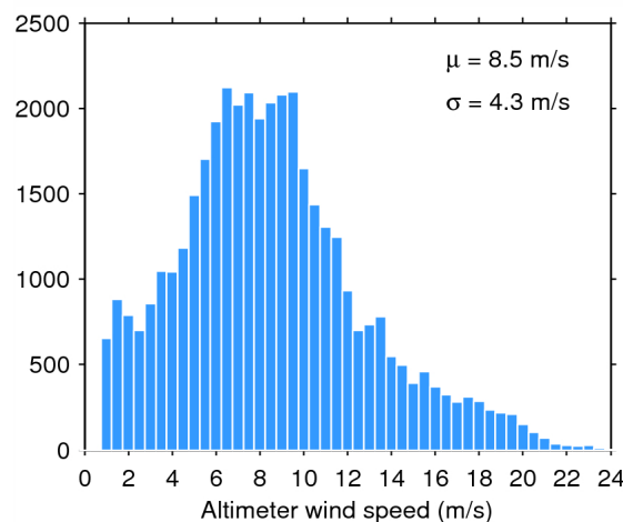
Figure 35. Histogram of science-valid wind over oceans and lakes for 31/07/2014. The mean ( \mu ) and standard deviation ( \sigma ) are also shown. Note that values larger than 24 m/s are excluded from the histogram for the sake of readability but not from the computation of \mu and \sigma .
