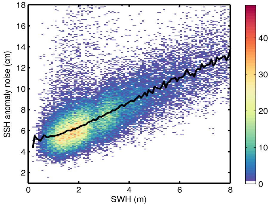
Figure 9. 2D histogram showing flag-valid SSH anomaly noise as a function of SWH for 31/07/2014. The black line denotes the median SSH anomaly as a function of SWH.
