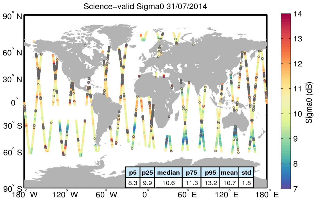
Figure 27. Geographical distribution of science-valid sigma0 data over oceans and lakes for 31/07/2014. The statistical values shown in the table refer to the sigma0 in dB and are calculated over all measurements shown in the figure. Gray circles denote records that have been rejected based on the editing criteria described in Table 4.
