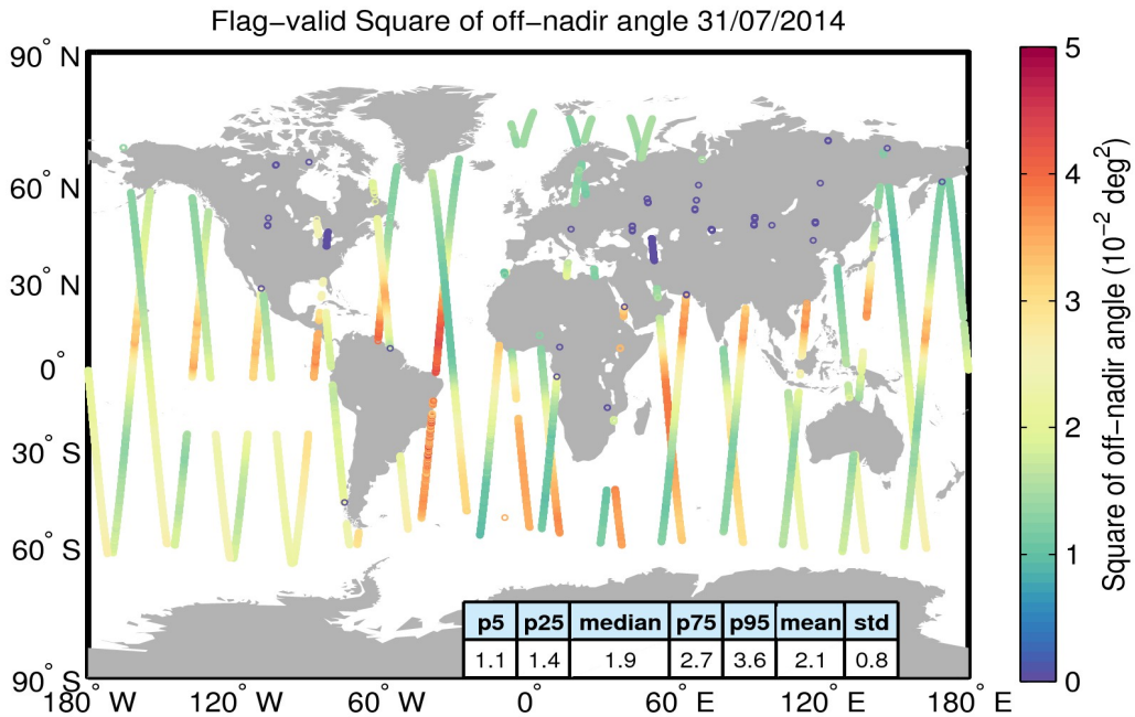
Figure 37. Geographical distribution of flag-valid mispointing data over oceans and lakes for 31/07/2014. The statistical values shown in the table refer to the mispointing in 10^{-2} \text{ deg}^2 and are calculated over all measurements shown in the figure.
