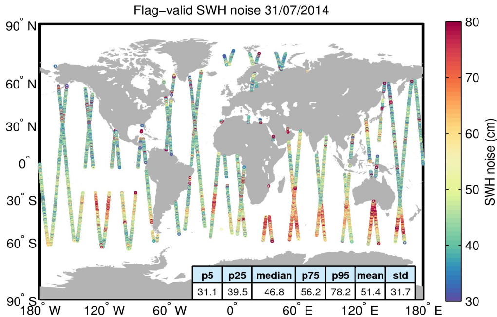
Figure 18. Geographical distribution of flag-valid 20-Hz SWH measurement noise over oceans and lakes for 31/07/2014. The statistical values shown in the figure refer to the SWH noise and are calculated over all measurements shown in the figure.
