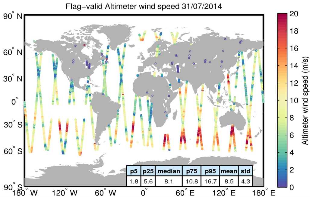
Figure 31. Geographical distribution of flag-valid wind data over oceans and lakes for 31/07/2014. The statistical values shown in the table refer to the wind in m/s and are calculated over all measurements shown in the figure.
