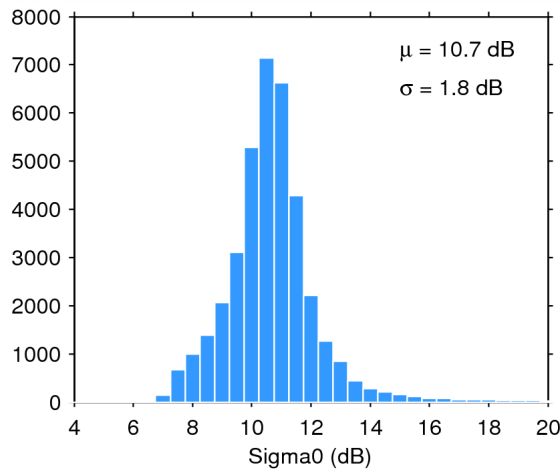
Figure 28. Histogram of science-valid sigma0 over oceans and lakes for 31/07/2014. The mean ( \mu ) and standard deviation ( \sigma ) are also shown. Note that values outside [4 20] dB are excluded from the histogram for the sake of readability but not from the computation of \mu and \sigma .
