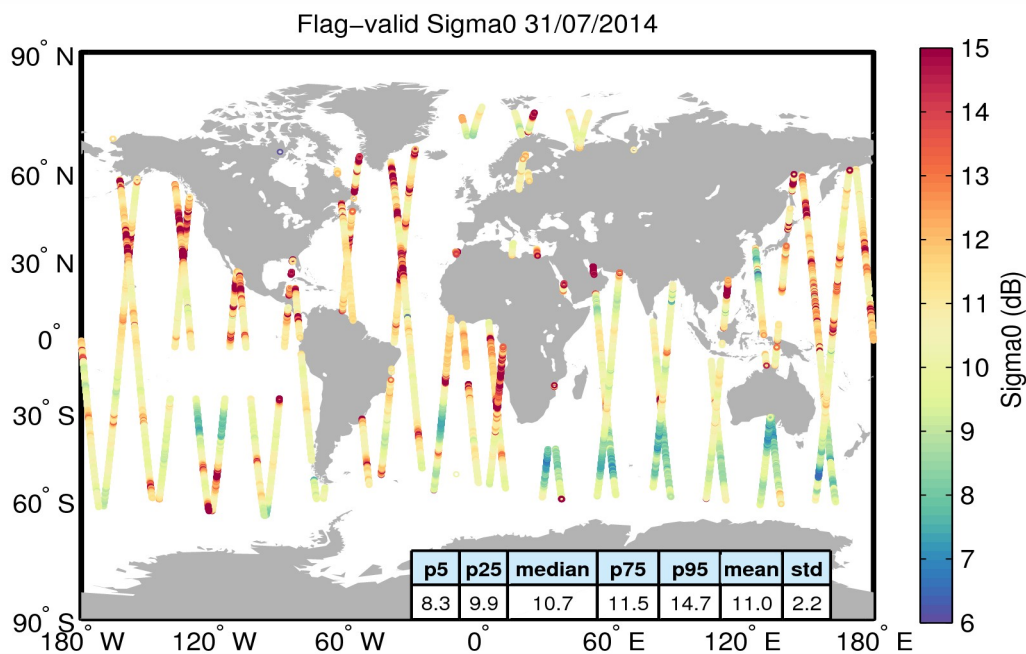
Figure 23. Geographical distribution of flag-valid sigma0 data over oceans and lakes for 31/07/2014. The statistical values shown in the table refer to the sigma0 in dB and are calculated over all measurements shown in the figure.
