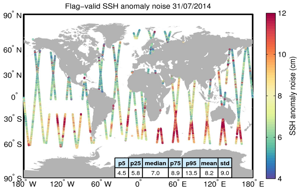
Figure 8. Geographical distribution of flag-valid 20-Hz SSH anomaly measurement noise over oceans and lakes for 31/07/2014. The statistical values shown in the table refer to the SSH anomaly noise and are calculated over all measurements shown in the figure.
