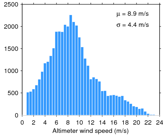
Figure 33. Histogram of flag-valid wind over oceans and lakes for 29/07/2014. The mean ( \mu ) and standard deviation ( \sigma ) are also shown. Note that values larger than 24 m/s are excluded from the histogram for the sake of readability but not from the computation of \mu and \sigma .
