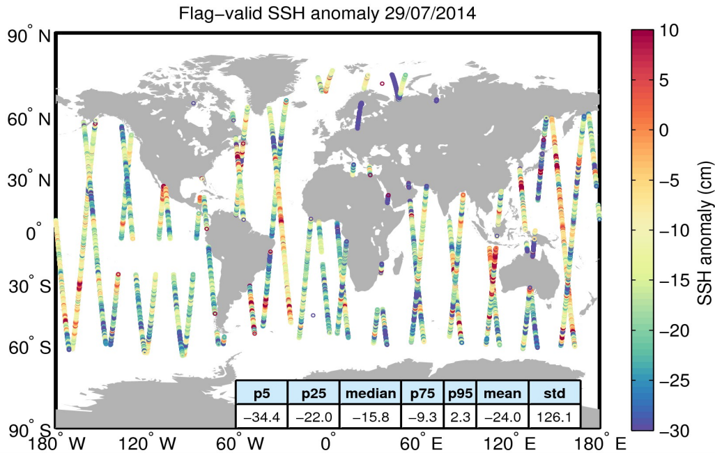
Figure 5. Geographical distribution of flag-valid 1-Hz SSH anomaly data over oceans and lakes for 29/07/2014. The statistical values shown in the table refer to the SSH anomaly in cm and are calculated over all measurements shown in the figure.
