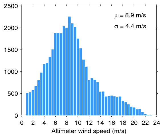
Figure 35. Histogram of science-valid wind over oceans and lakes for 29/07/2014. The mean ( \mu ) and standard deviation ( \sigma ) are also shown. Note that values larger than 24 m/s are excluded from the histogram for the sake of readability but not from the computation of \mu and \sigma .
