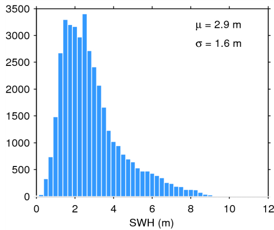
Figure 17. Histogram of flag-valid SWH over oceans and lakes for 29/07/2014. The mean ( \mu ) and standard deviation ( \sigma ) are also shown. Note that values larger than 12 m are excluded from the histogram for the sake of readability but not from the computation of \mu and \sigma .
