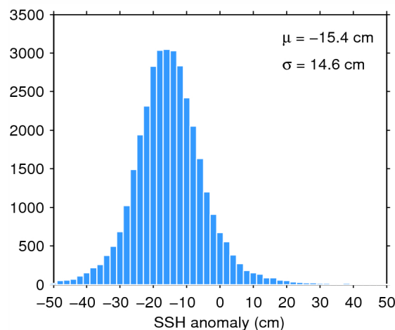
Figure 11. Histogram of science-valid SSH anomaly over oceans and lakes for 29/07/2014. The mean ( \mu ) and standard deviation ( \sigma ) are also shown. Note that values outside [-50 50] cm are excluded from the histogram for the sake of readability but not from the computation of \mu and \sigma .
