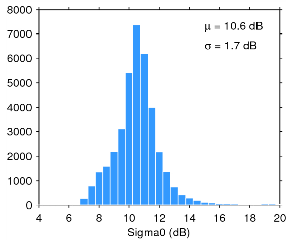
Figure 28. Histogram of science-valid sigma0 over oceans and lakes for 29/07/2014. The mean ( \mu ) and standard deviation ( \sigma ) are also shown. Note that values outside [4 20] dB are excluded from the histogram for the sake of readability but not from the computation of \mu and \sigma .
