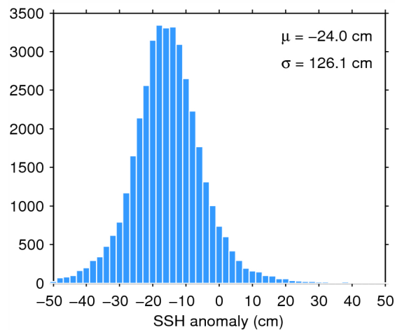
Figure 7. Histogram of flag-valid SSH anomaly over oceans and lakes for 29/07/2014. The mean ( \mu ) and standard deviation ( \sigma ) are also shown. Note that values outside [-50 50] cm are excluded from the histogram for the sake of readability but not from the computation of \mu and \sigma .
