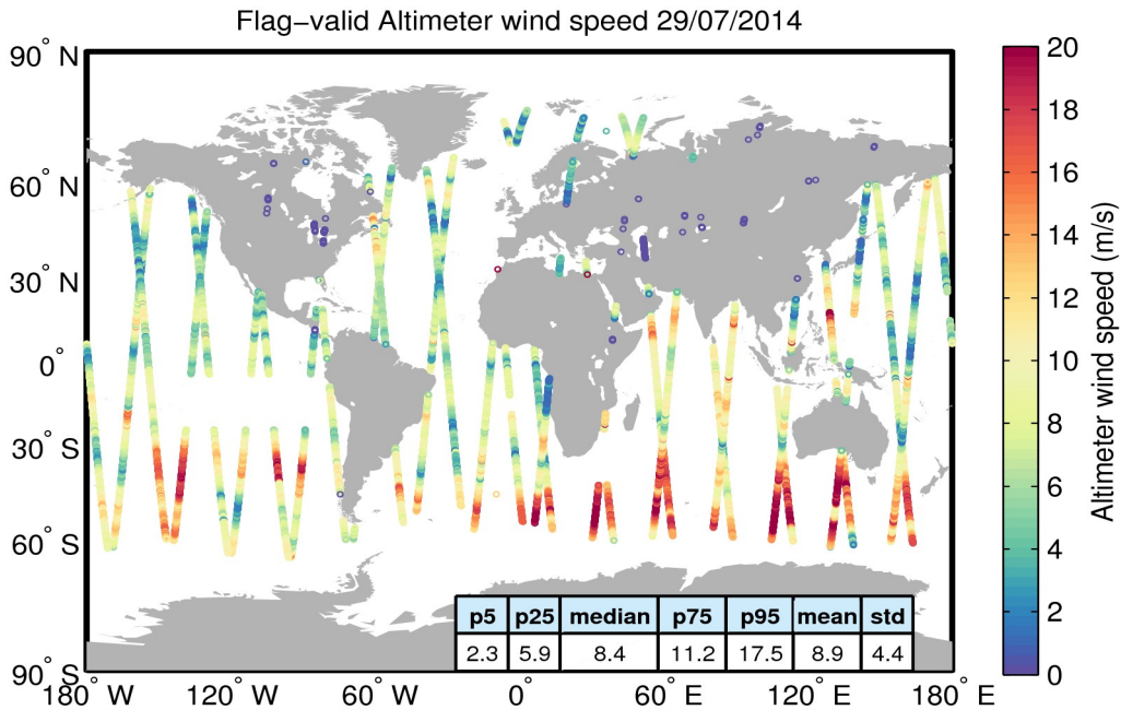
Figure 31. Geographical distribution of flag-valid wind data over oceans and lakes for 29/07/2014. The statistical values shown in the table refer to the wind in m/s and are calculated over all measurements shown in the figure.
