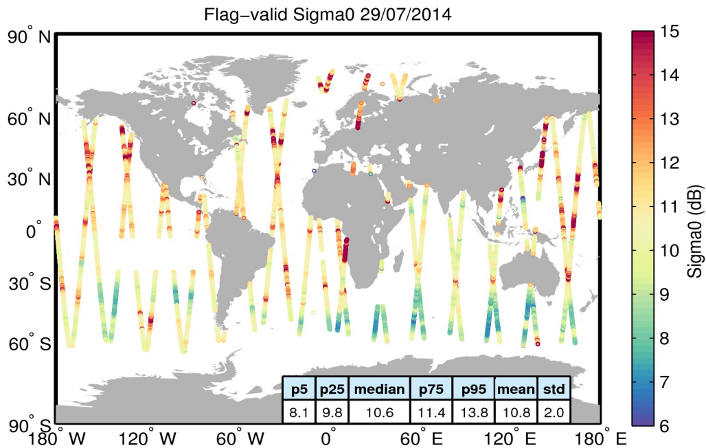
Figure 23. Geographical distribution of flag-valid sigma0 data over oceans and lakes for 29/07/2014. The statistical values shown in the table refer to the sigma0 in dB and are calculated over all measurements shown in the figure.
