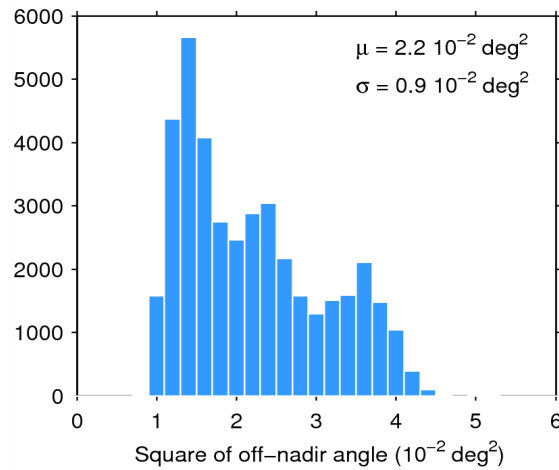
Figure 39. Histogram of flag-valid mispointing over oceans and lakes for 29/07/2014. The mean ( \mu ) and standard deviation ( \sigma ) are also shown. Note that values than 6 \cdot 10^{-2} \text{ deg}^2 are excluded from the histogram for the sake of readability but not from the computation of \mu and \sigma .
