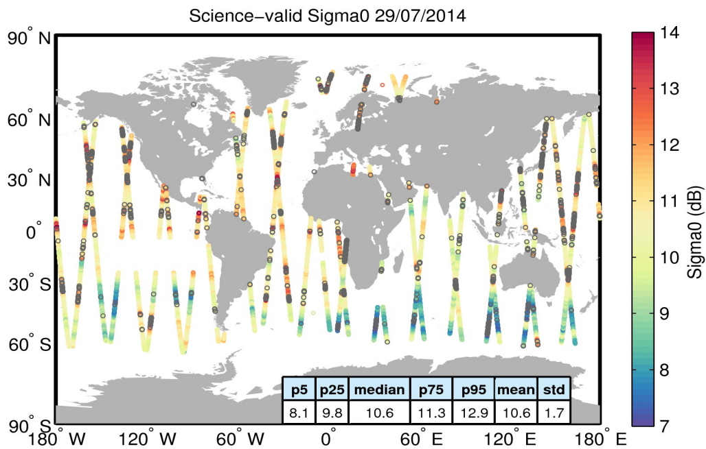
Figure 27. Geographical distribution of science-valid sigma0 data over oceans and lakes for 29/07/2014. The statistical values shown in the table refer to the sigma0 in dB and are calculated over all measurements shown in the figure. Gray circles denote records that have been rejected based on the editing criteria described in Table 4.
