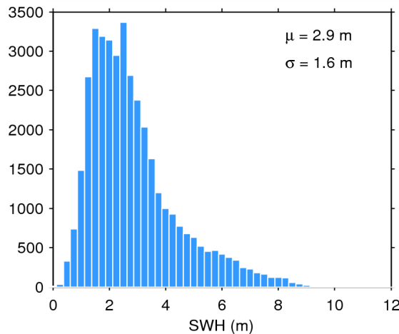
Figure 20. Histogram of science-valid SWH over oceans and lakes for 29/07/2014. The mean ( \mu ) and standard deviation ( \sigma ) are also shown. Note that values larger than 12 m are excluded from the histogram for the sake of readability but not from the computation of \mu and \sigma .
