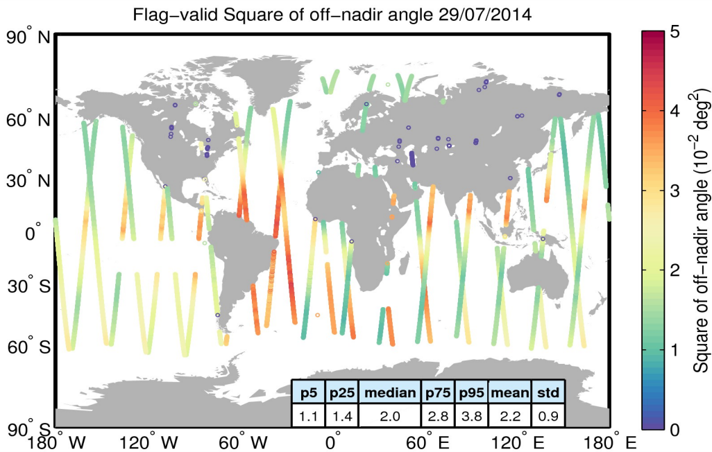
Figure 37. Geographical distribution of flag-valid mispointing data over oceans and lakes for 29/07/2014. The statistical values shown in the table refer to the mispointing in 10^{-2} \text{ deg}^2 and are calculated over all measurements shown in the figure.
