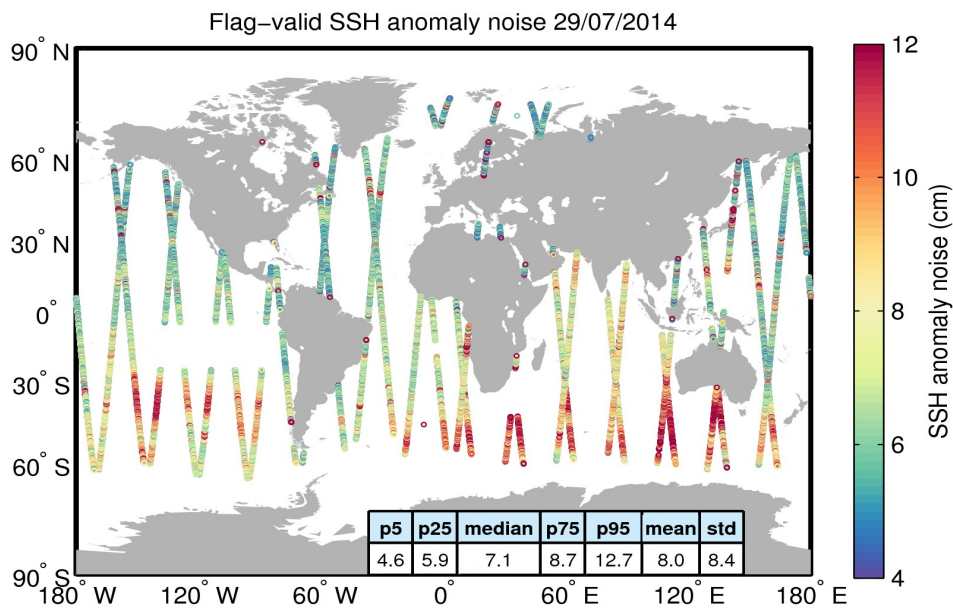
Figure 8. Geographical distribution of flag-valid 20-Hz SSH anomaly measurement noise over oceans and lakes for 29/07/2014. The statistical values shown in the table refer to the SSH anomaly noise and are calculated over all measurements shown in the figure.
