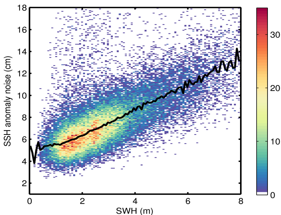
Figure 9. 2D histogram showing flag-valid SSH anomaly noise as a function of SWH for 29/07/2014. The black line denotes the median SSH anomaly as a function of SWH.
