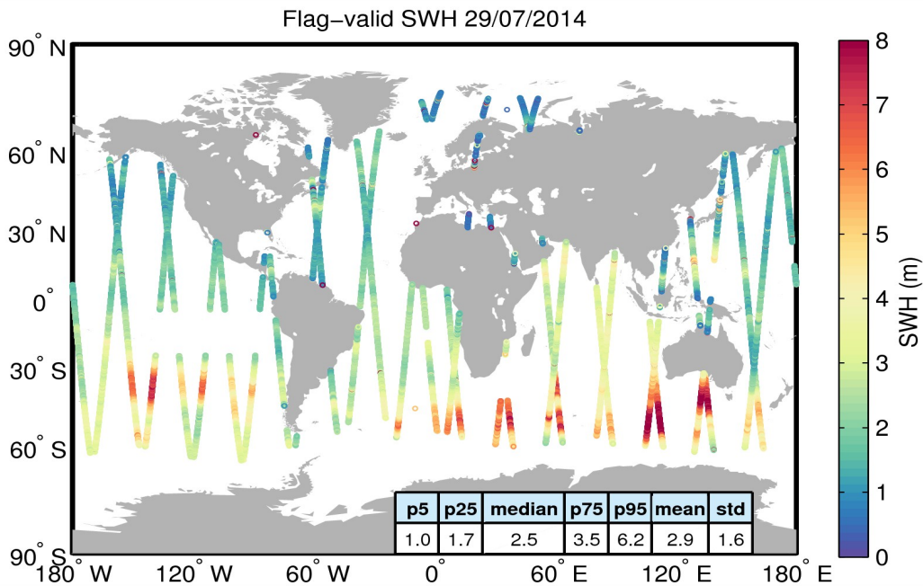
Figure 15. Geographical distribution of flag-valid SWH data over oceans and lakes for 29/07/2014. The statistical values shown in the table refer to the SWH in m and are calculated over all measurements shown in the figure.
