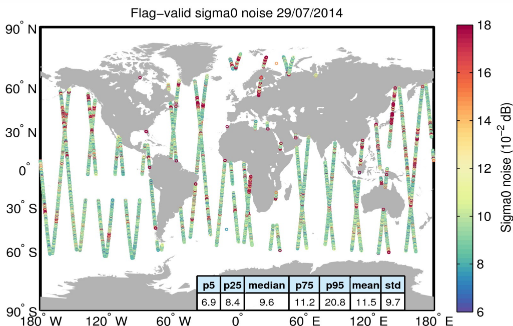
Figure 26. Geographical distribution of flag-valid 20-Hz sigma0 measurement noise over oceans and lakes for 29/07/2014. The statistical values shown in the table refer to the sigma0 noise and are calculated over all measurements shown in the figure.
