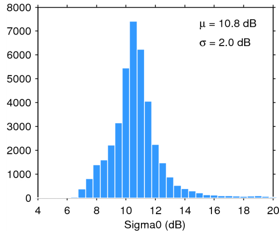
Figure 25. Histogram of flag-valid sigma0 over oceans and lakes for 29/07/2014. The mean ( \mu ) and standard deviation ( \sigma ) are also shown. Note that values outside [4 20] dB are excluded from the histogram for the sake of readability but not from the computation of \mu and \sigma .
