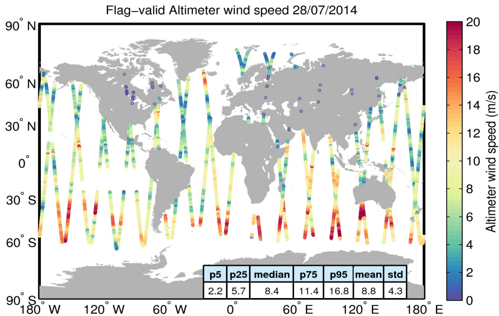
Figure 31. Geographical distribution of flag-valid wind data over oceans and lakes for 28/07/2014. The statistical values shown in the table refer to the wind in m/s and are calculated over all measurements shown in the figure.
