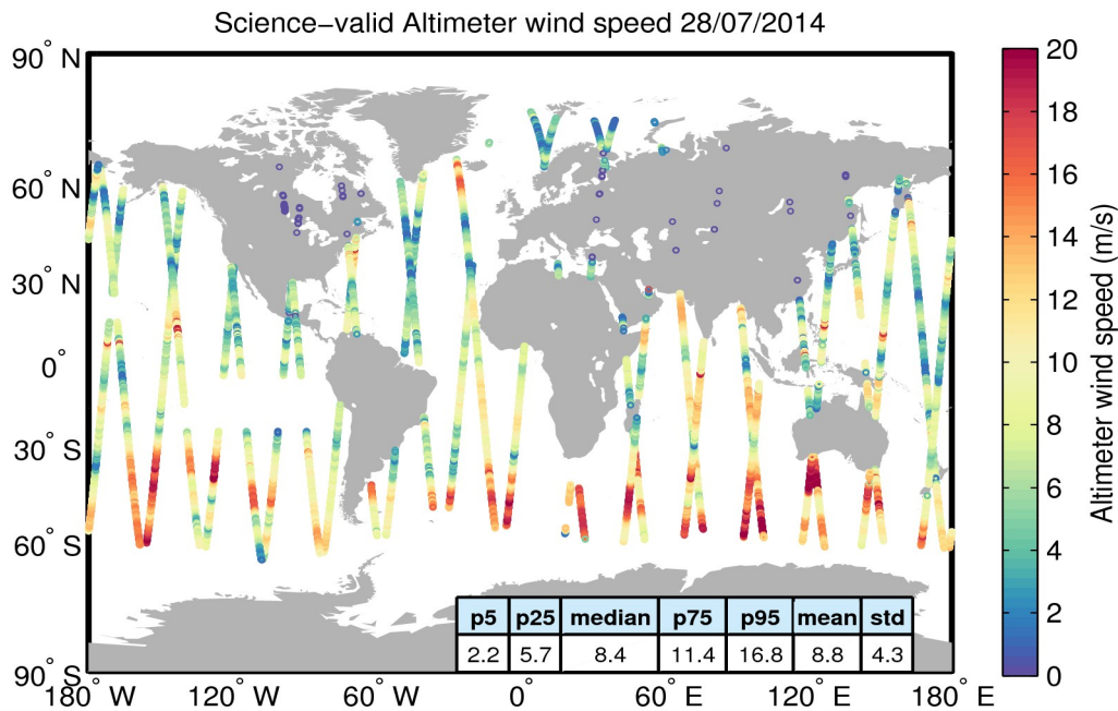
Figure 34. Geographical distribution of science-valid wind data over oceans and lakes for 28/07/2014. The statistical values shown in the table refer to the wind in m/s and are calculated over all measurements shown in the figure. Gray circles denote records that have been rejected based on the editing criteria described in Table 5.
