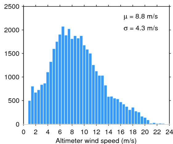
Figure 35. Histogram of science-valid wind over oceans and lakes for 28/07/2014. The mean ( \mu ) and standard deviation ( \sigma ) are also shown. Note that values larger than 24 m/s are excluded from the histogram for the sake of readability but not from the computation of \mu and \sigma .
