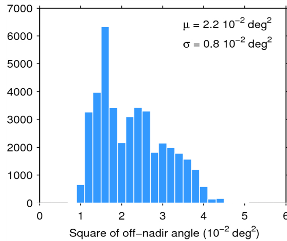
Figure 39. Histogram of flag-valid mispointing over oceans and lakes for 28/07/2014. The mean ( \mu ) and standard deviation ( \sigma ) are also shown. Note that values than 6 \cdot 10^{-2} \text{ deg}^2 are excluded from the histogram for the sake of readability but not from the computation of \mu and \sigma .
