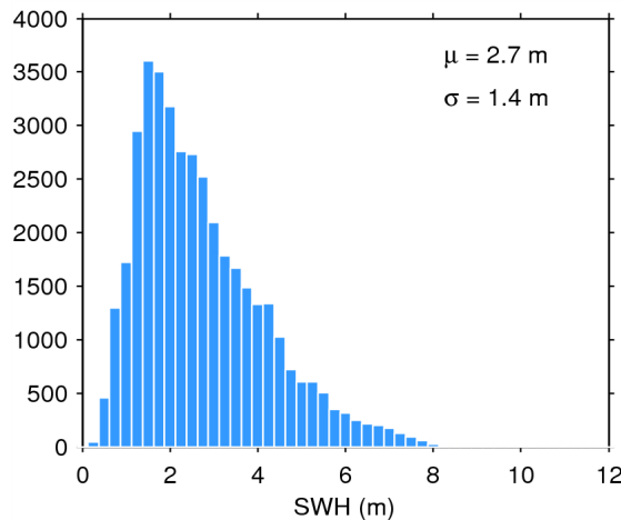
Figure 20. Histogram of science-valid SWH over oceans and lakes for 28/07/2014. The mean ( \mu ) and standard deviation ( \sigma ) are also shown. Note that values larger than 12 m are excluded from the histogram for the sake of readability but not from the computation of \mu and \sigma .
