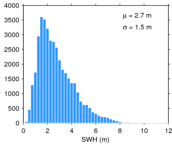
Figure 17. Histogram of flag-valid SWH over oceans and lakes for 28/07/2014. The mean ( \mu ) and standard deviation ( \sigma ) are also shown. Note that values larger than 12 m are excluded from the histogram for the sake of readability but not from the computation of \mu and \sigma .
