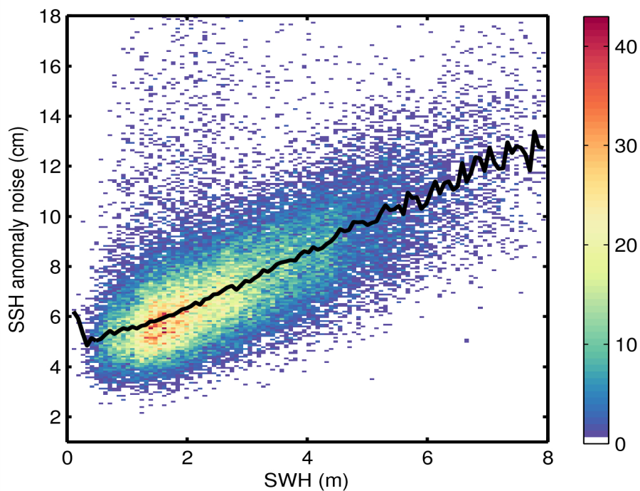
Figure 9. 2D histogram showing flag-valid SSH anomaly noise as a function of SWH for 28/07/2014. The black line denotes the median SSH anomaly as a function of SWH.
