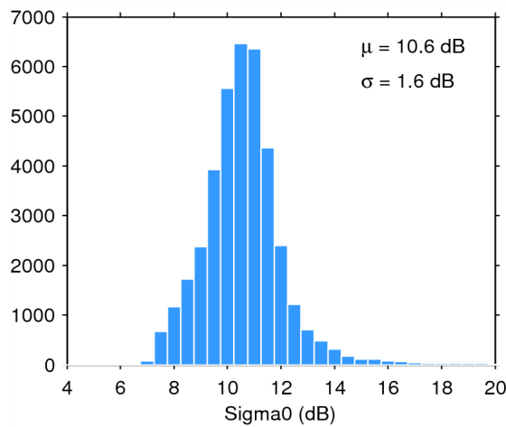
Figure 28. Histogram of science-valid sigma0 over oceans and lakes for 28/07/2014. The mean ( \mu ) and standard deviation ( \sigma ) are also shown. Note that values outside [4 20] dB are excluded from the histogram for the sake of readability but not from the computation of \mu and \sigma .
