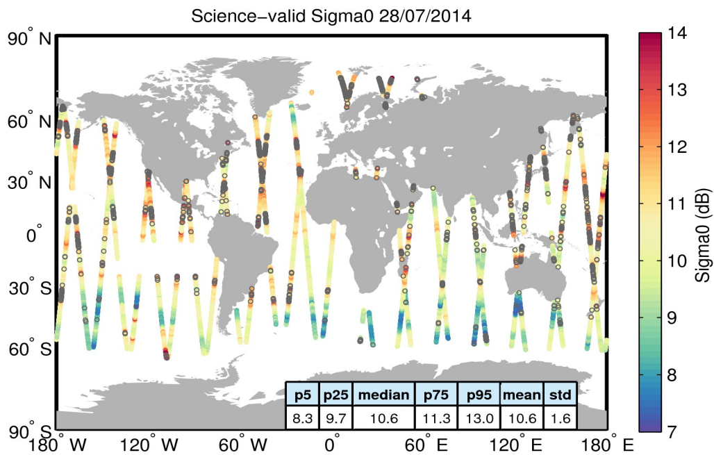
Figure 27. Geographical distribution of science-valid sigma0 data over oceans and lakes for 28/07/2014. The statistical values shown in the table refer to the sigma0 in dB and are calculated over all measurements shown in the figure. Gray circles denote records that have been rejected based on the editing criteria described in Table 4.
