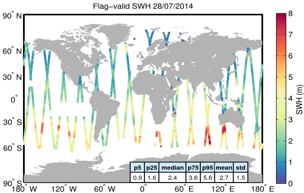
Figure 15. Geographical distribution of flag-valid SWH data over oceans and lakes for 28/07/2014. The statistical values shown in the table refer to the SWH in m and are calculated over all measurements shown in the figure.
