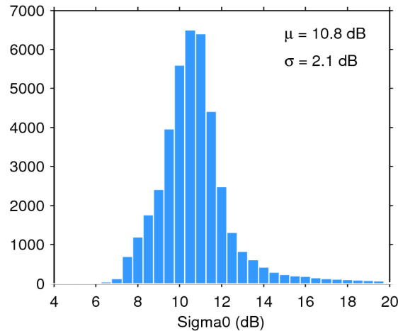
Figure 25. Histogram of flag-valid sigma0 over oceans and lakes for 28/07/2014. The mean ( \mu ) and standard deviation ( \sigma ) are also shown. Note that values outside [4 20] dB are excluded from the histogram for the sake of readability but not from the computation of \mu and \sigma .
