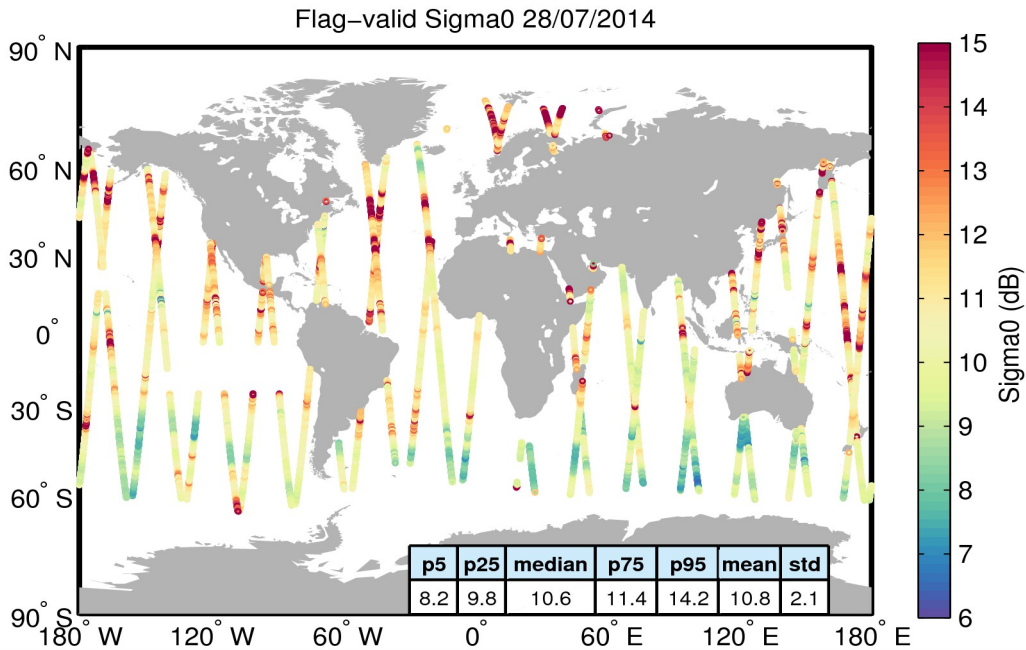
Figure 23. Geographical distribution of flag-valid sigma0 data over oceans and lakes for 28/07/2014. The statistical values shown in the table refer to the sigma0 in dB and are calculated over all measurements shown in the figure.
