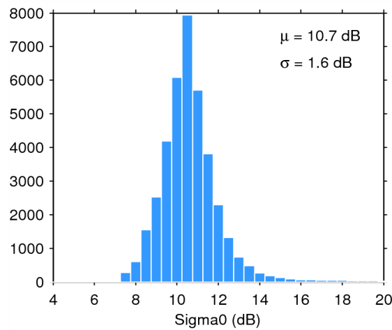
Figure 28. Histogram of science-valid sigma0 over oceans and lakes for 26/07/2014. The mean ( \mu ) and standard deviation ( \sigma ) are also shown. Note that values outside [4 20] dB are excluded from the histogram for the sake of readability but not from the computation of \mu and \sigma .
