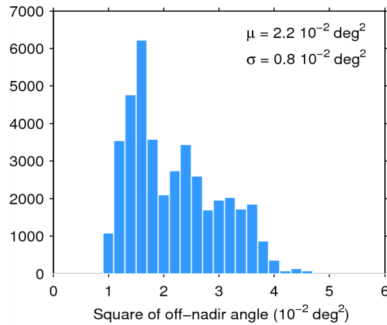
Figure 39. Histogram of flag-valid mispointing over oceans and lakes for 26/07/2014. The mean ( \mu ) and standard deviation ( \sigma ) are also shown. Note that values than 6 \cdot 10^{-2} \text{ deg}^2 are excluded from the histogram for the sake of readability but not from the computation of \mu and \sigma .
