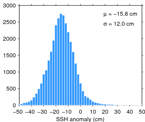
Figure 11. Histogram of science-valid SSH anomaly over oceans and lakes for 26/07/2014. The mean ( \mu ) and standard deviation ( \sigma ) are also shown. Note that values outside [-50 50] cm are excluded from the histogram for the sake of readability but not from the computation of \mu and \sigma .
