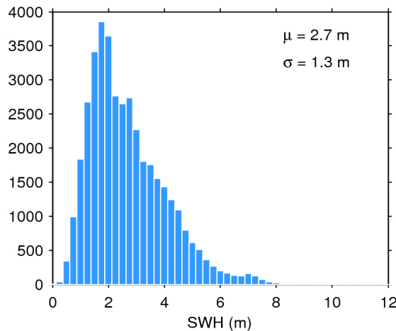
Figure 20. Histogram of science-valid SWH over oceans and lakes for 26/07/2014. The mean ( \mu ) and standard deviation ( \sigma ) are also shown. Note that values larger than 12 m are excluded from the histogram for the sake of readability but not from the computation of \mu and \sigma .
