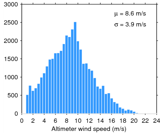
Figure 33. Histogram of flag-valid wind over oceans and lakes for 26/07/2014. The mean ( \mu ) and standard deviation ( \sigma ) are also shown. Note that values larger than 24 m/s are excluded from the histogram for the sake of readability but not from the computation of \mu and \sigma .
