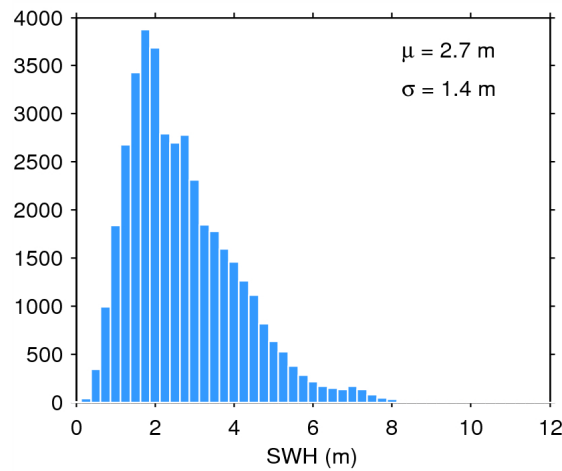
Figure 17. Histogram of flag-valid SWH over oceans and lakes for 26/07/2014. The mean ( \mu ) and standard deviation ( \sigma ) are also shown. Note that values larger than 12 m are excluded from the histogram for the sake of readability but not from the computation of \mu and \sigma .
