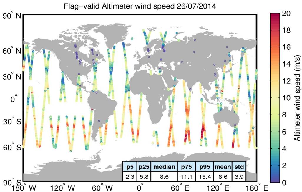
Figure 31. Geographical distribution of flag-valid wind data over oceans and lakes for 26/07/2014. The statistical values shown in the table refer to the wind in m/s and are calculated over all measurements shown in the figure.
