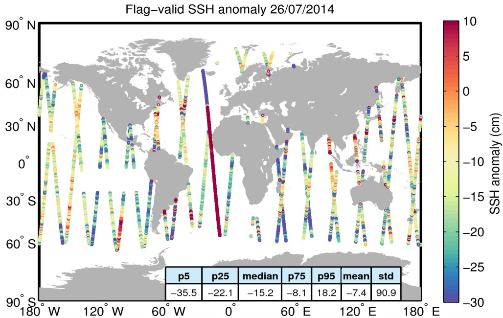
Figure 5. Geographical distribution of flag-valid 1-Hz SSH anomaly data over oceans and lakes for 26/07/2014. The statistical values shown in the table refer to the SSH anomaly in cm and are calculated over all measurements shown in the figure.
