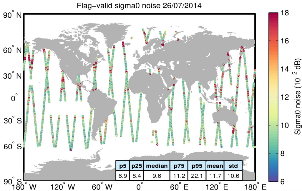
Figure 26. Geographical distribution of flag-valid 20-Hz sigma0 measurement noise over oceans and lakes for 26/07/2014. The statistical values shown in the table refer to the sigma0 noise and are calculated over all measurements shown in the figure.
