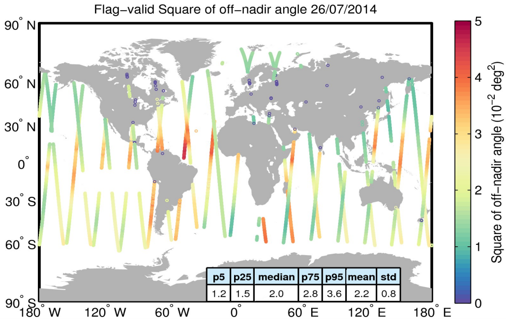
Figure 37. Geographical distribution of flag-valid mispointing data over oceans and lakes for 26/07/2014. The statistical values shown in the table refer to the mispointing in 10^{-2} deg 2 and are calculated over all measurements shown in the figure.
