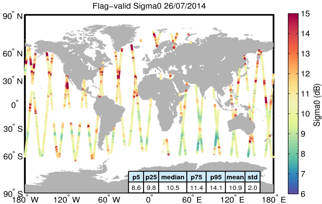
Figure 23. Geographical distribution of flag-valid sigma0 data over oceans and lakes for 26/07/2014. The statistical values shown in the table refer to the sigma0 in dB and are calculated over all measurements shown in the figure.
