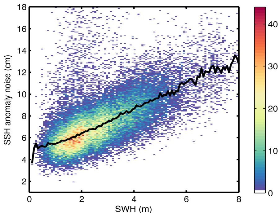
Figure 9. 2D histogram showing flag-valid SSH anomaly noise as a function of SWH for 26/07/2014. The black line denotes the median SSH anomaly as a function of SWH.
