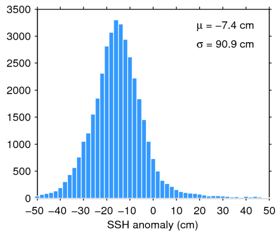
Figure 7. Histogram of flag-valid SSH anomaly over oceans and lakes for 26/07/2014. The mean ( \mu ) and standard deviation ( \sigma ) are also shown. Note that values outside [-50 50] cm are excluded from the histogram for the sake of readability but not from the computation of \mu and \sigma .
