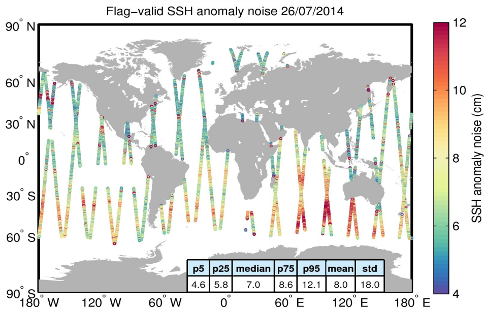
Figure 8. Geographical distribution of flag-valid 20-Hz SSH anomaly measurement noise over oceans and lakes for 26/07/2014. The statistical values shown in the table refer to the SSH anomaly noise and are calculated over all measurements shown in the figure.
