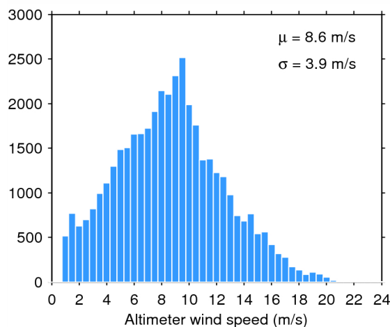
Figure 35. Histogram of science-valid wind over oceans and lakes for 26/07/2014. The mean ( \mu ) and standard deviation ( \sigma ) are also shown. Note that values larger than 24 m/s are excluded from the histogram for the sake of readability but not from the computation of \mu and \sigma .
