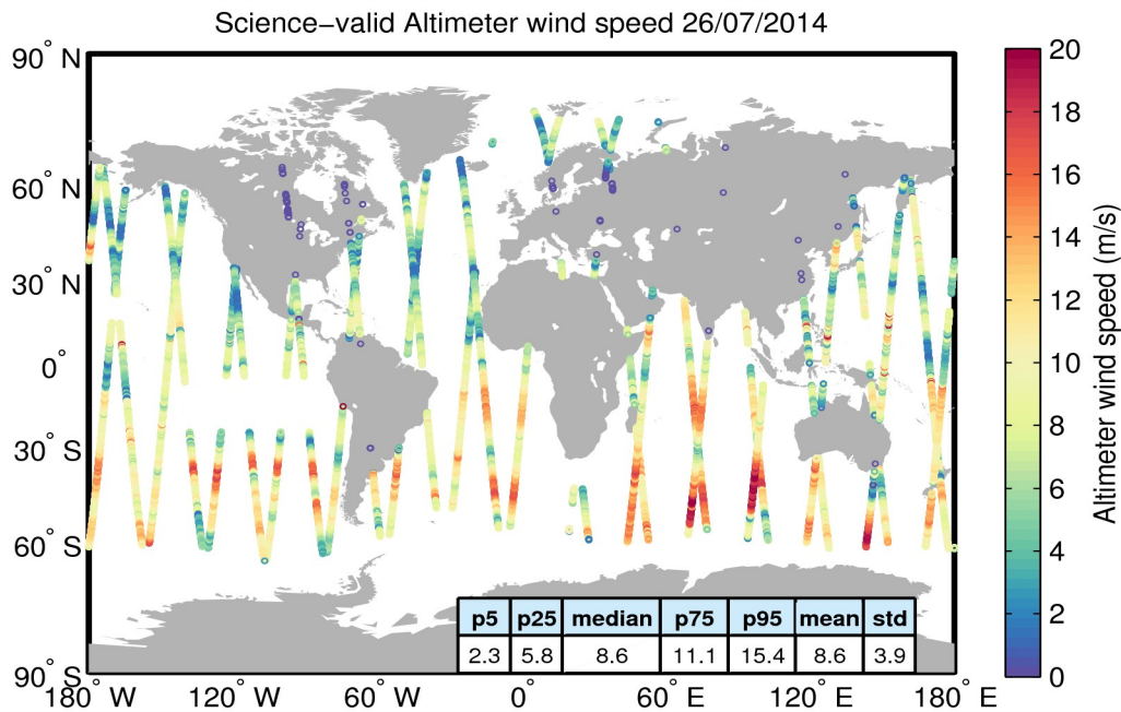
Figure 34. Geographical distribution of science-valid wind data over oceans and lakes for 26/07/2014. The statistical values shown in the table refer to the wind in m/s and are calculated over all measurements shown in the figure. Gray circles denote records that have been rejected based on the editing criteria described in Table 5.
