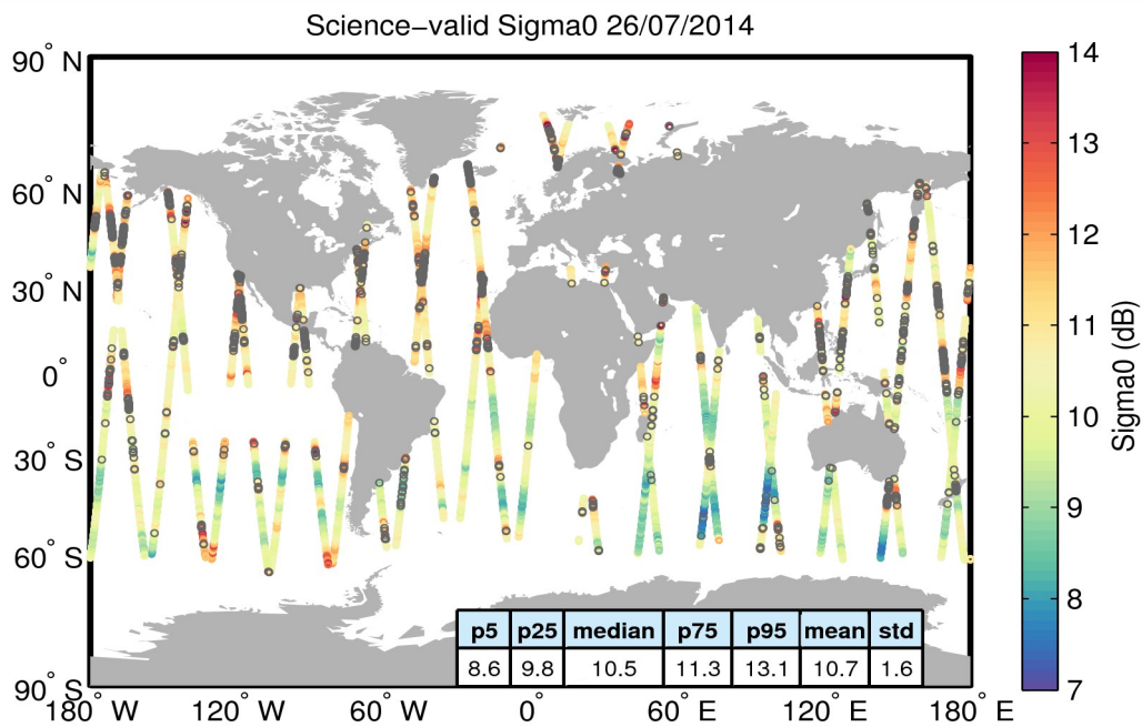
Figure 27. Geographical distribution of science-valid sigma0 data over oceans and lakes for 26/07/2014. The statistical values shown in the table refer to the sigma0 in dB and are calculated over all measurements shown in the figure. Gray circles denote records that have been rejected based on the editing criteria described in Table 4.
