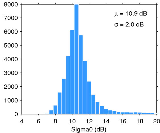
Figure 25. Histogram of flag-valid sigma0 over oceans and lakes for 26/07/2014. The mean ( \mu ) and standard deviation ( \sigma ) are also shown. Note that values outside [4 20] dB are excluded from the histogram for the sake of readability but not from the computation of \mu and \sigma .
