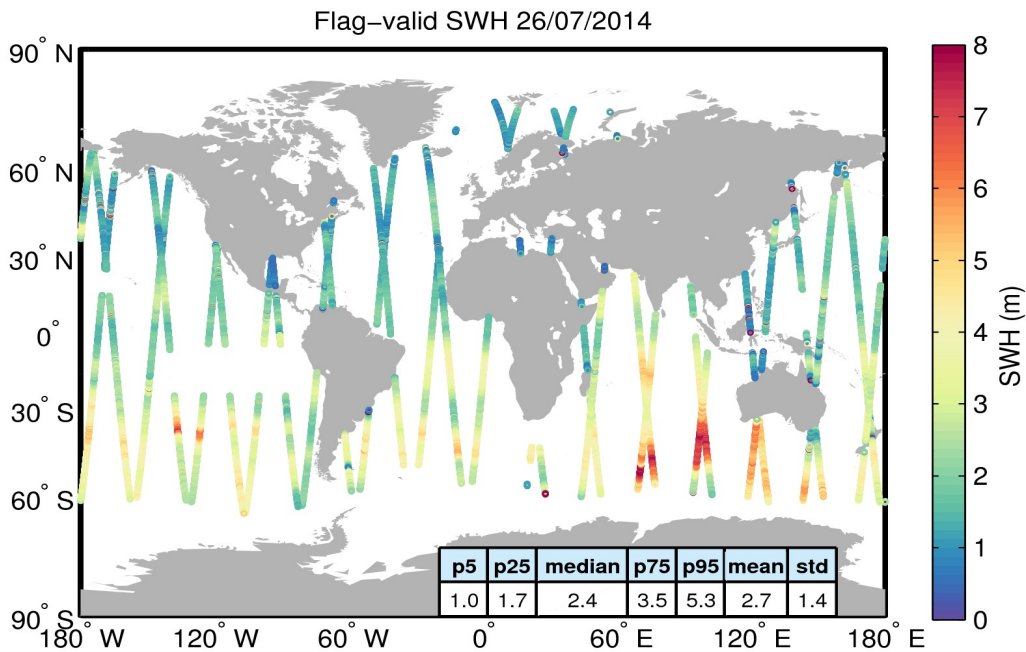
Figure 15. Geographical distribution of flag-valid SWH data over oceans and lakes for 26/07/2014. The statistical values shown in the table refer to the SWH in m and are calculated over all measurements shown in the figure.
