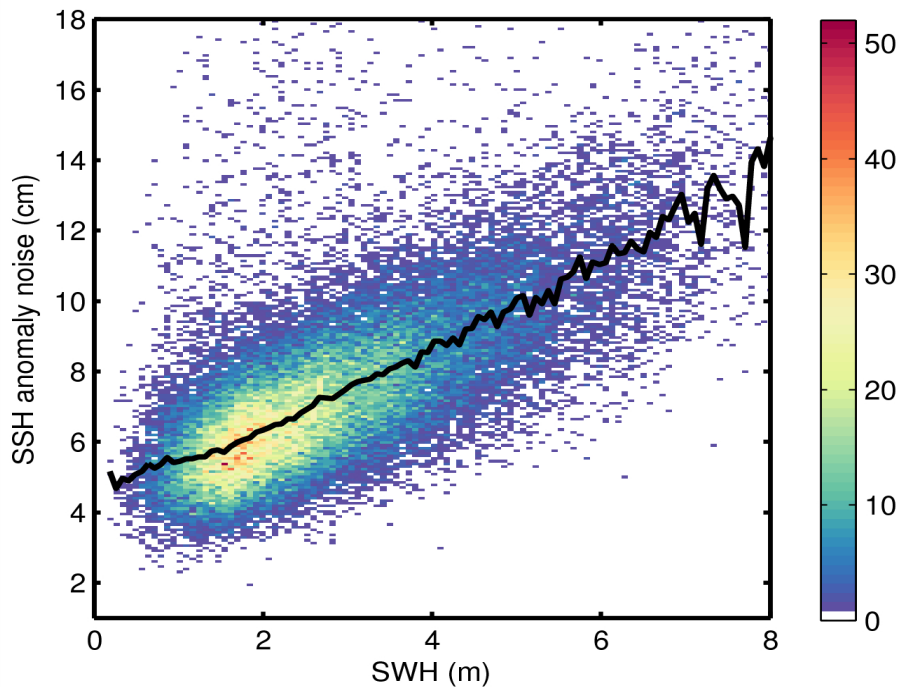
Figure 9. 2D histogram showing flag-valid SSH anomaly noise as a function of SWH for 25/07/2014. The black line denotes the median SSH anomaly as a function of SWH.
