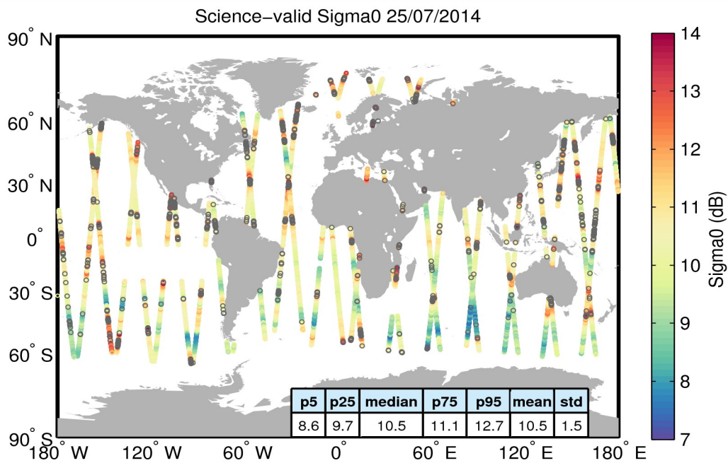
Figure 27. Geographical distribution of science-valid sigma0 data over oceans and lakes for 25/07/2014. The statistical values shown in the table refer to the sigma0 in dB and are calculated over all measurements shown in the figure. Gray circles denote records that have been rejected based on the editing criteria described in Table 4.
