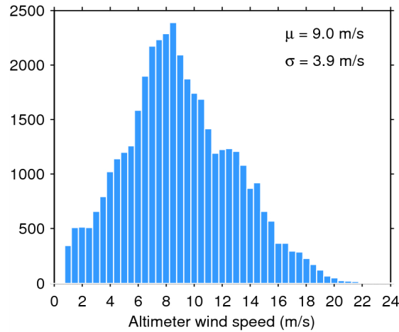
Figure 33. Histogram of flag-valid wind over oceans and lakes for 25/07/2014. The mean ( \mu ) and standard deviation ( \sigma ) are also shown. Note that values larger than 24 m/s are excluded from the histogram for the sake of readability but not from the computation of \mu and \sigma .
