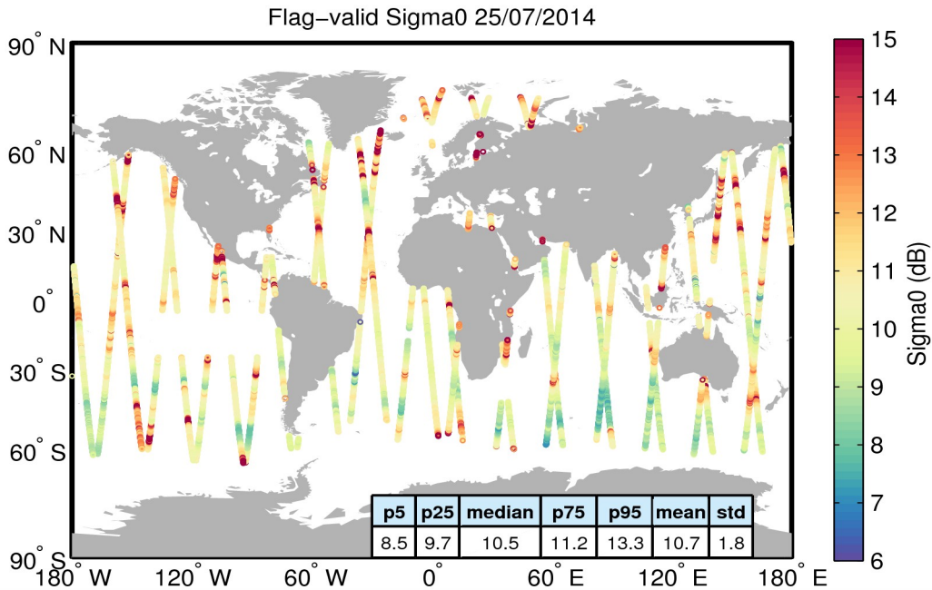
Figure 23. Geographical distribution of flag-valid sigma0 data over oceans and lakes for 25/07/2014. The statistical values shown in the table refer to the sigma0 in dB and are calculated over all measurements shown in the figure.
