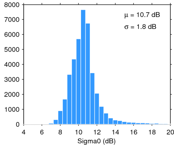
Figure 25. Histogram of flag-valid sigma0 over oceans and lakes for 25/07/2014. The mean ( \mu ) and standard deviation ( \sigma ) are also shown. Note that values outside [4 20] dB are excluded from the histogram for the sake of readability but not from the computation of \mu and \sigma .
