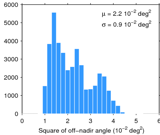
Figure 39. Histogram of flag-valid mispointing over oceans and lakes for 25/07/2014. The mean ( \mu ) and standard deviation ( \sigma ) are also shown. Note that values than 6 \cdot 10^{-2} \text{ deg}^2 are excluded from the histogram for the sake of readability but not from the computation of \mu and \sigma .
