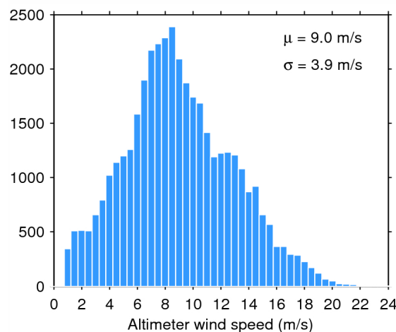
Figure 35. Histogram of science-valid wind over oceans and lakes for 25/07/2014. The mean ( \mu ) and standard deviation ( \sigma ) are also shown. Note that values larger than 24 m/s are excluded from the histogram for the sake of readability but not from the computation of \mu and \sigma .
