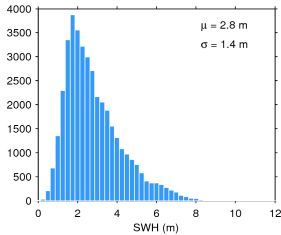
Figure 17. Histogram of flag-valid SWH over oceans and lakes for 25/07/2014. The mean ( \mu ) and standard deviation ( \sigma ) are also shown. Note that values larger than 12 m are excluded from the histogram for the sake of readability but not from the computation of \mu and \sigma .
