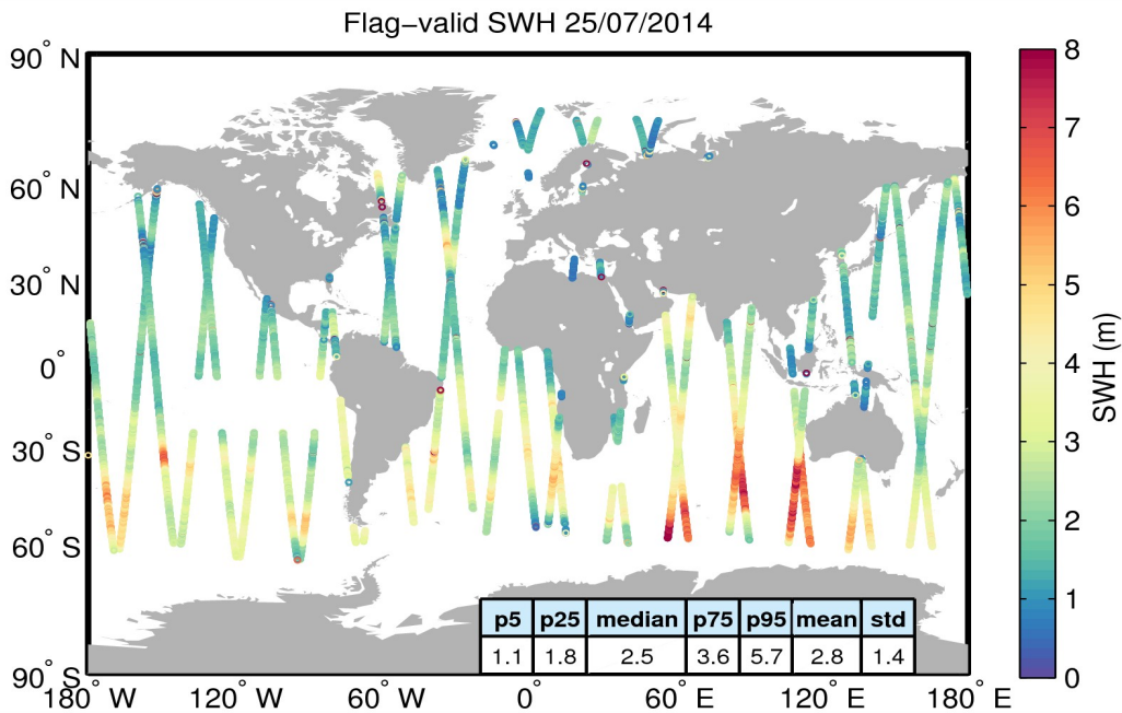
Figure 15. Geographical distribution of flag-valid SWH data over oceans and lakes for 25/07/2014. The statistical values shown in the table refer to the SWH in m and are calculated over all measurements shown in the figure.
