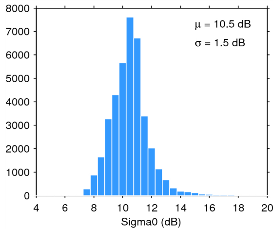
Figure 28. Histogram of science-valid sigma0 over oceans and lakes for 25/07/2014. The mean ( \mu ) and standard deviation ( \sigma ) are also shown. Note that values outside [4 20] dB are excluded from the histogram for the sake of readability but not from the computation of \mu and \sigma .
