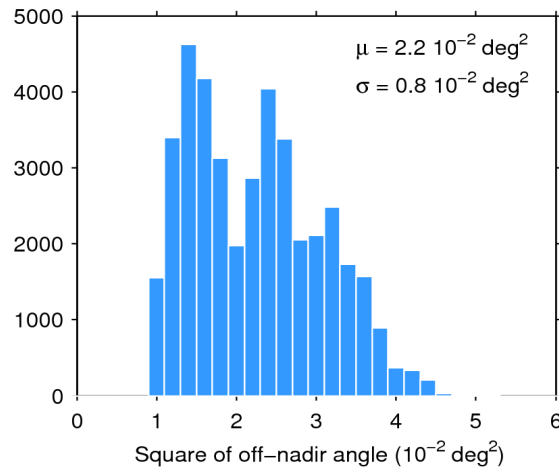
Figure 39. Histogram of flag-valid mispointing over oceans and lakes for 24/07/2014. The mean ( \mu ) and standard deviation ( \sigma ) are also shown. Note that values than 6 \cdot 10^{-2} \text{ deg}^2 are excluded from the histogram for the sake of readability but not from the computation of \mu and \sigma .
