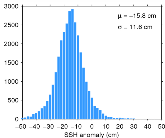
Figure 11. Histogram of science-valid SSH anomaly over oceans and lakes for 24/07/2014. The mean ( \mu ) and standard deviation ( \sigma ) are also shown. Note that values outside [-50 50] cm are excluded from the histogram for the sake of readability but not from the computation of \mu and \sigma .
