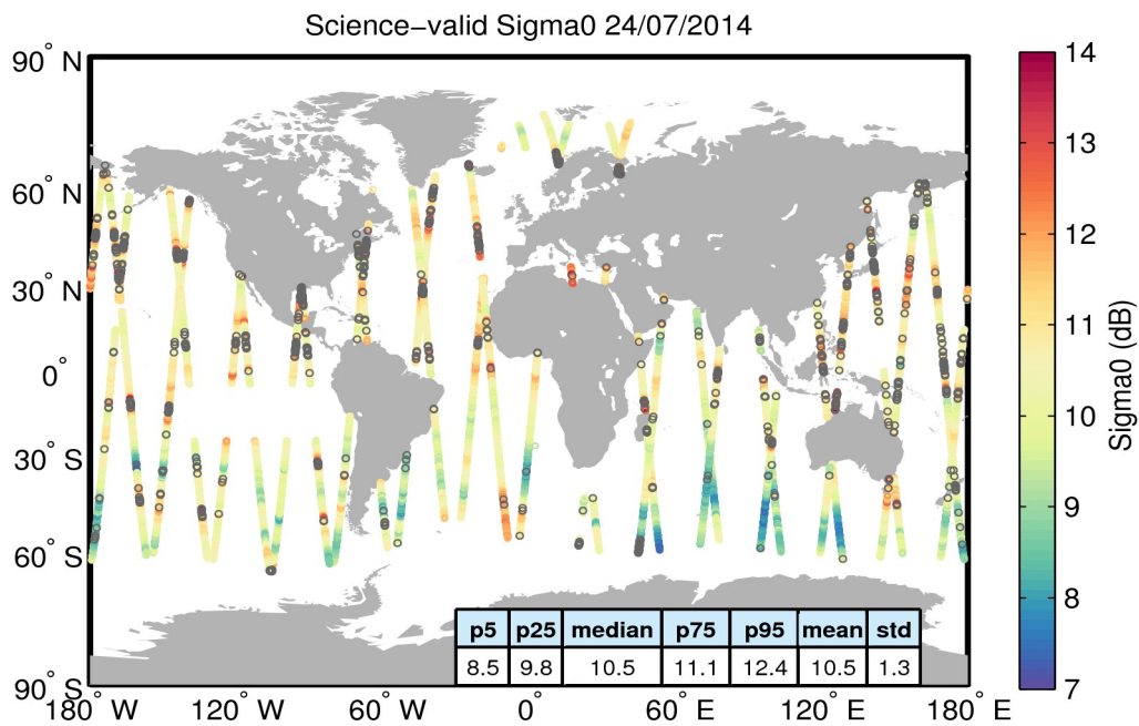
Figure 27. Geographical distribution of science-valid sigma0 data over oceans and lakes for 24/07/2014. The statistical values shown in the table refer to the sigma0 in dB and are calculated over all measurements shown in the figure. Gray circles denote records that have been rejected based on the editing criteria described in Table 4.
