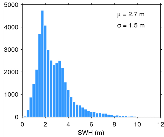
Figure 17. Histogram of flag-valid SWH over oceans and lakes for 24/07/2014. The mean ( \mu ) and standard deviation ( \sigma ) are also shown. Note that values larger than 12 m are excluded from the histogram for the sake of readability but not from the computation of \mu and \sigma .
