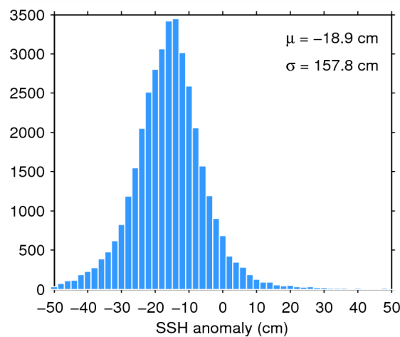
Figure 7. Histogram of flag-valid SSH anomaly over oceans and lakes for 24/07/2014. The mean ( \mu ) and standard deviation ( \sigma ) are also shown. Note that values outside [-50 50] cm are excluded from the histogram for the sake of readability but not from the computation of \mu and \sigma .
