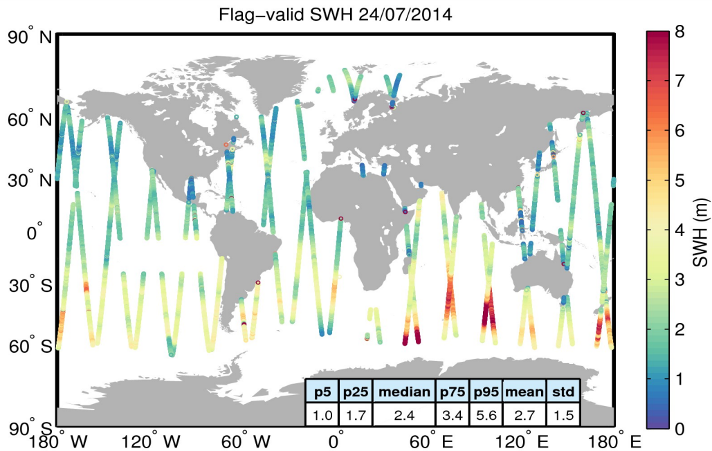
Figure 15. Geographical distribution of flag-valid SWH data over oceans and lakes for 24/07/2014. The statistical values shown in the table refer to the SWH in m and are calculated over all measurements shown in the figure.
