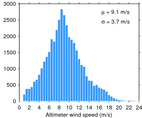
Figure 33. Histogram of flag-valid wind over oceans and lakes for 24/07/2014. The mean ( \mu ) and standard deviation ( \sigma ) are also shown. Note that values larger than 24 m/s are excluded from the histogram for the sake of readability but not from the computation of \mu and \sigma .
