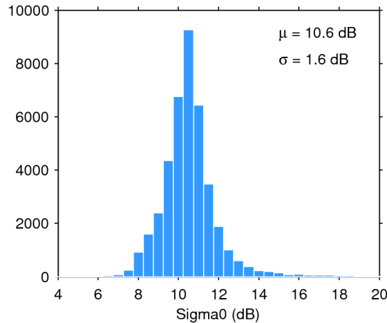
Figure 25. Histogram of flag-valid sigma0 over oceans and lakes for 24/07/2014. The mean ( \mu ) and standard deviation ( \sigma ) are also shown. Note that values outside [4 20] dB are excluded from the histogram for the sake of readability but not from the computation of \mu and \sigma .
