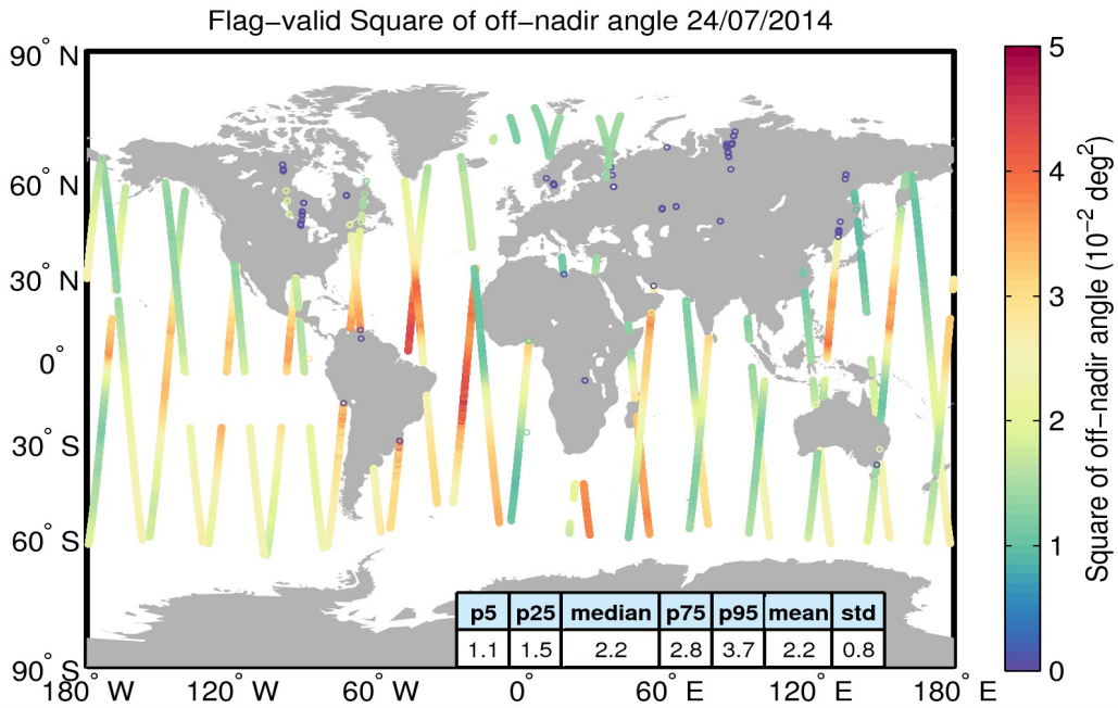
Figure 37. Geographical distribution of flag-valid mispointing data over oceans and lakes for 24/07/2014. The statistical values shown in the table refer to the mispointing in 10^{-2} \text{ deg}^2 and are calculated over all measurements shown in the figure.
