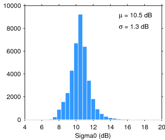
Figure 28. Histogram of science-valid sigma0 over oceans and lakes for 24/07/2014. The mean ( \mu ) and standard deviation ( \sigma ) are also shown. Note that values outside [4 20] dB are excluded from the histogram for the sake of readability but not from the computation of \mu and \sigma .
