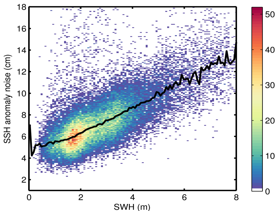
Figure 9. 2D histogram showing flag-valid SSH anomaly noise as a function of SWH for 24/07/2014. The black line denotes the median SSH anomaly as a function of SWH.
