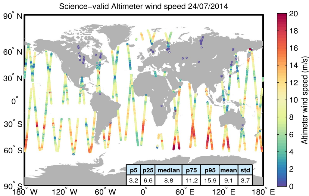
Figure 34. Geographical distribution of science-valid wind data over oceans and lakes for 24/07/2014. The statistical values shown in the table refer to the wind in m/s and are calculated over all measurements shown in the figure. Gray circles denote records that have been rejected based on the editing criteria described in Table 5.
