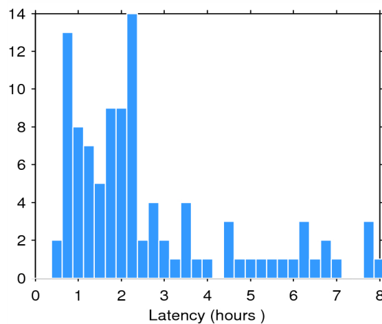
Figure 2. Histogram of the data latency for 24/07/2014. The y-axis denotes the number of files that are made available with a delay of x-hours with respect to the mean time of the records stored in the file.
