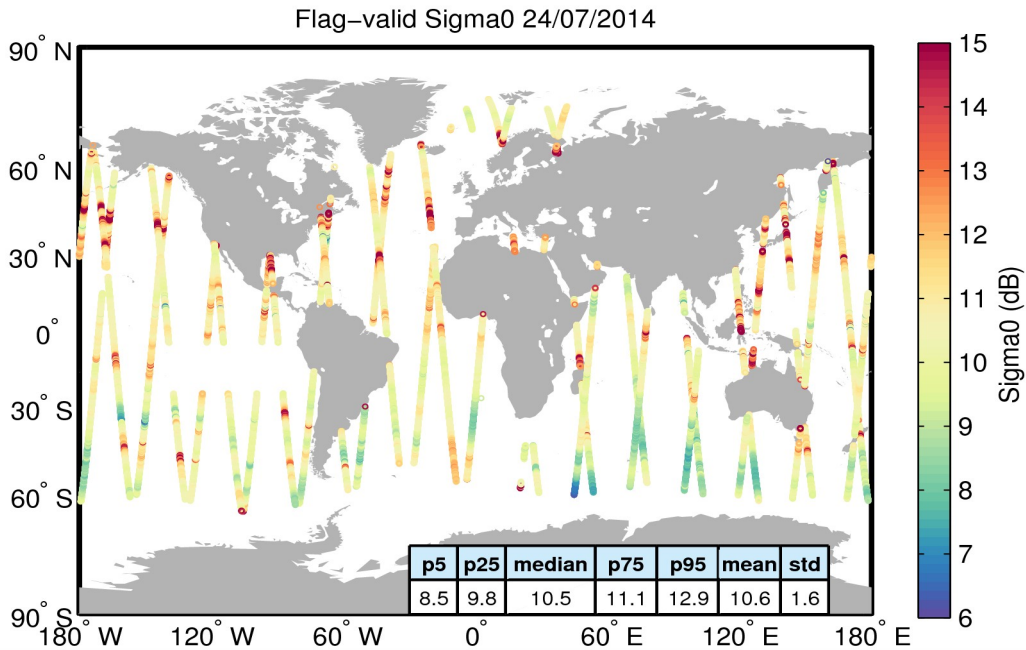
Figure 23. Geographical distribution of flag-valid sigma0 data over oceans and lakes for 24/07/2014. The statistical values shown in the table refer to the sigma0 in dB and are calculated over all measurements shown in the figure.
