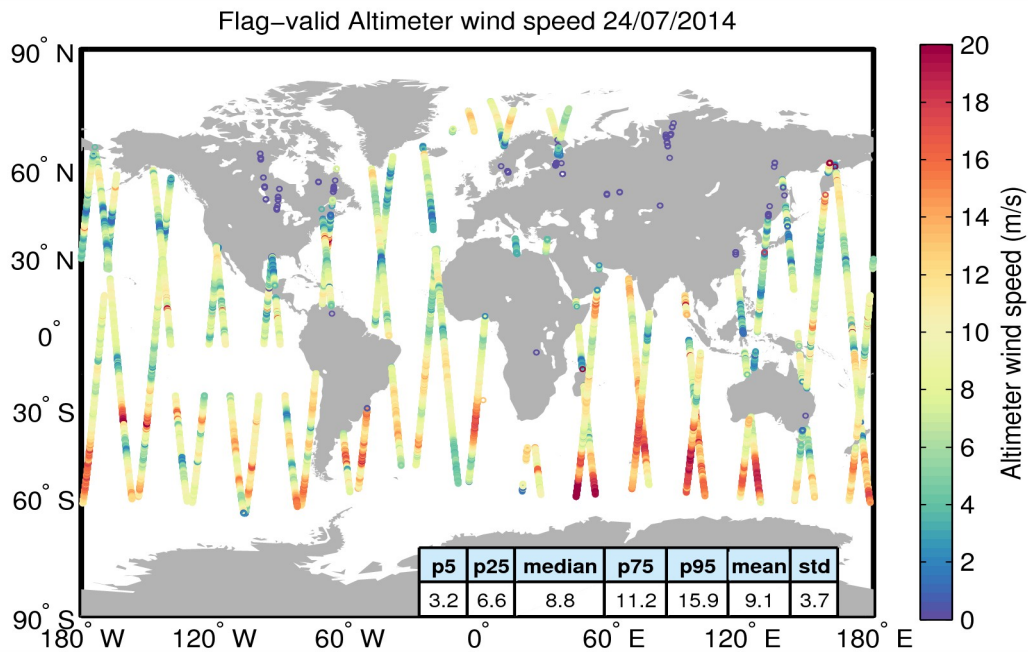
Figure 31. Geographical distribution of flag-valid wind data over oceans and lakes for 24/07/2014. The statistical values shown in the table refer to the wind in m/s and are calculated over all measurements shown in the figure.
