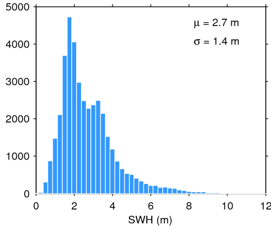
Figure 20. Histogram of science-valid SWH over oceans and lakes for 24/07/2014. The mean ( \mu ) and standard deviation ( \sigma ) are also shown. Note that values larger than 12 m are excluded from the histogram for the sake of readability but not from the computation of \mu and \sigma .
