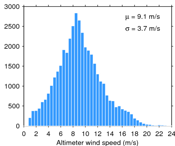
Figure 35. Histogram of science-valid wind over oceans and lakes for 24/07/2014. The mean ( \mu ) and standard deviation ( \sigma ) are also shown. Note that values larger than 24 m/s are excluded from the histogram for the sake of readability but not from the computation of \mu and \sigma .
