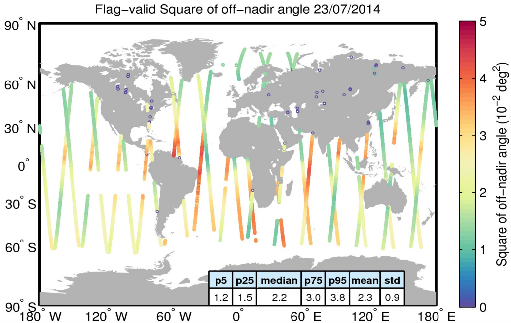
Figure 37. Geographical distribution of flag-valid mispointing data over oceans and lakes for 23/07/2014. The statistical values shown in the table refer to the mispointing in 10^{-2} \text{ deg}^2 and are calculated over all measurements shown in the figure.
