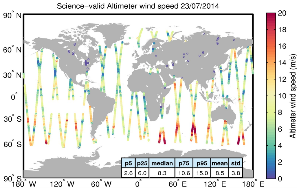
Figure 34. Geographical distribution of science-valid wind data over oceans and lakes for 23/07/2014. The statistical values shown in the table refer to the wind in m/s and are calculated over all measurements shown in the figure. Gray circles denote records that have been rejected based on the editing criteria described in Table 5.
