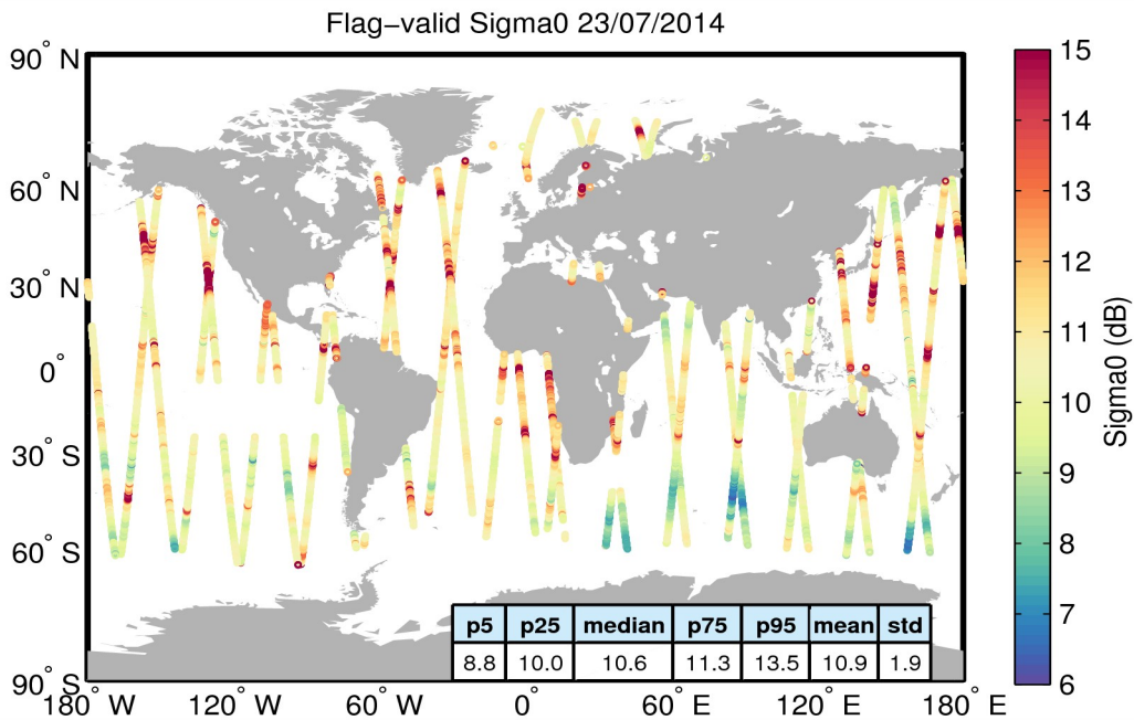
Figure 23. Geographical distribution of flag-valid sigma0 data over oceans and lakes for 23/07/2014. The statistical values shown in the table refer to the sigma0 in dB and are calculated over all measurements shown in the figure.
