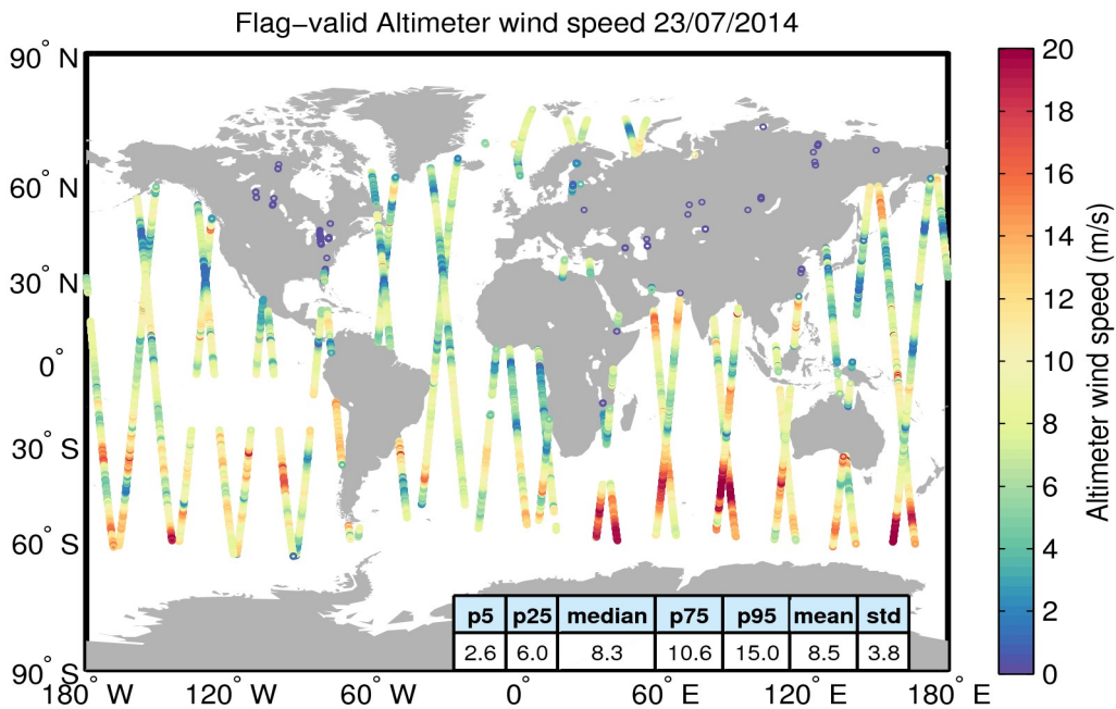
Figure 31. Geographical distribution of flag-valid wind data over oceans and lakes for 23/07/2014. The statistical values shown in the table refer to the wind in m/s and are calculated over all measurements shown in the figure.
