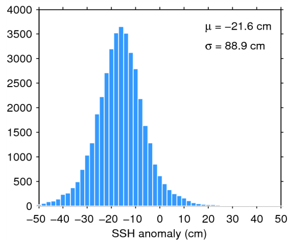
Figure 7. Histogram of flag-valid SSH anomaly over oceans and lakes for 23/07/2014. The mean ( \mu ) and standard deviation ( \sigma ) are also shown. Note that values outside [-50 50] cm are excluded from the histogram for the sake of readability but not from the computation of \mu and \sigma .
