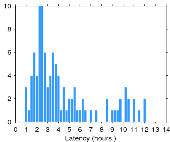
Figure 2. Histogram of the data latency for 23/07/2014. The y-axis denotes the number of files that are made available with a delay of x-hours with respect to the mean time of the records stored in the file.
