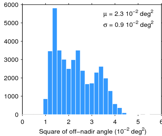
Figure 39. Histogram of flag-valid mispointing over oceans and lakes for 23/07/2014. The mean ( \mu ) and standard deviation ( \sigma ) are also shown. Note that values than 6 \cdot 10^{-2} \text{ deg}^2 are excluded from the histogram for the sake of readability but not from the computation of \mu and \sigma .
