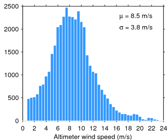
Figure 35. Histogram of science-valid wind over oceans and lakes for 23/07/2014. The mean ( \mu ) and standard deviation ( \sigma ) are also shown. Note that values larger than 24 m/s are excluded from the histogram for the sake of readability but not from the computation of \mu and \sigma .
