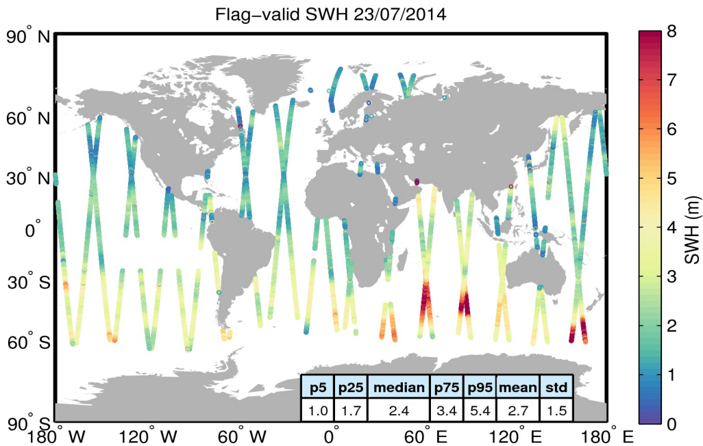
Figure 15. Geographical distribution of flag-valid SWH data over oceans and lakes for 23/07/2014. The statistical values shown in the table refer to the SWH in m and are calculated over all measurements shown in the figure.
