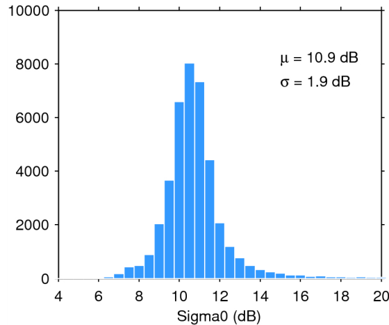
Figure 25. Histogram of flag-valid sigma0 over oceans and lakes for 23/07/2014. The mean ( \mu ) and standard deviation ( \sigma ) are also shown. Note that values outside [4 20] dB are excluded from the histogram for the sake of readability but not from the computation of \mu and \sigma .
