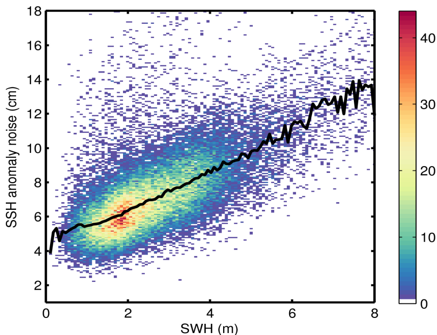
Figure 9. 2D histogram showing flag-valid SSH anomaly noise as a function of SWH for 23/07/2014. The black line denotes the median SSH anomaly as a function of SWH.
