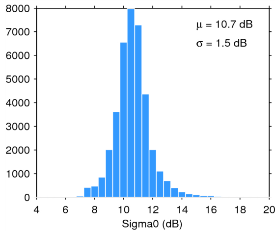
Figure 28. Histogram of science-valid sigma0 over oceans and lakes for 23/07/2014. The mean ( \mu ) and standard deviation ( \sigma ) are also shown. Note that values outside [4 20] dB are excluded from the histogram for the sake of readability but not from the computation of \mu and \sigma .
