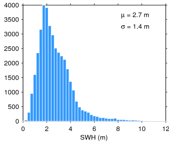
Figure 20. Histogram of science-valid SWH over oceans and lakes for 23/07/2014. The mean ( \mu ) and standard deviation ( \sigma ) are also shown. Note that values larger than 12 m are excluded from the histogram for the sake of readability but not from the computation of \mu and \sigma .
