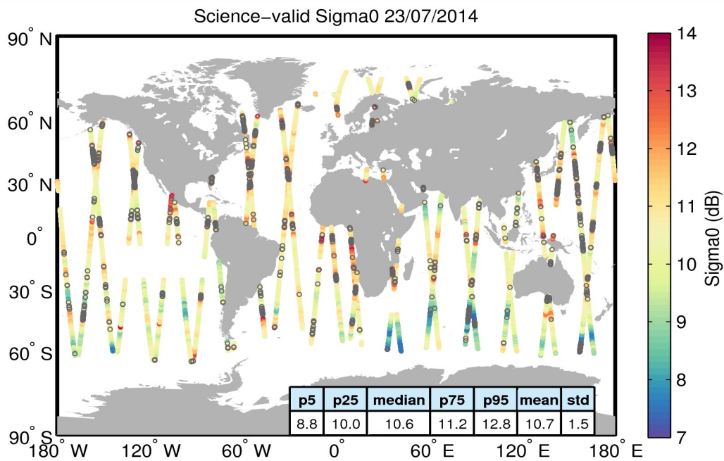
Figure 27. Geographical distribution of science-valid sigma0 data over oceans and lakes for 23/07/2014. The statistical values shown in the table refer to the sigma0 in dB and are calculated over all measurements shown in the figure. Gray circles denote records that have been rejected based on the editing criteria described in Table 4.
