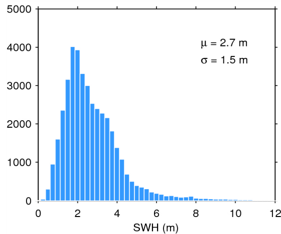
Figure 17. Histogram of flag-valid SWH over oceans and lakes for 23/07/2014. The mean ( \mu ) and standard deviation ( \sigma ) are also shown. Note that values larger than 12 m are excluded from the histogram for the sake of readability but not from the computation of \mu and \sigma .
