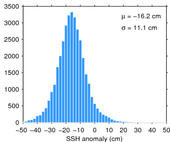
Figure 11. Histogram of science-valid SSH anomaly over oceans and lakes for 23/07/2014. The mean ( \mu ) and standard deviation ( \sigma ) are also shown. Note that values outside [-50 50] cm are excluded from the histogram for the sake of readability but not from the computation of \mu and \sigma .
