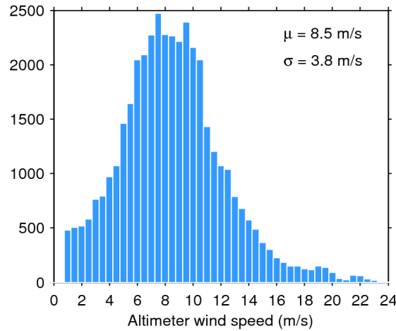
Figure 33. Histogram of flag-valid wind over oceans and lakes for 23/07/2014. The mean ( \mu ) and standard deviation ( \sigma ) are also shown. Note that values larger than 24 m/s are excluded from the histogram for the sake of readability but not from the computation of \mu and \sigma .
