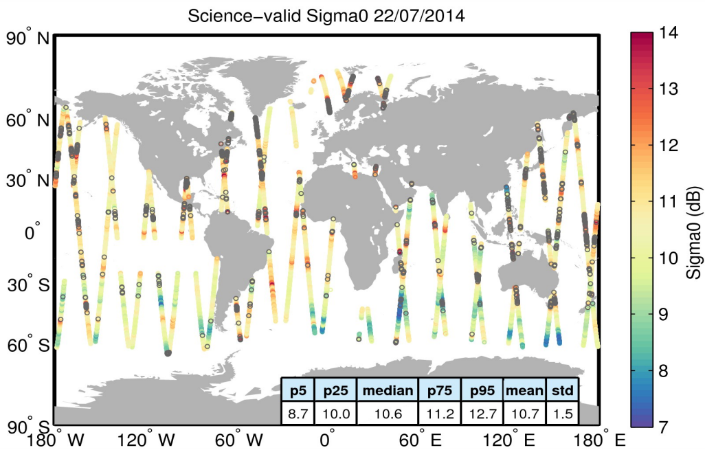
Figure 27. Geographical distribution of science-valid sigma0 data over oceans and lakes for 22/07/2014. The statistical values shown in the table refer to the sigma0 in dB and are calculated over all measurements shown in the figure. Gray circles denote records that have been rejected based on the editing criteria described in Table 4.
