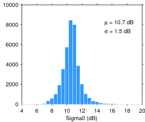
Figure 28. Histogram of science-valid sigma0 over oceans and lakes for 22/07/2014. The mean ( \mu ) and standard deviation ( \sigma ) are also shown. Note that values outside [4 20] dB are excluded from the histogram for the sake of readability but not from the computation of \mu and \sigma .
