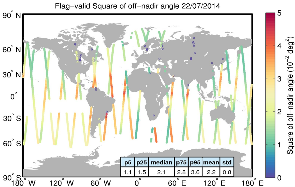
Figure 37. Geographical distribution of flag-valid mispointing data over oceans and lakes for 22/07/2014. The statistical values shown in the table refer to the mispointing in 10^{-2} \text{ deg}^2 and are calculated over all measurements shown in the figure.
