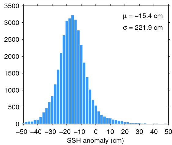
Figure 7. Histogram of flag-valid SSH anomaly over oceans and lakes for 22/07/2014. The mean ( \mu ) and standard deviation ( \sigma ) are also shown. Note that values outside [-50\ 50] cm are excluded from the histogram for the sake of readability but not from the computation of \mu and \sigma .
