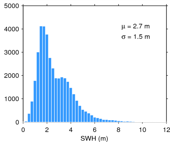
Figure 17. Histogram of flag-valid SWH over oceans and lakes for 22/07/2014. The mean ( \mu ) and standard deviation ( \sigma ) are also shown. Note that values larger than 12 m are excluded from the histogram for the sake of readability but not from the computation of \mu and \sigma .
