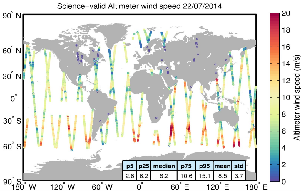
Figure 34. Geographical distribution of science-valid wind data over oceans and lakes for 22/07/2014. The statistical values shown in the table refer to the wind in m/s and are calculated over all measurements shown in the figure. Gray circles denote records that have been rejected based on the editing criteria described in Table 5.
