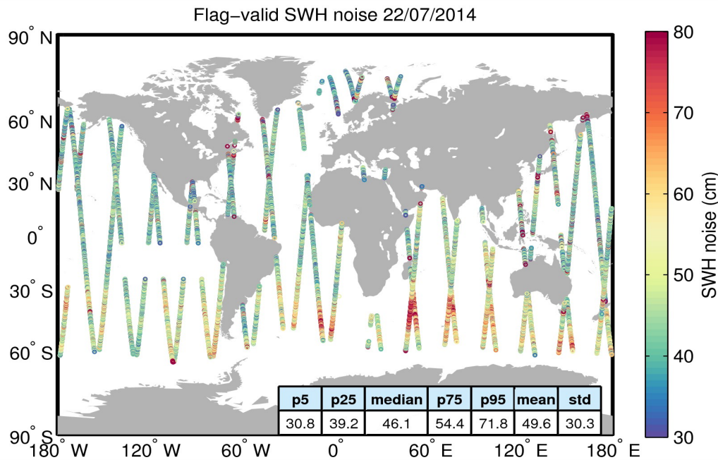
Figure 18. Geographical distribution of flag-valid 20-Hz SWH measurement noise over oceans and lakes for 22/07/2014. The statistical values shown in the figure refer to the SWH noise and are calculated over all measurements shown in the figure.
