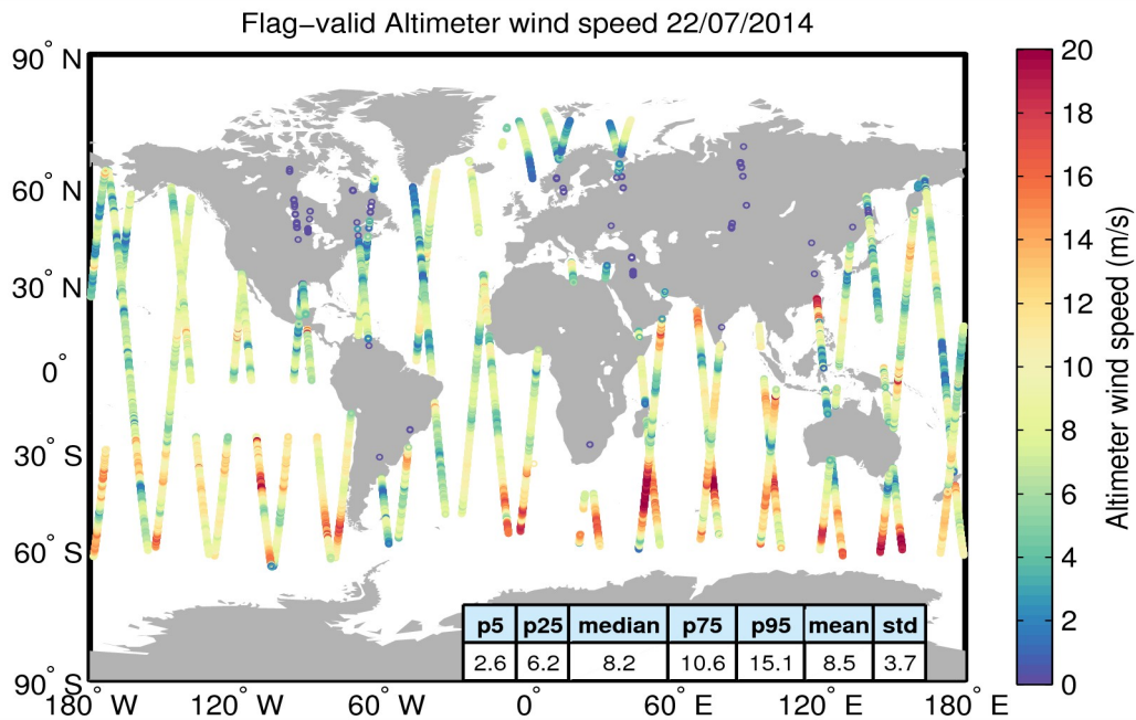
Figure 31. Geographical distribution of flag-valid wind data over oceans and lakes for 22/07/2014. The statistical values shown in the table refer to the wind in m/s and are calculated over all measurements shown in the figure.
