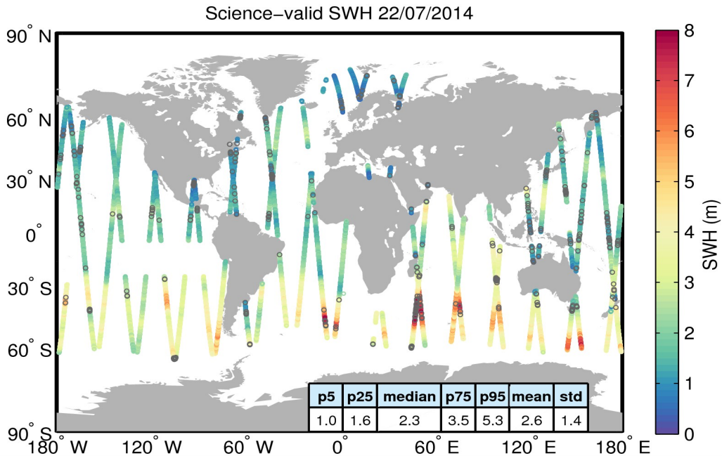
Figure 19. Geographical distribution of science-valid SWH data over oceans and lakes for 22/07/2014. The statistical values shown in the table refer to the SWH in m and are calculated over all measurements shown in the figure. Gray circles denote records that have been rejected based on the editing criteria described in Table 3.
