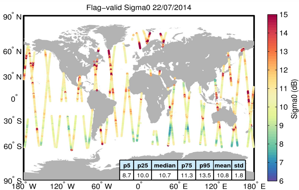
Figure 23. Geographical distribution of flag-valid sigma0 data over oceans and lakes for 22/07/2014. The statistical values shown in the table refer to the sigma0 in dB and are calculated over all measurements shown in the figure.
