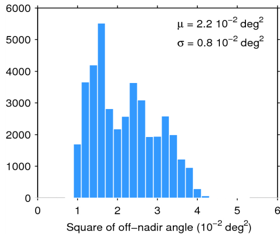
Figure 39. Histogram of flag-valid mispointing over oceans and lakes for 22/07/2014. The mean ( \mu ) and standard deviation ( \sigma ) are also shown. Note that values than 6 \cdot 10^{-2} \text{ deg}^2 are excluded from the histogram for the sake of readability but not from the computation of \mu and \sigma .
