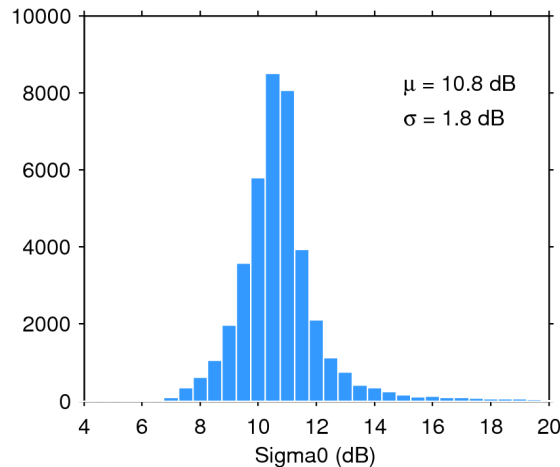
Figure 25. Histogram of flag-valid sigma0 over oceans and lakes for 22/07/2014. The mean ( \mu ) and standard deviation ( \sigma ) are also shown. Note that values outside [4 20] dB are excluded from the histogram for the sake of readability but not from the computation of \mu and \sigma .
