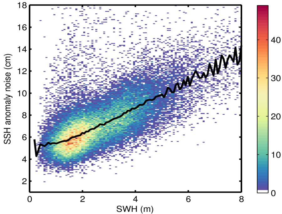
Figure 9. 2D histogram showing flag-valid SSH anomaly noise as a function of SWH for 22/07/2014. The black line denotes the median SSH anomaly as a function of SWH.
