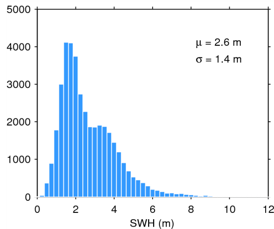
Figure 20. Histogram of science-valid SWH over oceans and lakes for 22/07/2014. The mean ( \mu ) and standard deviation ( \sigma ) are also shown. Note that values larger than 12 m are excluded from the histogram for the sake of readability but not from the computation of \mu and \sigma .
