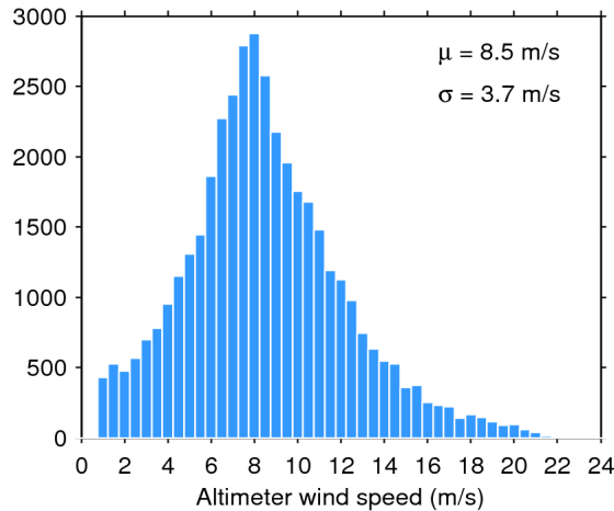
Figure 33. Histogram of flag-valid wind over oceans and lakes for 22/07/2014. The mean ( \mu ) and standard deviation ( \sigma ) are also shown. Note that values larger than 24 m/s are excluded from the histogram for the sake of readability but not from the computation of \mu and \sigma .
