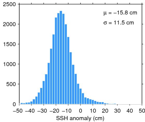
Figure 11. Histogram of science-valid SSH anomaly over oceans and lakes for 22/07/2014. The mean ( \mu ) and standard deviation ( \sigma ) are also shown. Note that values outside [-50 50] cm are excluded from the histogram for the sake of readability but not from the computation of \mu and \sigma .
