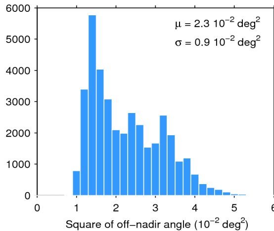
Figure 39. Histogram of flag-valid mispointing over oceans and lakes for 21/07/2014. The mean ( \mu ) and standard deviation ( \sigma ) are also shown. Note that values than 6 \cdot 10^{-2} \text{ deg}^2 are excluded from the histogram for the sake of readability but not from the computation of \mu and \sigma .
