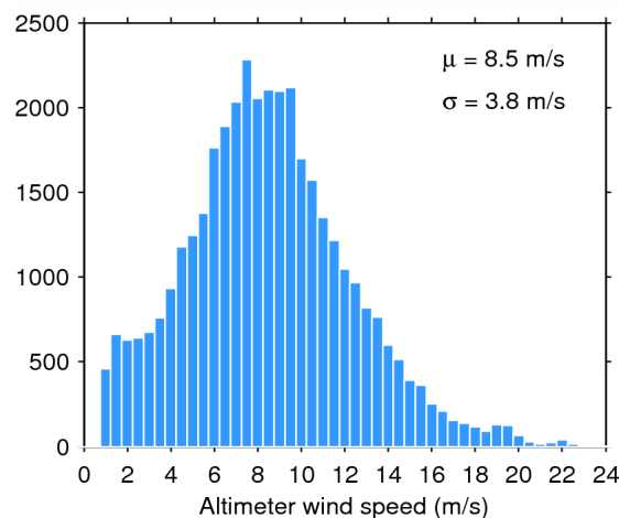
Figure 35. Histogram of science-valid wind over oceans and lakes for 21/07/2014. The mean ( \mu ) and standard deviation ( \sigma ) are also shown. Note that values larger than 24 m/s are excluded from the histogram for the sake of readability but not from the computation of \mu and \sigma .
