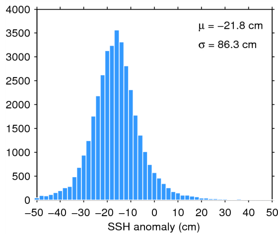
Figure 7. Histogram of flag-valid SSH anomaly over oceans and lakes for 21/07/2014. The mean ( \mu ) and standard deviation ( \sigma ) are also shown. Note that values outside [-50\ 50] cm are excluded from the histogram for the sake of readability but not from the computation of \mu and \sigma .
