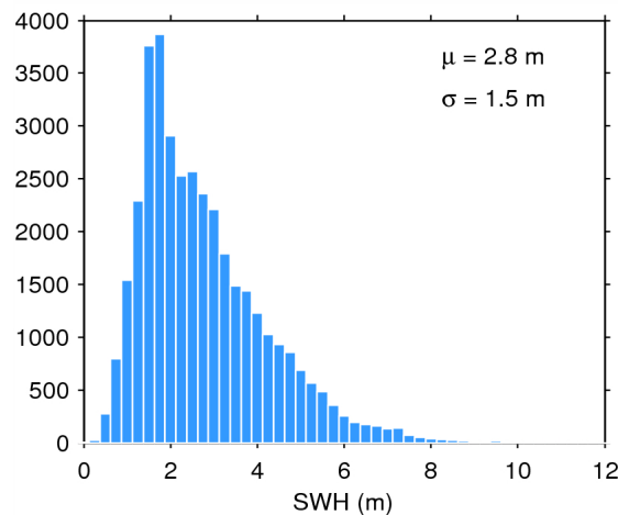
Figure 17. Histogram of flag-valid SWH over oceans and lakes for 21/07/2014. The mean ( \mu ) and standard deviation ( \sigma ) are also shown. Note that values larger than 12 m are excluded from the histogram for the sake of readability but not from the computation of \mu and \sigma .
