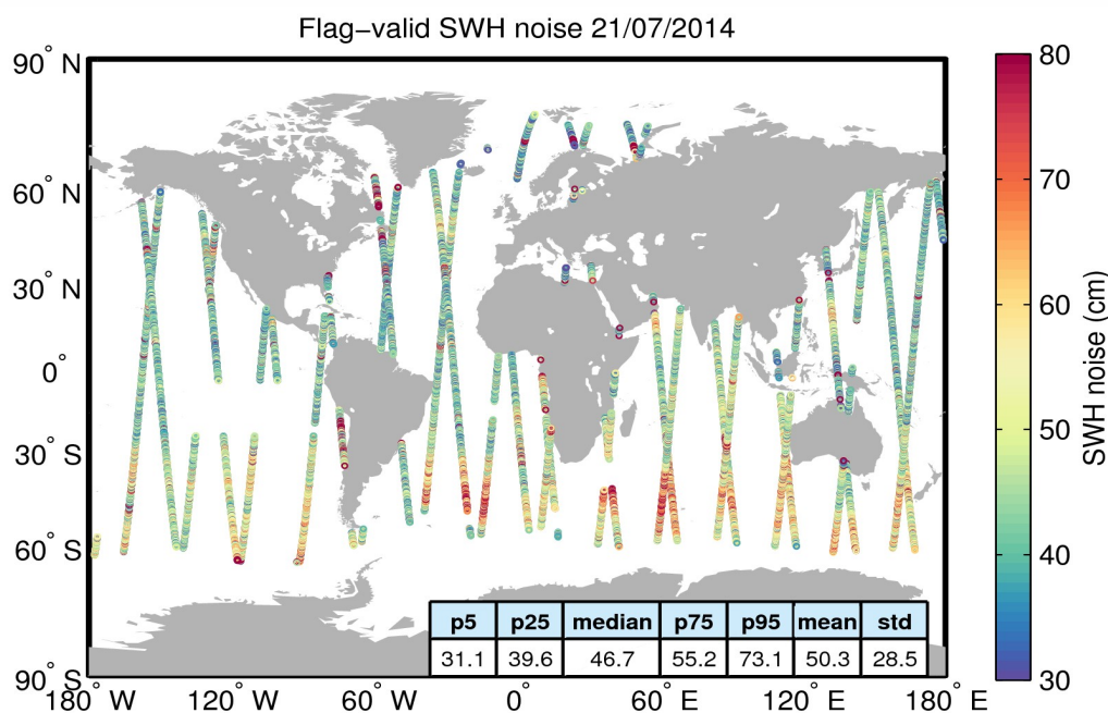
Figure 18. Geographical distribution of flag-valid 20-Hz SWH measurement noise over oceans and lakes for 21/07/2014. The statistical values shown in the figure refer to the SWH noise and are calculated over all measurements shown in the figure.
