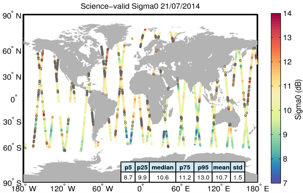
Figure 27. Geographical distribution of science-valid sigma0 data over oceans and lakes for 21/07/2014. The statistical values shown in the table refer to the sigma0 in dB and are calculated over all measurements shown in the figure. Gray circles denote records that have been rejected based on the editing criteria described in Table 4.
