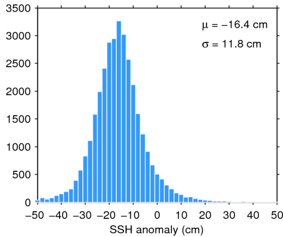
Figure 11. Histogram of science-valid SSH anomaly over oceans and lakes for 21/07/2014. The mean ( \mu ) and standard deviation ( \sigma ) are also shown. Note that values outside [-50 50] cm are excluded from the histogram for the sake of readability but not from the computation of \mu and \sigma .
