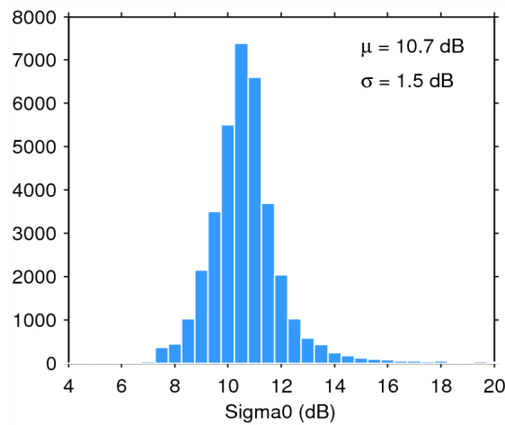
Figure 28. Histogram of science-valid sigma0 over oceans and lakes for 21/07/2014. The mean ( \mu ) and standard deviation ( \sigma ) are also shown. Note that values outside [4 20] dB are excluded from the histogram for the sake of readability but not from the computation of \mu and \sigma .
