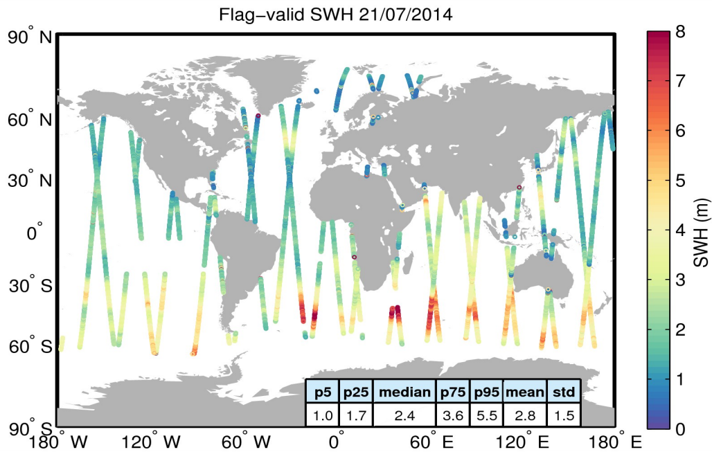
Figure 15. Geographical distribution of flag-valid SWH data over oceans and lakes for 21/07/2014. The statistical values shown in the table refer to the SWH in m and are calculated over all measurements shown in the figure.
