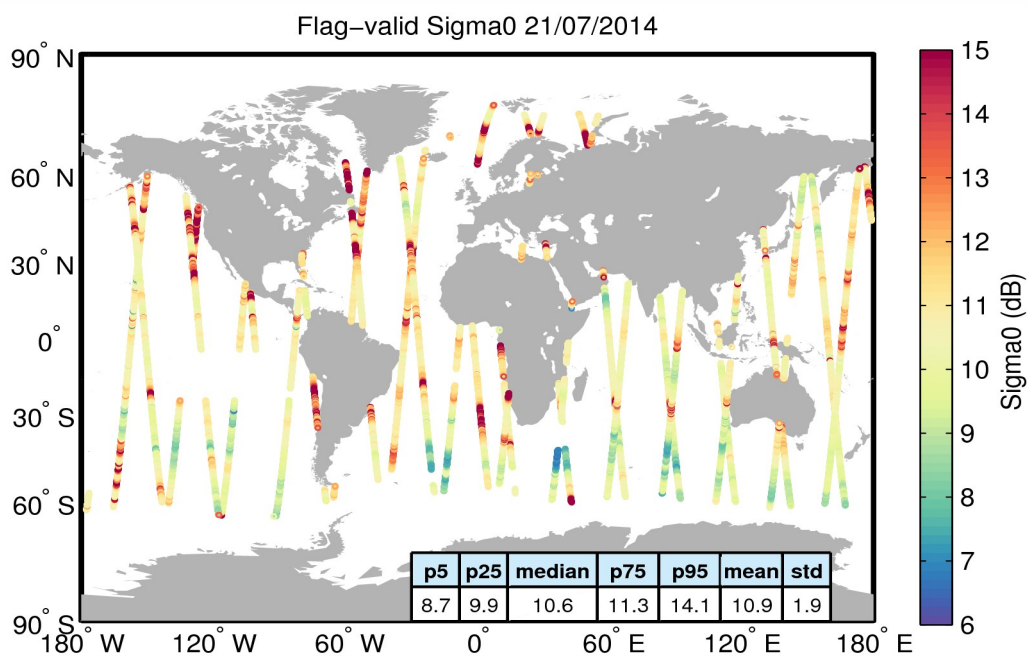
Figure 23. Geographical distribution of flag-valid sigma0 data over oceans and lakes for 21/07/2014. The statistical values shown in the table refer to the sigma0 in dB and are calculated over all measurements shown in the figure.
