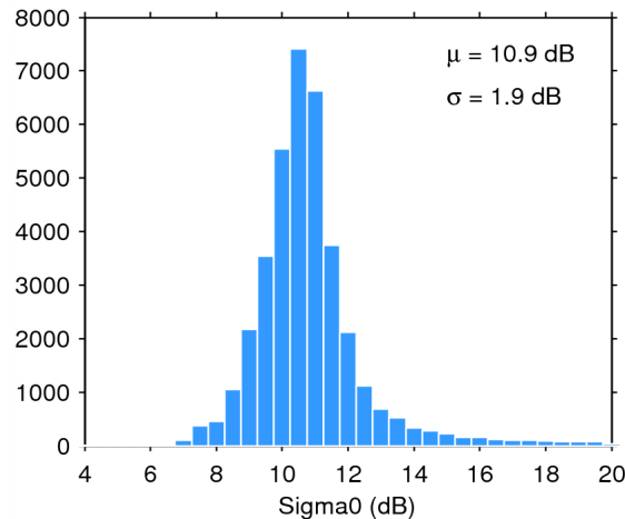
Figure 25. Histogram of flag-valid sigma0 over oceans and lakes for 21/07/2014. The mean ( \mu ) and standard deviation ( \sigma ) are also shown. Note that values outside [4 20] dB are excluded from the histogram for the sake of readability but not from the computation of \mu and \sigma .
