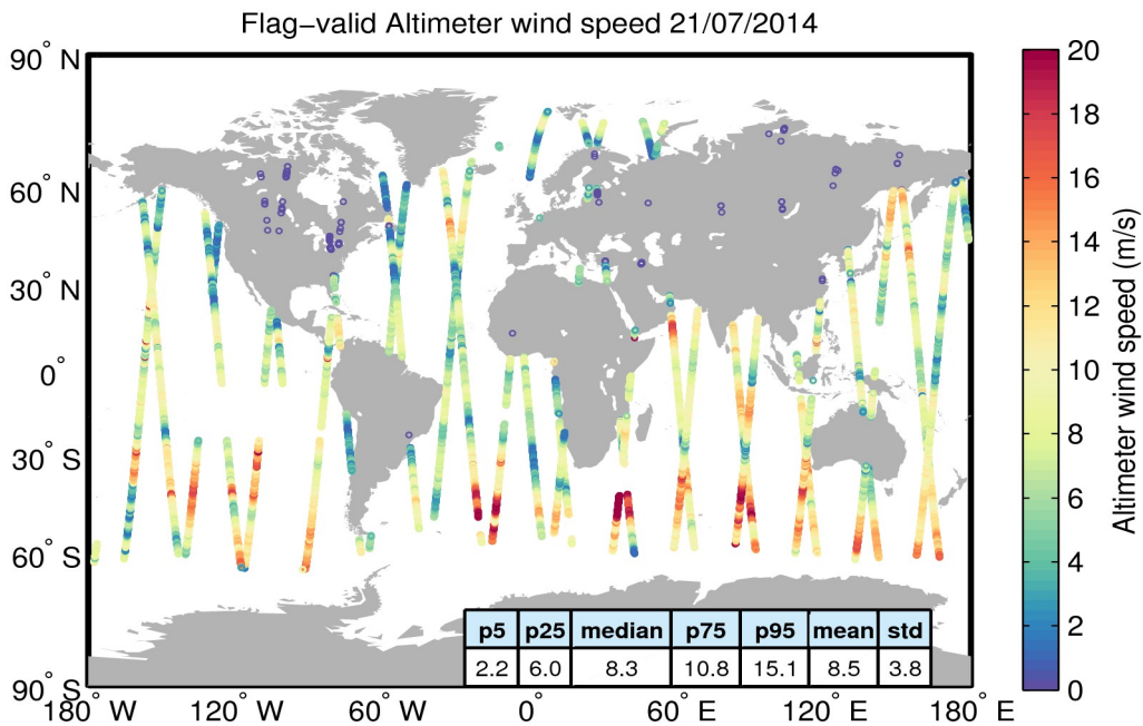
Figure 31. Geographical distribution of flag-valid wind data over oceans and lakes for 21/07/2014. The statistical values shown in the table refer to the wind in m/s and are calculated over all measurements shown in the figure.
