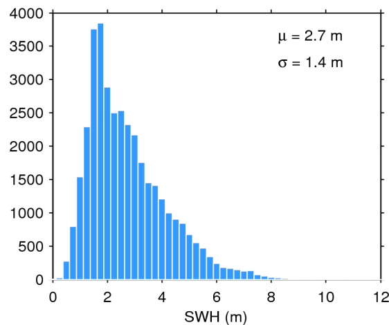
Figure 20. Histogram of science-valid SWH over oceans and lakes for 21/07/2014. The mean ( \mu ) and standard deviation ( \sigma ) are also shown. Note that values larger than 12 m are excluded from the histogram for the sake of readability but not from the computation of \mu and \sigma .
