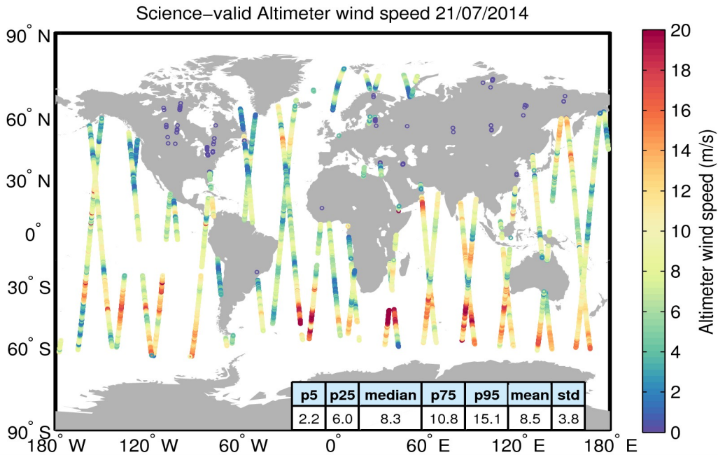
Figure 34. Geographical distribution of science-valid wind data over oceans and lakes for 21/07/2014. The statistical values shown in the table refer to the wind in m/s and are calculated over all measurements shown in the figure. Gray circles denote records that have been rejected based on the editing criteria described in Table 5.
