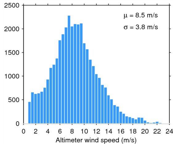
Figure 33. Histogram of flag-valid wind over oceans and lakes for 21/07/2014. The mean ( \mu ) and standard deviation ( \sigma ) are also shown. Note that values larger than 24 m/s are excluded from the histogram for the sake of readability but not from the computation of \mu and \sigma .
