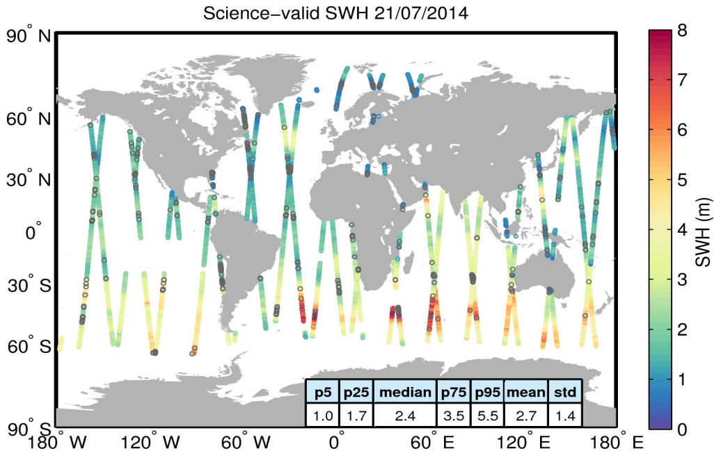
Figure 19. Geographical distribution of science-valid SWH data over oceans and lakes for 21/07/2014. The statistical values shown in the table refer to the SWH in m and are calculated over all measurements shown in the figure. Gray circles denote records that have been rejected based on the editing criteria described in Table 3.
