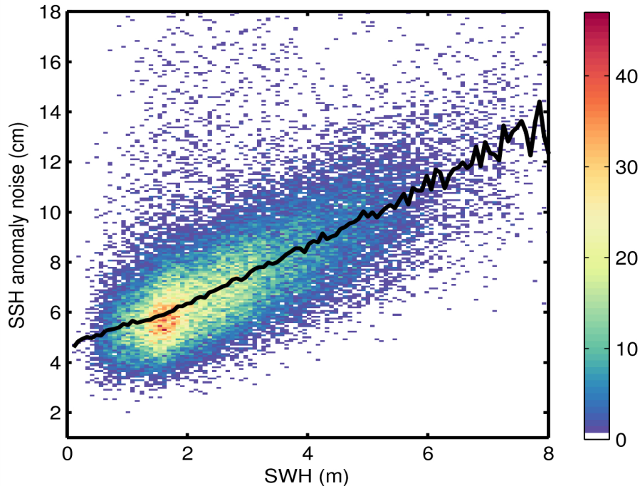
Figure 9. 2D histogram showing flag-valid SSH anomaly noise as a function of SWH for 21/07/2014. The black line denotes the median SSH anomaly as a function of SWH.
