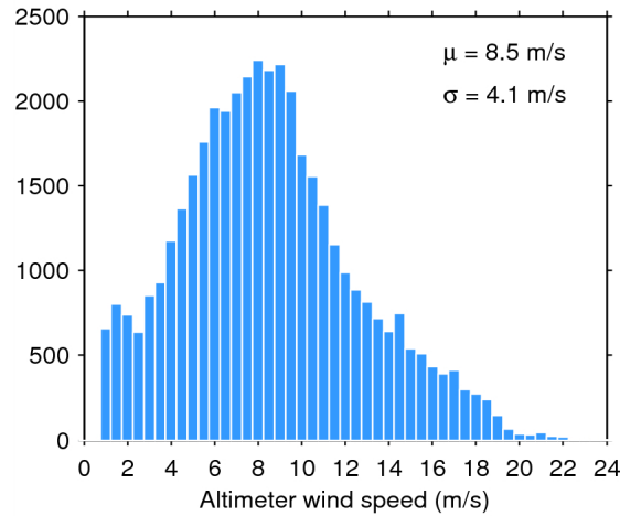
Figure 33. Histogram of flag-valid wind over oceans and lakes for 19/07/2014. The mean ( \mu ) and standard deviation ( \sigma ) are also shown. Note that values larger than 24 m/s are excluded from the histogram for the sake of readability but not from the computation of \mu and \sigma .
