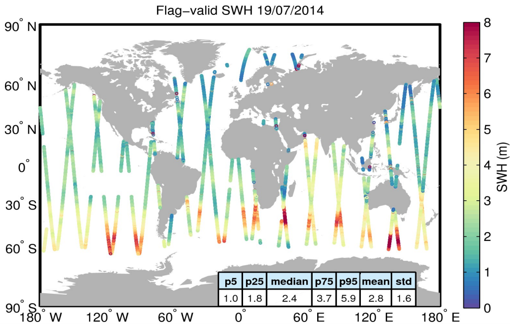
Figure 15. Geographical distribution of flag-valid SWH data over oceans and lakes for 19/07/2014. The statistical values shown in the table refer to the SWH in m and are calculated over all measurements shown in the figure.
