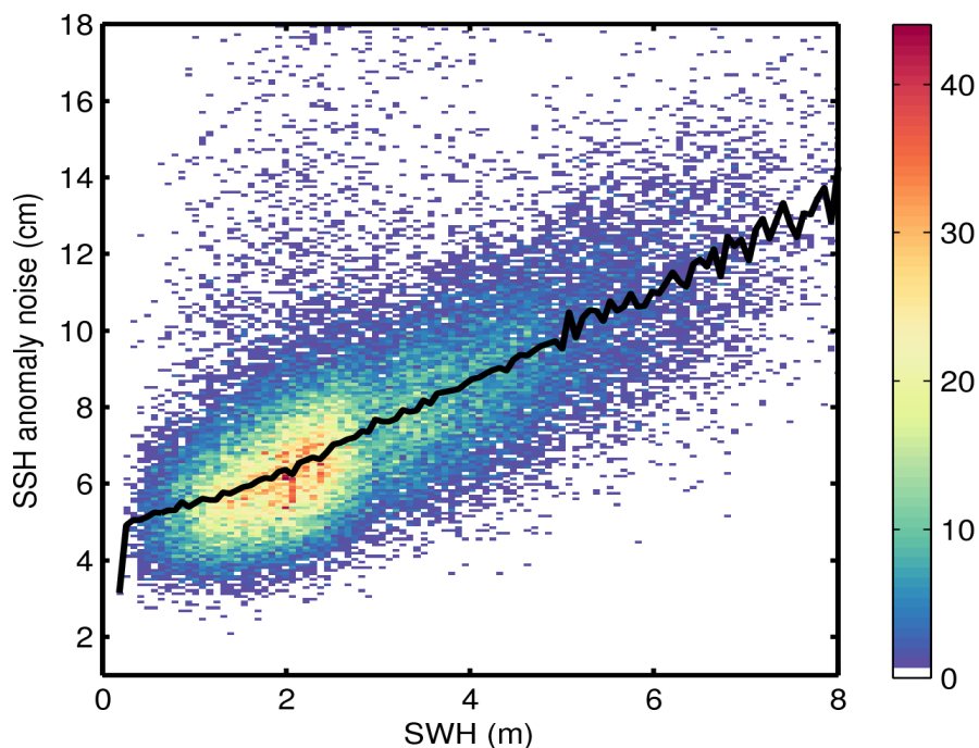
Figure 9. 2D histogram showing flag-valid SSH anomaly noise as a function of SWH for 19/07/2014. The black line denotes the median SSH anomaly as a function of SWH.
