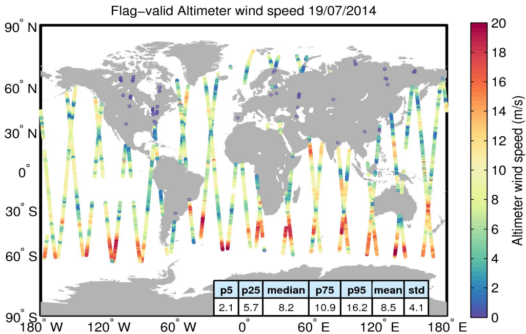
Figure 31. Geographical distribution of flag-valid wind data over oceans and lakes for 19/07/2014. The statistical values shown in the table refer to the wind in m/s and are calculated over all measurements shown in the figure.
