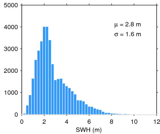
Figure 17. Histogram of flag-valid SWH over oceans and lakes for 19/07/2014. The mean ( \mu ) and standard deviation ( \sigma ) are also shown. Note that values larger than 12 m are excluded from the histogram for the sake of readability but not from the computation of \mu and \sigma .
