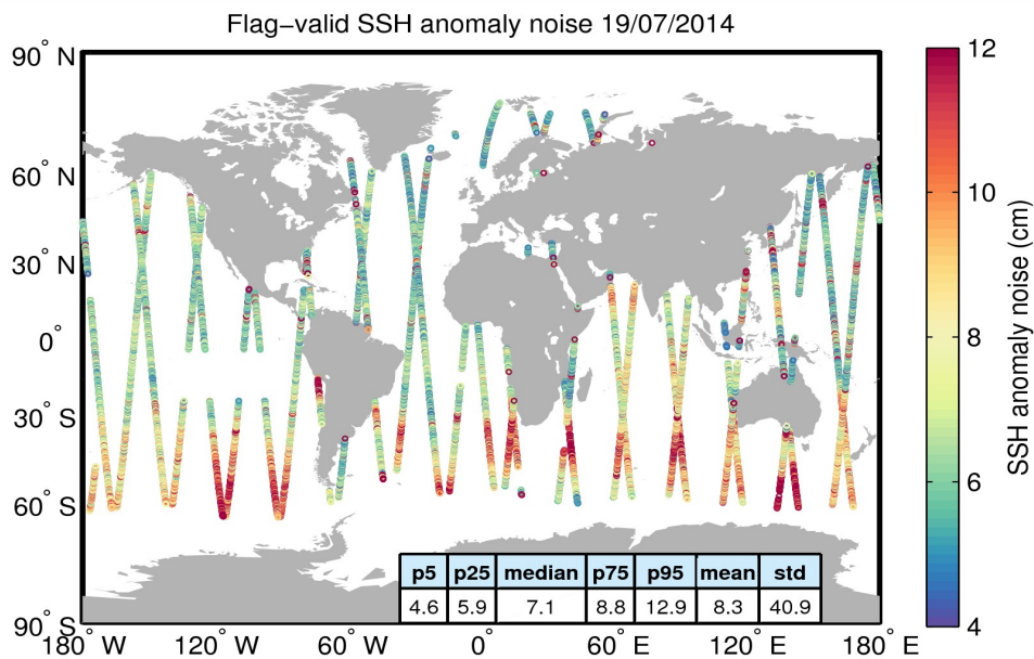
Figure 8. Geographical distribution of flag-valid 20-Hz SSH anomaly measurement noise over oceans and lakes for 19/07/2014. The statistical values shown in the table refer to the SSH anomaly noise and are calculated over all measurements shown in the figure.
