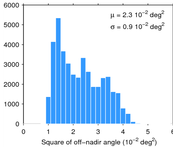
Figure 39. Histogram of flag-valid mispointing over oceans and lakes for 19/07/2014. The mean ( \mu ) and standard deviation ( \sigma ) are also shown. Note that values than 6 \cdot 10^{-2} \text{ deg}^2 are excluded from the histogram for the sake of readability but not from the computation of \mu and \sigma .
