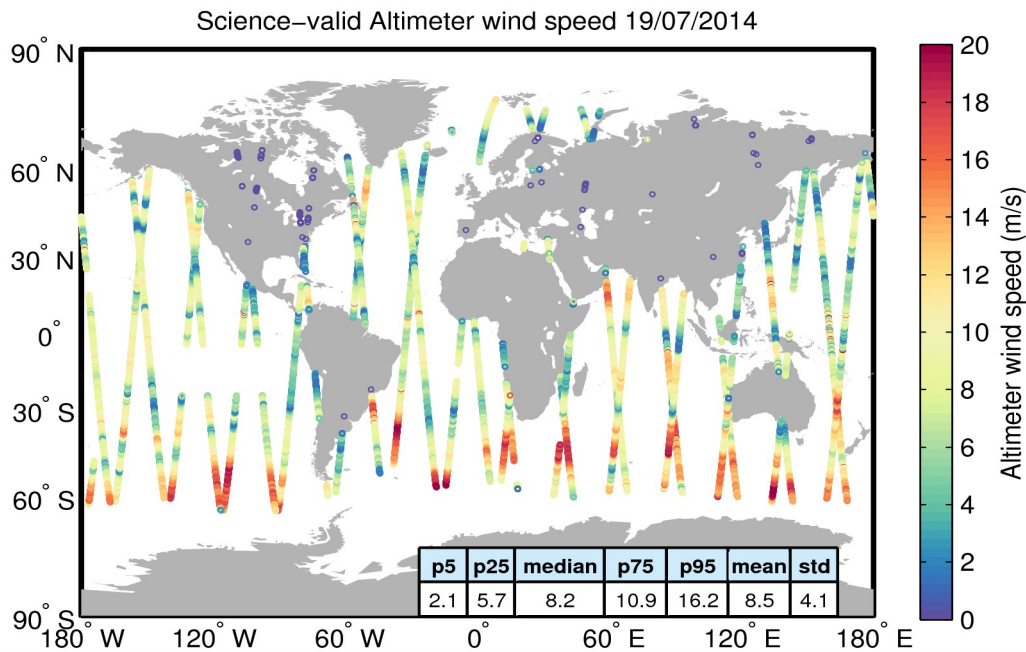
Figure 34. Geographical distribution of science-valid wind data over oceans and lakes for 19/07/2014. The statistical values shown in the table refer to the wind in m/s and are calculated over all measurements shown in the figure. Gray circles denote records that have been rejected based on the editing criteria described in Table 5.
