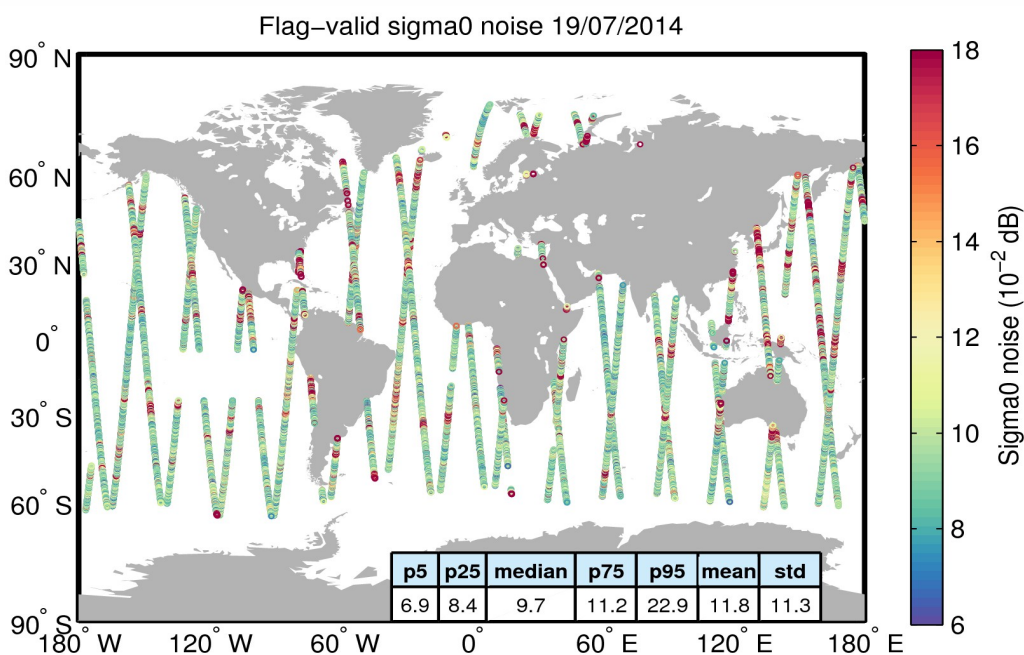
Figure 26. Geographical distribution of flag-valid 20-Hz sigma0 measurement noise over oceans and lakes for 19/07/2014. The statistical values shown in the table refer to the sigma0 noise and are calculated over all measurements shown in the figure.
