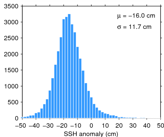
Figure 11. Histogram of science-valid SSH anomaly over oceans and lakes for 19/07/2014. The mean ( \mu ) and standard deviation ( \sigma ) are also shown. Note that values outside [-50 50] cm are excluded from the histogram for the sake of readability but not from the computation of \mu and \sigma .
