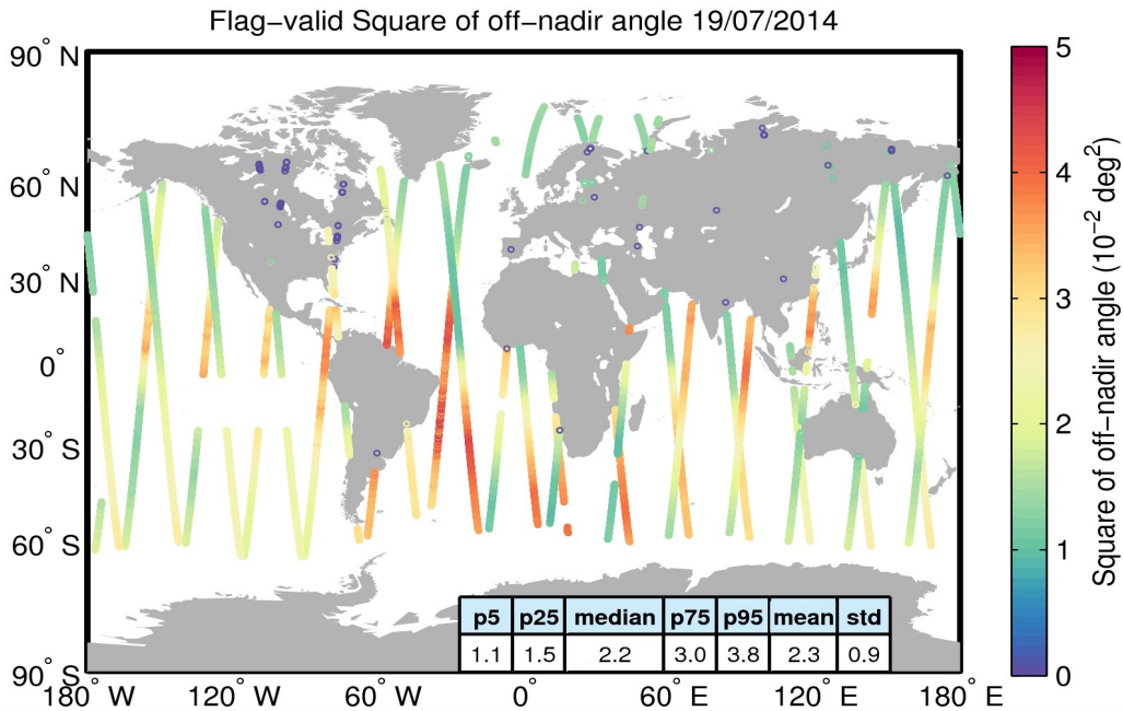
Figure 37. Geographical distribution of flag-valid mispointing data over oceans and lakes for 19/07/2014. The statistical values shown in the table refer to the mispointing in 10^{-2} \text{deg}^2 and are calculated over all measurements shown in the figure.
