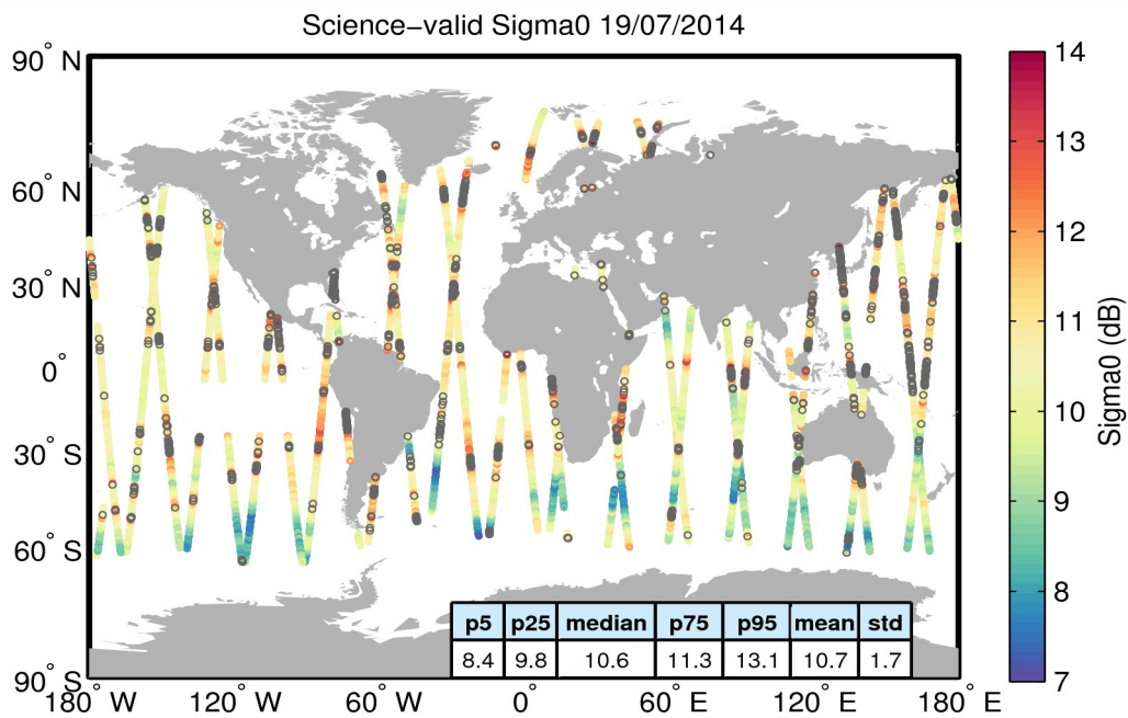
Figure 27. Geographical distribution of science-valid sigma0 data over oceans and lakes for 19/07/2014. The statistical values shown in the table refer to the sigma0 in dB and are calculated over all measurements shown in the figure. Gray circles denote records that have been rejected based on the editing criteria described in Table 4.
