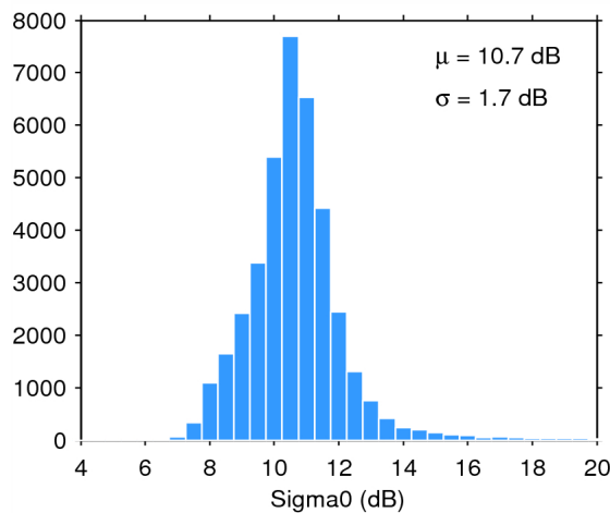
Figure 28. Histogram of science-valid sigma0 over oceans and lakes for 19/07/2014. The mean ( \mu ) and standard deviation ( \sigma ) are also shown. Note that values outside [4 20] dB are excluded from the histogram for the sake of readability but not from the computation of \mu and \sigma .
