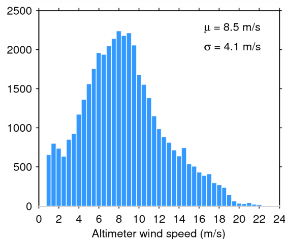
Figure 35. Histogram of science-valid wind over oceans and lakes for 19/07/2014. The mean ( \mu ) and standard deviation ( \sigma ) are also shown. Note that values larger than 24 m/s are excluded from the histogram for the sake of readability but not from the computation of \mu and \sigma .
