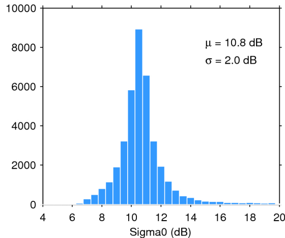
Figure 25. Histogram of flag-valid sigma0 over oceans and lakes for 18/07/2014. The mean ( \mu ) and standard deviation ( \sigma ) are also shown. Note that values outside [4 20] dB are excluded from the histogram for the sake of readability but not from the computation of \mu and \sigma .
