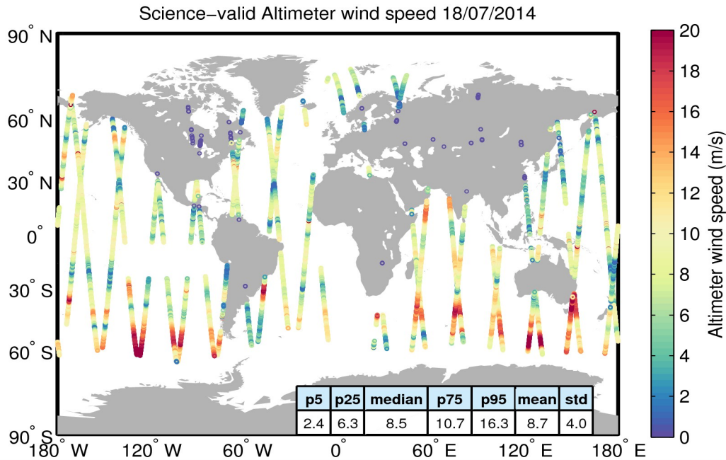
Figure 34. Geographical distribution of science-valid wind data over oceans and lakes for 18/07/2014. The statistical values shown in the table refer to the wind in m/s and are calculated over all measurements shown in the figure. Gray circles denote records that have been rejected based on the editing criteria described in Table 5.
