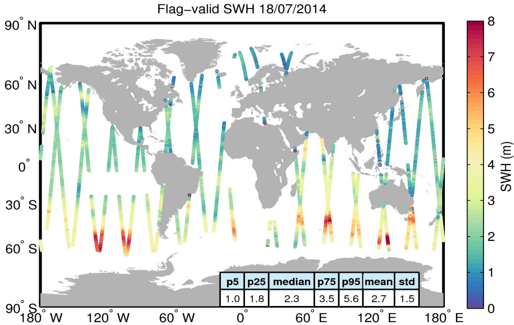
Figure 15. Geographical distribution of flag-valid SWH data over oceans and lakes for 18/07/2014. The statistical values shown in the table refer to the SWH in m and are calculated over all measurements shown in the figure.
