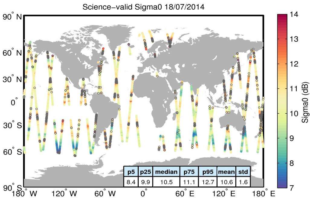
Figure 27. Geographical distribution of science-valid sigma0 data over oceans and lakes for 18/07/2014. The statistical values shown in the table refer to the sigma0 in dB and are calculated over all measurements shown in the figure. Gray circles denote records that have been rejected based on the editing criteria described in Table 4.
