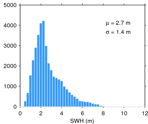
Figure 20. Histogram of science-valid SWH over oceans and lakes for 18/07/2014. The mean ( \mu ) and standard deviation ( \sigma ) are also shown. Note that values larger than 12 m are excluded from the histogram for the sake of readability but not from the computation of \mu and \sigma .
