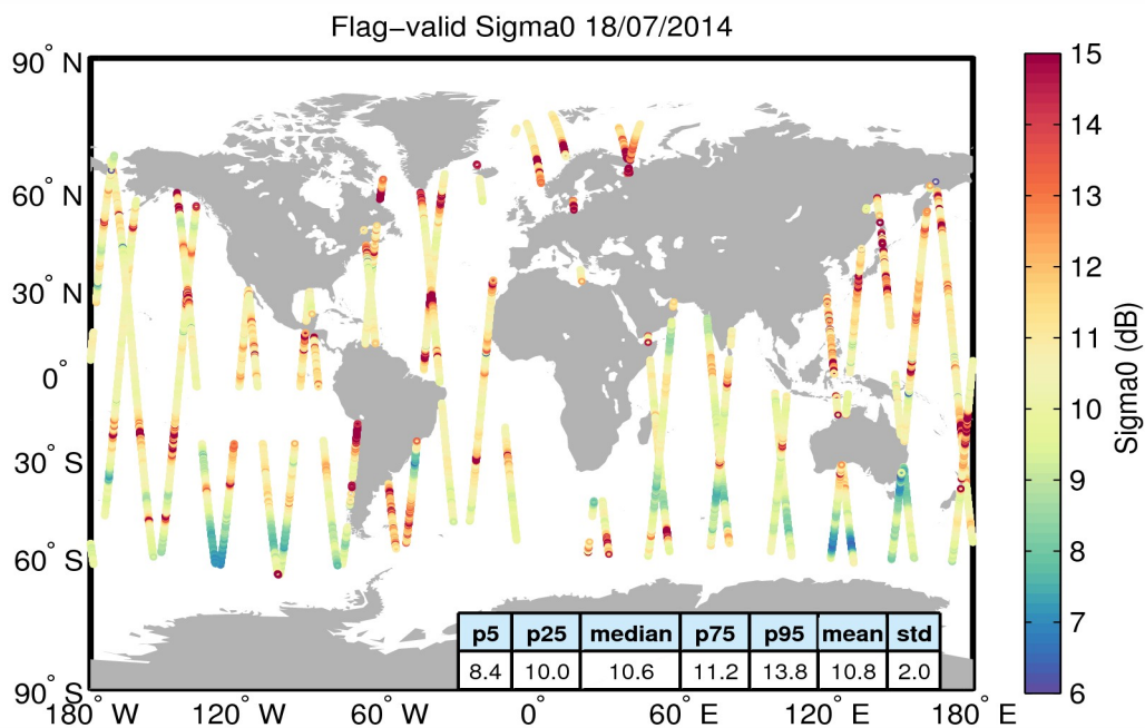
Figure 23. Geographical distribution of flag-valid sigma0 data over oceans and lakes for 18/07/2014. The statistical values shown in the table refer to the sigma0 in dB and are calculated over all measurements shown in the figure.
