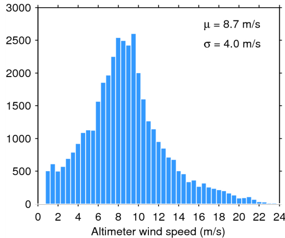
Figure 33. Histogram of flag-valid wind over oceans and lakes for 18/07/2014. The mean ( \mu ) and standard deviation ( \sigma ) are also shown. Note that values larger than 24 m/s are excluded from the histogram for the sake of readability but not from the computation of \mu and \sigma .
