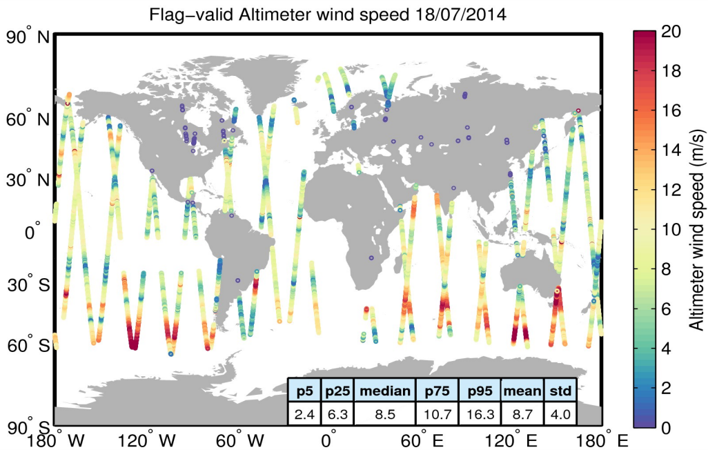
Figure 31. Geographical distribution of flag-valid wind data over oceans and lakes for 18/07/2014. The statistical values shown in the table refer to the wind in m/s and are calculated over all measurements shown in the figure.
