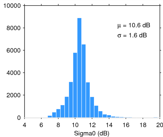
Figure 28. Histogram of science-valid sigma0 over oceans and lakes for 18/07/2014. The mean ( \mu ) and standard deviation ( \sigma ) are also shown. Note that values outside [4 20] dB are excluded from the histogram for the sake of readability but not from the computation of \mu and \sigma .
