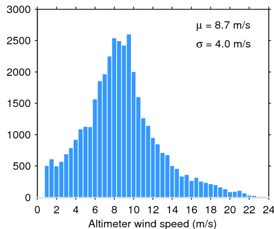
Figure 35. Histogram of science-valid wind over oceans and lakes for 18/07/2014. The mean ( \mu ) and standard deviation ( \sigma ) are also shown. Note that values larger than 24 m/s are excluded from the histogram for the sake of readability but not from the computation of \mu and \sigma .
