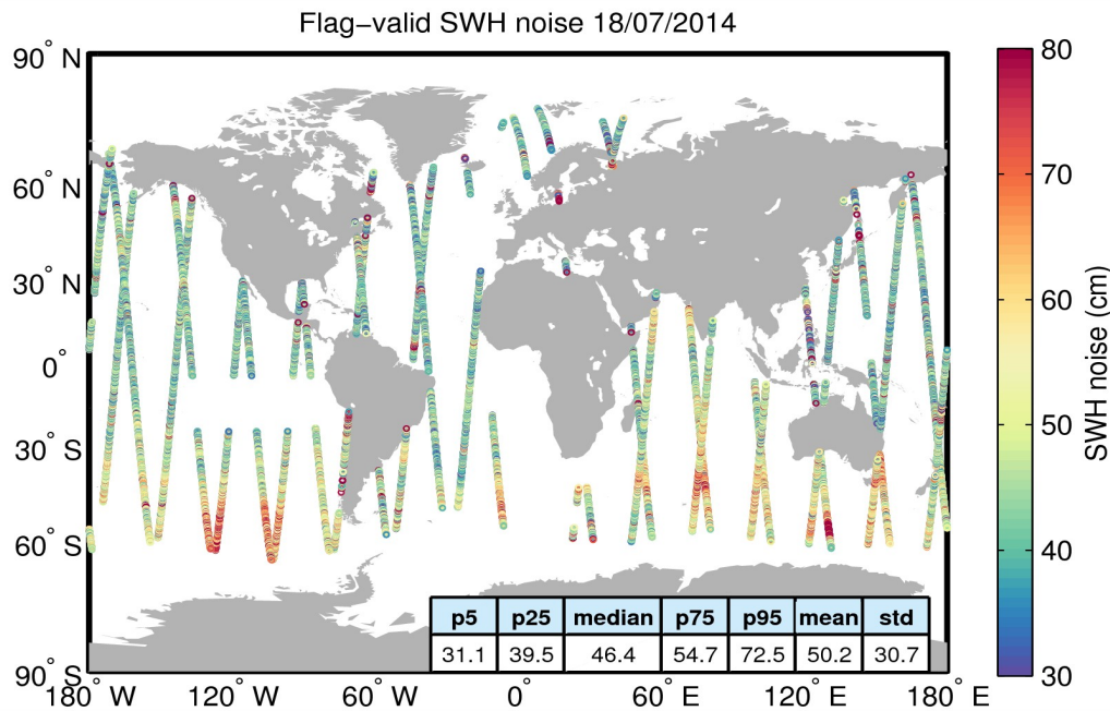
Figure 18. Geographical distribution of flag-valid 20-Hz SWH measurement noise over oceans and lakes for 18/07/2014. The statistical values shown in the figure refer to the SWH noise and are calculated over all measurements shown in the figure.
