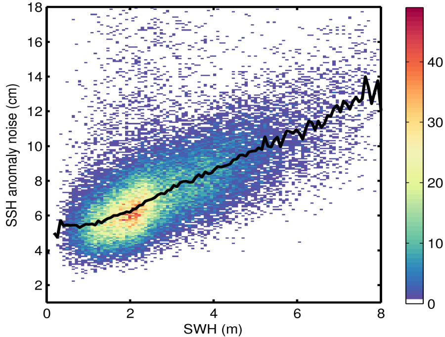
Figure 9. 2D histogram showing flag-valid SSH anomaly noise as a function of SWH for 18/07/2014. The black line denotes the median SSH anomaly as a function of SWH.
