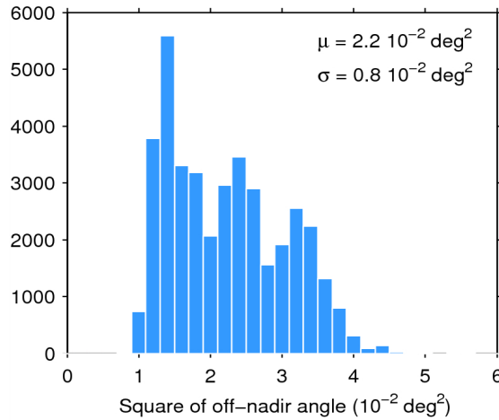
Figure 39. Histogram of flag-valid mispointing over oceans and lakes for 18/07/2014. The mean ( \mu ) and standard deviation ( \sigma ) are also shown. Note that values than 6 \cdot 10^{-2} \text{ deg}^2 are excluded from the histogram for the sake of readability but not from the computation of \mu and \sigma .
