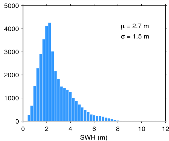
Figure 17. Histogram of flag-valid SWH over oceans and lakes for 18/07/2014. The mean ( \mu ) and standard deviation ( \sigma ) are also shown. Note that values larger than 12 m are excluded from the histogram for the sake of readability but not from the computation of \mu and \sigma .
