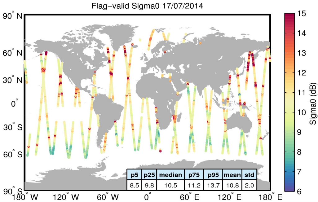
Figure 23. Geographical distribution of flag-valid sigma0 data over oceans and lakes for 17/07/2014. The statistical values shown in the table refer to the sigma0 in dB and are calculated over all measurements shown in the figure.
