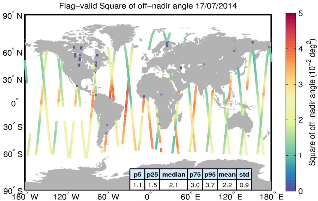
Figure 37. Geographical distribution of flag-valid mispointing data over oceans and lakes for 17/07/2014. The statistical values shown in the table refer to the mispointing in 10^{-2} \text{ deg}^2 and are calculated over all measurements shown in the figure.
