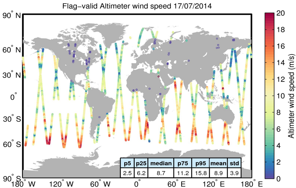
Figure 31. Geographical distribution of flag-valid wind data over oceans and lakes for 17/07/2014. The statistical values shown in the table refer to the wind in m/s and are calculated over all measurements shown in the figure.
