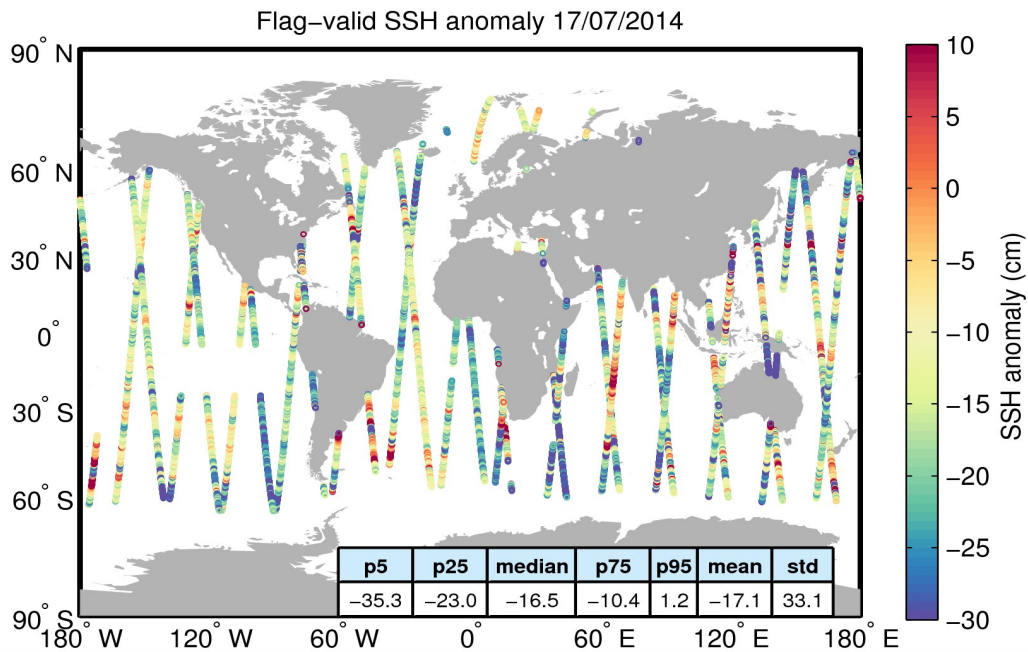
Figure 5. Geographical distribution of flag-valid 1-Hz SSH anomaly data over oceans and lakes for 17/07/2014. The statistical values shown in the table refer to the SSH anomaly in cm and are calculated over all measurements shown in the figure.
