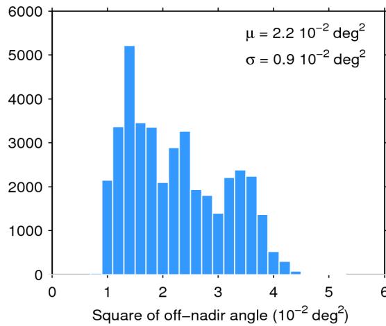
Figure 39. Histogram of flag-valid mispointing over oceans and lakes for 17/07/2014. The mean ( \mu ) and standard deviation ( \sigma ) are also shown. Note that values than 6 \cdot 10^{-2} \text{ deg}^2 are excluded from the histogram for the sake of readability but not from the computation of \mu and \sigma .
