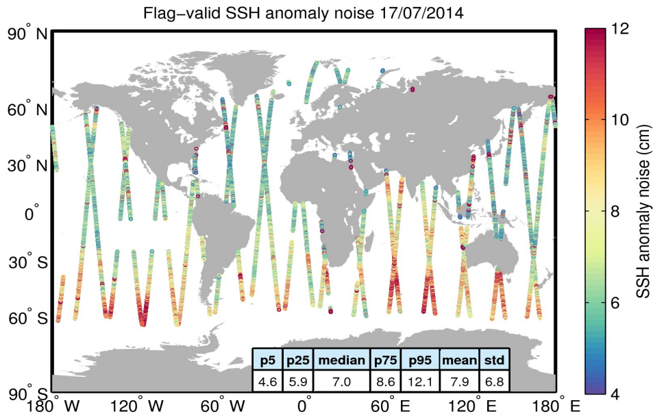
Figure 8. Geographical distribution of flag-valid 20-Hz SSH anomaly measurement noise over oceans and lakes for 17/07/2014. The statistical values shown in the table refer to the SSH anomaly noise and are calculated over all measurements shown in the figure.
