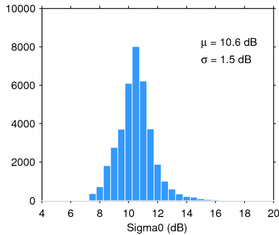
Figure 28. Histogram of science-valid sigma0 over oceans and lakes for 17/07/2014. The mean ( \mu ) and standard deviation ( \sigma ) are also shown. Note that values outside [4 20] dB are excluded from the histogram for the sake of readability but not from the computation of \mu and \sigma .
