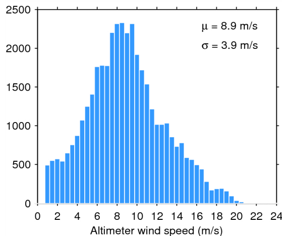
Figure 35. Histogram of science-valid wind over oceans and lakes for 17/07/2014. The mean ( \mu ) and standard deviation ( \sigma ) are also shown. Note that values larger than 24 m/s are excluded from the histogram for the sake of readability but not from the computation of \mu and \sigma .
