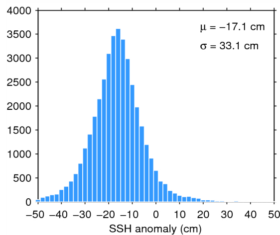
Figure 7. Histogram of flag-valid SSH anomaly over oceans and lakes for 17/07/2014. The mean ( \mu ) and standard deviation ( \sigma ) are also shown. Note that values outside [-50 50] cm are excluded from the histogram for the sake of readability but not from the computation of \mu and \sigma .
