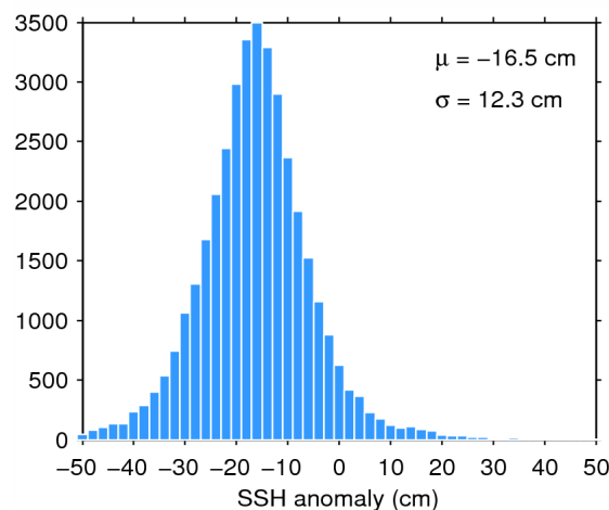
Figure 11. Histogram of science-valid SSH anomaly over oceans and lakes for 17/07/2014. The mean ( \mu ) and standard deviation ( \sigma ) are also shown. Note that values outside [-50 50] cm are excluded from the histogram for the sake of readability but not from the computation of \mu and \sigma .
