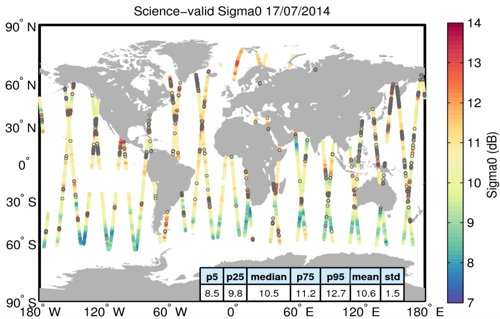
Figure 27. Geographical distribution of science-valid sigma0 data over oceans and lakes for 17/07/2014. The statistical values shown in the table refer to the sigma0 in dB and are calculated over all measurements shown in the figure. Gray circles denote records that have been rejected based on the editing criteria described in Table 4.
