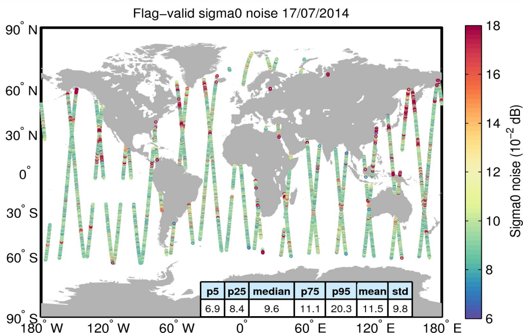
Figure 26. Geographical distribution of flag-valid 20-Hz sigma0 measurement noise over oceans and lakes for 17/07/2014. The statistical values shown in the table refer to the sigma0 noise and are calculated over all measurements shown in the figure.
