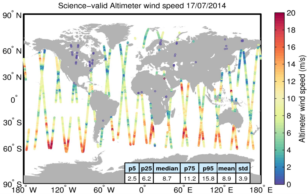
Figure 34. Geographical distribution of science-valid wind data over oceans and lakes for 17/07/2014. The statistical values shown in the table refer to the wind in m/s and are calculated over all measurements shown in the figure. Gray circles denote records that have been rejected based on the editing criteria described in Table 5.
