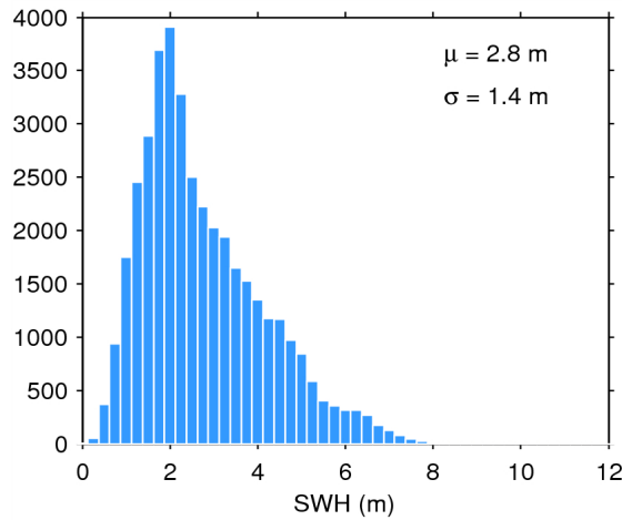
Figure 17. Histogram of flag-valid SWH over oceans and lakes for 17/07/2014. The mean ( \mu ) and standard deviation ( \sigma ) are also shown. Note that values larger than 12 m are excluded from the histogram for the sake of readability but not from the computation of \mu and \sigma .
