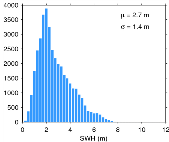
Figure 20. Histogram of science-valid SWH over oceans and lakes for 17/07/2014. The mean ( \mu ) and standard deviation ( \sigma ) are also shown. Note that values larger than 12 m are excluded from the histogram for the sake of readability but not from the computation of \mu and \sigma .
