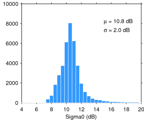
Figure 25. Histogram of flag-valid sigma0 over oceans and lakes for 17/07/2014. The mean ( \mu ) and standard deviation ( \sigma ) are also shown. Note that values outside [4 20] dB are excluded from the histogram for the sake of readability but not from the computation of \mu and \sigma .
