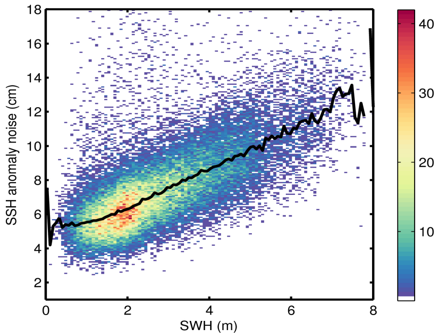
Figure 9. 2D histogram showing flag-valid SSH anomaly noise as a function of SWH for 17/07/2014. The black line denotes the median SSH anomaly as a function of SWH.
