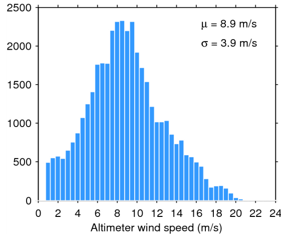
Figure 33. Histogram of flag-valid wind over oceans and lakes for 17/07/2014. The mean ( \mu ) and standard deviation ( \sigma ) are also shown. Note that values larger than 24 m/s are excluded from the histogram for the sake of readability but not from the computation of \mu and \sigma .
