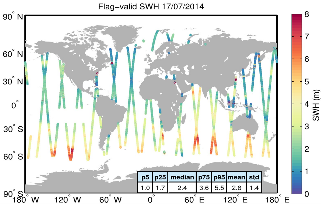
Figure 15. Geographical distribution of flag-valid SWH data over oceans and lakes for 17/07/2014. The statistical values shown in the table refer to the SWH in m and are calculated over all measurements shown in the figure.
