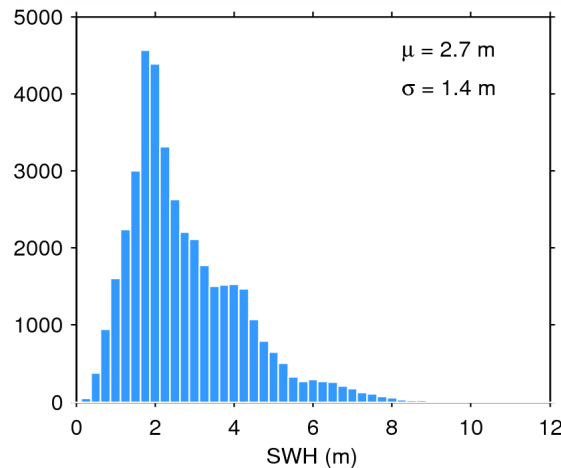
Figure 20. Histogram of science-valid SWH over oceans and lakes for 16/07/2014. The mean ( \mu ) and standard deviation ( \sigma ) are also shown. Note that values larger than 12 m are excluded from the histogram for the sake of readability but not from the computation of \mu and \sigma .
