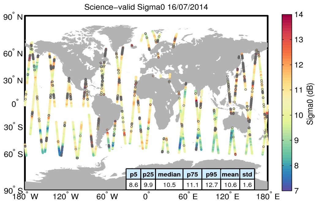
Figure 27. Geographical distribution of science-valid sigma0 data over oceans and lakes for 16/07/2014. The statistical values shown in the table refer to the sigma0 in dB and are calculated over all measurements shown in the figure. Gray circles denote records that have been rejected based on the editing criteria described in Table 4.
