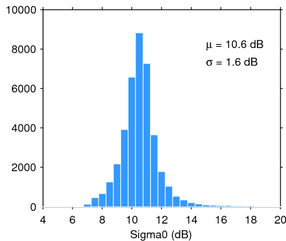
Figure 28. Histogram of science-valid sigma0 over oceans and lakes for 16/07/2014. The mean ( \mu ) and standard deviation ( \sigma ) are also shown. Note that values outside [4 20] dB are excluded from the histogram for the sake of readability but not from the computation of \mu and \sigma .
