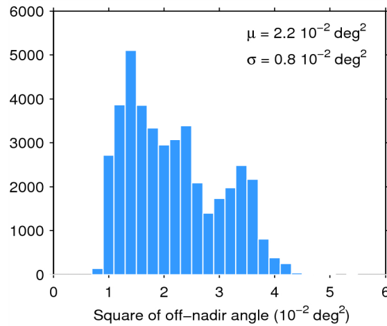
Figure 39. Histogram of flag-valid mispointing over oceans and lakes for 16/07/2014. The mean ( \mu ) and standard deviation ( \sigma ) are also shown. Note that values than 6 \cdot 10^{-2} \text{ deg}^2 are excluded from the histogram for the sake of readability but not from the computation of \mu and \sigma .
