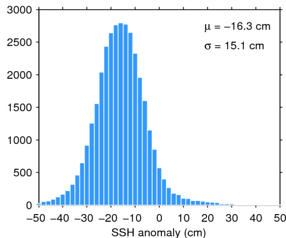
Figure 11. Histogram of science-valid SSH anomaly over oceans and lakes for 16/07/2014. The mean ( \mu ) and standard deviation ( \sigma ) are also shown. Note that values outside [-50 50] cm are excluded from the histogram for the sake of readability but not from the computation of \mu and \sigma .
