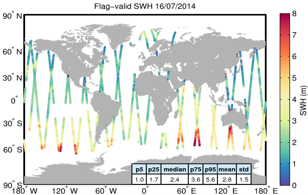
Figure 15. Geographical distribution of flag-valid SWH data over oceans and lakes for 16/07/2014. The statistical values shown in the table refer to the SWH in m and are calculated over all measurements shown in the figure.
