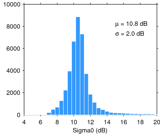
Figure 25. Histogram of flag-valid sigma0 over oceans and lakes for 16/07/2014. The mean ( \mu ) and standard deviation ( \sigma ) are also shown. Note that values outside [4 20] dB are excluded from the histogram for the sake of readability but not from the computation of \mu and \sigma .
