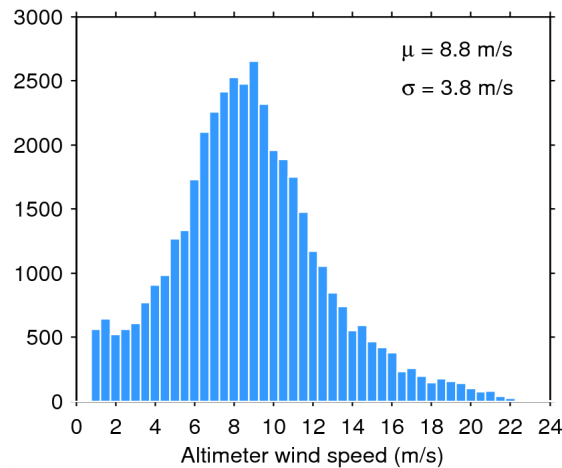
Figure 33. Histogram of flag-valid wind over oceans and lakes for 16/07/2014. The mean ( \mu ) and standard deviation ( \sigma ) are also shown. Note that values larger than 24 m/s are excluded from the histogram for the sake of readability but not from the computation of \mu and \sigma .
