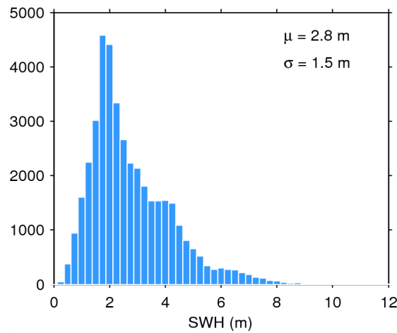
Figure 17. Histogram of flag-valid SWH over oceans and lakes for 16/07/2014. The mean ( \mu ) and standard deviation ( \sigma ) are also shown. Note that values larger than 12 m are excluded from the histogram for the sake of readability but not from the computation of \mu and \sigma .
