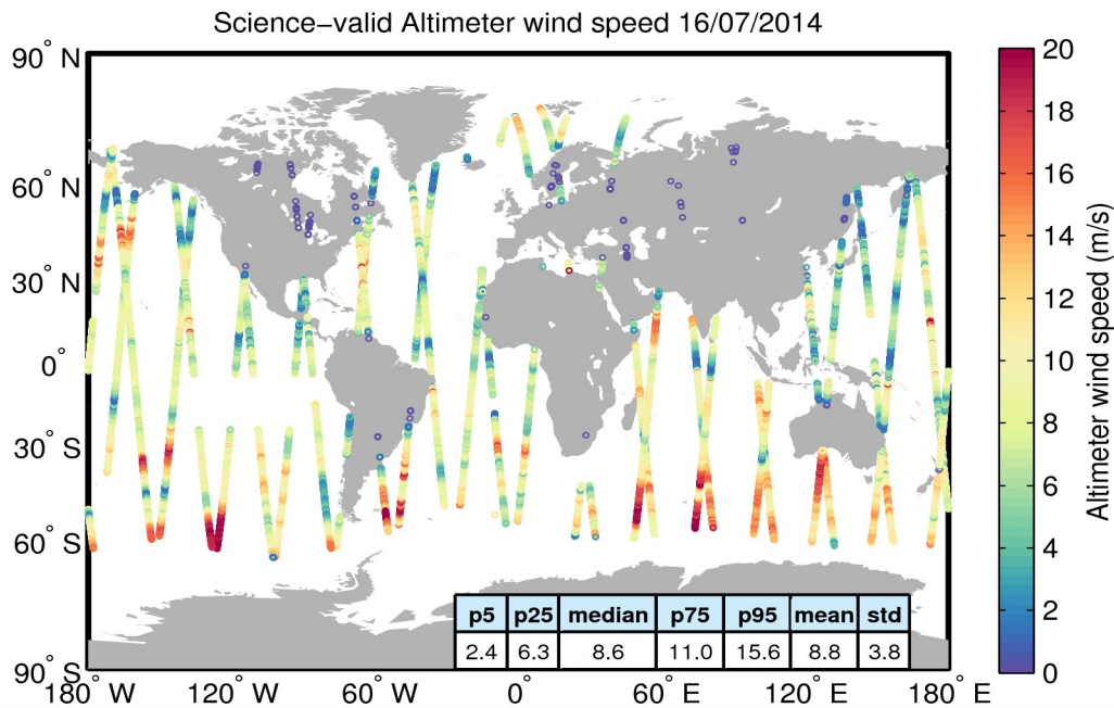
Figure 34. Geographical distribution of science-valid wind data over oceans and lakes for 16/07/2014. The statistical values shown in the table refer to the wind in m/s and are calculated over all measurements shown in the figure. Gray circles denote records that have been rejected based on the editing criteria described in Table 5.
