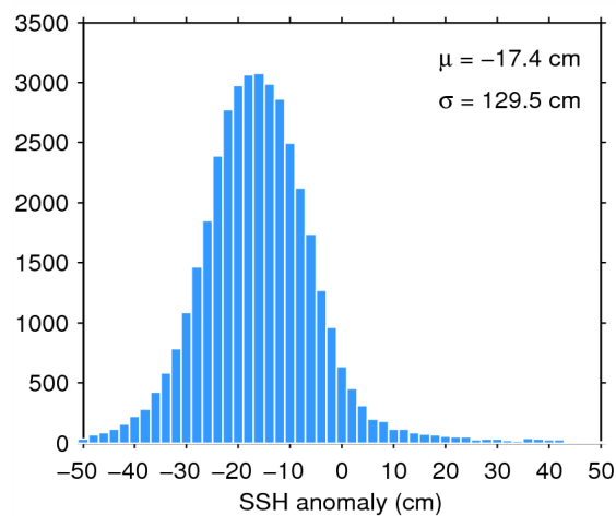
Figure 7. Histogram of flag-valid SSH anomaly over oceans and lakes for 16/07/2014. The mean ( \mu ) and standard deviation ( \sigma ) are also shown. Note that values outside [-50 50] cm are excluded from the histogram for the sake of readability but not from the computation of \mu and \sigma .
