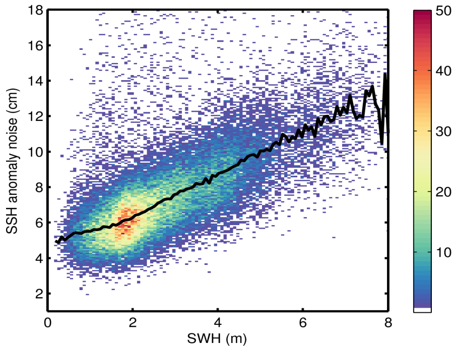
Figure 9. 2D histogram showing flag-valid SSH anomaly noise as a function of SWH for 16/07/2014. The black line denotes the median SSH anomaly as a function of SWH.
