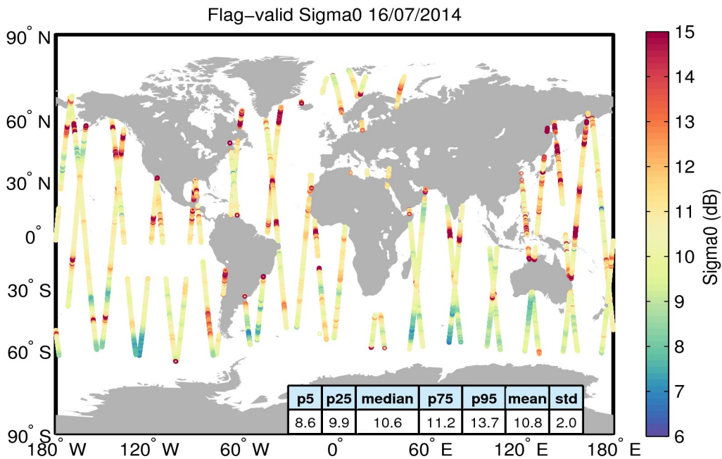
Figure 23. Geographical distribution of flag-valid sigma0 data over oceans and lakes for 16/07/2014. The statistical values shown in the table refer to the sigma0 in dB and are calculated over all measurements shown in the figure.
