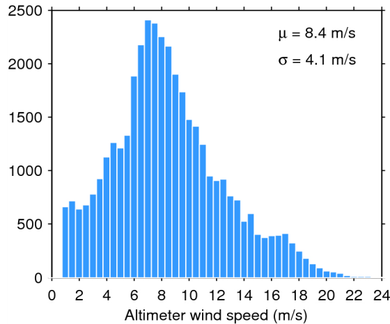
Figure 33. Histogram of flag-valid wind over oceans and lakes for 14/07/2014. The mean ( \mu ) and standard deviation ( \sigma ) are also shown. Note that values larger than 24 m/s are excluded from the histogram for the sake of readability but not from the computation of \mu and \sigma .
