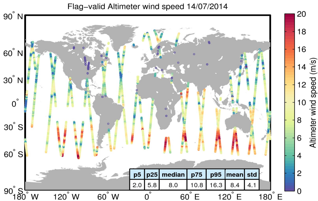
Figure 31. Geographical distribution of flag-valid wind data over oceans and lakes for 14/07/2014. The statistical values shown in the table refer to the wind in m/s and are calculated over all measurements shown in the figure.
