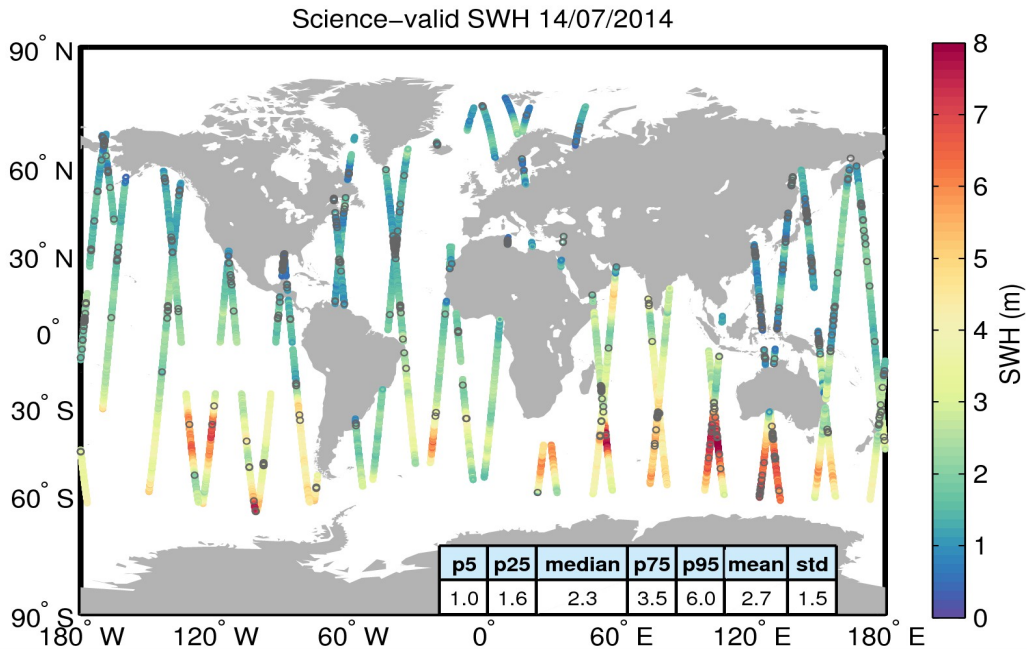
Figure 19. Geographical distribution of science-valid SWH data over oceans and lakes for 14/07/2014. The statistical values shown in the table refer to the SWH in m and are calculated over all measurements shown in the figure. Gray circles denote records that have been rejected based on the editing criteria described in Table 3.
