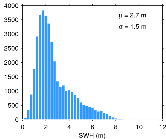
Figure 20. Histogram of science-valid SWH over oceans and lakes for 14/07/2014. The mean ( \mu ) and standard deviation ( \sigma ) are also shown. Note that values larger than 12 m are excluded from the histogram for the sake of readability but not from the computation of \mu and \sigma .
