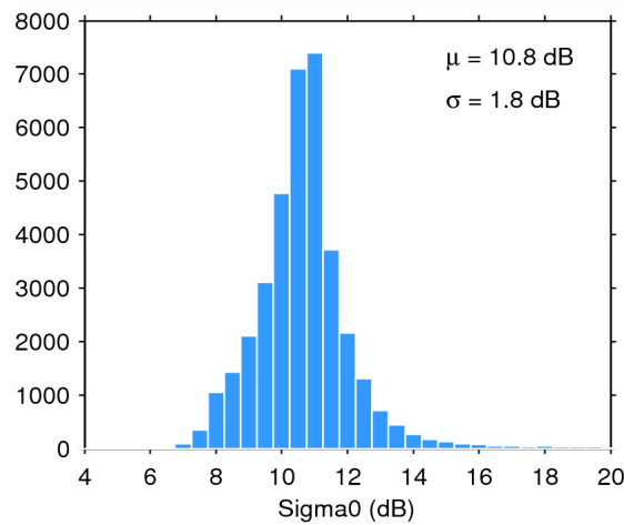
Figure 28. Histogram of science-valid sigma0 over oceans and lakes for 14/07/2014. The mean ( \mu ) and standard deviation ( \sigma ) are also shown. Note that values outside [4 20] dB are excluded from the histogram for the sake of readability but not from the computation of \mu and \sigma .
