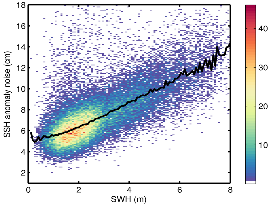
Figure 9. 2D histogram showing flag-valid SSH anomaly noise as a function of SWH for 14/07/2014. The black line denotes the median SSH anomaly as a function of SWH.
