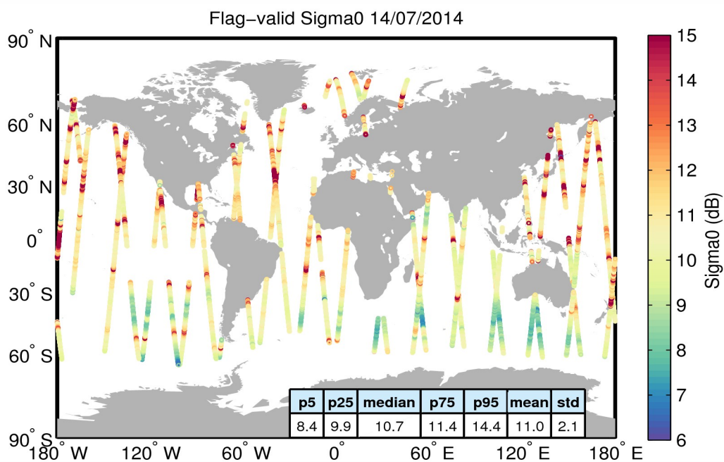
Figure 23. Geographical distribution of flag-valid sigma0 data over oceans and lakes for 14/07/2014. The statistical values shown in the table refer to the sigma0 in dB and are calculated over all measurements shown in the figure.
