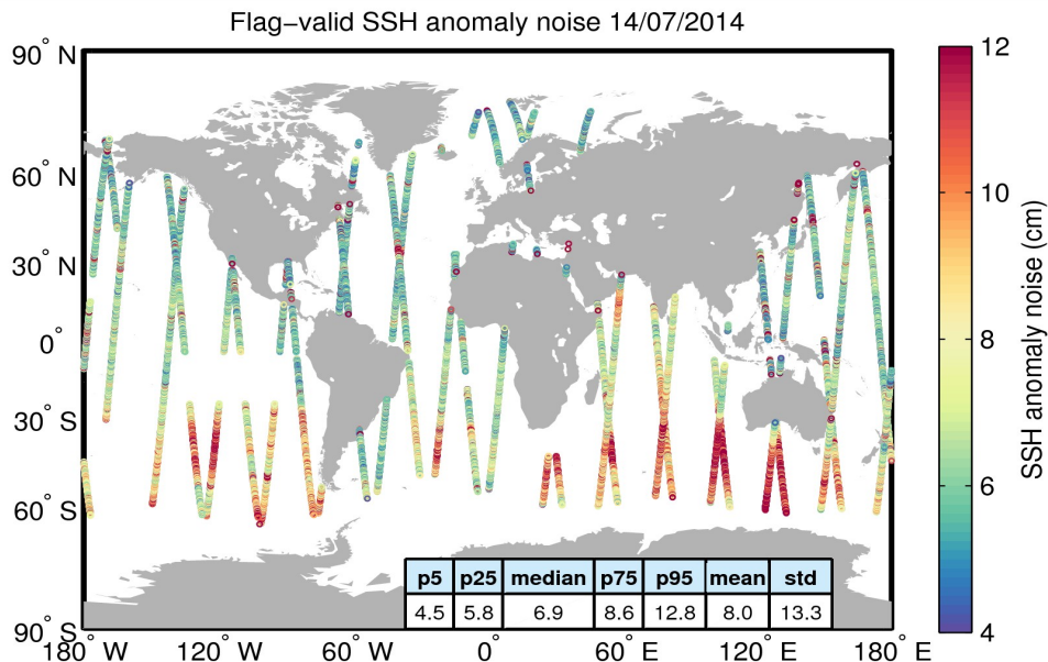
Figure 8. Geographical distribution of flag-valid 20-Hz SSH anomaly measurement noise over oceans and lakes for 14/07/2014. The statistical values shown in the table refer to the SSH anomaly noise and are calculated over all measurements shown in the figure.
