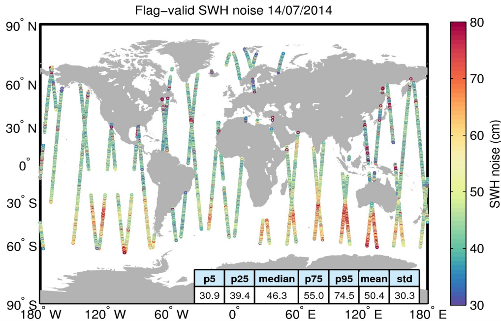
Figure 18. Geographical distribution of flag-valid 20-Hz SWH measurement noise over oceans and lakes for 14/07/2014. The statistical values shown in the figure refer to the SWH noise and are calculated over all measurements shown in the figure.
