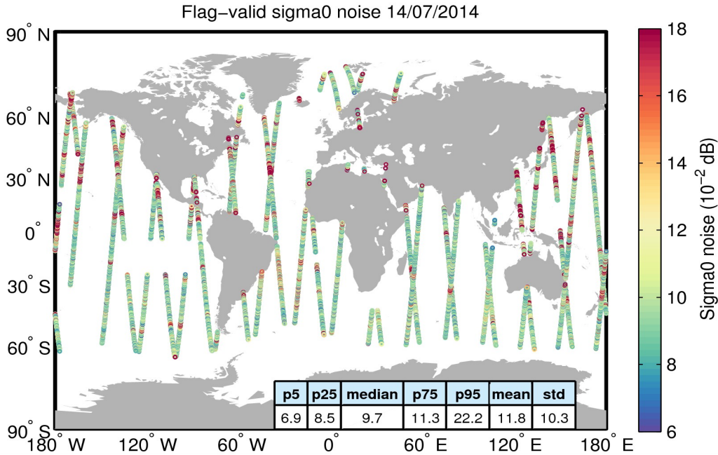
Figure 26. Geographical distribution of flag-valid 20-Hz sigma0 measurement noise over oceans and lakes for 14/07/2014. The statistical values shown in the table refer to the sigma0 noise and are calculated over all measurements shown in the figure.
