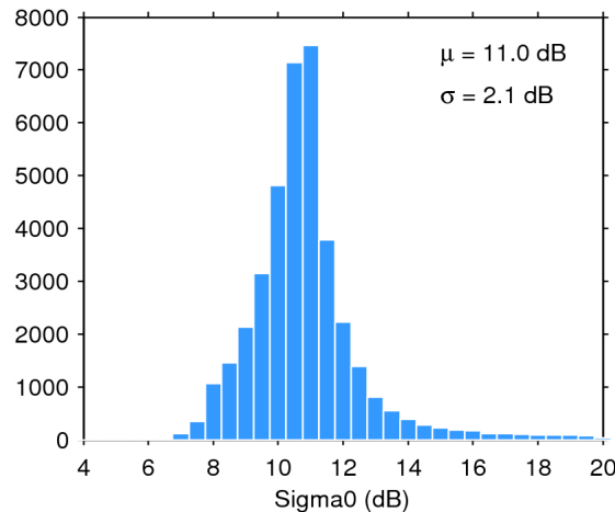
Figure 25. Histogram of flag-valid sigma0 over oceans and lakes for 14/07/2014. The mean ( \mu ) and standard deviation ( \sigma ) are also shown. Note that values outside [4 20] dB are excluded from the histogram for the sake of readability but not from the computation of \mu and \sigma .
