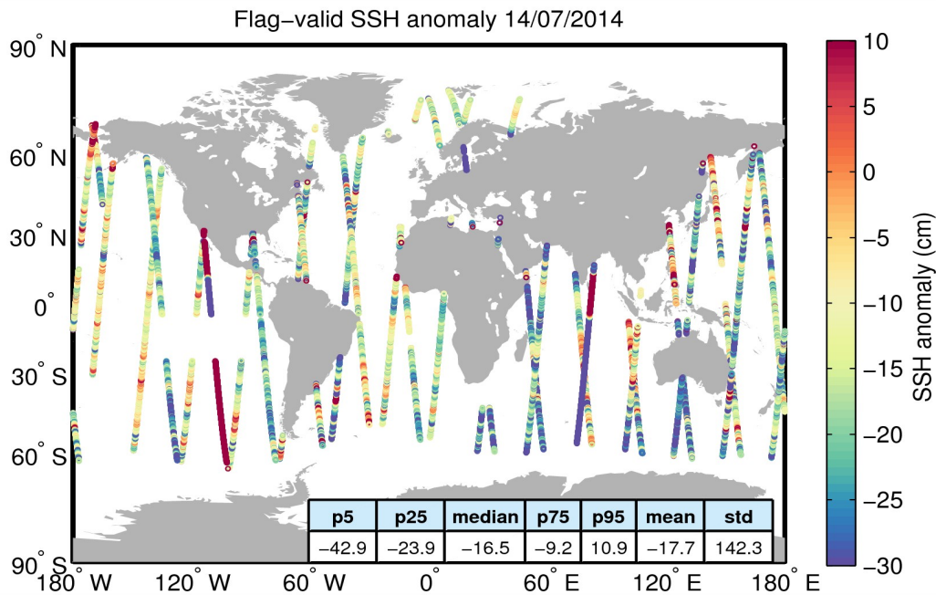
Figure 5. Geographical distribution of flag-valid 1-Hz SSH anomaly data over oceans and lakes for 14/07/2014. The statistical values shown in the table refer to the SSH anomaly in cm and are calculated over all measurements shown in the figure.
