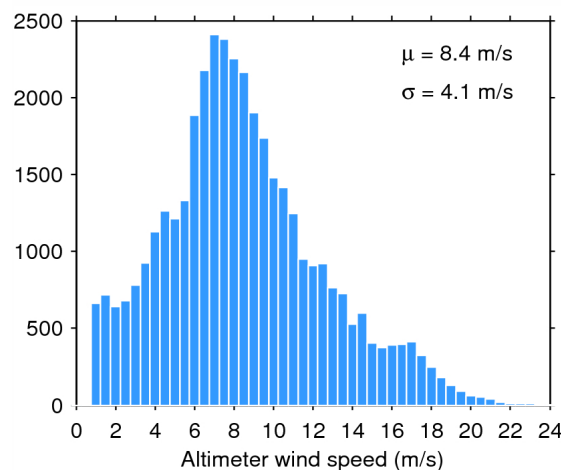
Figure 35. Histogram of science-valid wind over oceans and lakes for 14/07/2014. The mean ( \mu ) and standard deviation ( \sigma ) are also shown. Note that values larger than 24 m/s are excluded from the histogram for the sake of readability but not from the computation of \mu and \sigma .
