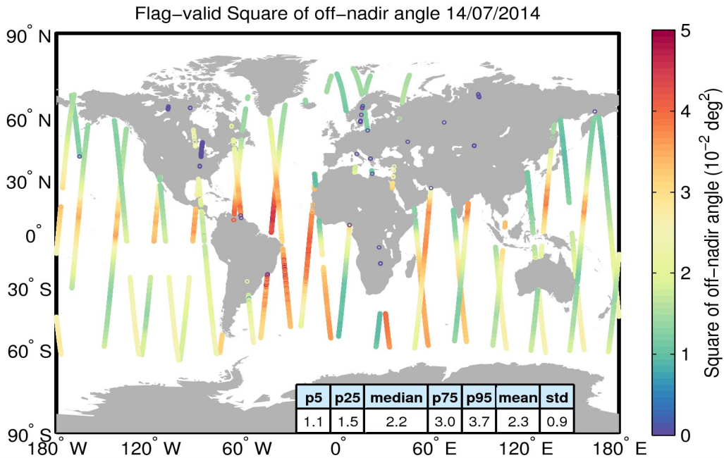
Figure 37. Geographical distribution of flag-valid mispointing data over oceans and lakes for 14/07/2014. The statistical values shown in the table refer to the mispointing in 10^{-2} \text{ deg}^2 and are calculated over all measurements shown in the figure.
