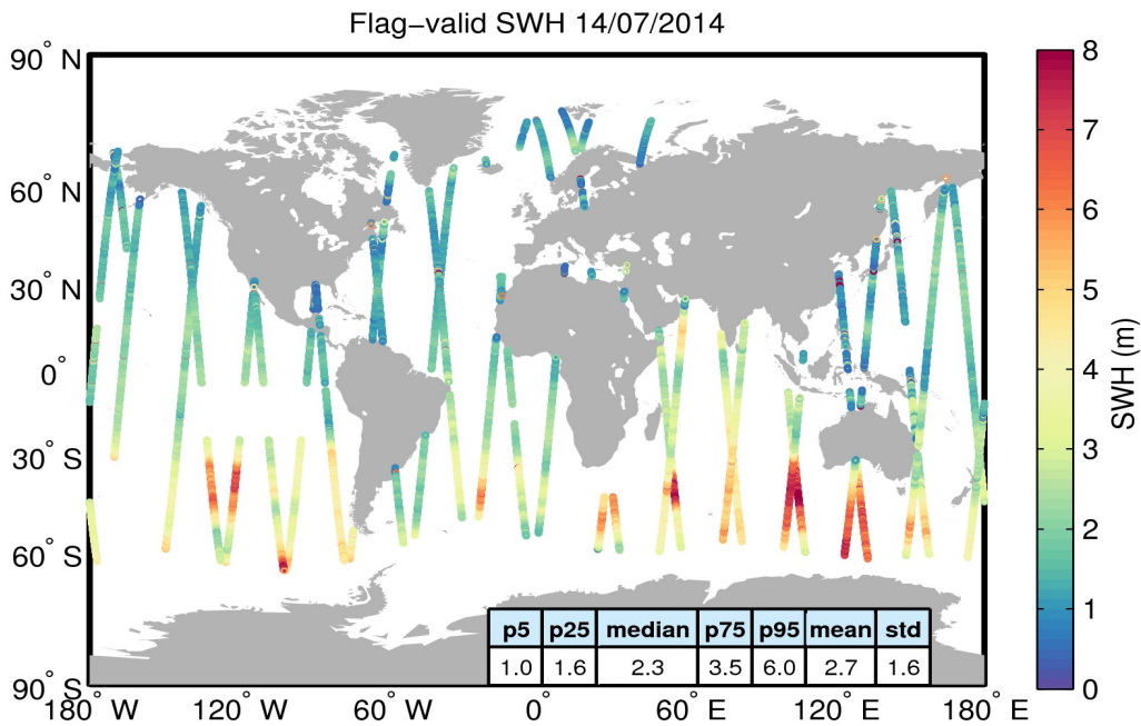
Figure 15. Geographical distribution of flag-valid SWH data over oceans and lakes for 14/07/2014. The statistical values shown in the table refer to the SWH in m and are calculated over all measurements shown in the figure.
