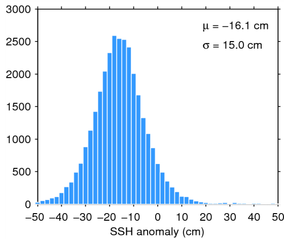
Figure 11. Histogram of science-valid SSH anomaly over oceans and lakes for 14/07/2014. The mean ( \mu ) and standard deviation ( \sigma ) are also shown. Note that values outside [-50 50] cm are excluded from the histogram for the sake of readability but not from the computation of \mu and \sigma .
