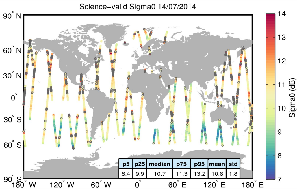
Figure 27. Geographical distribution of science-valid sigma0 data over oceans and lakes for 14/07/2014. The statistical values shown in the table refer to the sigma0 in dB and are calculated over all measurements shown in the figure. Gray circles denote records that have been rejected based on the editing criteria described in Table 4.
