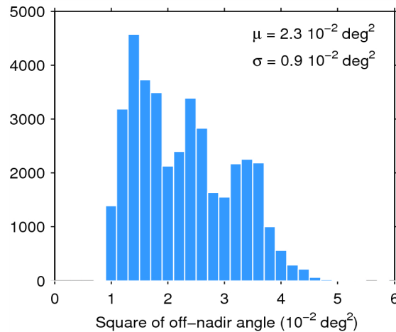
Figure 39. Histogram of flag-valid mispointing over oceans and lakes for 14/07/2014. The mean ( \mu ) and standard deviation ( \sigma ) are also shown. Note that values than 6 \cdot 10^{-2} \text{ deg}^2 are excluded from the histogram for the sake of readability but not from the computation of \mu and \sigma .
