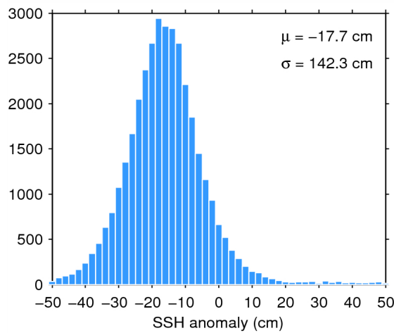
Figure 7. Histogram of flag-valid SSH anomaly over oceans and lakes for 14/07/2014. The mean ( \mu ) and standard deviation ( \sigma ) are also shown. Note that values outside [-50\ 50] cm are excluded from the histogram for the sake of readability but not from the computation of \mu and \sigma .
