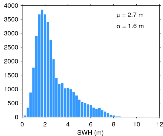
Figure 17. Histogram of flag-valid SWH over oceans and lakes for 14/07/2014. The mean ( \mu ) and standard deviation ( \sigma ) are also shown. Note that values larger than 12 m are excluded from the histogram for the sake of readability but not from the computation of \mu and \sigma .
