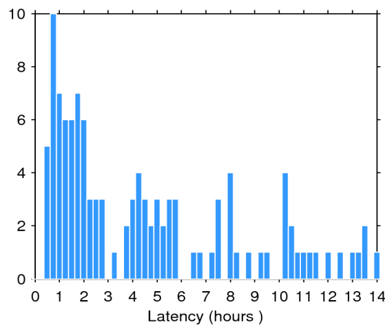
Figure 2. Histogram of the data latency for 14/07/2014. The y-axis denotes the number of files that are made available with a delay of x-hours with respect to the mean time of the records stored in the file.
