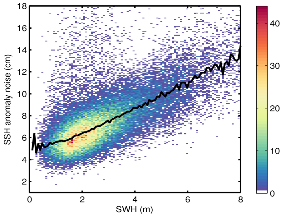
Figure 9. 2D histogram showing flag-valid SSH anomaly noise as a function of SWH for 13/07/2014. The black line denotes the median SSH anomaly as a function of SWH.
