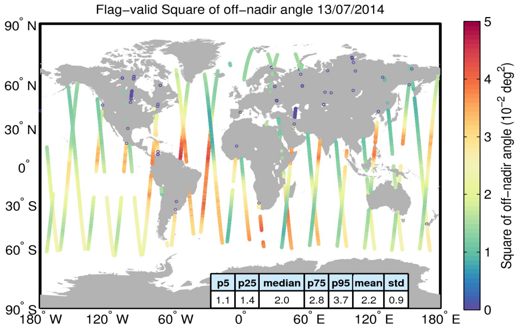
Figure 37. Geographical distribution of flag-valid mispointing data over oceans and lakes for 13/07/2014. The statistical values shown in the table refer to the mispointing in 10^{-2} \text{deg}^2 and are calculated over all measurements shown in the figure.
