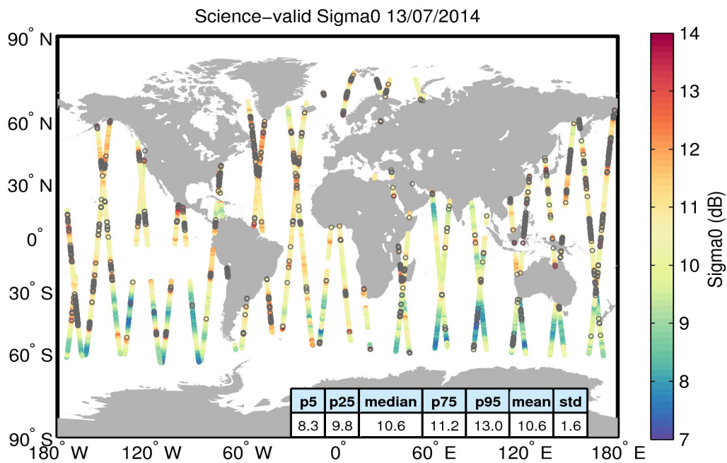
Figure 27. Geographical distribution of science-valid sigma0 data over oceans and lakes for 13/07/2014. The statistical values shown in the table refer to the sigma0 in dB and are calculated over all measurements shown in the figure. Gray circles denote records that have been rejected based on the editing criteria described in Table 4.
