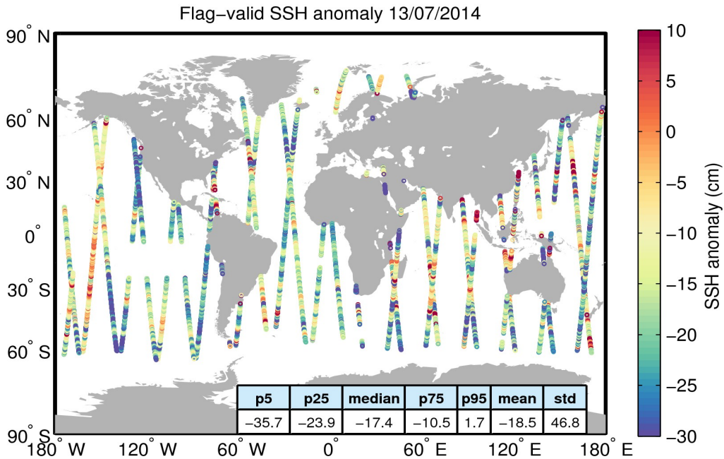
Figure 5. Geographical distribution of flag-valid 1-Hz SSH anomaly data over oceans and lakes for 13/07/2014. The statistical values shown in the table refer to the SSH anomaly in cm and are calculated over all measurements shown in the figure.
