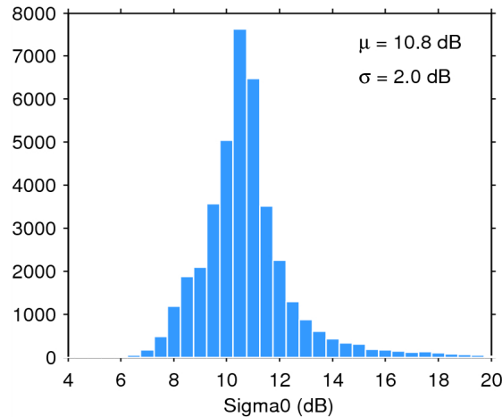
Figure 25. Histogram of flag-valid sigma0 over oceans and lakes for 13/07/2014. The mean ( \mu ) and standard deviation ( \sigma ) are also shown. Note that values outside [4 20] dB are excluded from the histogram for the sake of readability but not from the computation of \mu and \sigma .
