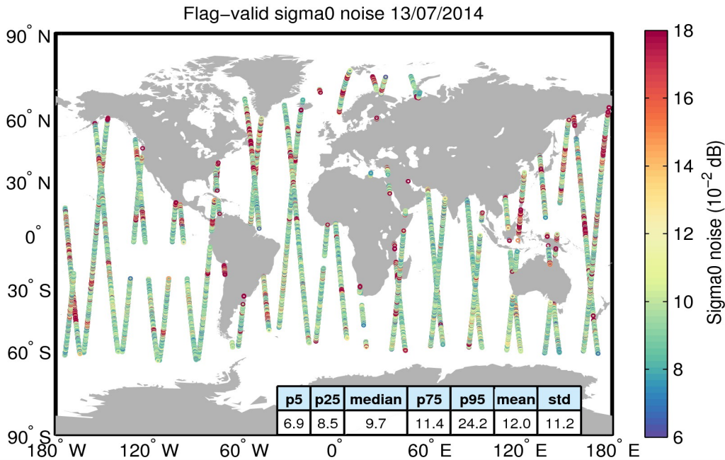
Figure 26. Geographical distribution of flag-valid 20-Hz sigma0 measurement noise over oceans and lakes for 13/07/2014. The statistical values shown in the table refer to the sigma0 noise and are calculated over all measurements shown in the figure.
