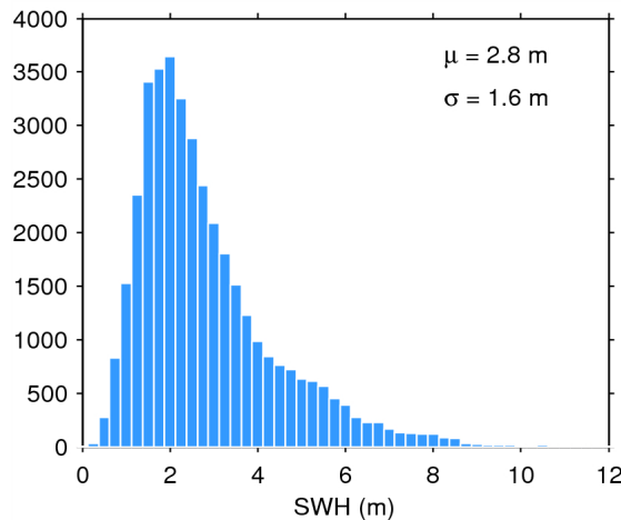
Figure 20. Histogram of science-valid SWH over oceans and lakes for 13/07/2014. The mean ( \mu ) and standard deviation ( \sigma ) are also shown. Note that values larger than 12 m are excluded from the histogram for the sake of readability but not from the computation of \mu and \sigma .
