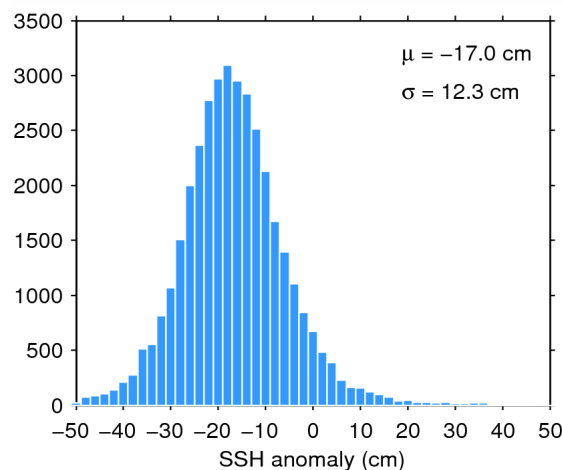
Figure 11. Histogram of science-valid SSH anomaly over oceans and lakes for 13/07/2014. The mean ( \mu ) and standard deviation ( \sigma ) are also shown. Note that values outside [-50 50] cm are excluded from the histogram for the sake of readability but not from the computation of \mu and \sigma .
