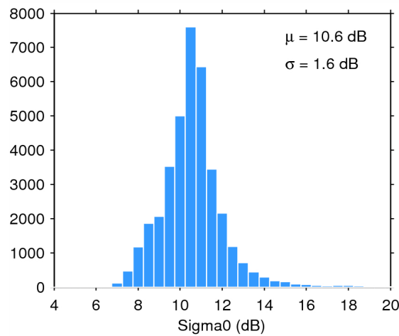
Figure 28. Histogram of science-valid sigma0 over oceans and lakes for 13/07/2014. The mean ( \mu ) and standard deviation ( \sigma ) are also shown. Note that values outside [4 20] dB are excluded from the histogram for the sake of readability but not from the computation of \mu and \sigma .
