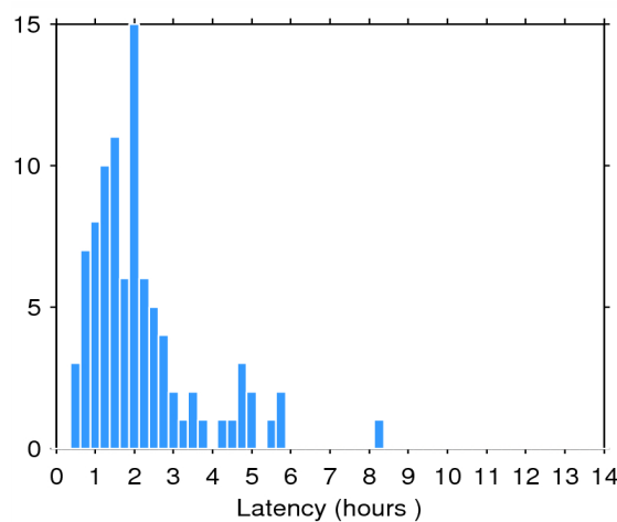
Figure 2. Histogram of the data latency for 13/07/2014. The y-axis denotes the number of files that are made available with a delay of x-hours with respect to the mean time of the records stored in the file.
