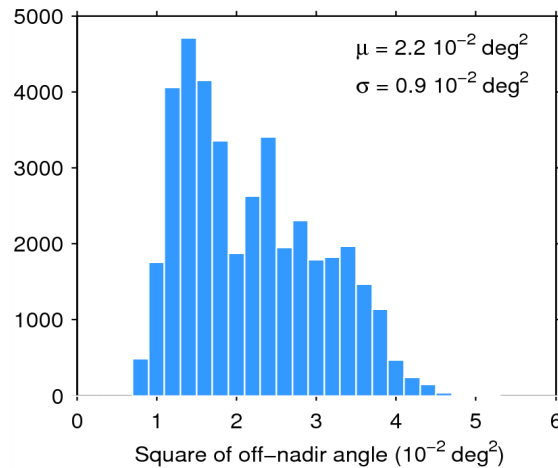
Figure 39. Histogram of flag-valid mispointing over oceans and lakes for 13/07/2014. The mean ( \mu ) and standard deviation ( \sigma ) are also shown. Note that values than 6 \cdot 10^{-2} \text{ deg}^2 are excluded from the histogram for the sake of readability but not from the computation of \mu and \sigma .
