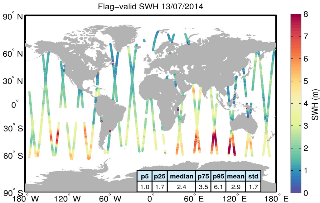
Figure 15. Geographical distribution of flag-valid SWH data over oceans and lakes for 13/07/2014. The statistical values shown in the table refer to the SWH in m and are calculated over all measurements shown in the figure.
