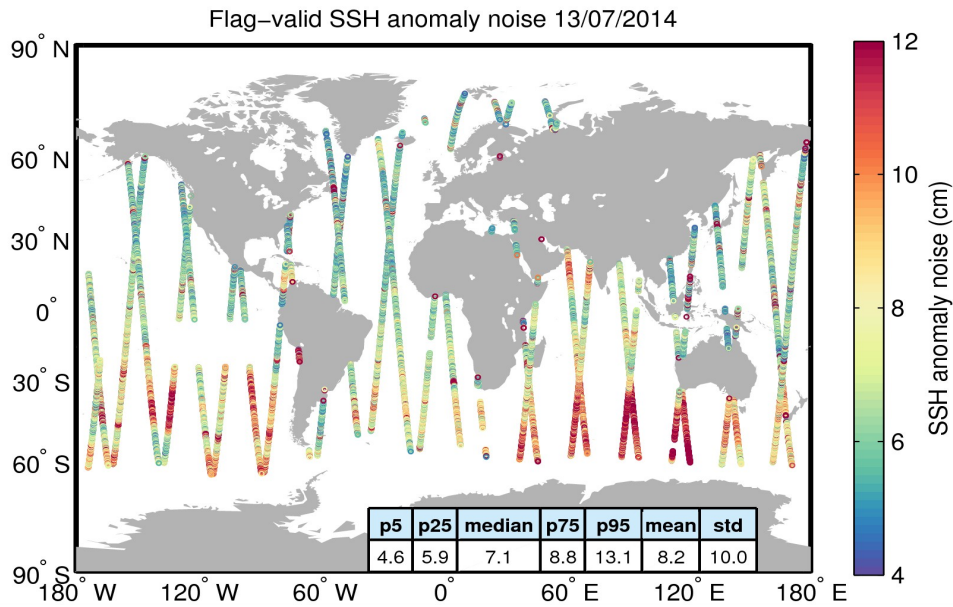
Figure 8. Geographical distribution of flag-valid 20-Hz SSH anomaly measurement noise over oceans and lakes for 13/07/2014. The statistical values shown in the table refer to the SSH anomaly noise and are calculated over all measurements shown in the figure.
