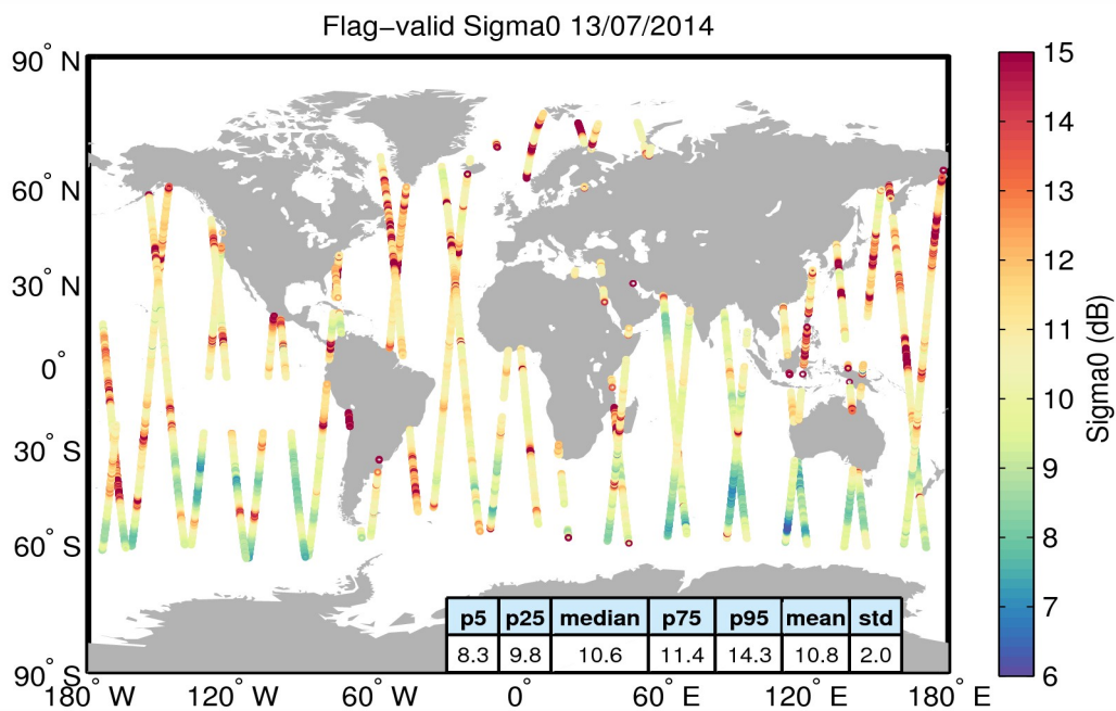
Figure 23. Geographical distribution of flag-valid sigma0 data over oceans and lakes for 13/07/2014. The statistical values shown in the table refer to the sigma0 in dB and are calculated over all measurements shown in the figure.
