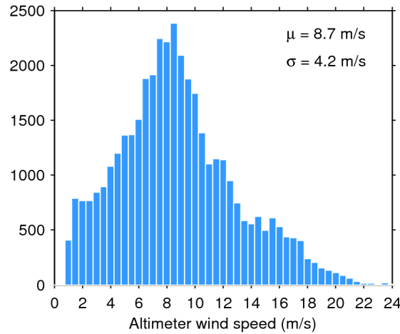
Figure 33. Histogram of flag-valid wind over oceans and lakes for 13/07/2014. The mean ( \mu ) and standard deviation ( \sigma ) are also shown. Note that values larger than 24 m/s are excluded from the histogram for the sake of readability but not from the computation of \mu and \sigma .
