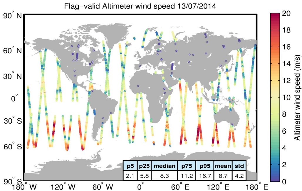
Figure 31. Geographical distribution of flag-valid wind data over oceans and lakes for 13/07/2014. The statistical values shown in the table refer to the wind in m/s and are calculated over all measurements shown in the figure.
