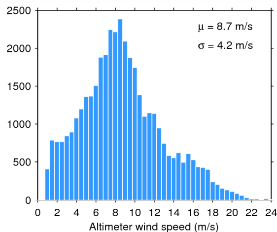
Figure 35. Histogram of science-valid wind over oceans and lakes for 13/07/2014. The mean ( \mu ) and standard deviation ( \sigma ) are also shown. Note that values larger than 24 m/s are excluded from the histogram for the sake of readability but not from the computation of \mu and \sigma .
