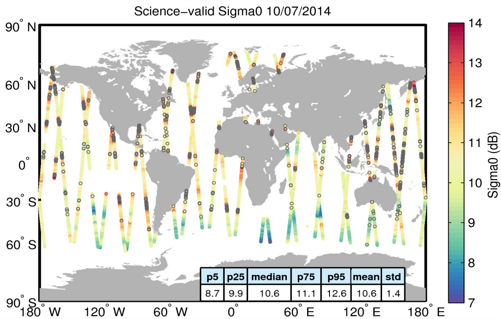
Figure 27. Geographical distribution of science-valid sigma0 data over oceans and lakes for 10/07/2014. The statistical values shown in the table refer to the sigma0 in dB and are calculated over all measurements shown in the figure. Gray circles denote records that have been rejected based on the editing criteria described in Table 4.
