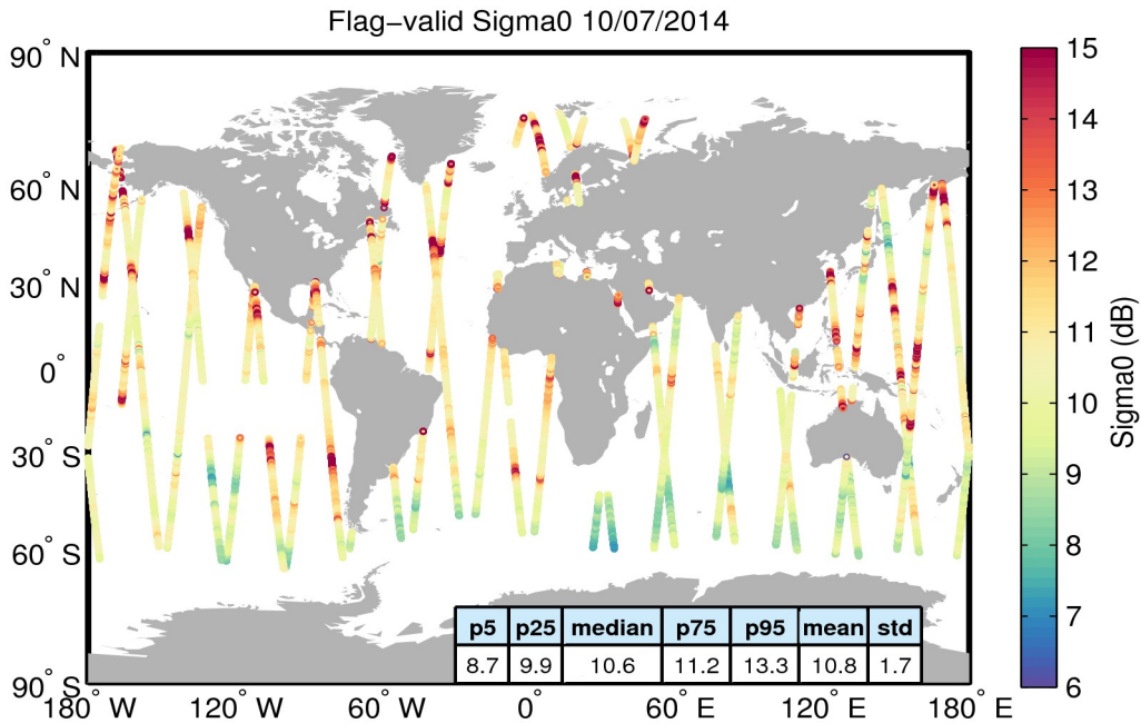
Figure 23. Geographical distribution of flag-valid sigma0 data over oceans and lakes for 10/07/2014. The statistical values shown in the table refer to the sigma0 in dB and are calculated over all measurements shown in the figure.
