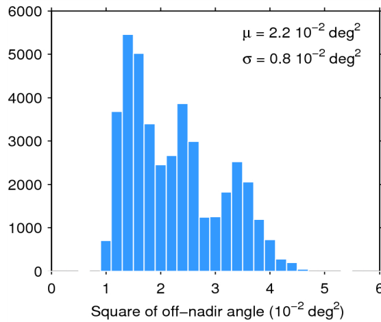
Figure 39. Histogram of flag-valid mispointing over oceans and lakes for 10/07/2014. The mean ( \mu ) and standard deviation ( \sigma ) are also shown. Note that values than 6 \cdot 10^{-2} \text{ deg}^2 are excluded from the histogram for the sake of readability but not from the computation of \mu and \sigma .
