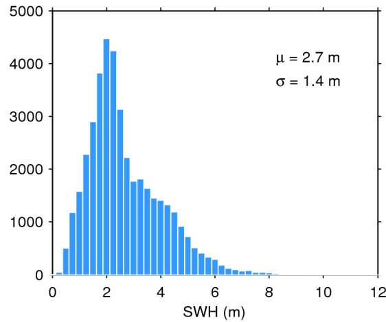
Figure 17. Histogram of flag-valid SWH over oceans and lakes for 10/07/2014. The mean ( \mu ) and standard deviation ( \sigma ) are also shown. Note that values larger than 12 m are excluded from the histogram for the sake of readability but not from the computation of \mu and \sigma .
