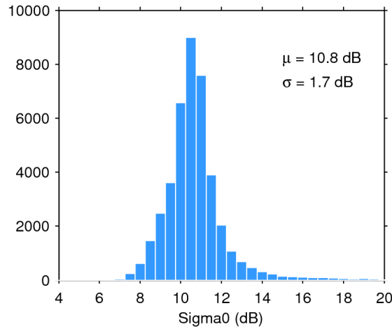
Figure 25. Histogram of flag-valid sigma0 over oceans and lakes for 10/07/2014. The mean ( \mu ) and standard deviation ( \sigma ) are also shown. Note that values outside [4 20] dB are excluded from the histogram for the sake of readability but not from the computation of \mu and \sigma .
