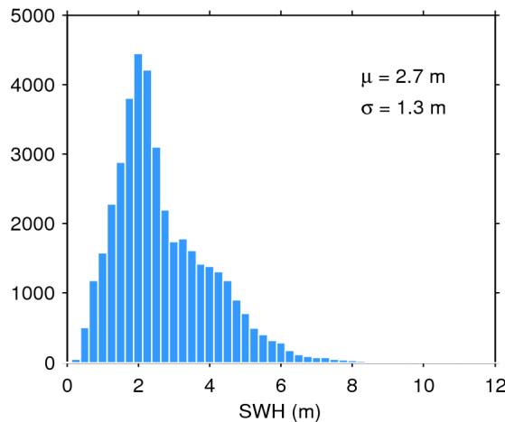
Figure 20. Histogram of science-valid SWH over oceans and lakes for 10/07/2014. The mean ( \mu ) and standard deviation ( \sigma ) are also shown. Note that values larger than 12 m are excluded from the histogram for the sake of readability but not from the computation of \mu and \sigma .
