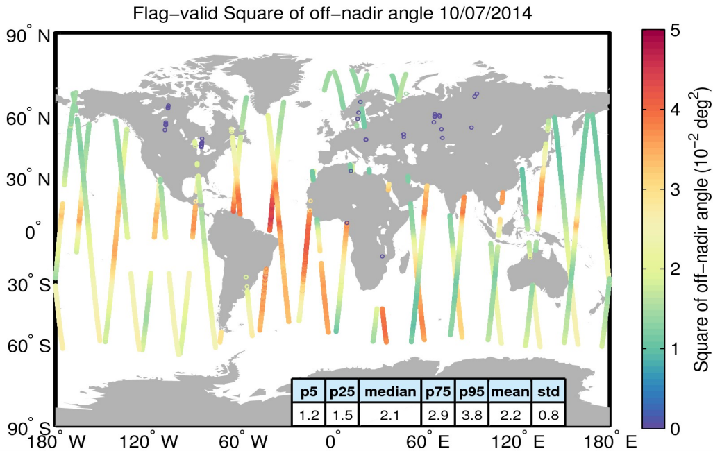
Figure 37. Geographical distribution of flag-valid mispointing data over oceans and lakes for 10/07/2014. The statistical values shown in the table refer to the mispointing in 10^{-2} \text{deg}^2 and are calculated over all measurements shown in the figure.
