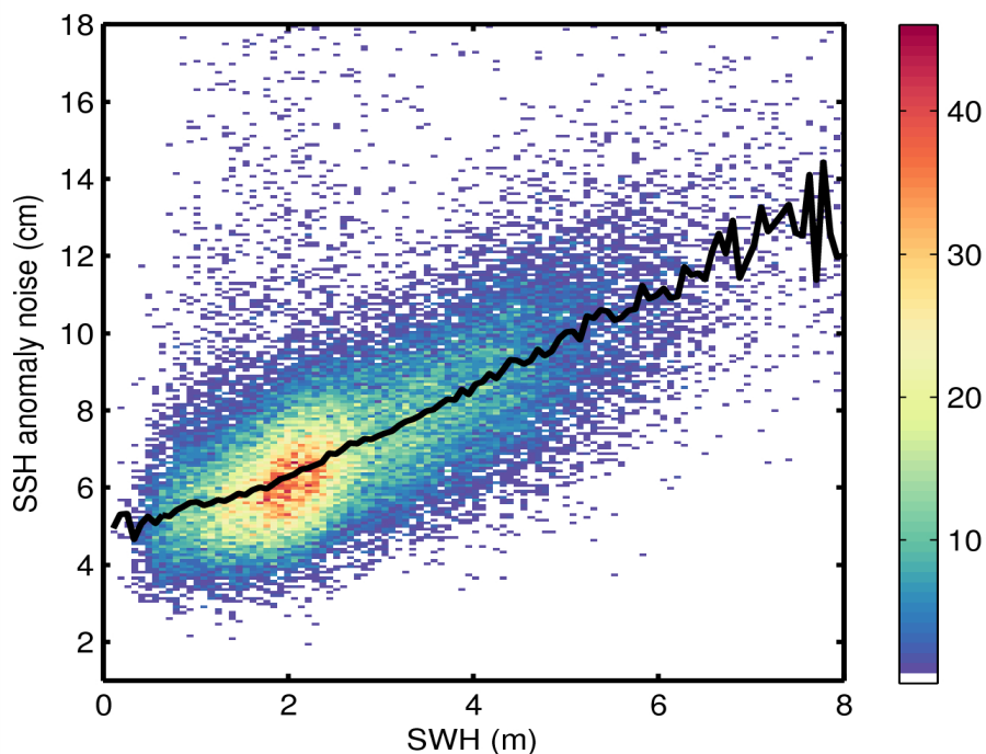
Figure 9. 2D histogram showing flag-valid SSH anomaly noise as a function of SWH for 10/07/2014. The black line denotes the median SSH anomaly as a function of SWH.
