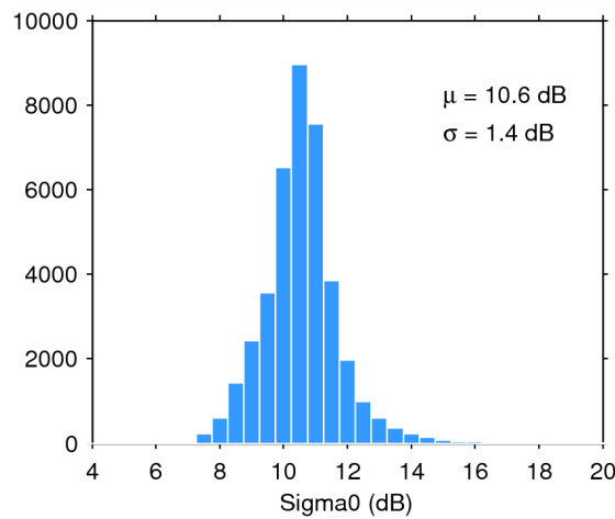
Figure 28. Histogram of science-valid sigma0 over oceans and lakes for 10/07/2014. The mean ( \mu ) and standard deviation ( \sigma ) are also shown. Note that values outside [4 20] dB are excluded from the histogram for the sake of readability but not from the computation of \mu and \sigma .
