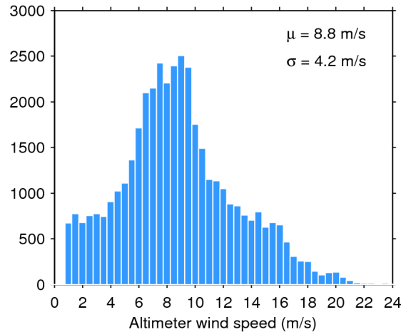
Figure 33. Histogram of flag-valid wind over oceans and lakes for 08/07/2014. The mean ( \mu ) and standard deviation ( \sigma ) are also shown. Note that values larger than 24 m/s are excluded from the histogram for the sake of readability but not from the computation of \mu and \sigma .
