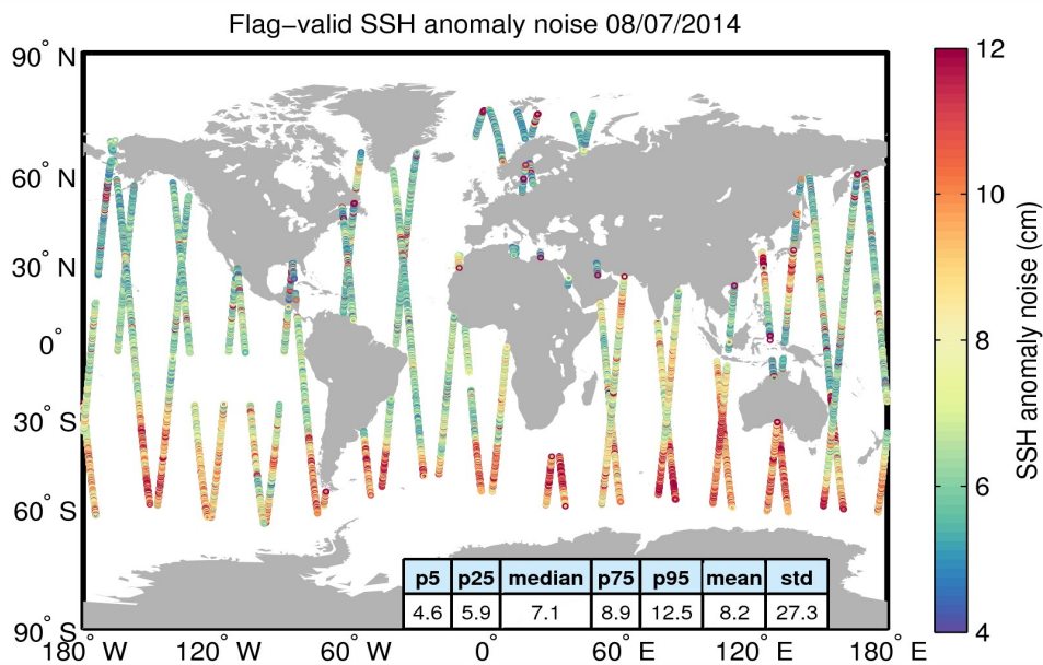
Figure 8. Geographical distribution of flag-valid 20-Hz SSH anomaly measurement noise over oceans and lakes for 08/07/2014. The statistical values shown in the table refer to the SSH anomaly noise and are calculated over all measurements shown in the figure.
