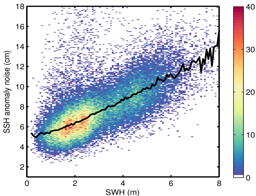
Figure 9. 2D histogram showing flag-valid SSH anomaly noise as a function of SWH for 08/07/2014. The black line denotes the median SSH anomaly as a function of SWH.
