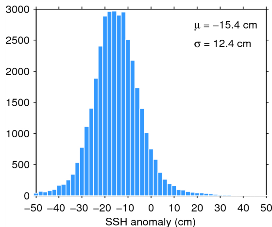
Figure 11. Histogram of science-valid SSH anomaly over oceans and lakes for 08/07/2014. The mean ( \mu ) and standard deviation ( \sigma ) are also shown. Note that values outside [-50 50] cm are excluded from the histogram for the sake of readability but not from the computation of \mu and \sigma .
