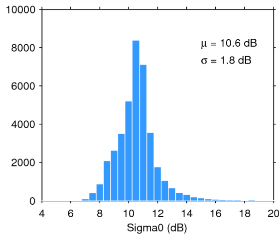
Figure 28. Histogram of science-valid sigma0 over oceans and lakes for 08/07/2014. The mean ( \mu ) and standard deviation ( \sigma ) are also shown. Note that values outside [4 20] dB are excluded from the histogram for the sake of readability but not from the computation of \mu and \sigma .
