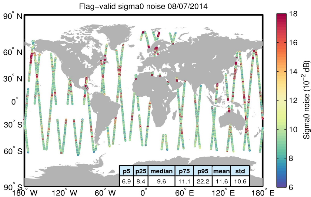
Figure 26. Geographical distribution of flag-valid 20-Hz sigma0 measurement noise over oceans and lakes for 08/07/2014. The statistical values shown in the table refer to the sigma0 noise and are calculated over all measurements shown in the figure.
