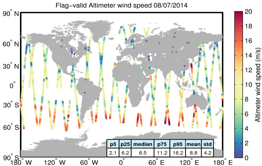
Figure 31. Geographical distribution of flag-valid wind data over oceans and lakes for 08/07/2014. The statistical values shown in the table refer to the wind in m/s and are calculated over all measurements shown in the figure.
