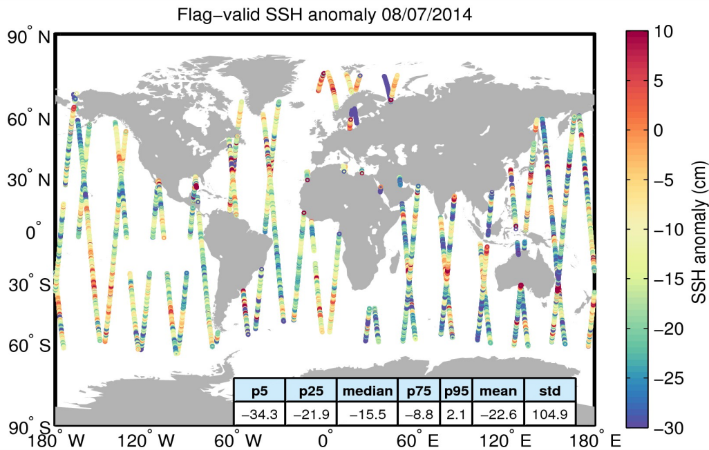
Figure 5. Geographical distribution of flag-valid 1-Hz SSH anomaly data over oceans and lakes for 08/07/2014. The statistical values shown in the table refer to the SSH anomaly in cm and are calculated over all measurements shown in the figure.
