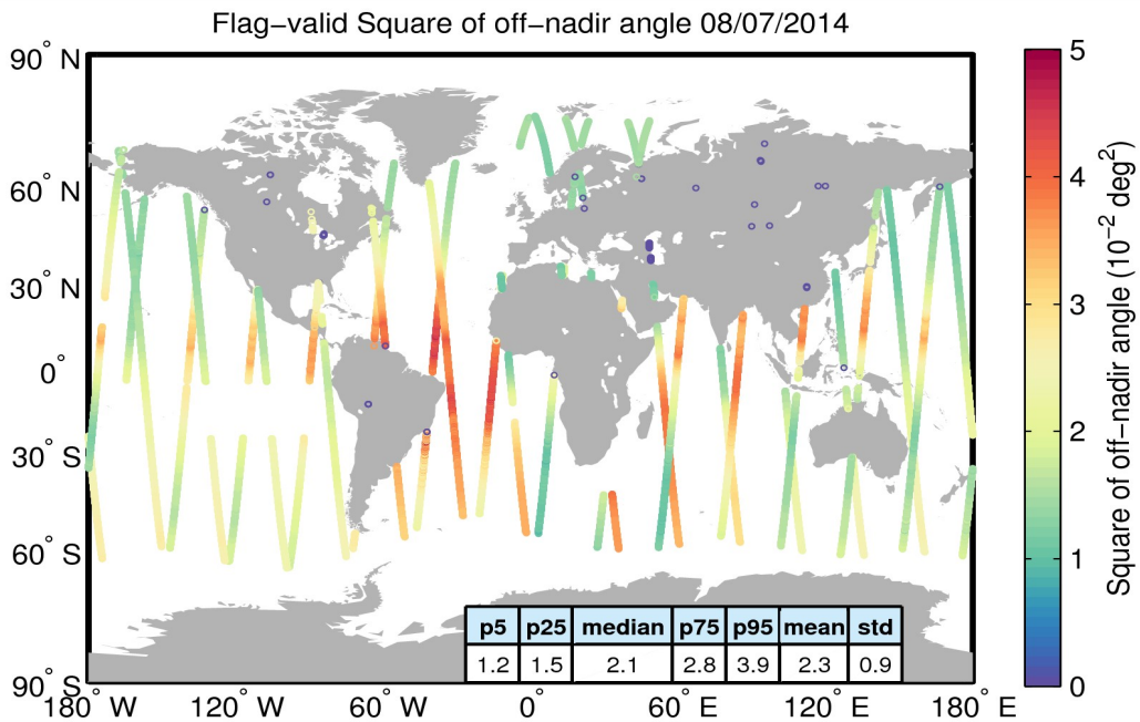
Figure 37. Geographical distribution of flag-valid mispointing data over oceans and lakes for 08/07/2014. The statistical values shown in the table refer to the mispointing in 10^{-2} \text{ deg}^2 and are calculated over all measurements shown in the figure.
