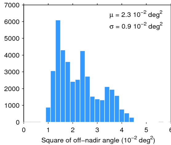
Figure 39. Histogram of flag-valid mispointing over oceans and lakes for 08/07/2014. The mean ( \mu ) and standard deviation ( \sigma ) are also shown. Note that values than 6 \cdot 10^{-2} \text{ deg}^2 are excluded from the histogram for the sake of readability but not from the computation of \mu and \sigma .
