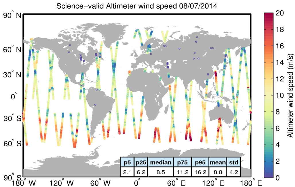
Figure 34. Geographical distribution of science-valid wind data over oceans and lakes for 08/07/2014. The statistical values shown in the table refer to the wind in m/s and are calculated over all measurements shown in the figure. Gray circles denote records that have been rejected based on the editing criteria described in Table 5.
