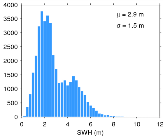
Figure 20. Histogram of science-valid SWH over oceans and lakes for 08/07/2014. The mean ( \mu ) and standard deviation ( \sigma ) are also shown. Note that values larger than 12 m are excluded from the histogram for the sake of readability but not from the computation of \mu and \sigma .
