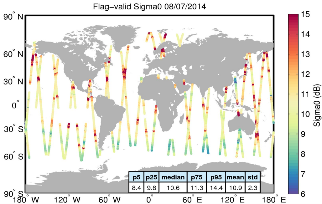
Figure 23. Geographical distribution of flag-valid sigma0 data over oceans and lakes for 08/07/2014. The statistical values shown in the table refer to the sigma0 in dB and are calculated over all measurements shown in the figure.
