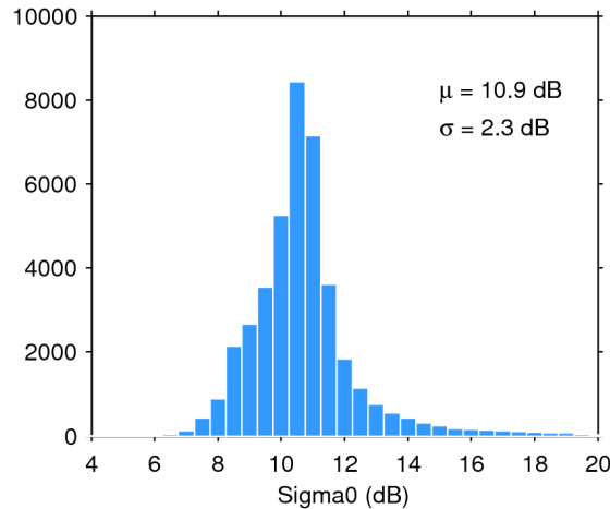
Figure 25. Histogram of flag-valid sigma0 over oceans and lakes for 08/07/2014. The mean ( \mu ) and standard deviation ( \sigma ) are also shown. Note that values outside [4 20] dB are excluded from the histogram for the sake of readability but not from the computation of \mu and \sigma .
