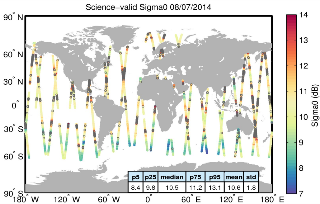
Figure 27. Geographical distribution of science-valid sigma0 data over oceans and lakes for 08/07/2014. The statistical values shown in the table refer to the sigma0 in dB and are calculated over all measurements shown in the figure. Gray circles denote records that have been rejected based on the editing criteria described in Table 4.
