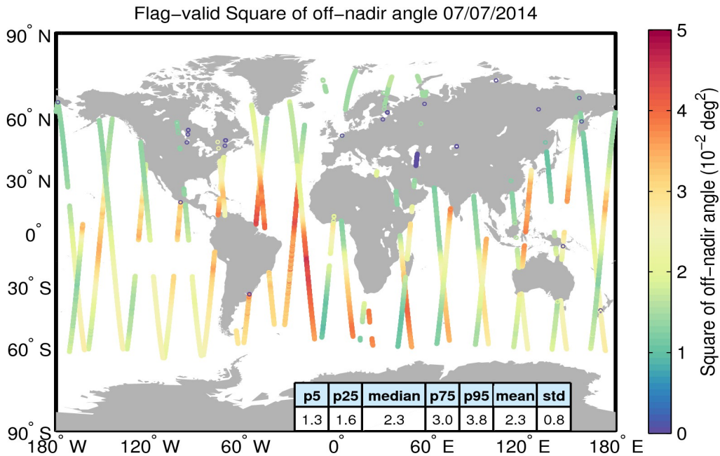
Figure 37. Geographical distribution of flag-valid mispointing data over oceans and lakes for 07/07/2014. The statistical values shown in the table refer to the mispointing in 10^{-2} \text{ deg}^2 and are calculated over all measurements shown in the figure.
