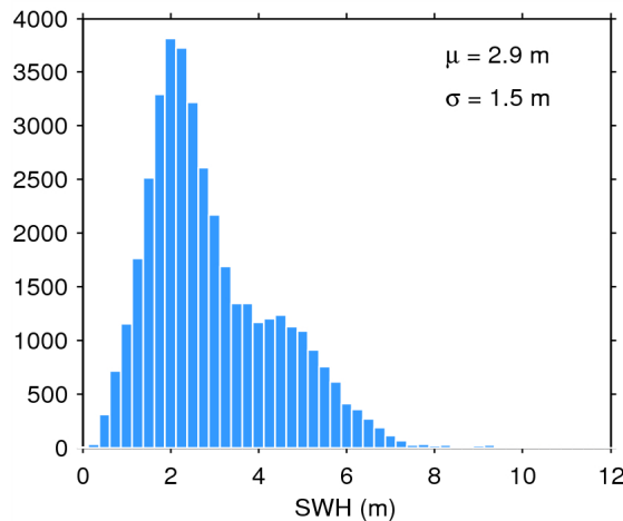
Figure 20. Histogram of science-valid SWH over oceans and lakes for 07/07/2014. The mean ( \mu ) and standard deviation ( \sigma ) are also shown. Note that values larger than 12 m are excluded from the histogram for the sake of readability but not from the computation of \mu and \sigma .
