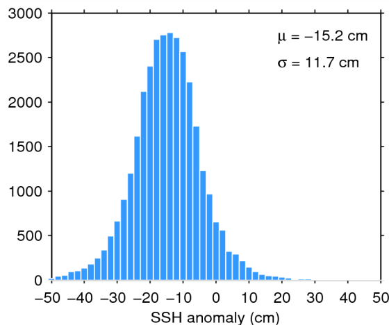
Figure 11. Histogram of science-valid SSH anomaly over oceans and lakes for 07/07/2014. The mean ( \mu ) and standard deviation ( \sigma ) are also shown. Note that values outside [-50 50] cm are excluded from the histogram for the sake of readability but not from the computation of \mu and \sigma .
