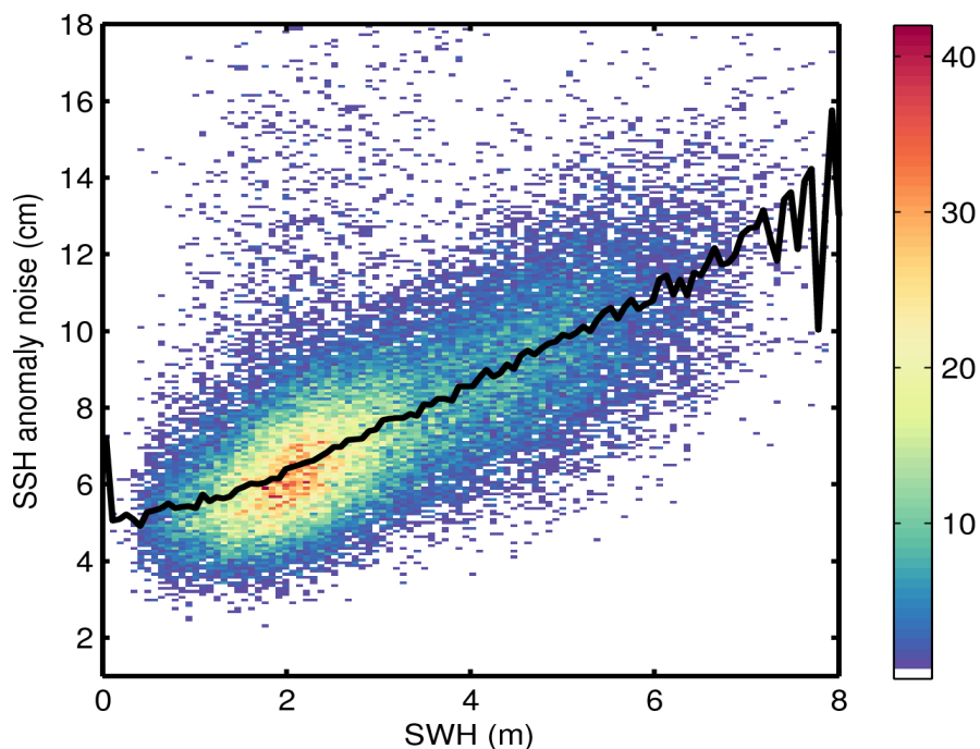
Figure 9. 2D histogram showing flag-valid SSH anomaly noise as a function of SWH for 07/07/2014. The black line denotes the median SSH anomaly as a function of SWH.
