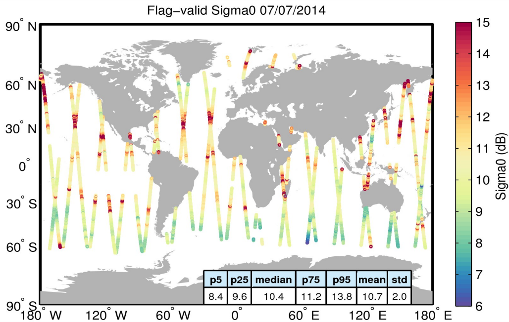
Figure 23. Geographical distribution of flag-valid sigma0 data over oceans and lakes for 07/07/2014. The statistical values shown in the table refer to the sigma0 in dB and are calculated over all measurements shown in the figure.
