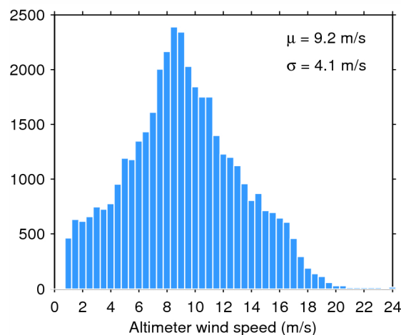
Figure 35. Histogram of science-valid wind over oceans and lakes for 07/07/2014. The mean ( \mu ) and standard deviation ( \sigma ) are also shown. Note that values larger than 24 m/s are excluded from the histogram for the sake of readability but not from the computation of \mu and \sigma .
