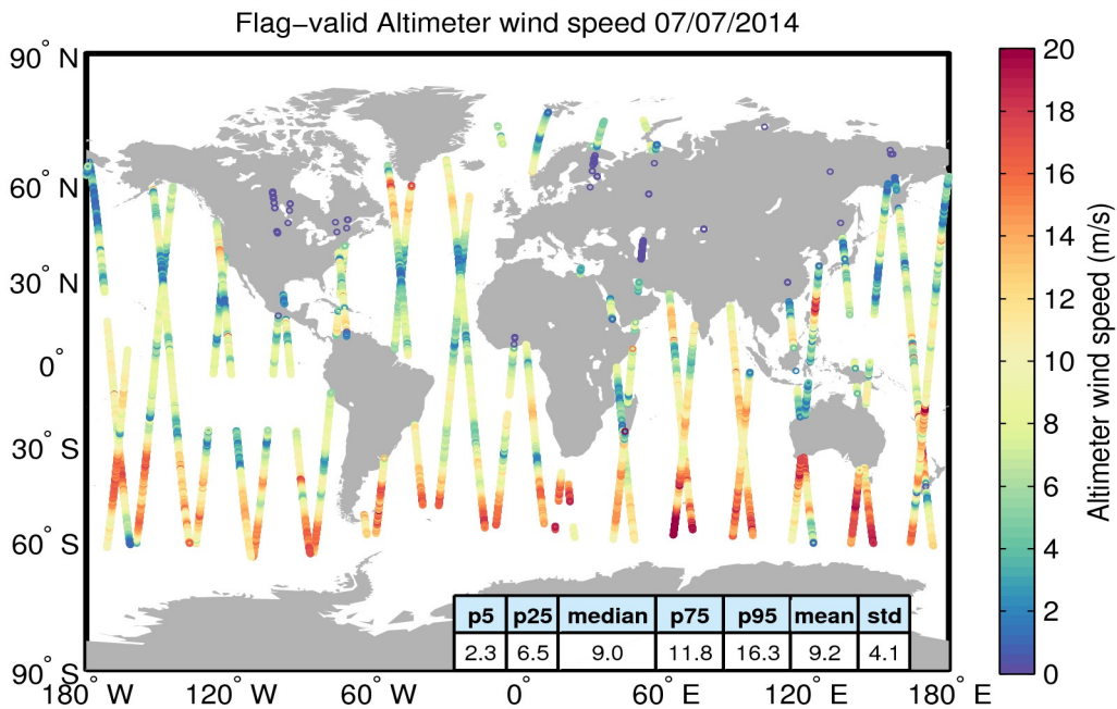
Figure 31. Geographical distribution of flag-valid wind data over oceans and lakes for 07/07/2014. The statistical values shown in the table refer to the wind in m/s and are calculated over all measurements shown in the figure.
