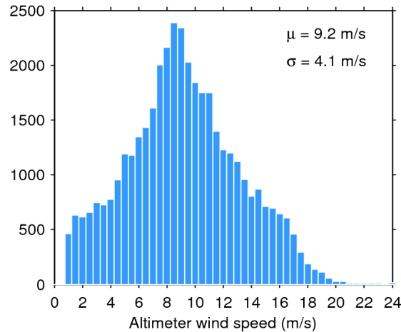
Figure 33. Histogram of flag-valid wind over oceans and lakes for 07/07/2014. The mean ( \mu ) and standard deviation ( \sigma ) are also shown. Note that values larger than 24 m/s are excluded from the histogram for the sake of readability but not from the computation of \mu and \sigma .
