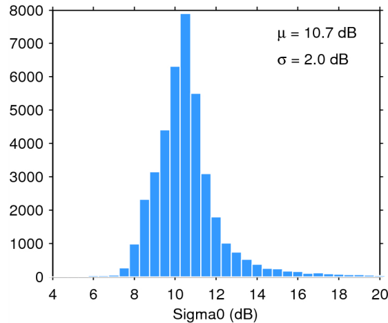
Figure 25. Histogram of flag-valid sigma0 over oceans and lakes for 07/07/2014. The mean ( \mu ) and standard deviation ( \sigma ) are also shown. Note that values outside [4 20] dB are excluded from the histogram for the sake of readability but not from the computation of \mu and \sigma .
