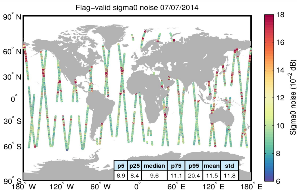
Figure 26. Geographical distribution of flag-valid 20-Hz sigma0 measurement noise over oceans and lakes for 07/07/2014. The statistical values shown in the table refer to the sigma0 noise and are calculated over all measurements shown in the figure.
