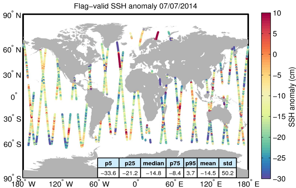
Figure 5. Geographical distribution of flag-valid 1-Hz SSH anomaly data over oceans and lakes for 07/07/2014. The statistical values shown in the table refer to the SSH anomaly in cm and are calculated over all measurements shown in the figure.
