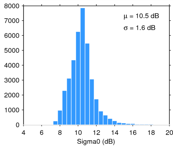
Figure 28. Histogram of science-valid sigma0 over oceans and lakes for 07/07/2014. The mean ( \mu ) and standard deviation ( \sigma ) are also shown. Note that values outside [4 20] dB are excluded from the histogram for the sake of readability but not from the computation of \mu and \sigma .
