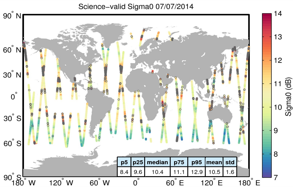
Figure 27. Geographical distribution of science-valid sigma0 data over oceans and lakes for 07/07/2014. The statistical values shown in the table refer to the sigma0 in dB and are calculated over all measurements shown in the figure. Gray circles denote records that have been rejected based on the editing criteria described in Table 4.
