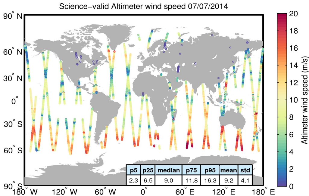
Figure 34. Geographical distribution of science-valid wind data over oceans and lakes for 07/07/2014. The statistical values shown in the table refer to the wind in m/s and are calculated over all measurements shown in the figure. Gray circles denote records that have been rejected based on the editing criteria described in Table 5.
