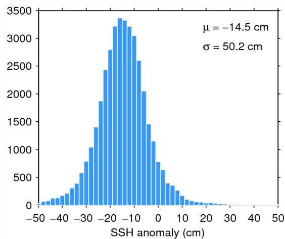
Figure 7. Histogram of flag-valid SSH anomaly over oceans and lakes for 07/07/2014. The mean ( \mu ) and standard deviation ( \sigma ) are also shown. Note that values outside [-50 50] cm are excluded from the histogram for the sake of readability but not from the computation of \mu and \sigma .
