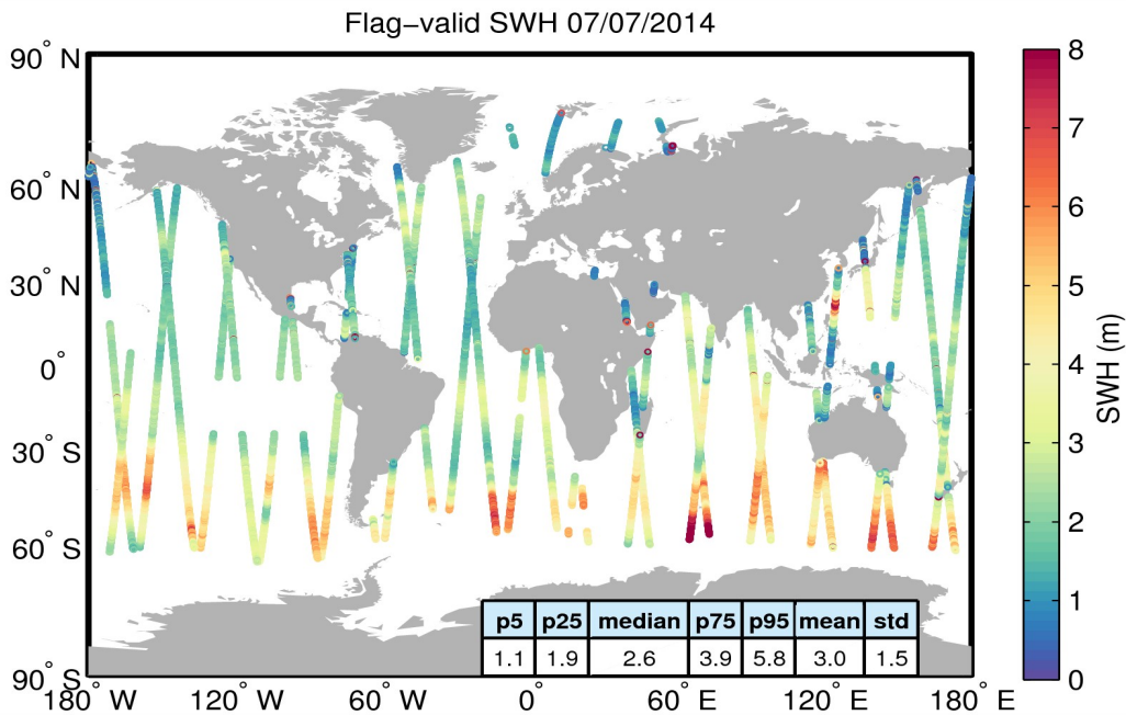
Figure 15. Geographical distribution of flag-valid SWH data over oceans and lakes for 07/07/2014. The statistical values shown in the table refer to the SWH in m and are calculated over all measurements shown in the figure.
