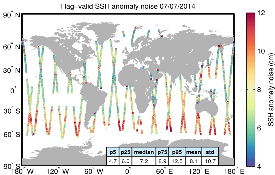
Figure 8. Geographical distribution of flag-valid 20-Hz SSH anomaly measurement noise over oceans and lakes for 07/07/2014. The statistical values shown in the table refer to the SSH anomaly noise and are calculated over all measurements shown in the figure.
