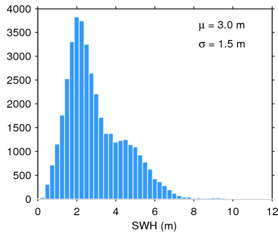
Figure 17. Histogram of flag-valid SWH over oceans and lakes for 07/07/2014. The mean ( \mu ) and standard deviation ( \sigma ) are also shown. Note that values larger than 12 m are excluded from the histogram for the sake of readability but not from the computation of \mu and \sigma .
