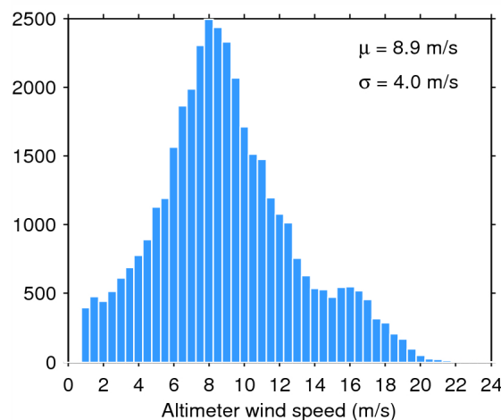
Figure 35. Histogram of science-valid wind over oceans and lakes for 02/07/2014. The mean ( \mu ) and standard deviation ( \sigma ) are also shown. Note that values larger than 24 m/s are excluded from the histogram for the sake of readability but not from the computation of \mu and \sigma .
