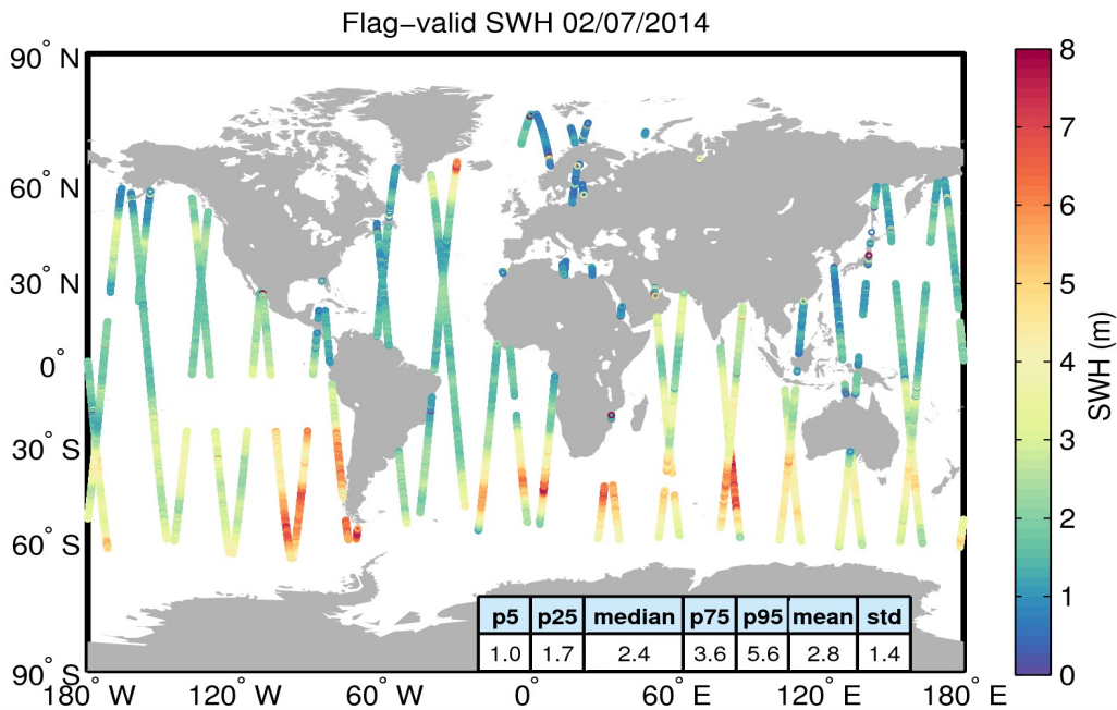
Figure 15. Geographical distribution of flag-valid SWH data over oceans and lakes for 02/07/2014. The statistical values shown in the table refer to the SWH in m and are calculated over all measurements shown in the figure.
