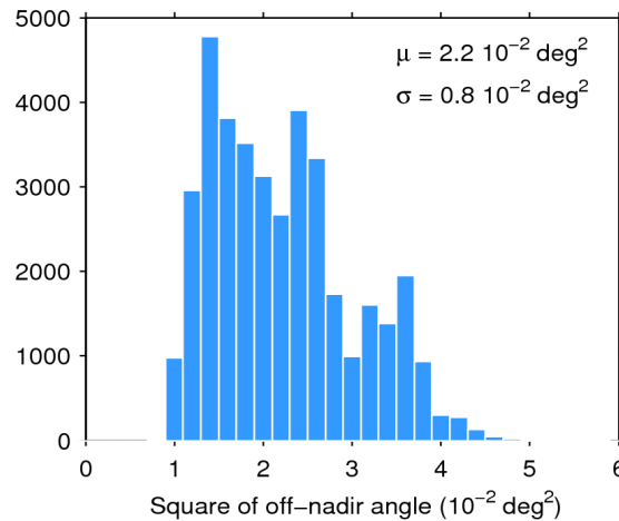
Figure 39. Histogram of flag-valid mispointing over oceans and lakes for 02/07/2014. The mean ( \mu ) and standard deviation ( \sigma ) are also shown. Note that values than 6 \cdot 10^{-2} \text{ deg}^2 are excluded from the histogram for the sake of readability but not from the computation of \mu and \sigma .
