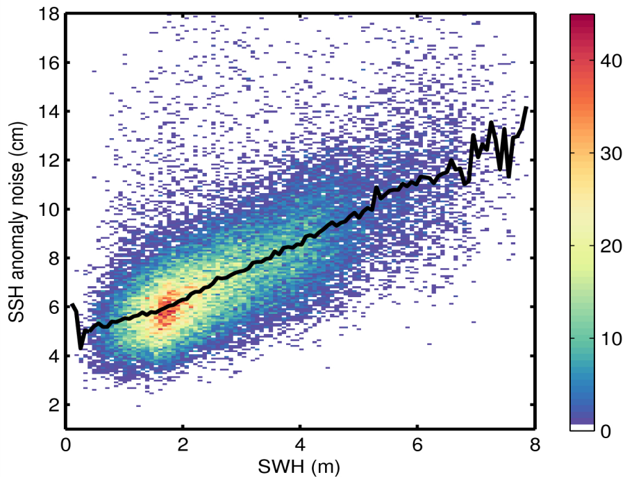
Figure 9. 2D histogram showing flag-valid SSH anomaly noise as a function of SWH for 02/07/2014. The black line denotes the median SSH anomaly as a function of SWH.
