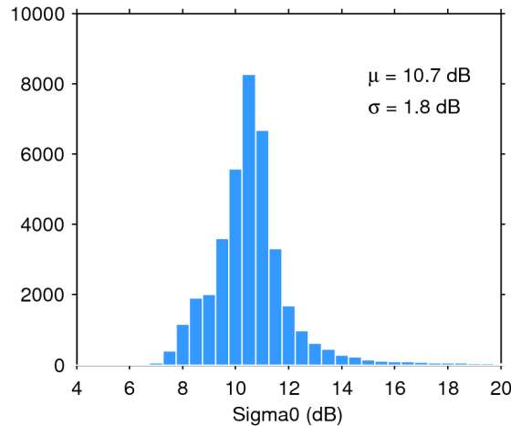
Figure 25. Histogram of flag-valid sigma0 over oceans and lakes for 02/07/2014. The mean ( \mu ) and standard deviation ( \sigma ) are also shown. Note that values outside [4 20] dB are excluded from the histogram for the sake of readability but not from the computation of \mu and \sigma .
