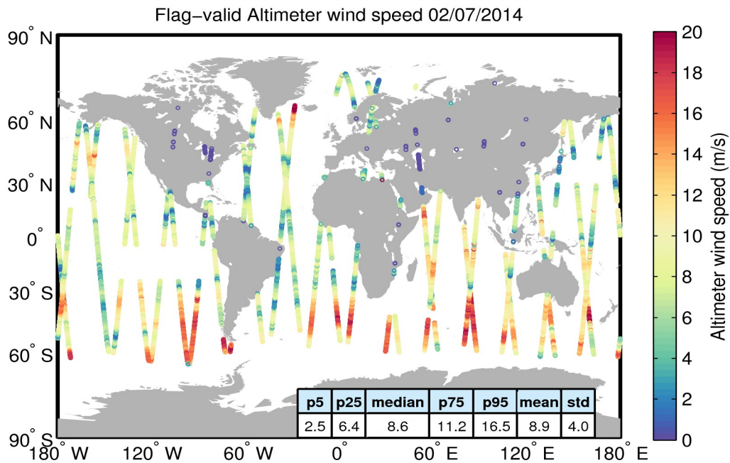
Figure 31. Geographical distribution of flag-valid wind data over oceans and lakes for 02/07/2014. The statistical values shown in the table refer to the wind in m/s and are calculated over all measurements shown in the figure.
