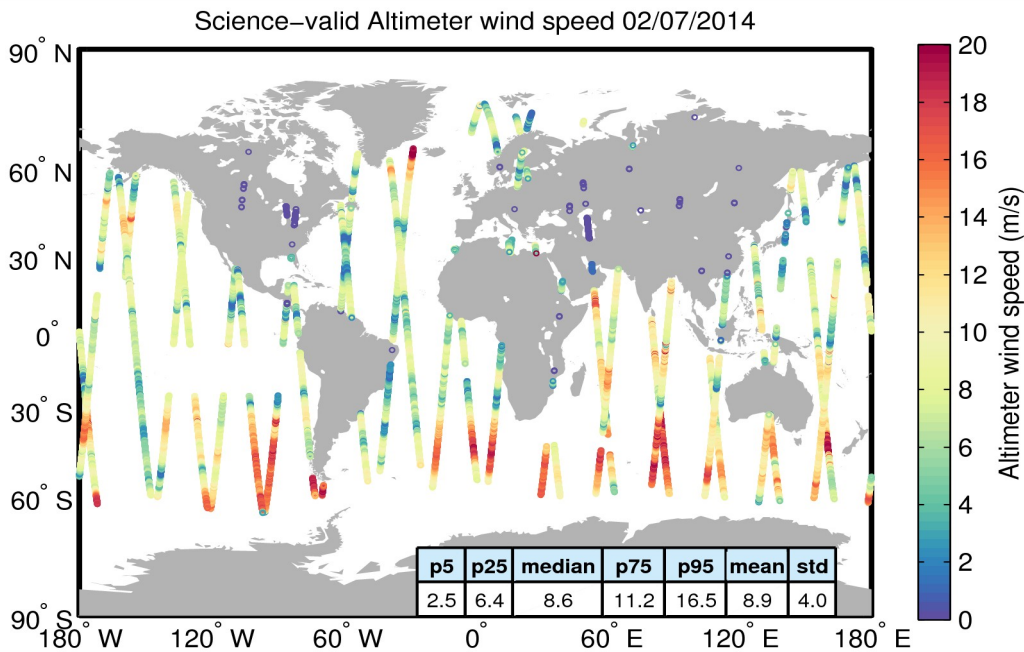
Figure 34. Geographical distribution of science-valid wind data over oceans and lakes for 02/07/2014. The statistical values shown in the table refer to the wind in m/s and are calculated over all measurements shown in the figure. Gray circles denote records that have been rejected based on the editing criteria described in Table 5.
