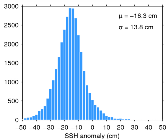
Figure 11. Histogram of science-valid SSH anomaly over oceans and lakes for 02/07/2014. The mean ( \mu ) and standard deviation ( \sigma ) are also shown. Note that values outside [-50 50] cm are excluded from the histogram for the sake of readability but not from the computation of \mu and \sigma .
