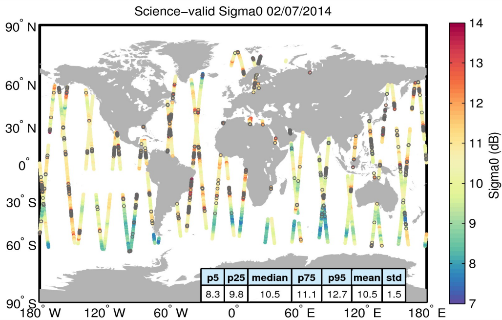
Figure 27. Geographical distribution of science-valid sigma0 data over oceans and lakes for 02/07/2014. The statistical values shown in the table refer to the sigma0 in dB and are calculated over all measurements shown in the figure. Gray circles denote records that have been rejected based on the editing criteria described in Table 4.
