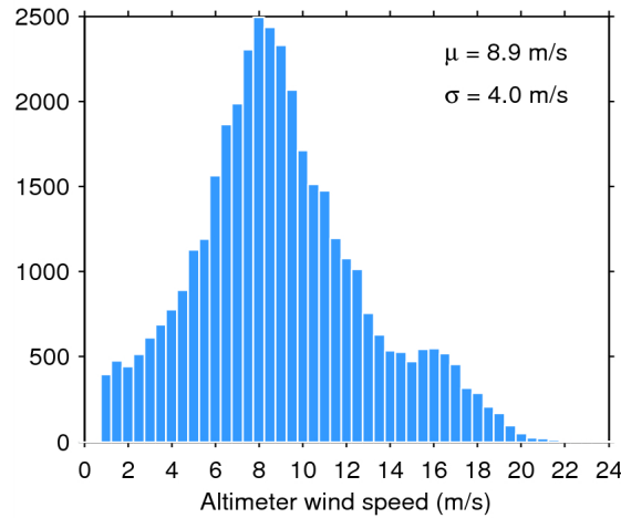
Figure 33. Histogram of flag-valid wind over oceans and lakes for 02/07/2014. The mean ( \mu ) and standard deviation ( \sigma ) are also shown. Note that values larger than 24 m/s are excluded from the histogram for the sake of readability but not from the computation of \mu and \sigma .
