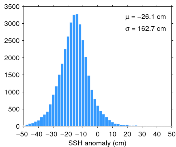
Figure 7. Histogram of flag-valid SSH anomaly over oceans and lakes for 02/07/2014. The mean ( \mu ) and standard deviation ( \sigma ) are also shown. Note that values outside [-50 50] cm are excluded from the histogram for the sake of readability but not from the computation of \mu and \sigma .
