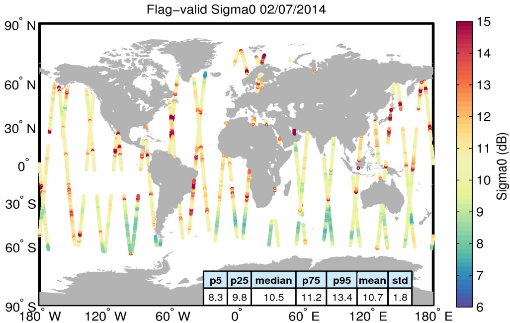
Figure 23. Geographical distribution of flag-valid sigma0 data over oceans and lakes for 02/07/2014. The statistical values shown in the table refer to the sigma0 in dB and are calculated over all measurements shown in the figure.
