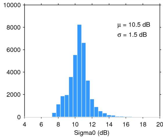
Figure 28. Histogram of science-valid sigma0 over oceans and lakes for 02/07/2014. The mean ( \mu ) and standard deviation ( \sigma ) are also shown. Note that values outside [4 20] dB are excluded from the histogram for the sake of readability but not from the computation of \mu and \sigma .
