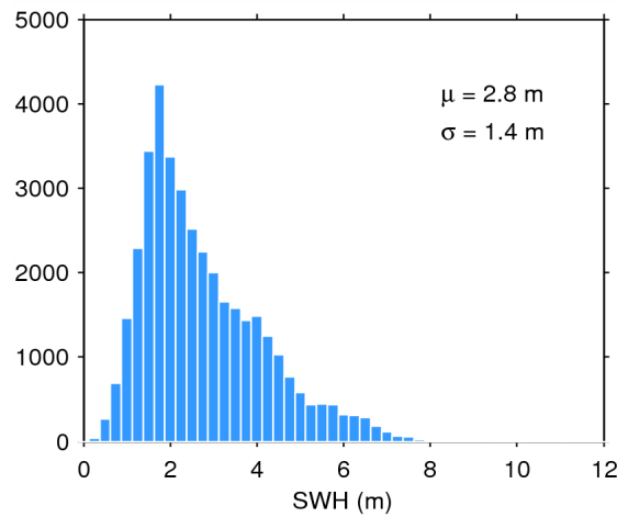
Figure 17. Histogram of flag-valid SWH over oceans and lakes for 02/07/2014. The mean ( \mu ) and standard deviation ( \sigma ) are also shown. Note that values larger than 12 m are excluded from the histogram for the sake of readability but not from the computation of \mu and \sigma .
