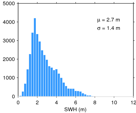
Figure 20. Histogram of science-valid SWH over oceans and lakes for 02/07/2014. The mean ( \mu ) and standard deviation ( \sigma ) are also shown. Note that values larger than 12 m are excluded from the histogram for the sake of readability but not from the computation of \mu and \sigma .
