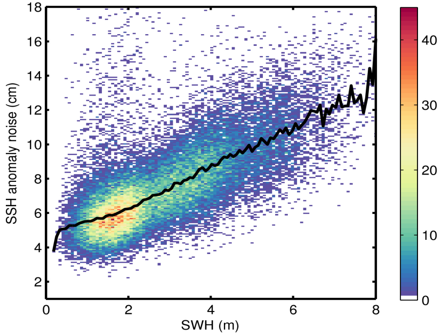
Figure 9. 2D histogram showing flag-valid SSH anomaly noise as a function of SWH for 26/06/2014. The black line denotes the median SSH anomaly as a function of SWH.
