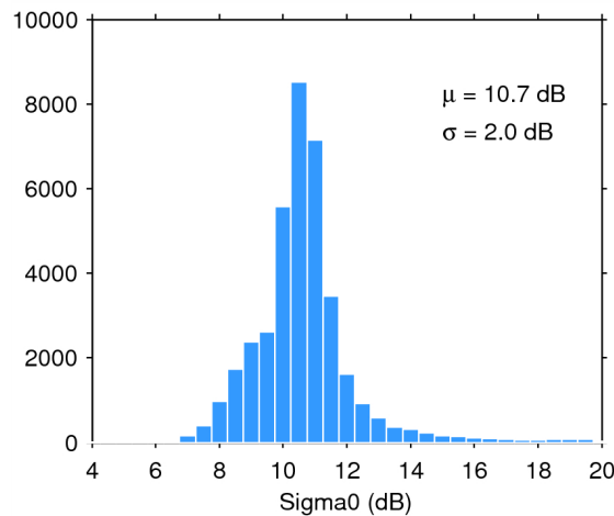
Figure 25. Histogram of flag-valid sigma0 over oceans and lakes for 26/06/2014. The mean ( \mu ) and standard deviation ( \sigma ) are also shown. Note that values outside [4 20] dB are excluded from the histogram for the sake of readability but not from the computation of \mu and \sigma .
