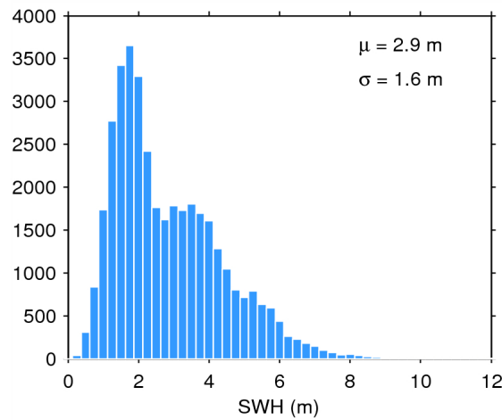
Figure 17. Histogram of flag-valid SWH over oceans and lakes for 26/06/2014. The mean ( \mu ) and standard deviation ( \sigma ) are also shown. Note that values larger than 12 m are excluded from the histogram for the sake of readability but not from the computation of \mu and \sigma .
