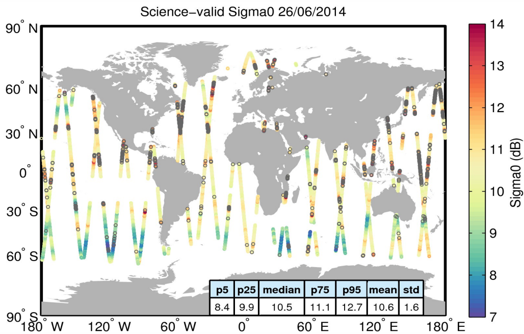
Figure 27. Geographical distribution of science-valid sigma0 data over oceans and lakes for 26/06/2014. The statistical values shown in the table refer to the sigma0 in dB and are calculated over all measurements shown in the figure. Gray circles denote records that have been rejected based on the editing criteria described in Table 4.
