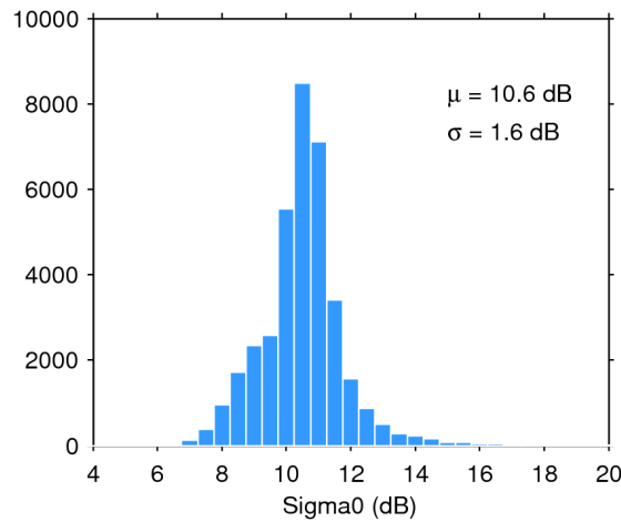
Figure 28. Histogram of science-valid sigma0 over oceans and lakes for 26/06/2014. The mean ( \mu ) and standard deviation ( \sigma ) are also shown. Note that values outside [4 20] dB are excluded from the histogram for the sake of readability but not from the computation of \mu and \sigma .
