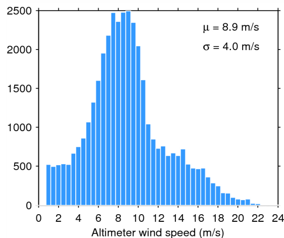
Figure 35. Histogram of science-valid wind over oceans and lakes for 26/06/2014. The mean ( \mu ) and standard deviation ( \sigma ) are also shown. Note that values larger than 24 m/s are excluded from the histogram for the sake of readability but not from the computation of \mu and \sigma .
