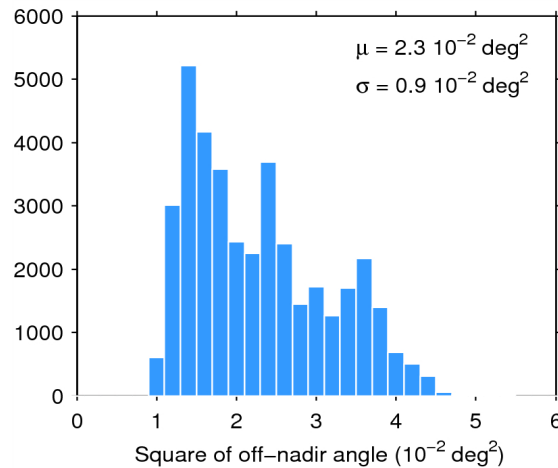
Figure 39. Histogram of flag-valid mispointing over oceans and lakes for 26/06/2014. The mean ( \mu ) and standard deviation ( \sigma ) are also shown. Note that values than 6 \cdot 10^{-2} \text{ deg}^2 are excluded from the histogram for the sake of readability but not from the computation of \mu and \sigma .
