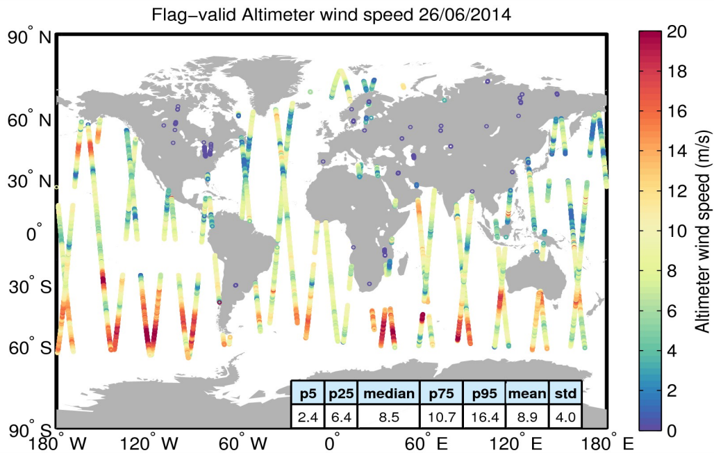
Figure 31. Geographical distribution of flag-valid wind data over oceans and lakes for 26/06/2014. The statistical values shown in the table refer to the wind in m/s and are calculated over all measurements shown in the figure.
