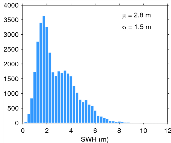
Figure 20. Histogram of science-valid SWH over oceans and lakes for 26/06/2014. The mean ( \mu ) and standard deviation ( \sigma ) are also shown. Note that values larger than 12 m are excluded from the histogram for the sake of readability but not from the computation of \mu and \sigma .
