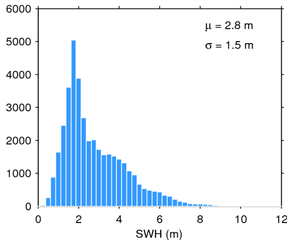
Figure 20. Histogram of science-valid SWH over oceans and lakes for 25/06/2014. The mean ( \mu ) and standard deviation ( \sigma ) are also shown. Note that values larger than 12 m are excluded from the histogram for the sake of readability but not from the computation of \mu and \sigma .
