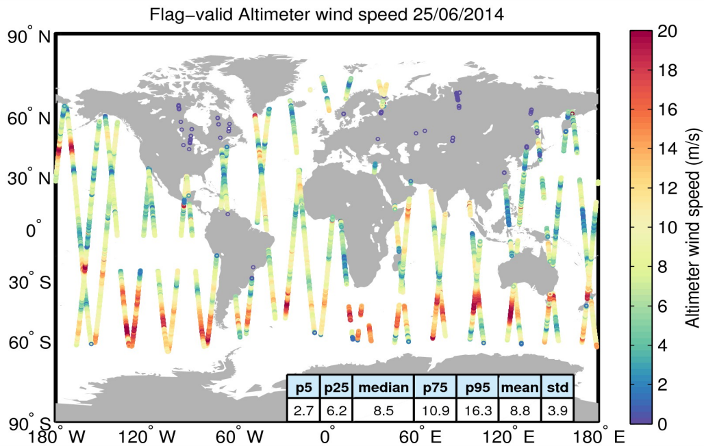
Figure 31. Geographical distribution of flag-valid wind data over oceans and lakes for 25/06/2014. The statistical values shown in the table refer to the wind in m/s and are calculated over all measurements shown in the figure.
