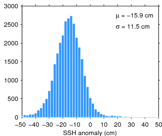
Figure 11. Histogram of science-valid SSH anomaly over oceans and lakes for 25/06/2014. The mean ( \mu ) and standard deviation ( \sigma ) are also shown. Note that values outside [-50 50] cm are excluded from the histogram for the sake of readability but not from the computation of \mu and \sigma .
