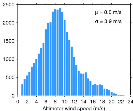
Figure 35. Histogram of science-valid wind over oceans and lakes for 25/06/2014. The mean ( \mu ) and standard deviation ( \sigma ) are also shown. Note that values larger than 24 m/s are excluded from the histogram for the sake of readability but not from the computation of \mu and \sigma .
