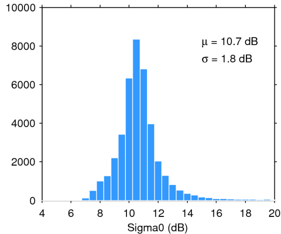
Figure 25. Histogram of flag-valid sigma0 over oceans and lakes for 25/06/2014. The mean ( \mu ) and standard deviation ( \sigma ) are also shown. Note that values outside [4 20] dB are excluded from the histogram for the sake of readability but not from the computation of \mu and \sigma .
