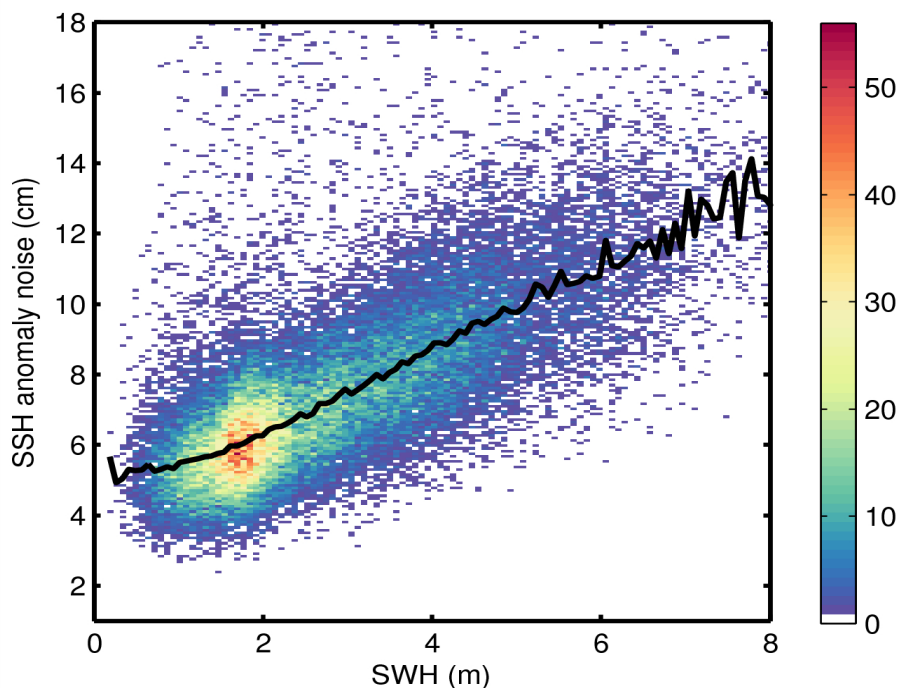
Figure 9. 2D histogram showing flag-valid SSH anomaly noise as a function of SWH for 25/06/2014. The black line denotes the median SSH anomaly as a function of SWH.
