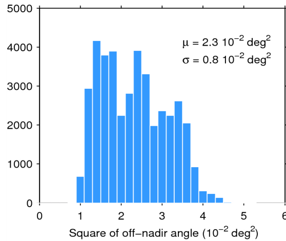
Figure 39. Histogram of flag-valid mispointing over oceans and lakes for 25/06/2014. The mean ( \mu ) and standard deviation ( \sigma ) are also shown. Note that values than 6 \cdot 10^{-2} \text{ deg}^2 are excluded from the histogram for the sake of readability but not from the computation of \mu and \sigma .
