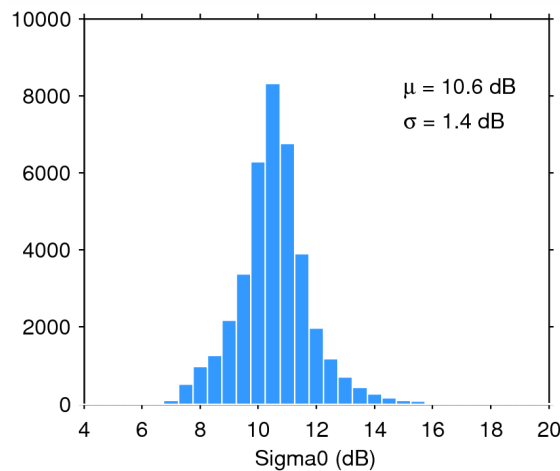
Figure 28. Histogram of science-valid sigma0 over oceans and lakes for 25/06/2014. The mean ( \mu ) and standard deviation ( \sigma ) are also shown. Note that values outside [4 20] dB are excluded from the histogram for the sake of readability but not from the computation of \mu and \sigma .
