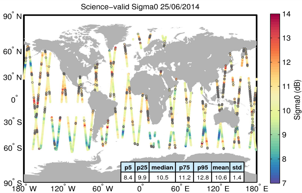
Figure 27. Geographical distribution of science-valid sigma0 data over oceans and lakes for 25/06/2014. The statistical values shown in the table refer to the sigma0 in dB and are calculated over all measurements shown in the figure. Gray circles denote records that have been rejected based on the editing criteria described in Table 4.
