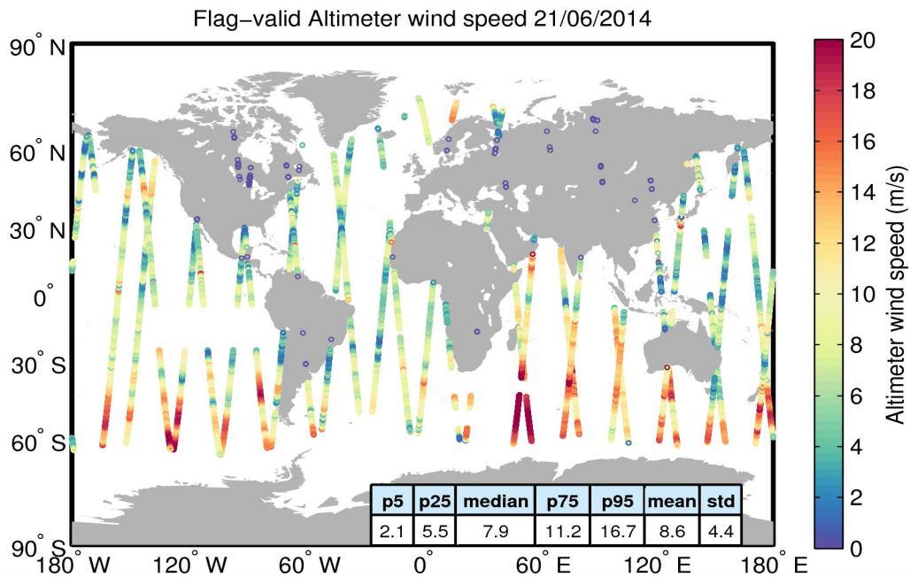
Figure 31. Geographical distribution of flag-valid wind data over oceans and lakes for 21/06/2014. The statistical values shown in the table refer to the wind in m/s and are calculated over all measurements shown in the figure.
