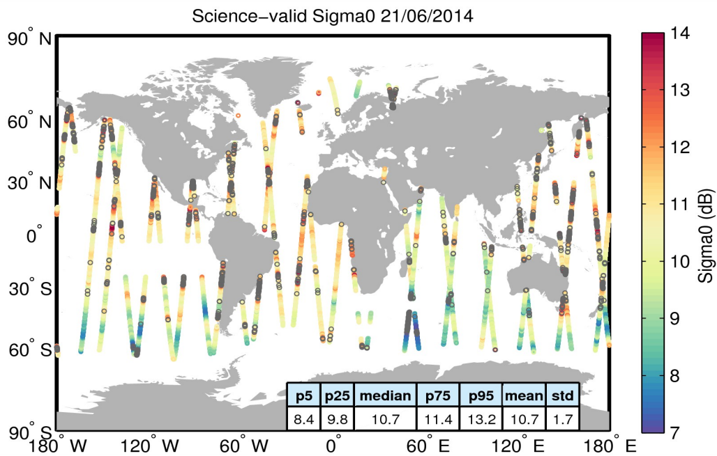
Figure 27. Geographical distribution of science-valid sigma0 data over oceans and lakes for 21/06/2014. The statistical values shown in the table refer to the sigma0 in dB and are calculated over all measurements shown in the figure. Gray circles denote records that have been rejected based on the editing criteria described in Table 4.
