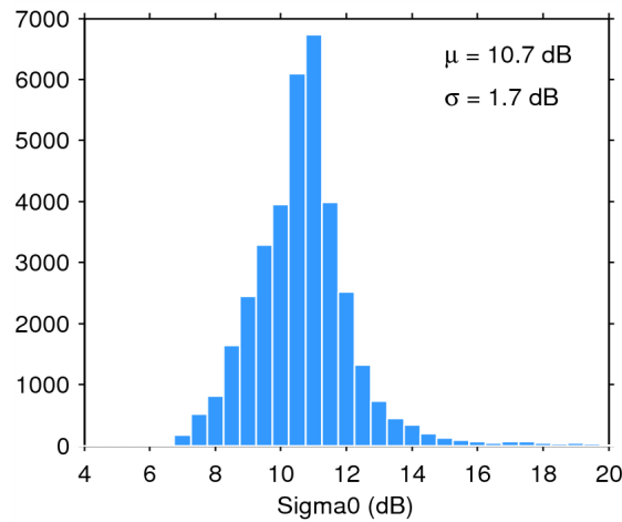
Figure 28. Histogram of science-valid sigma0 over oceans and lakes for 21/06/2014. The mean ( \mu ) and standard deviation ( \sigma ) are also shown. Note that values outside [4 20] dB are excluded from the histogram for the sake of readability but not from the computation of \mu and \sigma .
