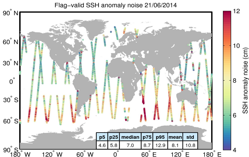
Figure 8. Geographical distribution of flag-valid 20-Hz SSH anomaly measurement noise over oceans and lakes for 21/06/2014. The statistical values shown in the table refer to the SSH anomaly noise and are calculated over all measurements shown in the figure.
