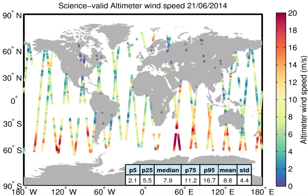
Figure 34. Geographical distribution of science-valid wind data over oceans and lakes for 21/06/2014. The statistical values shown in the table refer to the wind in m/s and are calculated over all measurements shown in the figure. Gray circles denote records that have been rejected based on the editing criteria described in Table 5.
