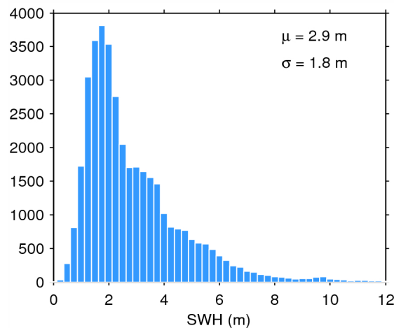
Figure 17. Histogram of flag-valid SWH over oceans and lakes for 21/06/2014. The mean ( \mu ) and standard deviation ( \sigma ) are also shown. Note that values larger than 12 m are excluded from the histogram for the sake of readability but not from the computation of \mu and \sigma .
