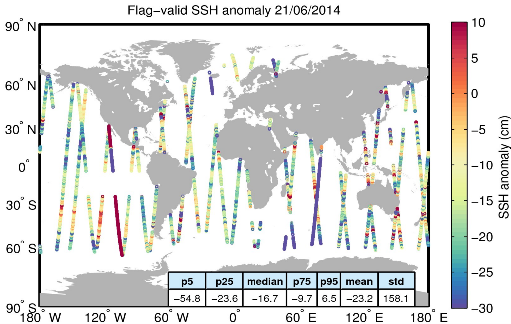
Figure 5. Geographical distribution of flag-valid 1-Hz SSH anomaly data over oceans and lakes for 21/06/2014. The statistical values shown in the table refer to the SSH anomaly in cm and are calculated over all measurements shown in the figure.
