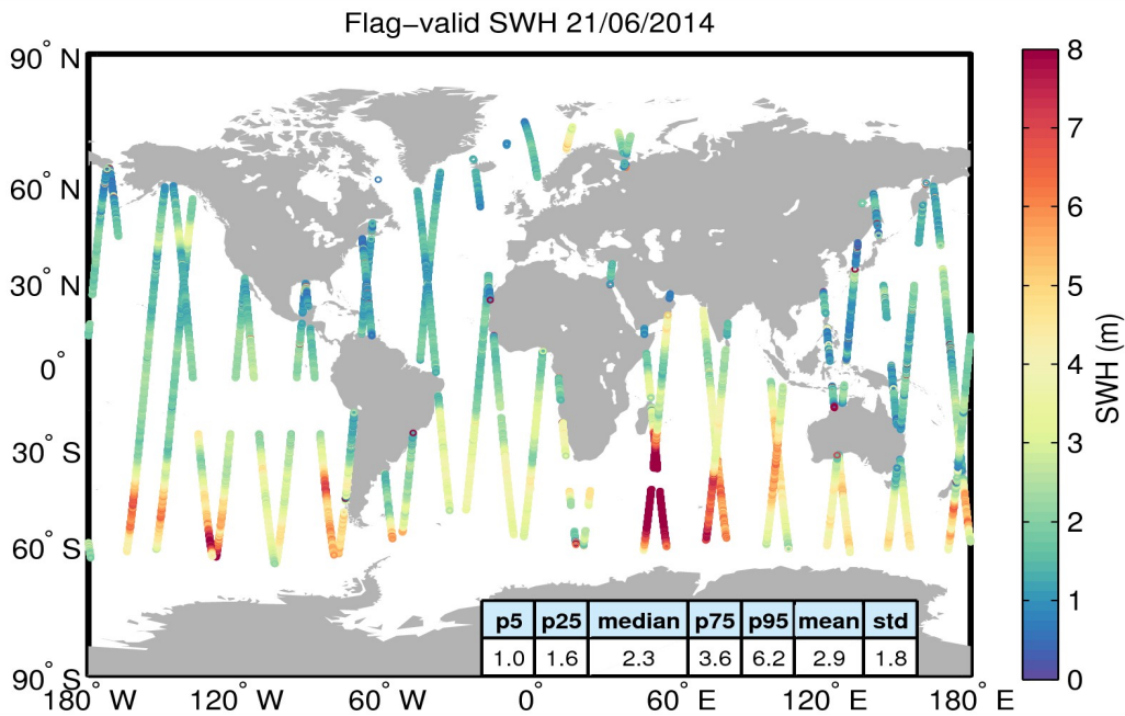
Figure 15. Geographical distribution of flag-valid SWH data over oceans and lakes for 21/06/2014. The statistical values shown in the table refer to the SWH in m and are calculated over all measurements shown in the figure.
