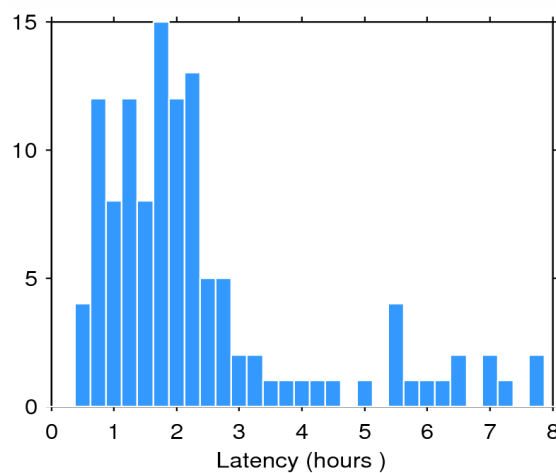
Figure 2. Histogram of the data latency for 21/06/2014. The y-axis denotes the number of files that are made available with a delay of x-hours with respect to the mean time of the records stored in the file.
