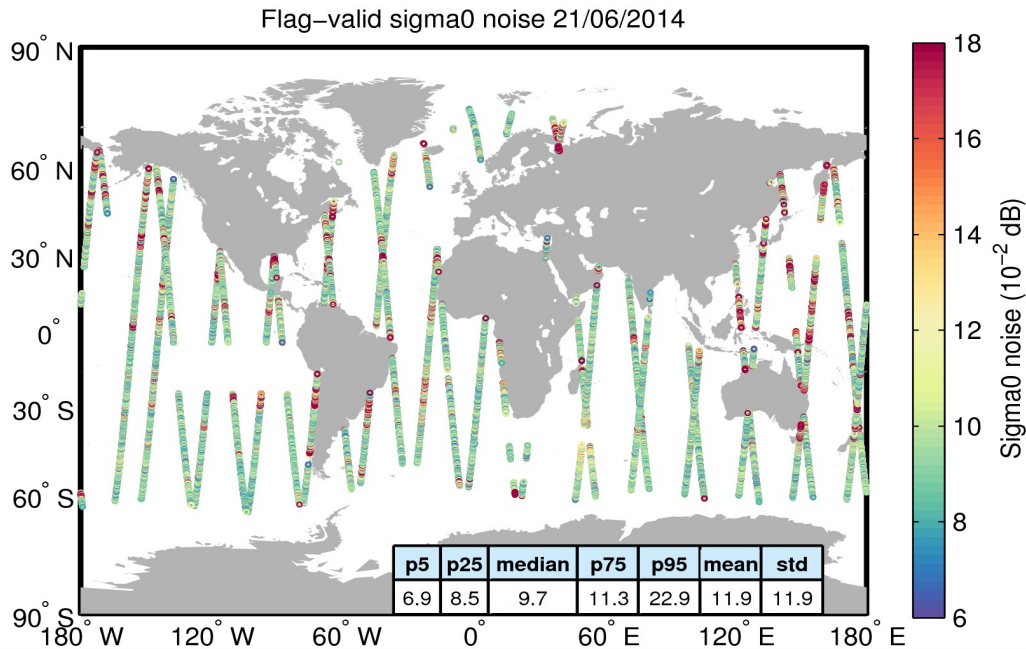
Figure 26. Geographical distribution of flag-valid 20-Hz sigma0 measurement noise over oceans and lakes for 21/06/2014. The statistical values shown in the table refer to the sigma0 noise and are calculated over all measurements shown in the figure.
