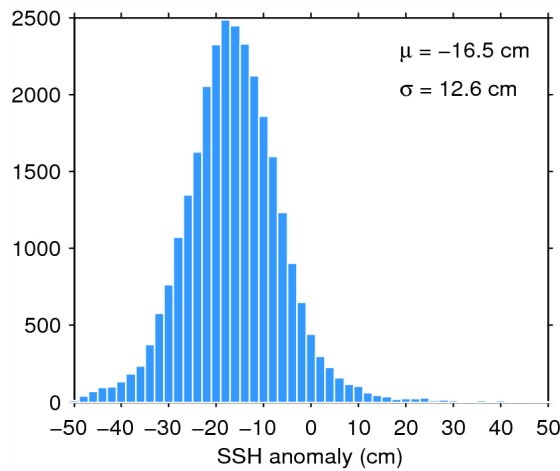
Figure 11. Histogram of science-valid SSH anomaly over oceans and lakes for 21/06/2014. The mean ( \mu ) and standard deviation ( \sigma ) are also shown. Note that values outside [-50 50] cm are excluded from the histogram for the sake of readability but not from the computation of \mu and \sigma .
