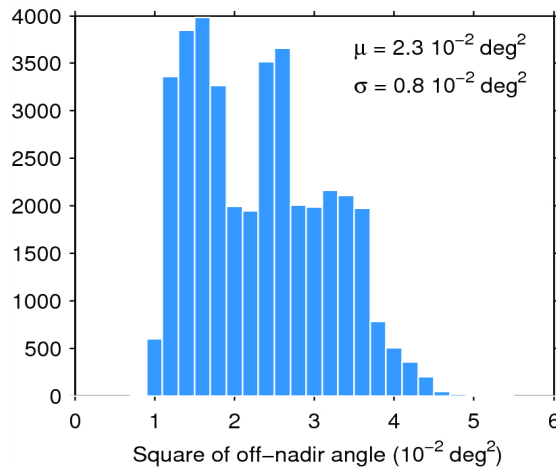
Figure 39. Histogram of flag-valid mispointing over oceans and lakes for 21/06/2014. The mean ( \mu ) and standard deviation ( \sigma ) are also shown. Note that values than 6 \cdot 10^{-2} \text{ deg}^2 are excluded from the histogram for the sake of readability but not from the computation of \mu and \sigma .
