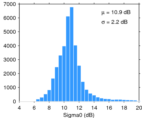
Figure 25. Histogram of flag-valid sigma0 over oceans and lakes for 21/06/2014. The mean ( \mu ) and standard deviation ( \sigma ) are also shown. Note that values outside [4 20] dB are excluded from the histogram for the sake of readability but not from the computation of \mu and \sigma .
