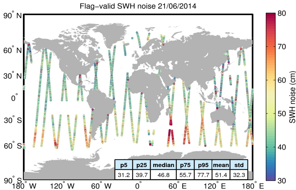
Figure 18. Geographical distribution of flag-valid 20-Hz SWH measurement noise over oceans and lakes for 21/06/2014. The statistical values shown in the figure refer to the SWH noise and are calculated over all measurements shown in the figure.
