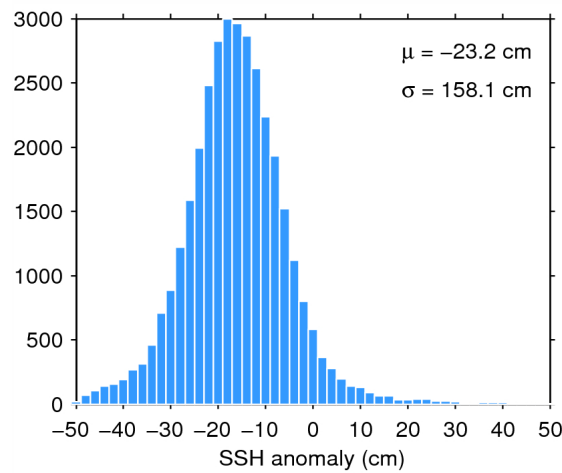
Figure 7. Histogram of flag-valid SSH anomaly over oceans and lakes for 21/06/2014. The mean ( \mu ) and standard deviation ( \sigma ) are also shown. Note that values outside [-50\ 50] cm are excluded from the histogram for the sake of readability but not from the computation of \mu and \sigma .
