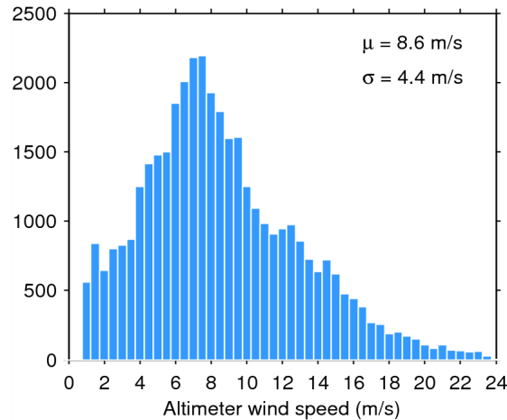
Figure 33. Histogram of flag-valid wind over oceans and lakes for 21/06/2014. The mean ( \mu ) and standard deviation ( \sigma ) are also shown. Note that values larger than 24 m/s are excluded from the histogram for the sake of readability but not from the computation of \mu and \sigma .
