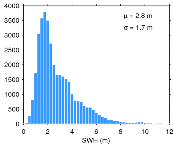
Figure 20. Histogram of science-valid SWH over oceans and lakes for 21/06/2014. The mean ( \mu ) and standard deviation ( \sigma ) are also shown. Note that values larger than 12 m are excluded from the histogram for the sake of readability but not from the computation of \mu and \sigma .
