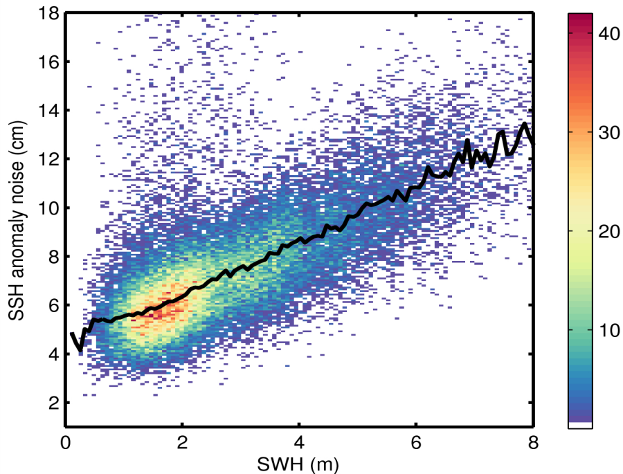
Figure 9. 2D histogram showing flag-valid SSH anomaly noise as a function of SWH for 21/06/2014. The black line denotes the median SSH anomaly as a function of SWH.
