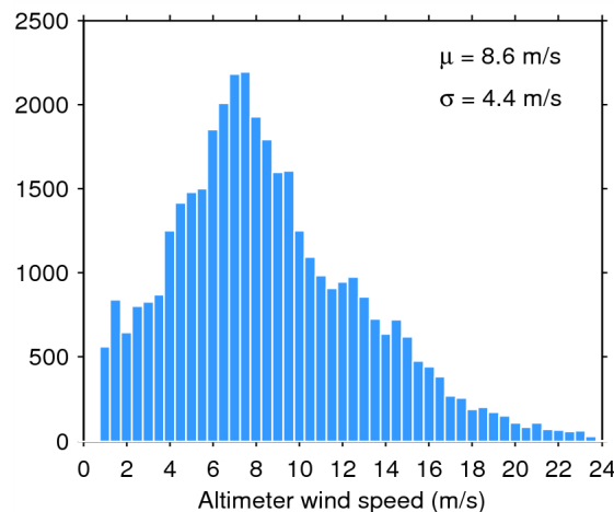
Figure 35. Histogram of science-valid wind over oceans and lakes for 21/06/2014. The mean ( \mu ) and standard deviation ( \sigma ) are also shown. Note that values larger than 24 m/s are excluded from the histogram for the sake of readability but not from the computation of \mu and \sigma .
