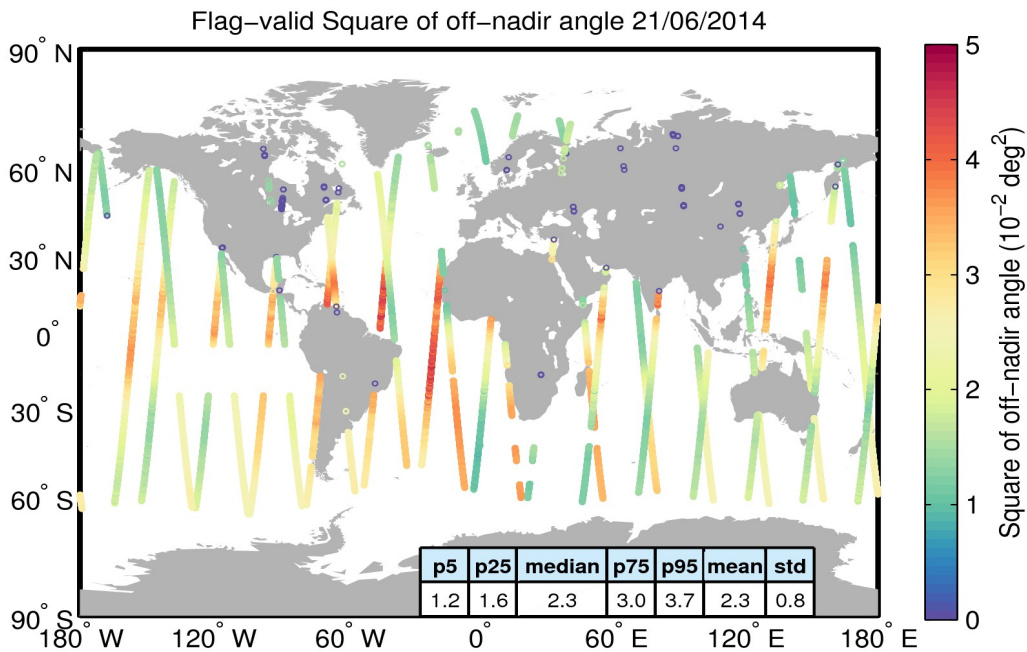
Figure 37. Geographical distribution of flag-valid mispointing data over oceans and lakes for 21/06/2014. The statistical values shown in the table refer to the mispointing in 10^{-2} \text{ deg}^2 and are calculated over all measurements shown in the figure.
