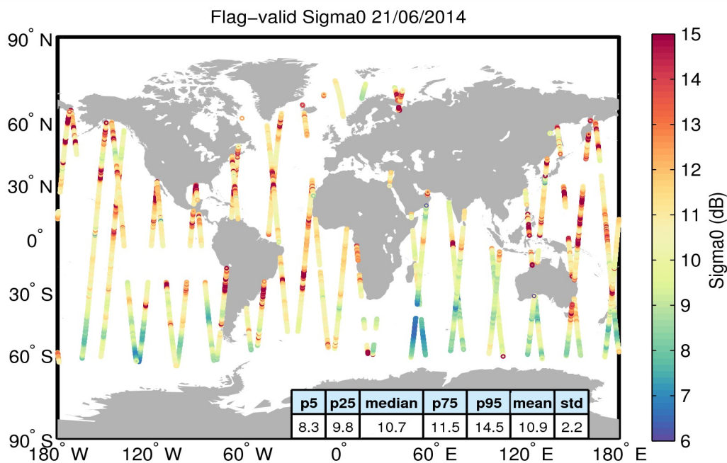
Figure 23. Geographical distribution of flag-valid sigma0 data over oceans and lakes for 21/06/2014. The statistical values shown in the table refer to the sigma0 in dB and are calculated over all measurements shown in the figure.
