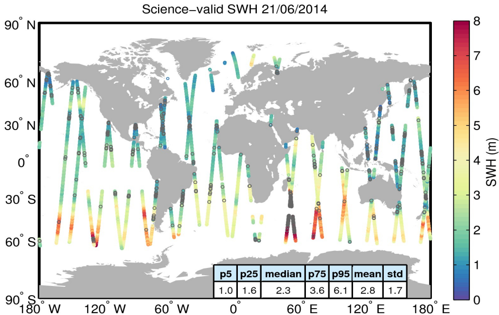
Figure 19. Geographical distribution of science-valid SWH data over oceans and lakes for 21/06/2014. The statistical values shown in the table refer to the SWH in m and are calculated over all measurements shown in the figure. Gray circles denote records that have been rejected based on the editing criteria described in Table 3.
