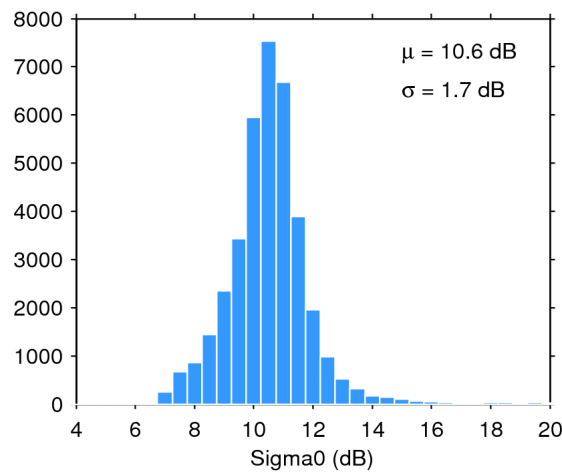
Figure 28. Histogram of science-valid sigma0 over oceans and lakes for 20/06/2014. The mean ( \mu ) and standard deviation ( \sigma ) are also shown. Note that values outside [4 20] dB are excluded from the histogram for the sake of readability but not from the computation of \mu and \sigma .
