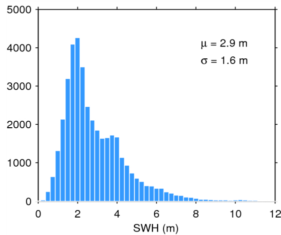
Figure 17. Histogram of flag-valid SWH over oceans and lakes for 20/06/2014. The mean ( \mu ) and standard deviation ( \sigma ) are also shown. Note that values larger than 12 m are excluded from the histogram for the sake of readability but not from the computation of \mu and \sigma .
