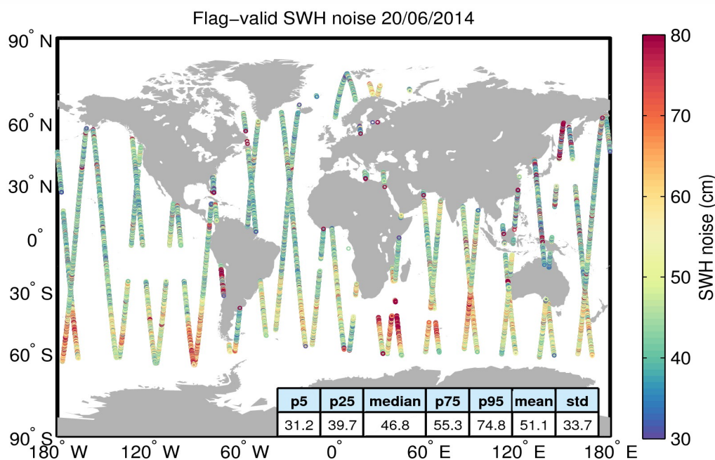
Figure 18. Geographical distribution of flag-valid 20-Hz SWH measurement noise over oceans and lakes for 20/06/2014. The statistical values shown in the figure refer to the SWH noise and are calculated over all measurements shown in the figure.
