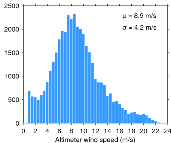
Figure 35. Histogram of science-valid wind over oceans and lakes for 20/06/2014. The mean ( \mu ) and standard deviation ( \sigma ) are also shown. Note that values larger than 24 m/s are excluded from the histogram for the sake of readability but not from the computation of \mu and \sigma .
