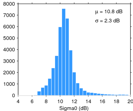
Figure 25. Histogram of flag-valid sigma0 over oceans and lakes for 20/06/2014. The mean ( \mu ) and standard deviation ( \sigma ) are also shown. Note that values outside [4 20] dB are excluded from the histogram for the sake of readability but not from the computation of \mu and \sigma .
