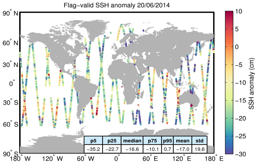
Figure 5. Geographical distribution of flag-valid 1-Hz SSH anomaly data over oceans and lakes for 20/06/2014. The statistical values shown in the table refer to the SSH anomaly in cm and are calculated over all measurements shown in the figure.
