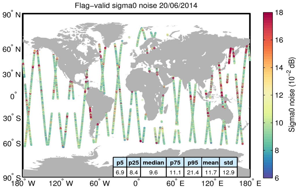
Figure 26. Geographical distribution of flag-valid 20-Hz sigma0 measurement noise over oceans and lakes for 20/06/2014. The statistical values shown in the table refer to the sigma0 noise and are calculated over all measurements shown in the figure.
