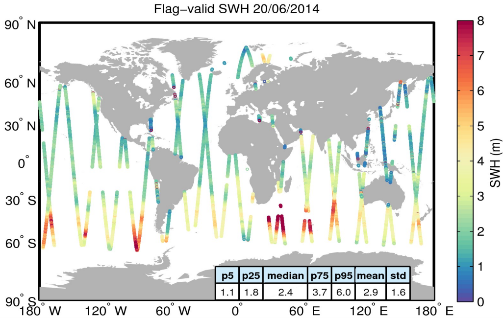
Figure 15. Geographical distribution of flag-valid SWH data over oceans and lakes for 20/06/2014. The statistical values shown in the table refer to the SWH in m and are calculated over all measurements shown in the figure.
