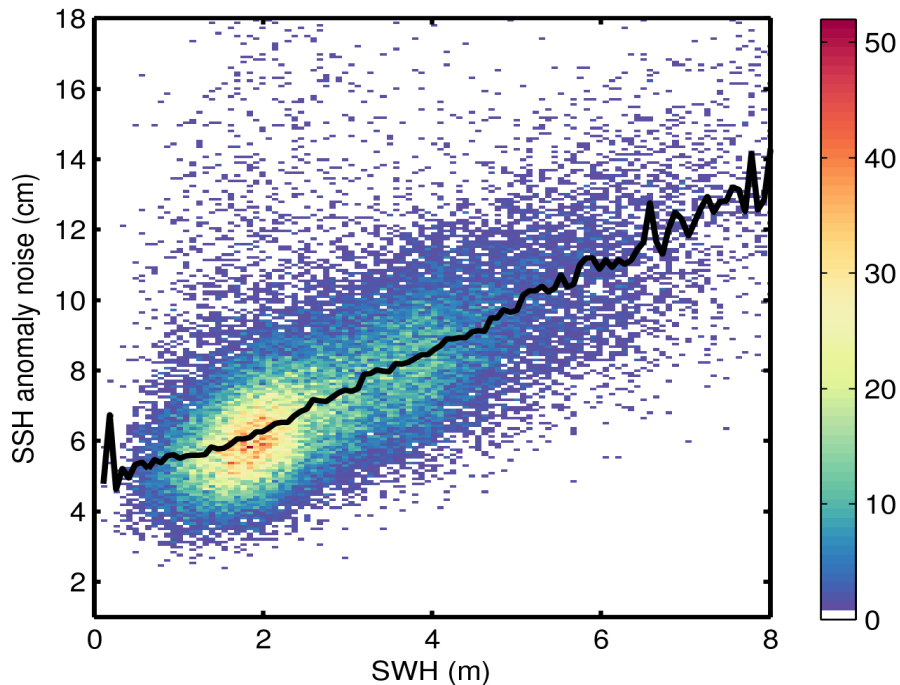
Figure 9. 2D histogram showing flag-valid SSH anomaly noise as a function of SWH for 20/06/2014. The black line denotes the median SSH anomaly as a function of SWH.
