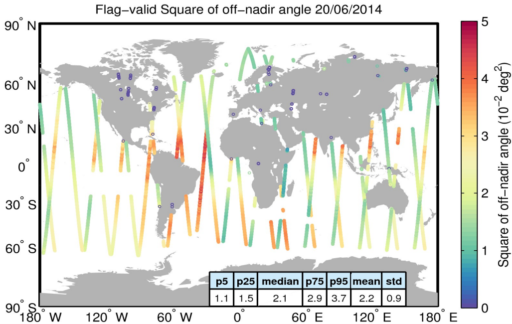
Figure 37. Geographical distribution of flag-valid mispointing data over oceans and lakes for 20/06/2014. The statistical values shown in the table refer to the mispointing in 10^{-2} \text{ deg}^2 and are calculated over all measurements shown in the figure.
