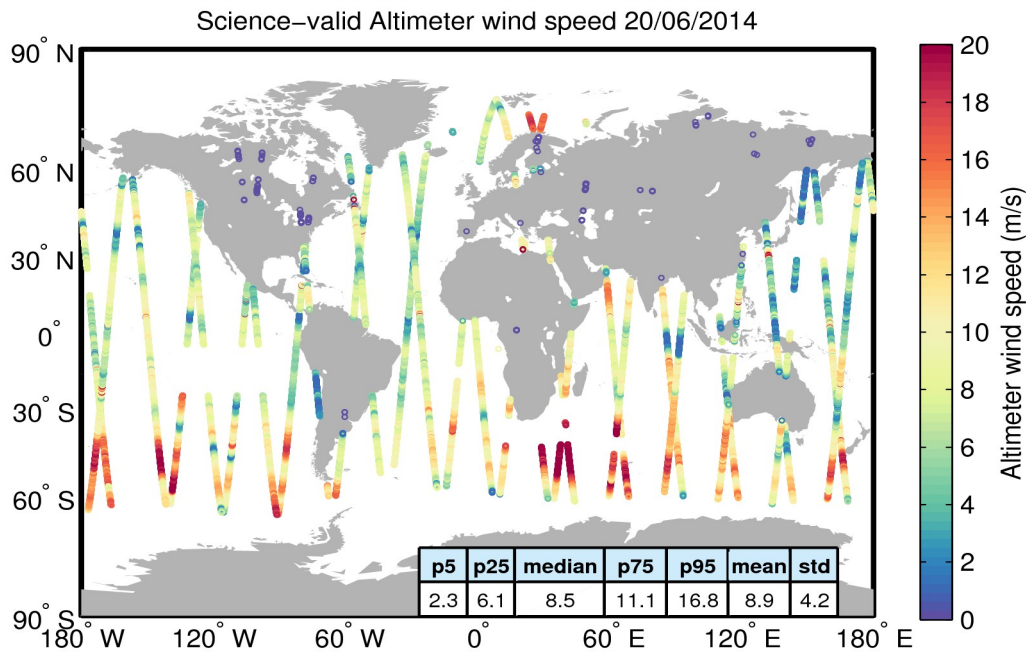
Figure 34. Geographical distribution of science-valid wind data over oceans and lakes for 20/06/2014. The statistical values shown in the table refer to the wind in m/s and are calculated over all measurements shown in the figure. Gray circles denote records that have been rejected based on the editing criteria described in Table 5.
