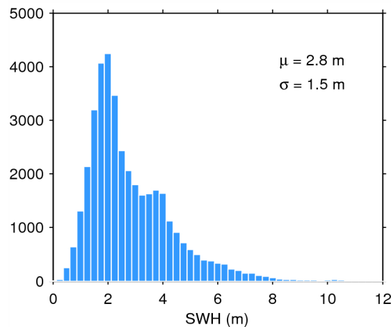
Figure 20. Histogram of science-valid SWH over oceans and lakes for 20/06/2014. The mean ( \mu ) and standard deviation ( \sigma ) are also shown. Note that values larger than 12 m are excluded from the histogram for the sake of readability but not from the computation of \mu and \sigma .
