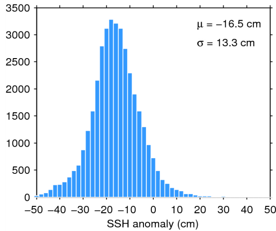
Figure 11. Histogram of science-valid SSH anomaly over oceans and lakes for 20/06/2014. The mean ( \mu ) and standard deviation ( \sigma ) are also shown. Note that values outside [-50 50] cm are excluded from the histogram for the sake of readability but not from the computation of \mu and \sigma .
