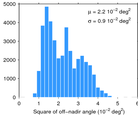
Figure 39. Histogram of flag-valid mispointing over oceans and lakes for 20/06/2014. The mean ( \mu ) and standard deviation ( \sigma ) are also shown. Note that values than 6 \cdot 10^{-2} \text{ deg}^2 are excluded from the histogram for the sake of readability but not from the computation of \mu and \sigma .
