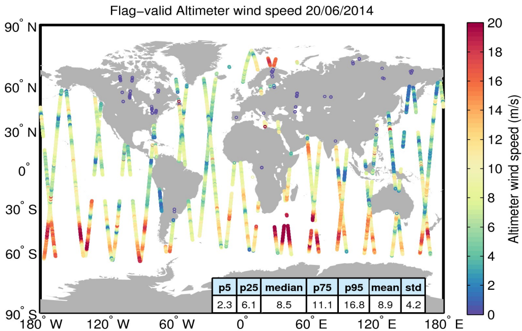
Figure 31. Geographical distribution of flag-valid wind data over oceans and lakes for 20/06/2014. The statistical values shown in the table refer to the wind in m/s and are calculated over all measurements shown in the figure.
