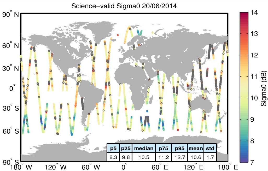
Figure 27. Geographical distribution of science-valid sigma0 data over oceans and lakes for 20/06/2014. The statistical values shown in the table refer to the sigma0 in dB and are calculated over all measurements shown in the figure. Gray circles denote records that have been rejected based on the editing criteria described in Table 4.
