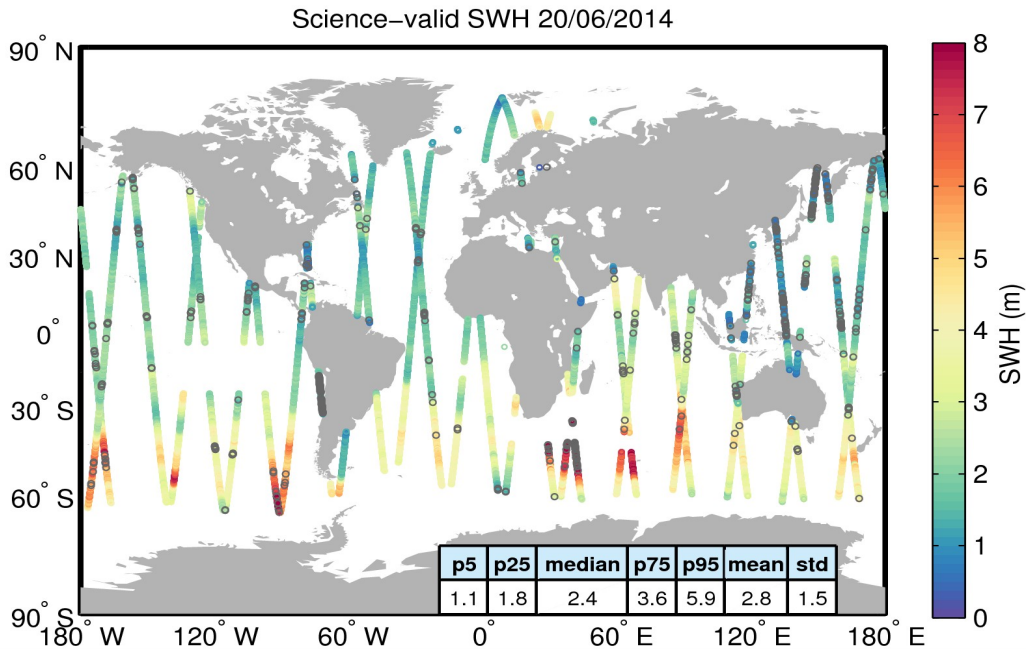
Figure 19. Geographical distribution of science-valid SWH data over oceans and lakes for 20/06/2014. The statistical values shown in the table refer to the SWH in m and are calculated over all measurements shown in the figure. Gray circles denote records that have been rejected based on the editing criteria described in Table 3.
