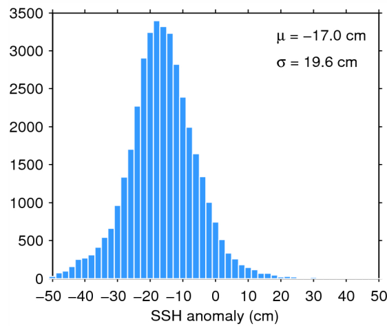
Figure 7. Histogram of flag-valid SSH anomaly over oceans and lakes for 20/06/2014. The mean ( \mu ) and standard deviation ( \sigma ) are also shown. Note that values outside [-50\ 50] cm are excluded from the histogram for the sake of readability but not from the computation of \mu and \sigma .
