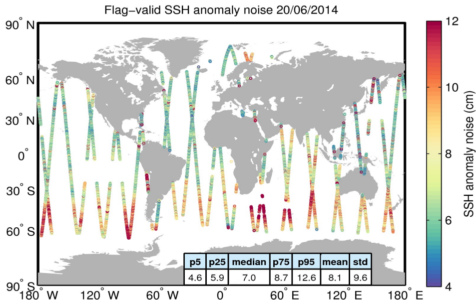
Figure 8. Geographical distribution of flag-valid 20-Hz SSH anomaly measurement noise over oceans and lakes for 20/06/2014. The statistical values shown in the table refer to the SSH anomaly noise and are calculated over all measurements shown in the figure.
