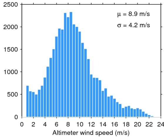
Figure 33. Histogram of flag-valid wind over oceans and lakes for 20/06/2014. The mean ( \mu ) and standard deviation ( \sigma ) are also shown. Note that values larger than 24 m/s are excluded from the histogram for the sake of readability but not from the computation of \mu and \sigma .
