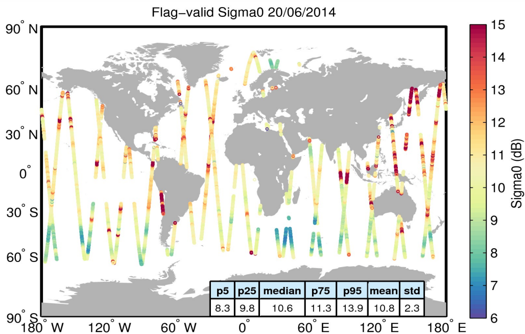
Figure 23. Geographical distribution of flag-valid sigma0 data over oceans and lakes for 20/06/2014. The statistical values shown in the table refer to the sigma0 in dB and are calculated over all measurements shown in the figure.
