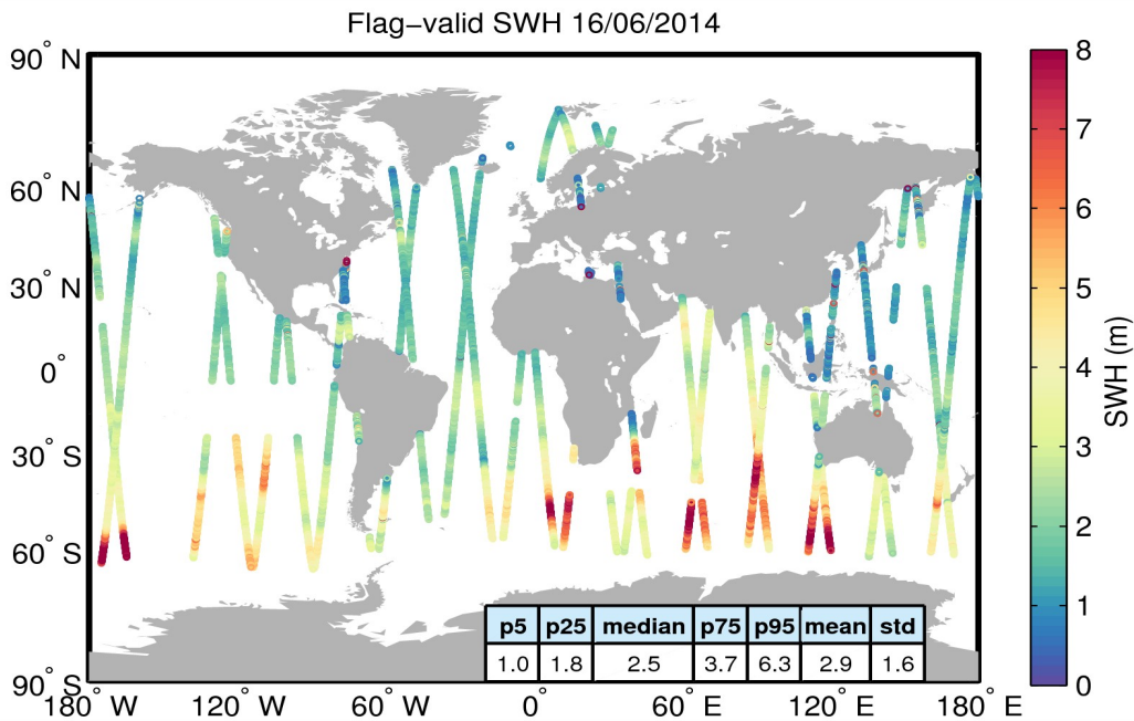
Figure 15. Geographical distribution of flag-valid SWH data over oceans and lakes for 16/06/2014. The statistical values shown in the table refer to the SWH in m and are calculated over all measurements shown in the figure.
