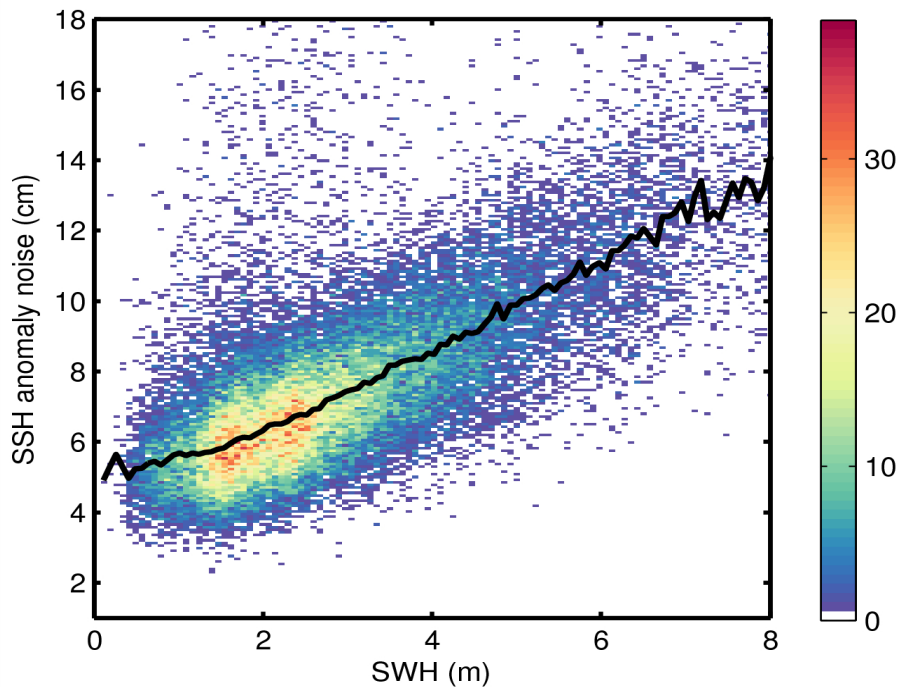
Figure 9. 2D histogram showing flag-valid SSH anomaly noise as a function of SWH for 16/06/2014. The black line denotes the median SSH anomaly as a function of SWH.
