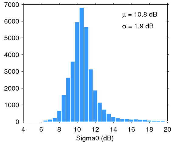
Figure 25. Histogram of flag-valid sigma0 over oceans and lakes for 16/06/2014. The mean ( \mu ) and standard deviation ( \sigma ) are also shown. Note that values outside [4 20] dB are excluded from the histogram for the sake of readability but not from the computation of \mu and \sigma .
