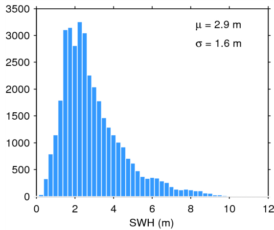
Figure 17. Histogram of flag-valid SWH over oceans and lakes for 16/06/2014. The mean ( \mu ) and standard deviation ( \sigma ) are also shown. Note that values larger than 12 m are excluded from the histogram for the sake of readability but not from the computation of \mu and \sigma .
