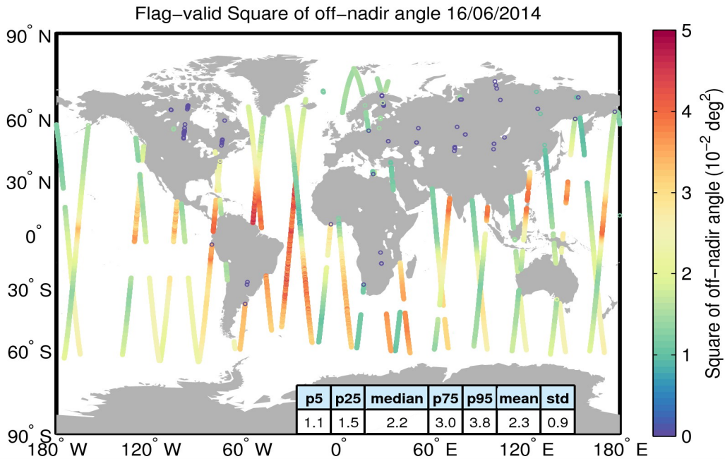
Figure 37. Geographical distribution of flag-valid mispointing data over oceans and lakes for 16/06/2014. The statistical values shown in the table refer to the mispointing in 10^{-2} deg 2 and are calculated over all measurements shown in the figure.
