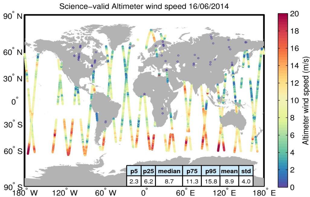
Figure 34. Geographical distribution of science-valid wind data over oceans and lakes for 16/06/2014. The statistical values shown in the table refer to the wind in m/s and are calculated over all measurements shown in the figure. Gray circles denote records that have been rejected based on the editing criteria described in Table 5.
