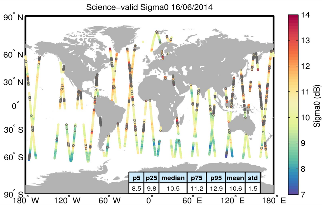
Figure 27. Geographical distribution of science-valid sigma0 data over oceans and lakes for 16/06/2014. The statistical values shown in the table refer to the sigma0 in dB and are calculated over all measurements shown in the figure. Gray circles denote records that have been rejected based on the editing criteria described in Table 4.
