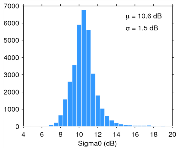
Figure 28. Histogram of science-valid sigma0 over oceans and lakes for 16/06/2014. The mean ( \mu ) and standard deviation ( \sigma ) are also shown. Note that values outside [4 20] dB are excluded from the histogram for the sake of readability but not from the computation of \mu and \sigma .
