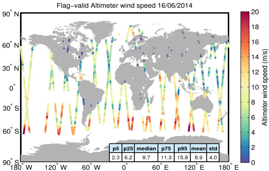
Figure 31. Geographical distribution of flag-valid wind data over oceans and lakes for 16/06/2014. The statistical values shown in the table refer to the wind in m/s and are calculated over all measurements shown in the figure.
