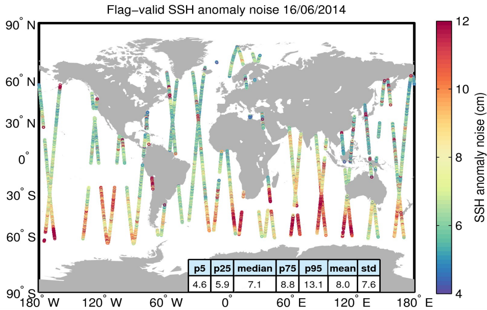
Figure 8. Geographical distribution of flag-valid 20-Hz SSH anomaly measurement noise over oceans and lakes for 16/06/2014. The statistical values shown in the table refer to the SSH anomaly noise and are calculated over all measurements shown in the figure.
