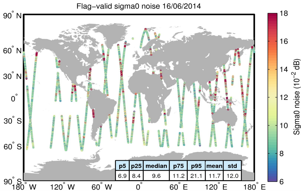
Figure 26. Geographical distribution of flag-valid 20-Hz sigma0 measurement noise over oceans and lakes for 16/06/2014. The statistical values shown in the table refer to the sigma0 noise and are calculated over all measurements shown in the figure.
