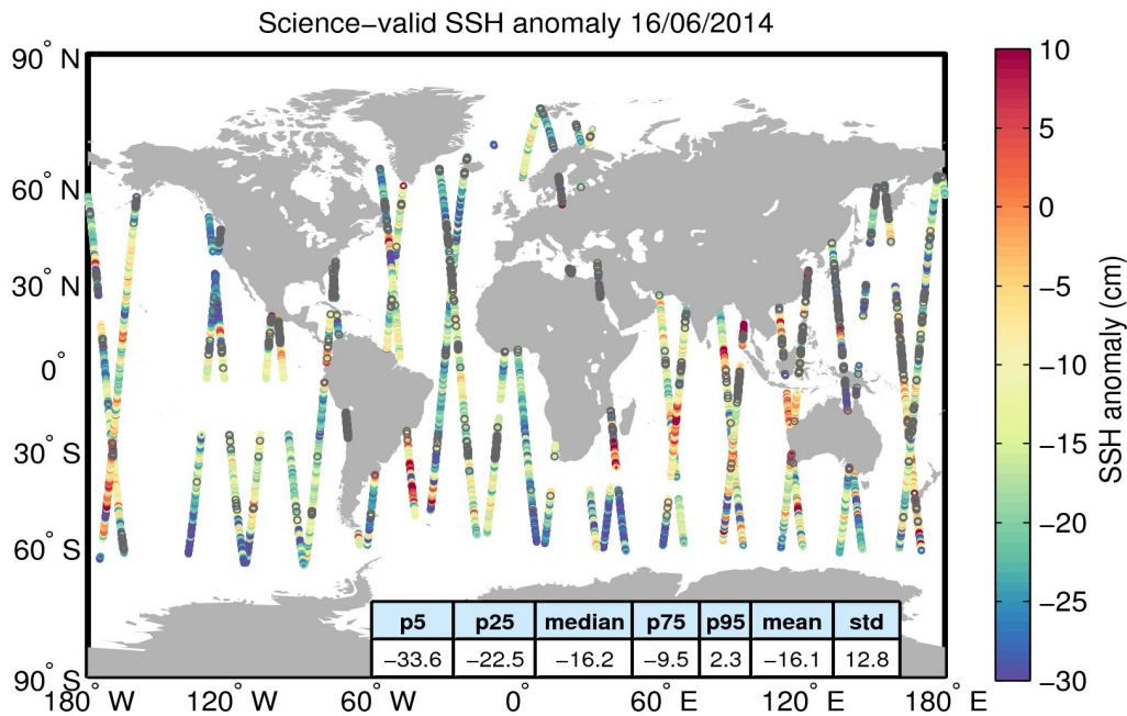
Figure 10. Geographical distribution of science-valid SSH anomaly data over oceans and lakes for 16/06/2014. The statistical values shown in the table refer to the SSH anomaly in cm and are calculated over all measurements shown in the figure. Gray circles denote records that have been rejected based on the editing criteria described in Table 2.
