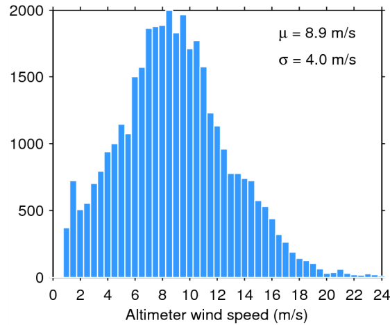
Figure 33. Histogram of flag-valid wind over oceans and lakes for 16/06/2014. The mean ( \mu ) and standard deviation ( \sigma ) are also shown. Note that values larger than 24 m/s are excluded from the histogram for the sake of readability but not from the computation of \mu and \sigma .
