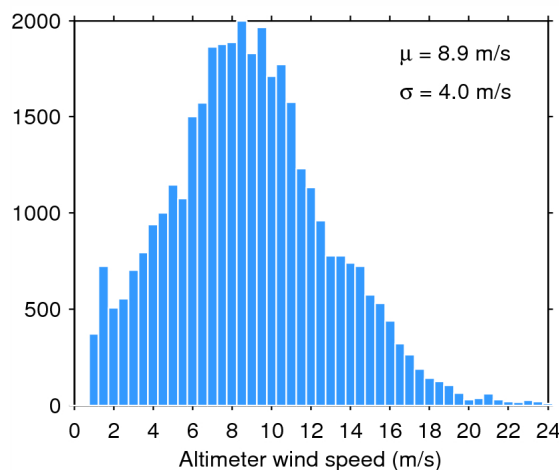
Figure 35. Histogram of science-valid wind over oceans and lakes for 16/06/2014. The mean ( \mu ) and standard deviation ( \sigma ) are also shown. Note that values larger than 24 m/s are excluded from the histogram for the sake of readability but not from the computation of \mu and \sigma .
