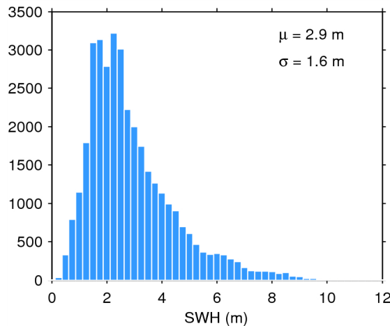
Figure 20. Histogram of science-valid SWH over oceans and lakes for 16/06/2014. The mean ( \mu ) and standard deviation ( \sigma ) are also shown. Note that values larger than 12 m are excluded from the histogram for the sake of readability but not from the computation of \mu and \sigma .
