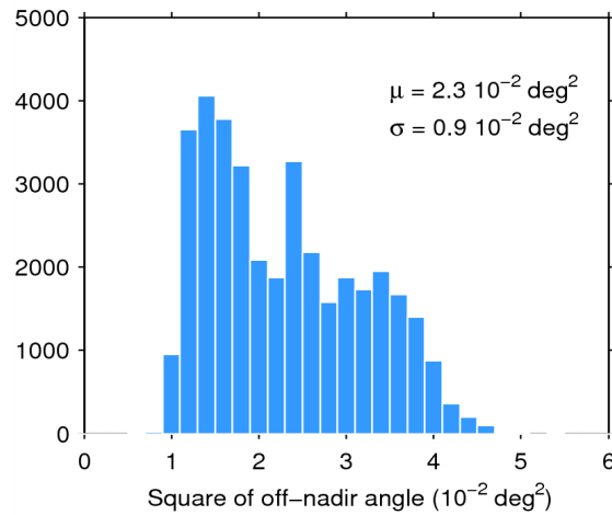
Figure 39. Histogram of flag-valid mispointing over oceans and lakes for 16/06/2014. The mean ( \mu ) and standard deviation ( \sigma ) are also shown. Note that values than 6 \cdot 10^{-2} \text{ deg}^2 are excluded from the histogram for the sake of readability but not from the computation of \mu and \sigma .
