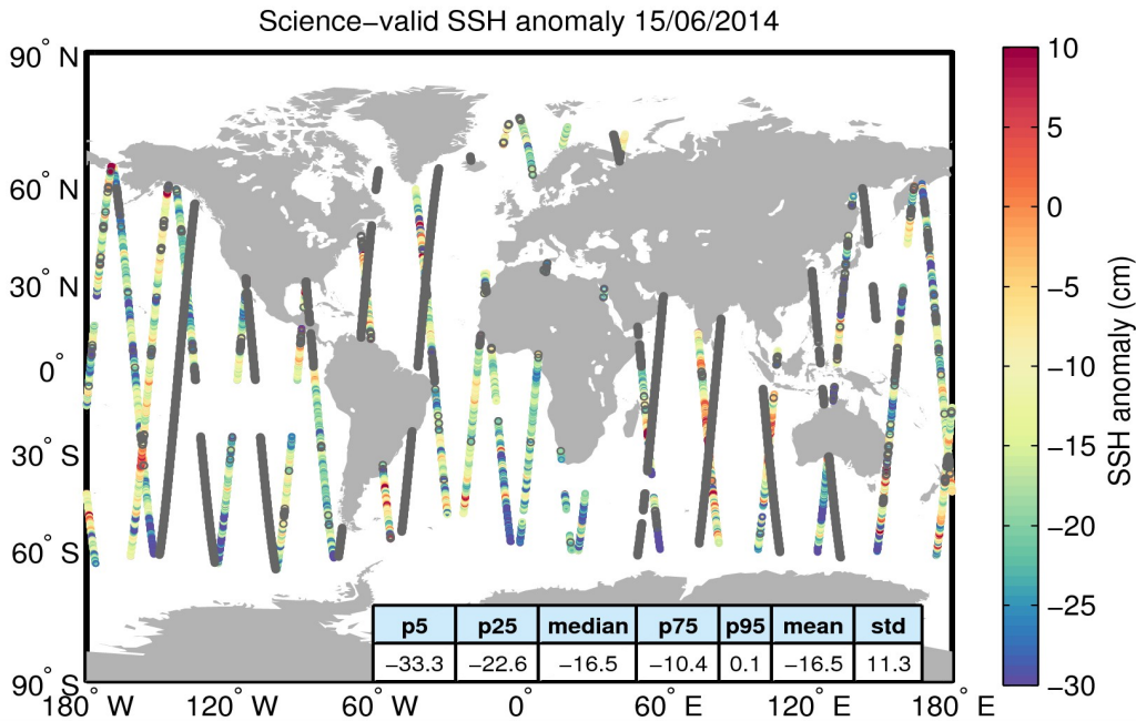
Figure 10. Geographical distribution of science-valid SSH anomaly data over oceans and lakes for 15/06/2014. The statistical values shown in the table refer to the SSH anomaly in cm and are calculated over all measurements shown in the figure. Gray circles denote records that have been rejected based on the editing criteria described in Table 2.
