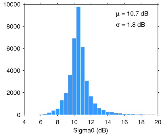
Figure 25. Histogram of flag-valid sigma0 over oceans and lakes for 15/06/2014. The mean ( \mu ) and standard deviation ( \sigma ) are also shown. Note that values outside [4 20] dB are excluded from the histogram for the sake of readability but not from the computation of \mu and \sigma .
