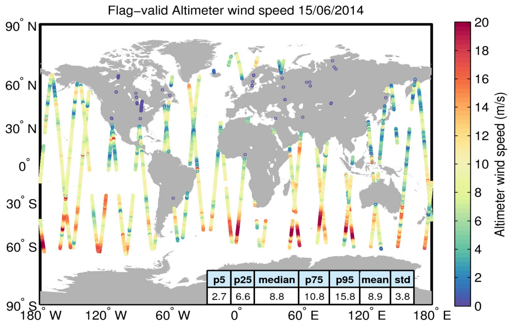
Figure 31. Geographical distribution of flag-valid wind data over oceans and lakes for 15/06/2014. The statistical values shown in the table refer to the wind in m/s and are calculated over all measurements shown in the figure.
