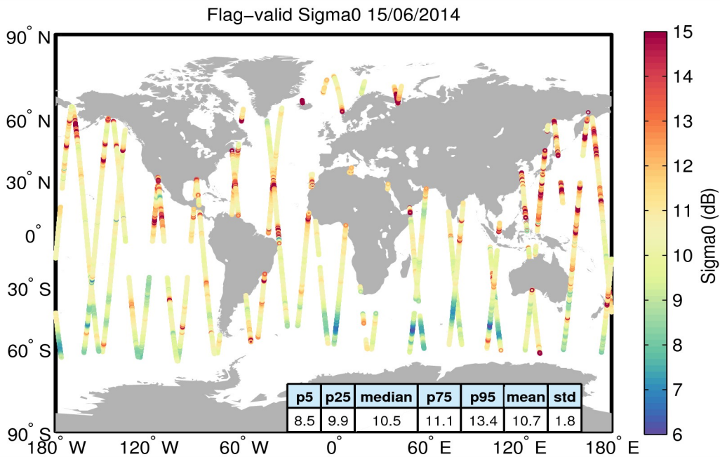
Figure 23. Geographical distribution of flag-valid sigma0 data over oceans and lakes for 15/06/2014. The statistical values shown in the table refer to the sigma0 in dB and are calculated over all measurements shown in the figure.
