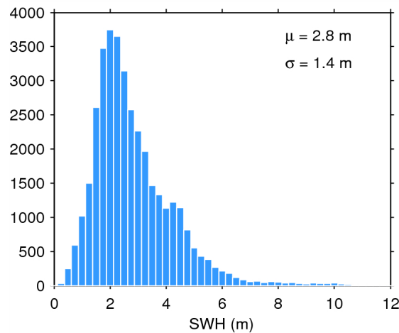
Figure 17. Histogram of flag-valid SWH over oceans and lakes for 14/06/2014. The mean ( \mu ) and standard deviation ( \sigma ) are also shown. Note that values larger than 12 m are excluded from the histogram for the sake of readability but not from the computation of \mu and \sigma .
