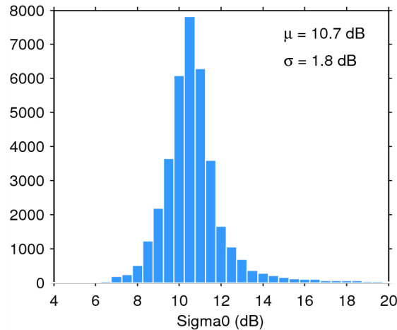
Figure 25. Histogram of flag-valid sigma0 over oceans and lakes for 14/06/2014. The mean ( \mu ) and standard deviation ( \sigma ) are also shown. Note that values outside [4 20] dB are excluded from the histogram for the sake of readability but not from the computation of \mu and \sigma .
