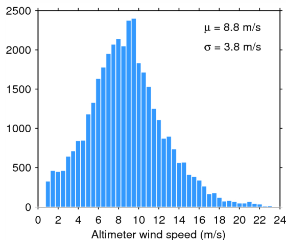
Figure 35. Histogram of science-valid wind over oceans and lakes for 14/06/2014. The mean ( \mu ) and standard deviation ( \sigma ) are also shown. Note that values larger than 24 m/s are excluded from the histogram for the sake of readability but not from the computation of \mu and \sigma .
