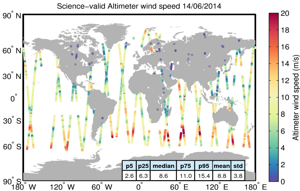
Figure 34. Geographical distribution of science-valid wind data over oceans and lakes for 14/06/2014. The statistical values shown in the table refer to the wind in m/s and are calculated over all measurements shown in the figure. Gray circles denote records that have been rejected based on the editing criteria described in Table 5.
