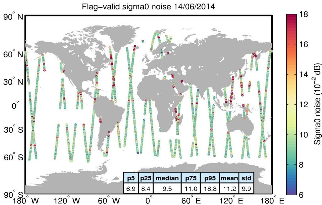
Figure 26. Geographical distribution of flag-valid 20-Hz sigma0 measurement noise over oceans and lakes for 14/06/2014. The statistical values shown in the table refer to the sigma0 noise and are calculated over all measurements shown in the figure.
