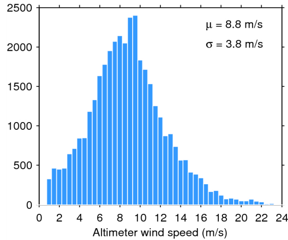
Figure 33. Histogram of flag-valid wind over oceans and lakes for 14/06/2014. The mean ( \mu ) and standard deviation ( \sigma ) are also shown. Note that values larger than 24 m/s are excluded from the histogram for the sake of readability but not from the computation of \mu and \sigma .
