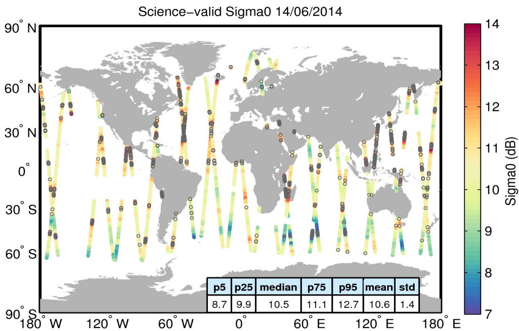
Figure 27. Geographical distribution of science-valid sigma0 data over oceans and lakes for 14/06/2014. The statistical values shown in the table refer to the sigma0 in dB and are calculated over all measurements shown in the figure. Gray circles denote records that have been rejected based on the editing criteria described in Table 4.
