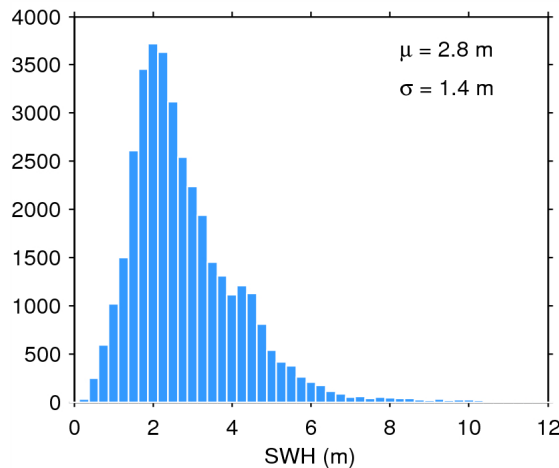
Figure 20. Histogram of science-valid SWH over oceans and lakes for 14/06/2014. The mean ( \mu ) and standard deviation ( \sigma ) are also shown. Note that values larger than 12 m are excluded from the histogram for the sake of readability but not from the computation of \mu and \sigma .
