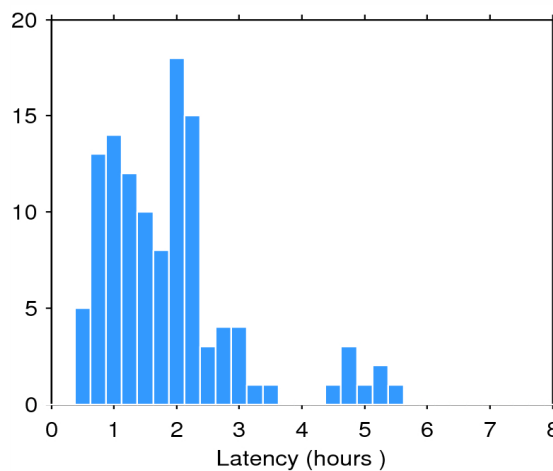
Figure 2. Histogram of the data latency for 14/06/2014. The y-axis denotes the number of files that are made available with a delay of x-hours with respect to the mean time of the records stored in the file.
