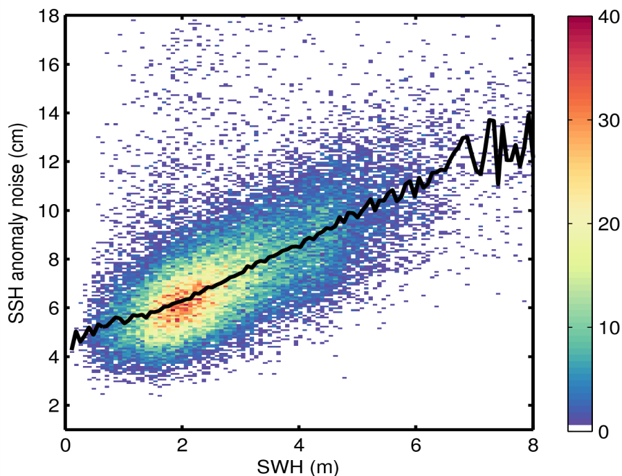
Figure 9. 2D histogram showing flag-valid SSH anomaly noise as a function of SWH for 14/06/2014. The black line denotes the median SSH anomaly as a function of SWH.
