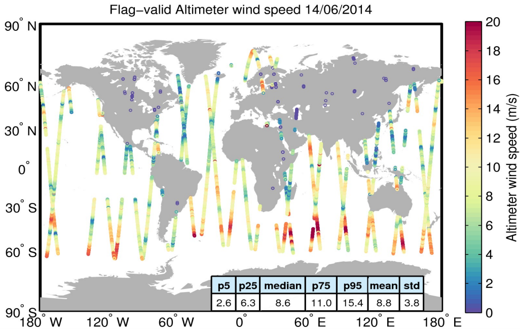
Figure 31. Geographical distribution of flag-valid wind data over oceans and lakes for 14/06/2014. The statistical values shown in the table refer to the wind in m/s and are calculated over all measurements shown in the figure.
