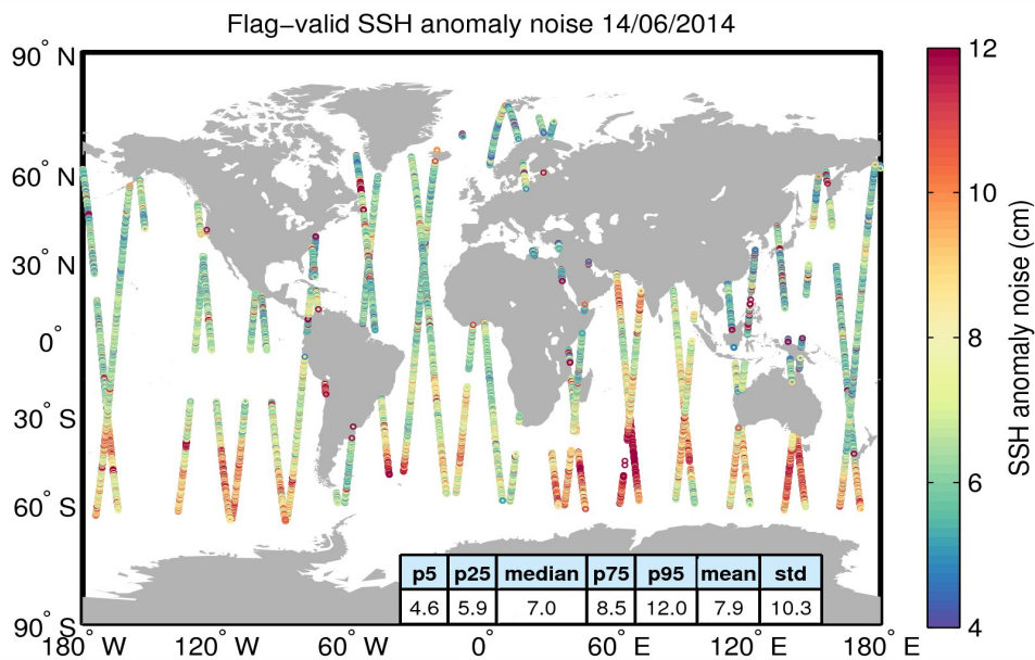
Figure 8. Geographical distribution of flag-valid 20-Hz SSH anomaly measurement noise over oceans and lakes for 14/06/2014. The statistical values shown in the table refer to the SSH anomaly noise and are calculated over all measurements shown in the figure.
