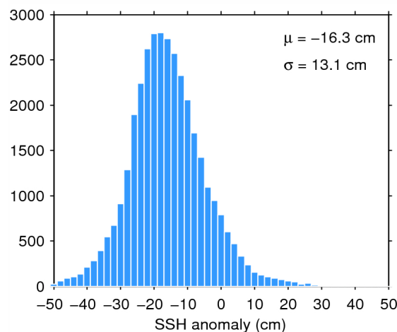
Figure 11. Histogram of science-valid SSH anomaly over oceans and lakes for 14/06/2014. The mean ( \mu ) and standard deviation ( \sigma ) are also shown. Note that values outside [-50 50] cm are excluded from the histogram for the sake of readability but not from the computation of \mu and \sigma .
