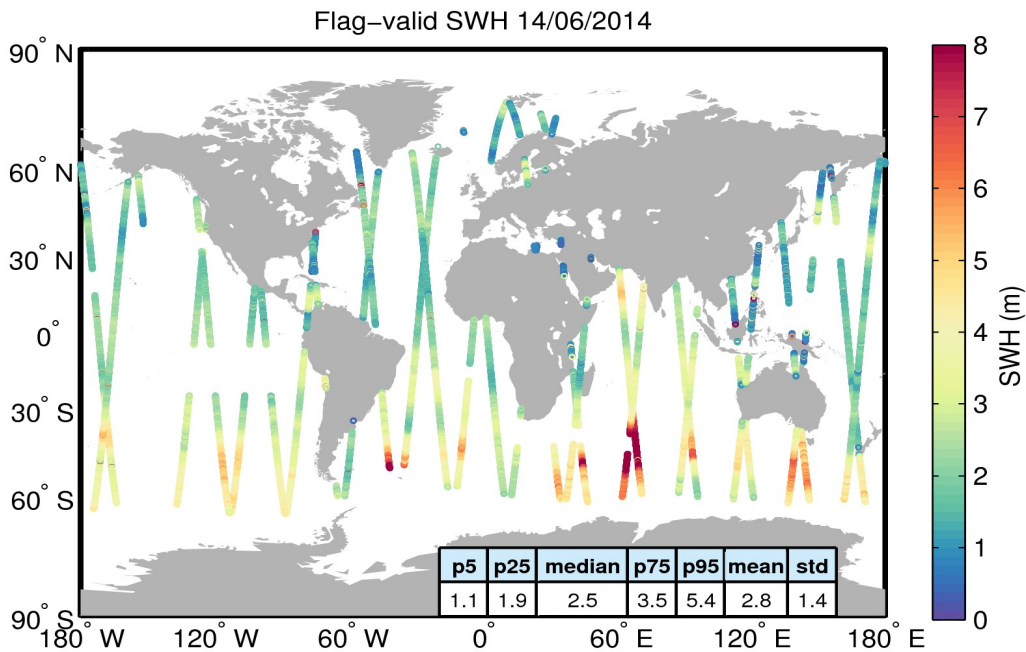
Figure 15. Geographical distribution of flag-valid SWH data over oceans and lakes for 14/06/2014. The statistical values shown in the table refer to the SWH in m and are calculated over all measurements shown in the figure.
