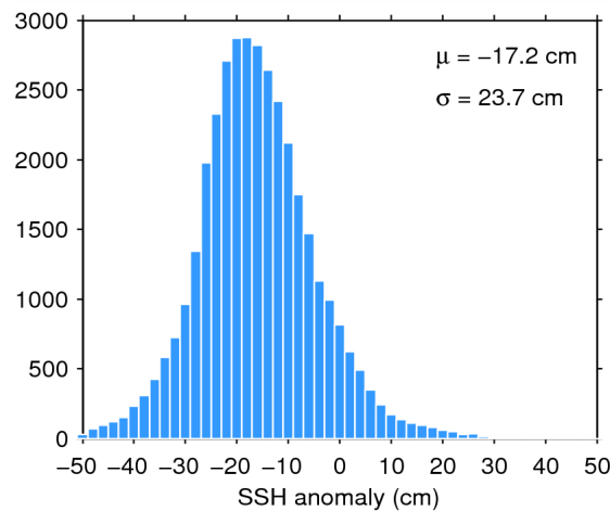
Figure 7. Histogram of flag-valid SSH anomaly over oceans and lakes for 14/06/2014. The mean ( \mu ) and standard deviation ( \sigma ) are also shown. Note that values outside [-50 50] cm are excluded from the histogram for the sake of readability but not from the computation of \mu and \sigma .
