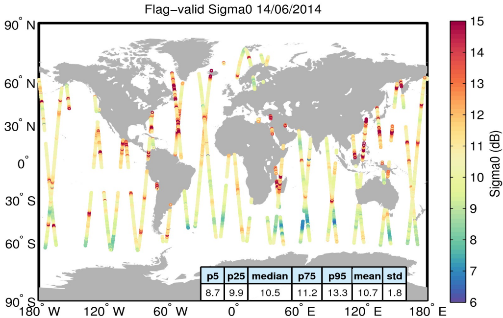
Figure 23. Geographical distribution of flag-valid sigma0 data over oceans and lakes for 14/06/2014. The statistical values shown in the table refer to the sigma0 in dB and are calculated over all measurements shown in the figure.
