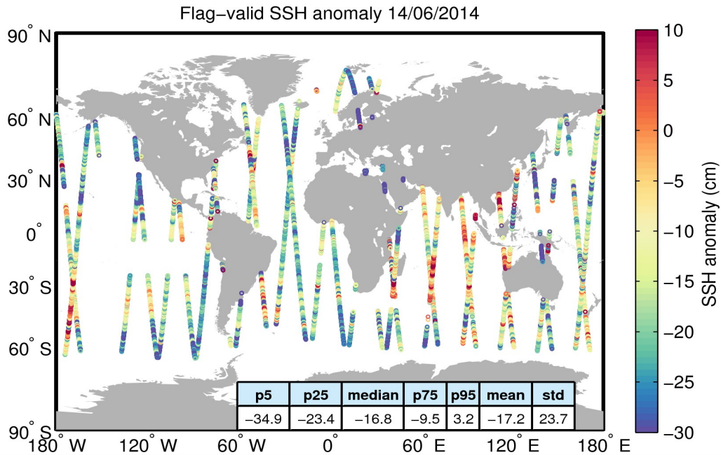
Figure 5. Geographical distribution of flag-valid 1-Hz SSH anomaly data over oceans and lakes for 14/06/2014. The statistical values shown in the table refer to the SSH anomaly in cm and are calculated over all measurements shown in the figure.
