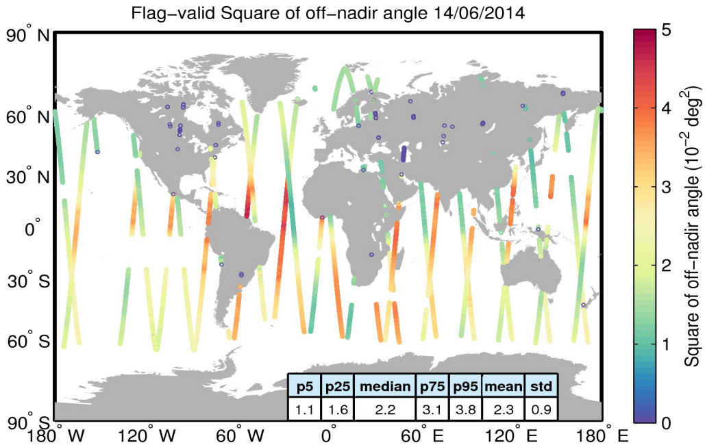
Figure 37. Geographical distribution of flag-valid mispointing data over oceans and lakes for 14/06/2014. The statistical values shown in the table refer to the mispointing in 10^{-2} \text{deg}^2 and are calculated over all measurements shown in the figure.
