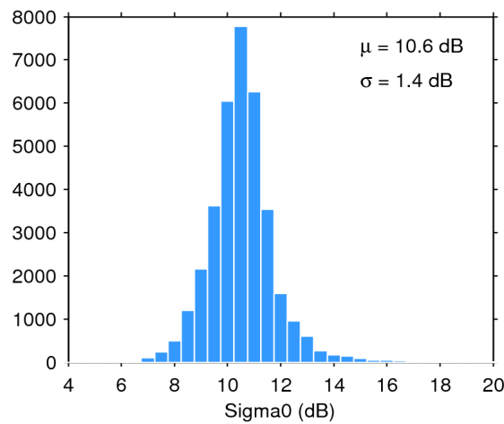
Figure 28. Histogram of science-valid sigma0 over oceans and lakes for 14/06/2014. The mean ( \mu ) and standard deviation ( \sigma ) are also shown. Note that values outside [4 20] dB are excluded from the histogram for the sake of readability but not from the computation of \mu and \sigma .
