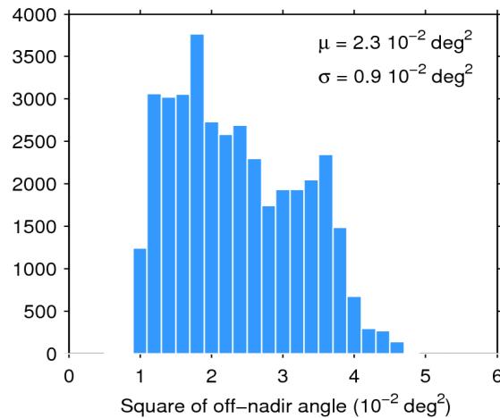
Figure 39. Histogram of flag-valid mispointing over oceans and lakes for 14/06/2014. The mean ( \mu ) and standard deviation ( \sigma ) are also shown. Note that values than 6 \cdot 10^{-2} \text{ deg}^2 are excluded from the histogram for the sake of readability but not from the computation of \mu and \sigma .
