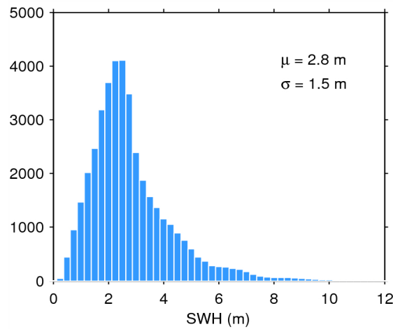
Figure 17. Histogram of flag-valid SWH over oceans and lakes for 13/06/2014. The mean ( \mu ) and standard deviation ( \sigma ) are also shown. Note that values larger than 12 m are excluded from the histogram for the sake of readability but not from the computation of \mu and \sigma .
