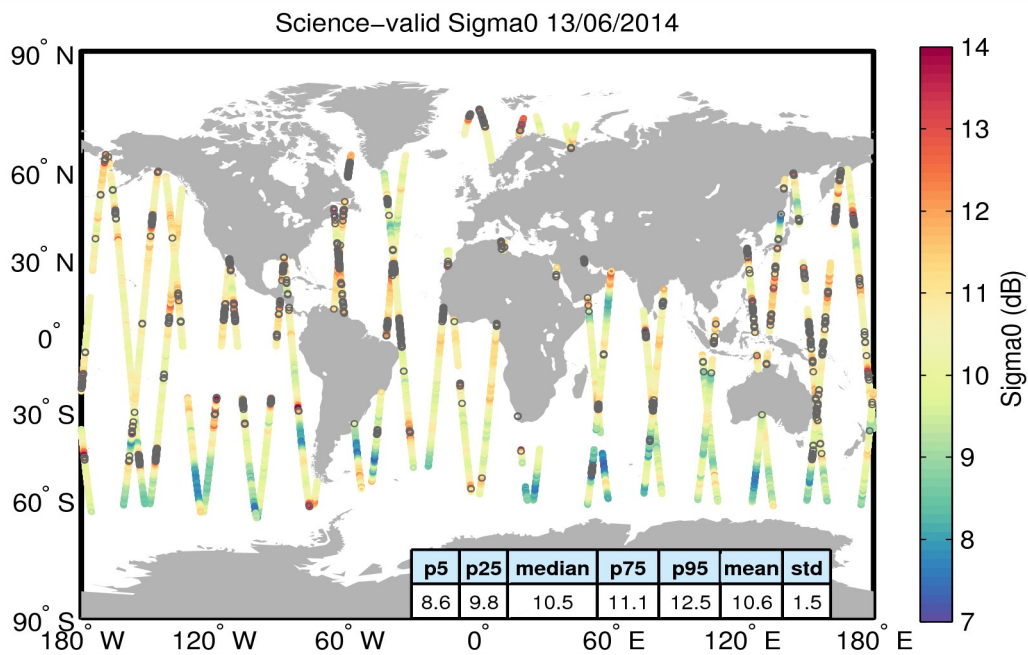
Figure 27. Geographical distribution of science-valid sigma0 data over oceans and lakes for 13/06/2014. The statistical values shown in the table refer to the sigma0 in dB and are calculated over all measurements shown in the figure. Gray circles denote records that have been rejected based on the editing criteria described in Table 4.
