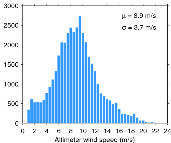
Figure 35. Histogram of science-valid wind over oceans and lakes for 13/06/2014. The mean ( \mu ) and standard deviation ( \sigma ) are also shown. Note that values larger than 24 m/s are excluded from the histogram for the sake of readability but not from the computation of \mu and \sigma .
