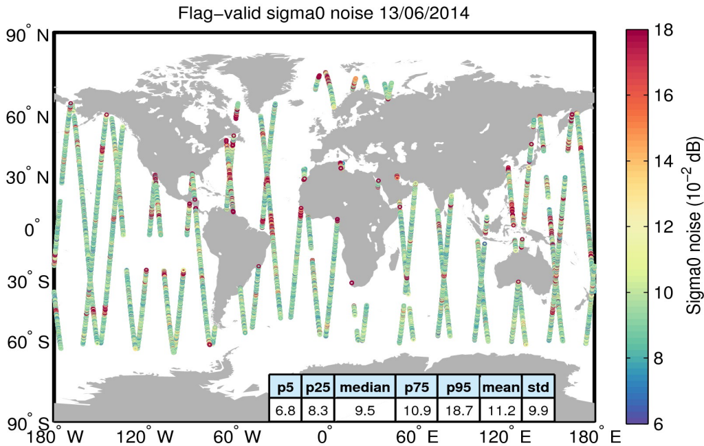
Figure 26. Geographical distribution of flag-valid 20-Hz sigma0 measurement noise over oceans and lakes for 13/06/2014. The statistical values shown in the table refer to the sigma0 noise and are calculated over all measurements shown in the figure.
