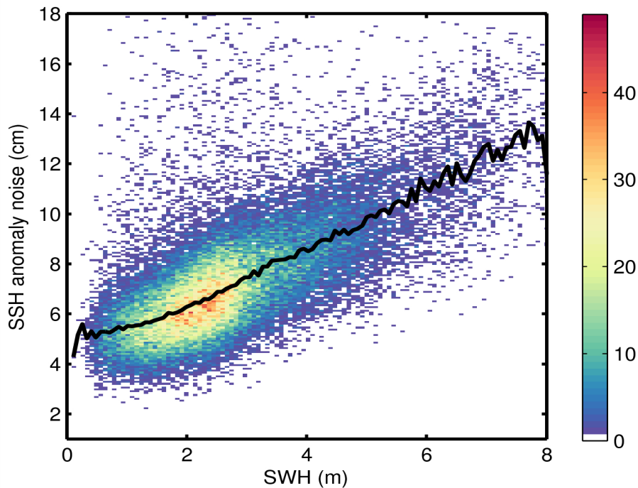
Figure 9. 2D histogram showing flag-valid SSH anomaly noise as a function of SWH for 13/06/2014. The black line denotes the median SSH anomaly as a function of SWH.
