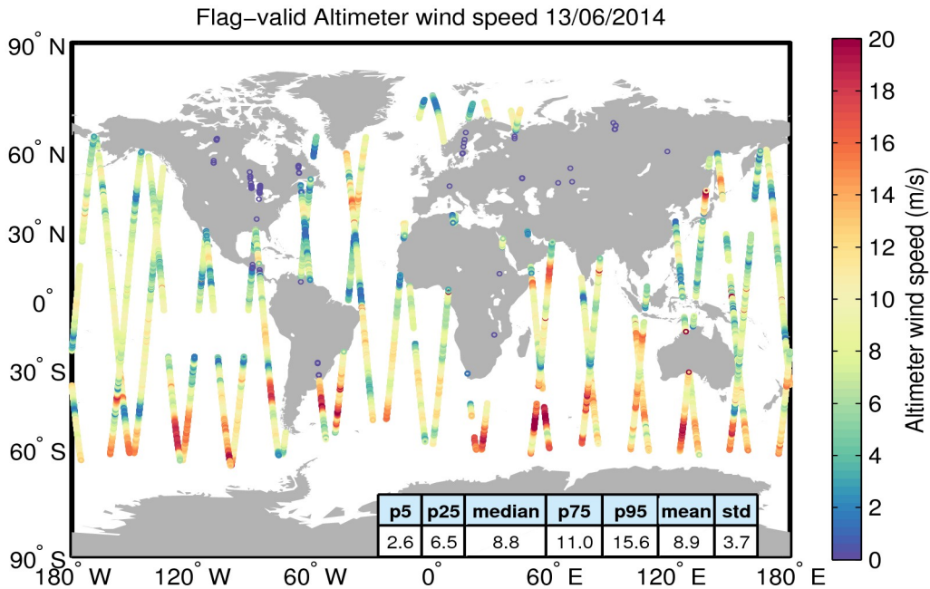
Figure 31. Geographical distribution of flag-valid wind data over oceans and lakes for 13/06/2014. The statistical values shown in the table refer to the wind in m/s and are calculated over all measurements shown in the figure.
