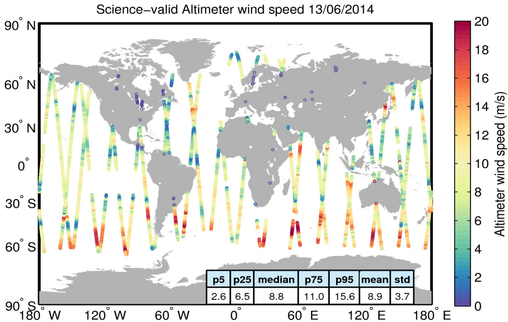
Figure 34. Geographical distribution of science-valid wind data over oceans and lakes for 13/06/2014. The statistical values shown in the table refer to the wind in m/s and are calculated over all measurements shown in the figure. Gray circles denote records that have been rejected based on the editing criteria described in Table 5.
