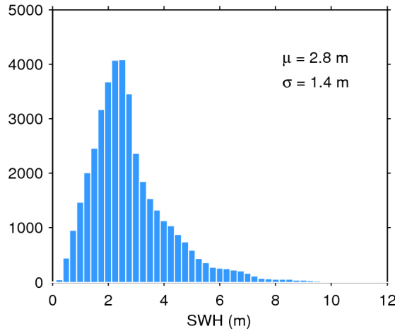
Figure 20. Histogram of science-valid SWH over oceans and lakes for 13/06/2014. The mean ( \mu ) and standard deviation ( \sigma ) are also shown. Note that values larger than 12 m are excluded from the histogram for the sake of readability but not from the computation of \mu and \sigma .
