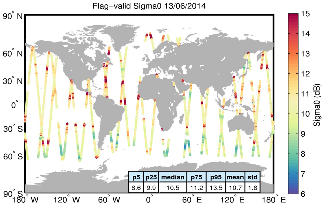
Figure 23. Geographical distribution of flag-valid sigma0 data over oceans and lakes for 13/06/2014. The statistical values shown in the table refer to the sigma0 in dB and are calculated over all measurements shown in the figure.
