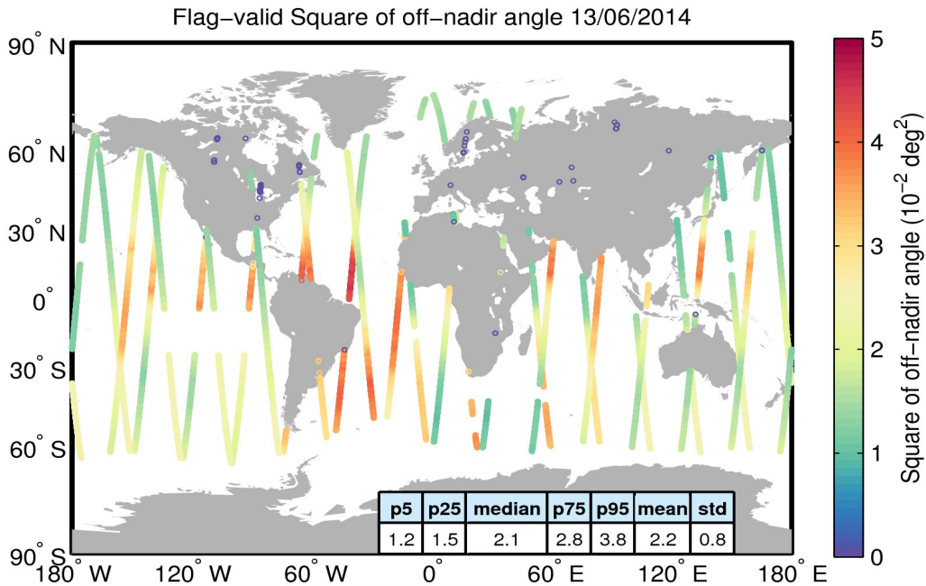
Figure 37. Geographical distribution of flag-valid mispointing data over oceans and lakes for 13/06/2014. The statistical values shown in the table refer to the mispointing in 10^{-2} \text{ deg}^2 and are calculated over all measurements shown in the figure.
