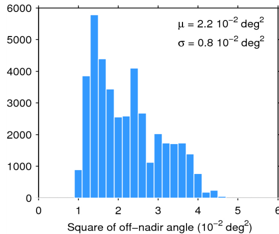
Figure 39. Histogram of flag-valid mispointing over oceans and lakes for 13/06/2014. The mean ( \mu ) and standard deviation ( \sigma ) are also shown. Note that values than 6 \cdot 10^{-2} \text{ deg}^2 are excluded from the histogram for the sake of readability but not from the computation of \mu and \sigma .
