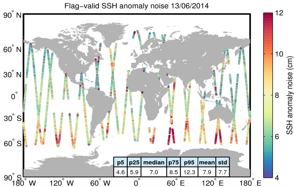
Figure 8. Geographical distribution of flag-valid 20-Hz SSH anomaly measurement noise over oceans and lakes for 13/06/2014. The statistical values shown in the table refer to the SSH anomaly noise and are calculated over all measurements shown in the figure.
