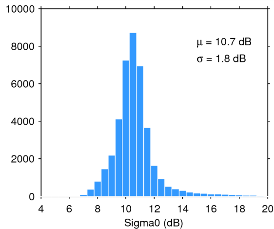
Figure 25. Histogram of flag-valid sigma0 over oceans and lakes for 13/06/2014. The mean ( \mu ) and standard deviation ( \sigma ) are also shown. Note that values outside [4 20] dB are excluded from the histogram for the sake of readability but not from the computation of \mu and \sigma .
