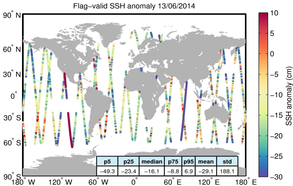
Figure 5. Geographical distribution of flag-valid 1-Hz SSH anomaly data over oceans and lakes for 13/06/2014. The statistical values shown in the table refer to the SSH anomaly in cm and are calculated over all measurements shown in the figure.
