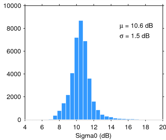
Figure 28. Histogram of science-valid sigma0 over oceans and lakes for 13/06/2014. The mean ( \mu ) and standard deviation ( \sigma ) are also shown. Note that values outside [4 20] dB are excluded from the histogram for the sake of readability but not from the computation of \mu and \sigma .
