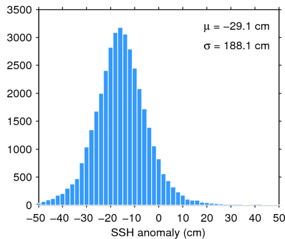
Figure 7. Histogram of flag-valid SSH anomaly over oceans and lakes for 13/06/2014. The mean ( \mu ) and standard deviation ( \sigma ) are also shown. Note that values outside [-50 50] cm are excluded from the histogram for the sake of readability but not from the computation of \mu and \sigma .
