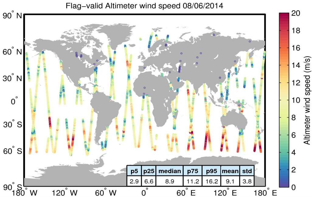
Figure 31. Geographical distribution of flag-valid wind data over oceans and lakes for 08/06/2014. The statistical values shown in the table refer to the wind in m/s and are calculated over all measurements shown in the figure.
