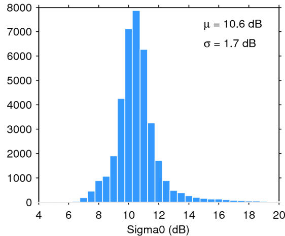
Figure 25. Histogram of flag-valid sigma0 over oceans and lakes for 08/06/2014. The mean ( \mu ) and standard deviation ( \sigma ) are also shown. Note that values outside [4 20] dB are excluded from the histogram for the sake of readability but not from the computation of \mu and \sigma .
