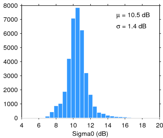
Figure 28. Histogram of science-valid sigma0 over oceans and lakes for 08/06/2014. The mean ( \mu ) and standard deviation ( \sigma ) are also shown. Note that values outside [4 20] dB are excluded from the histogram for the sake of readability but not from the computation of \mu and \sigma .
