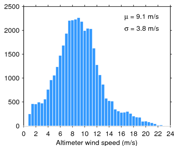
Figure 35. Histogram of science-valid wind over oceans and lakes for 08/06/2014. The mean ( \mu ) and standard deviation ( \sigma ) are also shown. Note that values larger than 24 m/s are excluded from the histogram for the sake of readability but not from the computation of \mu and \sigma .
