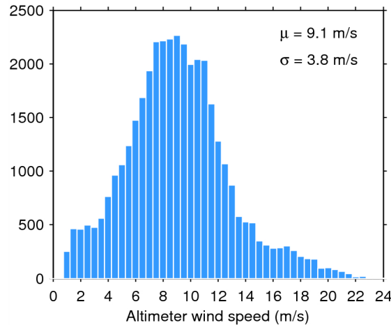
Figure 33. Histogram of flag-valid wind over oceans and lakes for 08/06/2014. The mean ( \mu ) and standard deviation ( \sigma ) are also shown. Note that values larger than 24 m/s are excluded from the histogram for the sake of readability but not from the computation of \mu and \sigma .
