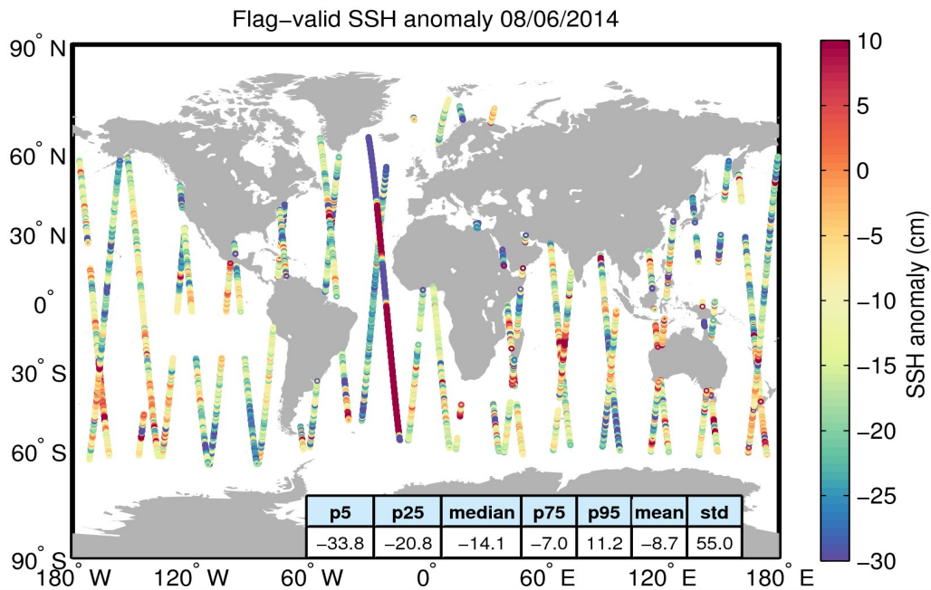
Figure 5. Geographical distribution of flag-valid 1-Hz SSH anomaly data over oceans and lakes for 08/06/2014. The statistical values shown in the table refer to the SSH anomaly in cm and are calculated over all measurements shown in the figure.
