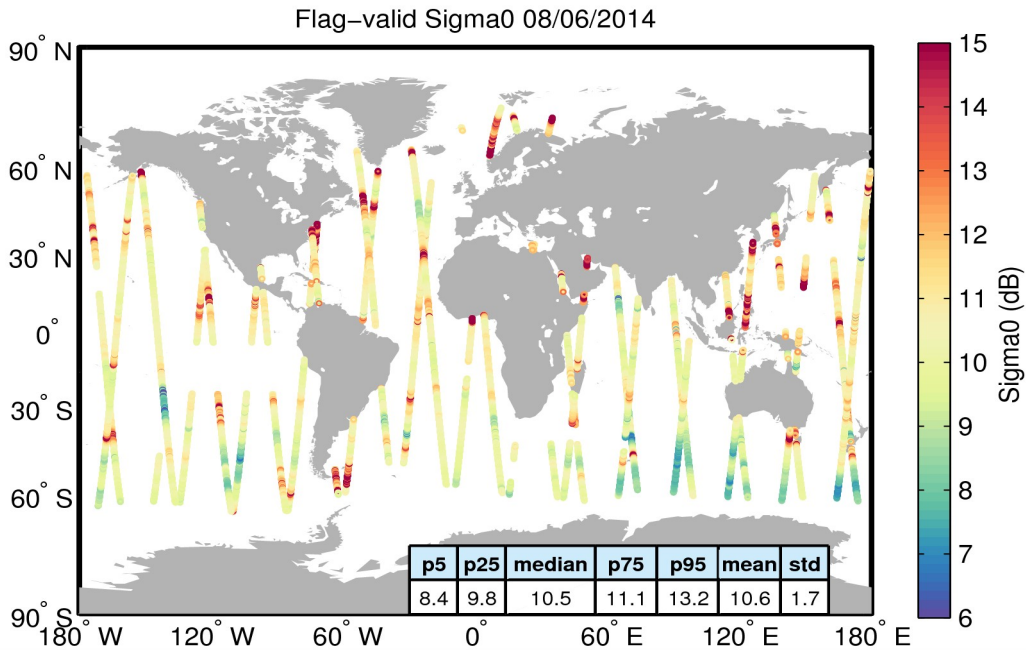
Figure 23. Geographical distribution of flag-valid sigma0 data over oceans and lakes for 08/06/2014. The statistical values shown in the table refer to the sigma0 in dB and are calculated over all measurements shown in the figure.
