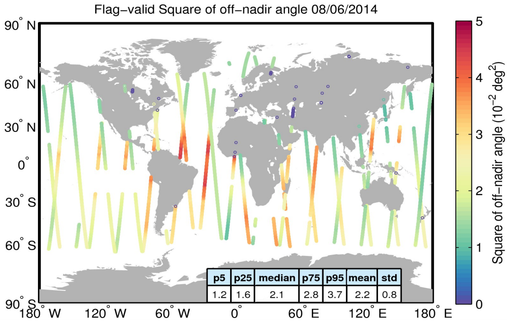
Figure 37. Geographical distribution of flag-valid mispointing data over oceans and lakes for 08/06/2014. The statistical values shown in the table refer to the mispointing in 10^{-2} \text{ deg}^2 and are calculated over all measurements shown in the figure.
