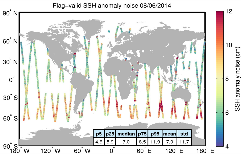
Figure 8. Geographical distribution of flag-valid 20-Hz SSH anomaly measurement noise over oceans and lakes for 08/06/2014. The statistical values shown in the table refer to the SSH anomaly noise and are calculated over all measurements shown in the figure.
