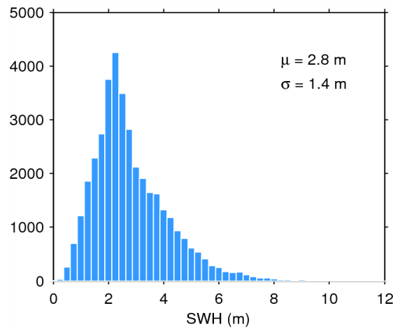
Figure 17. Histogram of flag-valid SWH over oceans and lakes for 08/06/2014. The mean ( \mu ) and standard deviation ( \sigma ) are also shown. Note that values larger than 12 m are excluded from the histogram for the sake of readability but not from the computation of \mu and \sigma .
