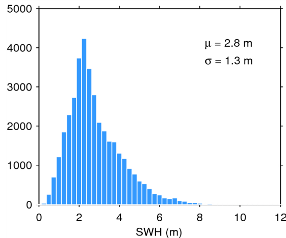
Figure 20. Histogram of science-valid SWH over oceans and lakes for 08/06/2014. The mean ( \mu ) and standard deviation ( \sigma ) are also shown. Note that values larger than 12 m are excluded from the histogram for the sake of readability but not from the computation of \mu and \sigma .
