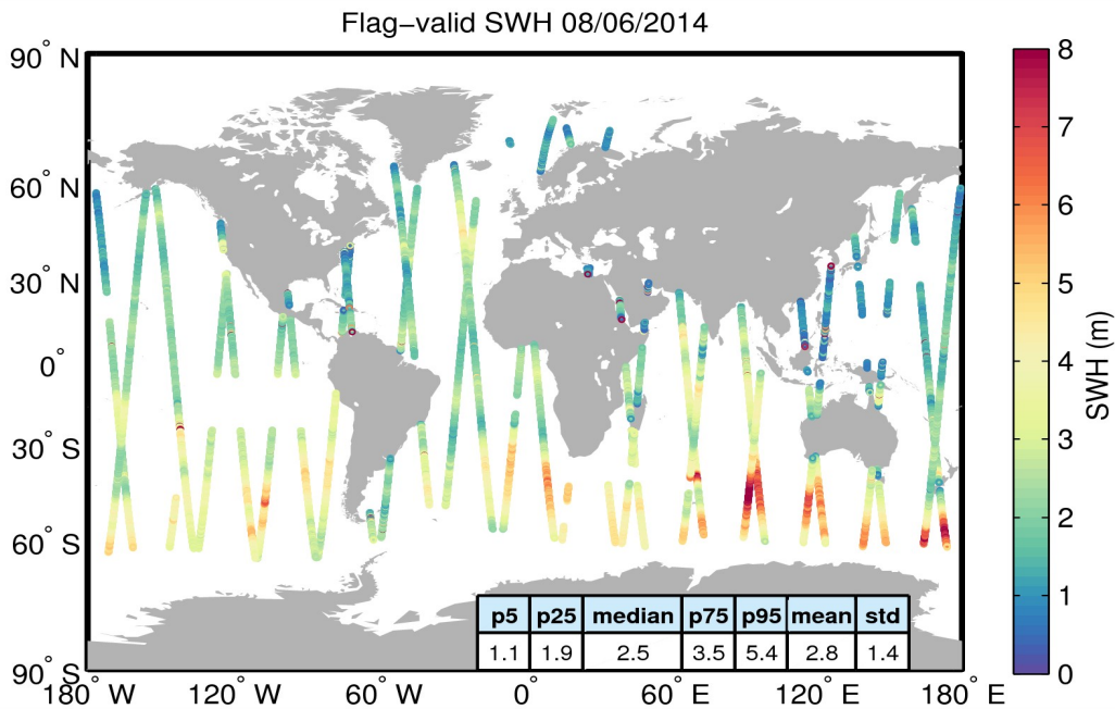
Figure 15. Geographical distribution of flag-valid SWH data over oceans and lakes for 08/06/2014. The statistical values shown in the table refer to the SWH in m and are calculated over all measurements shown in the figure.
