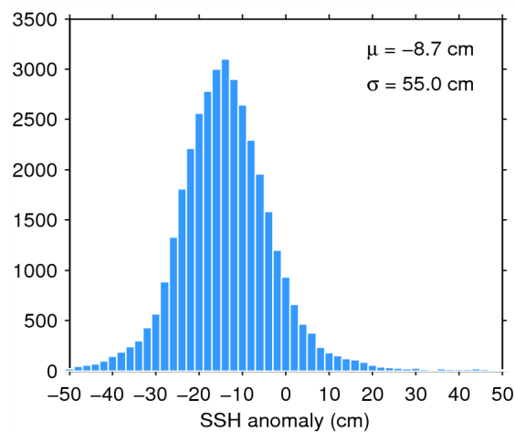
Figure 7. Histogram of flag-valid SSH anomaly over oceans and lakes for 08/06/2014. The mean ( \mu ) and standard deviation ( \sigma ) are also shown. Note that values outside [-50\ 50] cm are excluded from the histogram for the sake of readability but not from the computation of \mu and \sigma .
