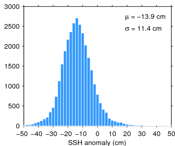
Figure 11. Histogram of science-valid SSH anomaly over oceans and lakes for 08/06/2014. The mean ( \mu ) and standard deviation ( \sigma ) are also shown. Note that values outside [-50 50] cm are excluded from the histogram for the sake of readability but not from the computation of \mu and \sigma .
