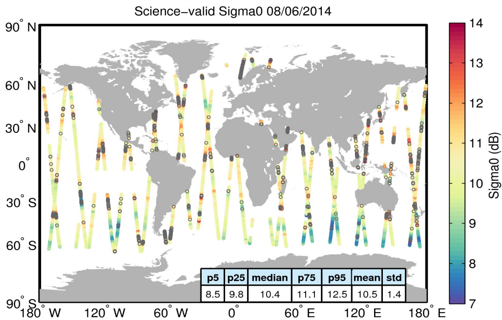
Figure 27. Geographical distribution of science-valid sigma0 data over oceans and lakes for 08/06/2014. The statistical values shown in the table refer to the sigma0 in dB and are calculated over all measurements shown in the figure. Gray circles denote records that have been rejected based on the editing criteria described in Table 4.
