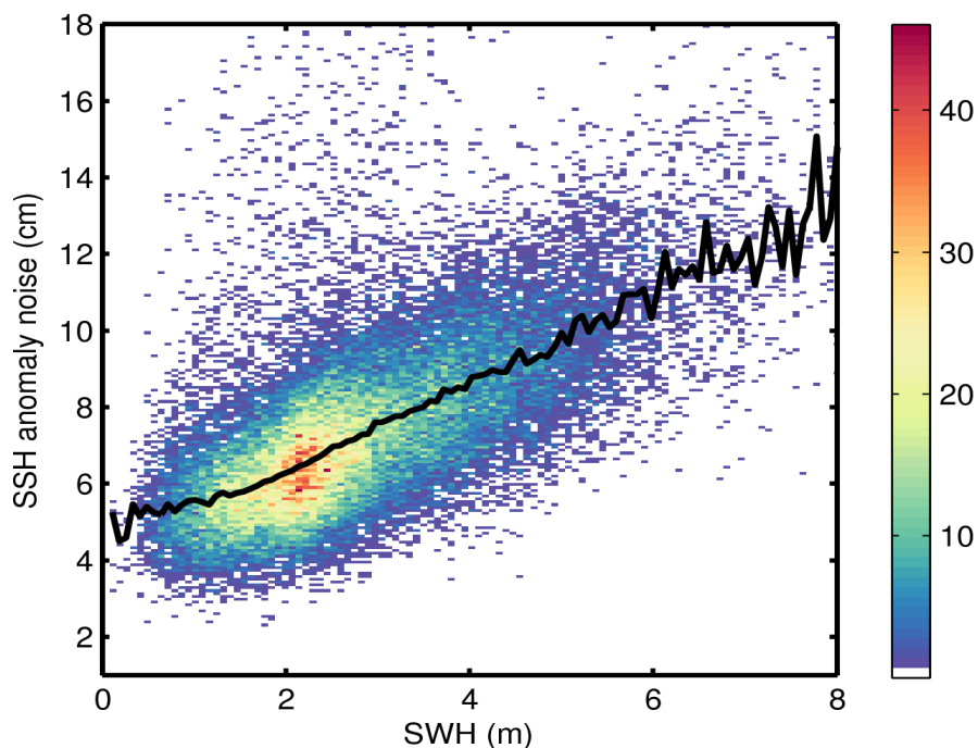
Figure 9. 2D histogram showing flag-valid SSH anomaly noise as a function of SWH for 08/06/2014. The black line denotes the median SSH anomaly as a function of SWH.
