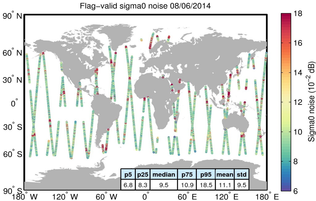
Figure 26. Geographical distribution of flag-valid 20-Hz sigma0 measurement noise over oceans and lakes for 08/06/2014. The statistical values shown in the table refer to the sigma0 noise and are calculated over all measurements shown in the figure.
