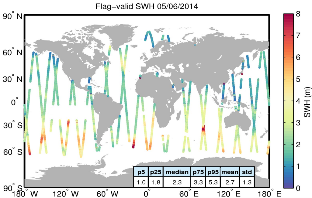
Figure 15. Geographical distribution of flag-valid SWH data over oceans and lakes for 05/06/2014. The statistical values shown in the table refer to the SWH in m and are calculated over all measurements shown in the figure.
