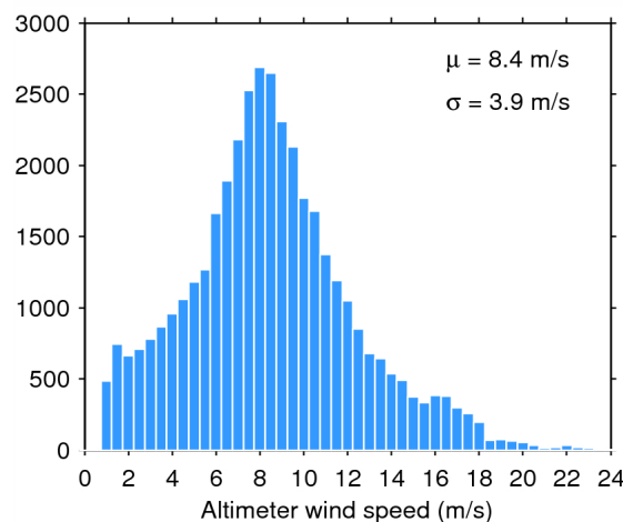
Figure 35. Histogram of science-valid wind over oceans and lakes for 05/06/2014. The mean ( \mu ) and standard deviation ( \sigma ) are also shown. Note that values larger than 24 m/s are excluded from the histogram for the sake of readability but not from the computation of \mu and \sigma .
