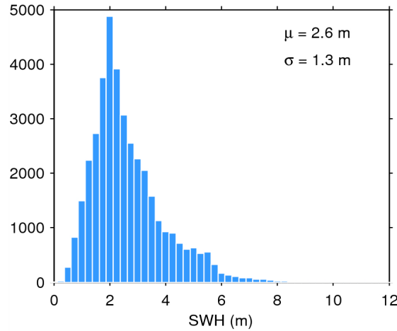
Figure 20. Histogram of science-valid SWH over oceans and lakes for 05/06/2014. The mean ( \mu ) and standard deviation ( \sigma ) are also shown. Note that values larger than 12 m are excluded from the histogram for the sake of readability but not from the computation of \mu and \sigma .
