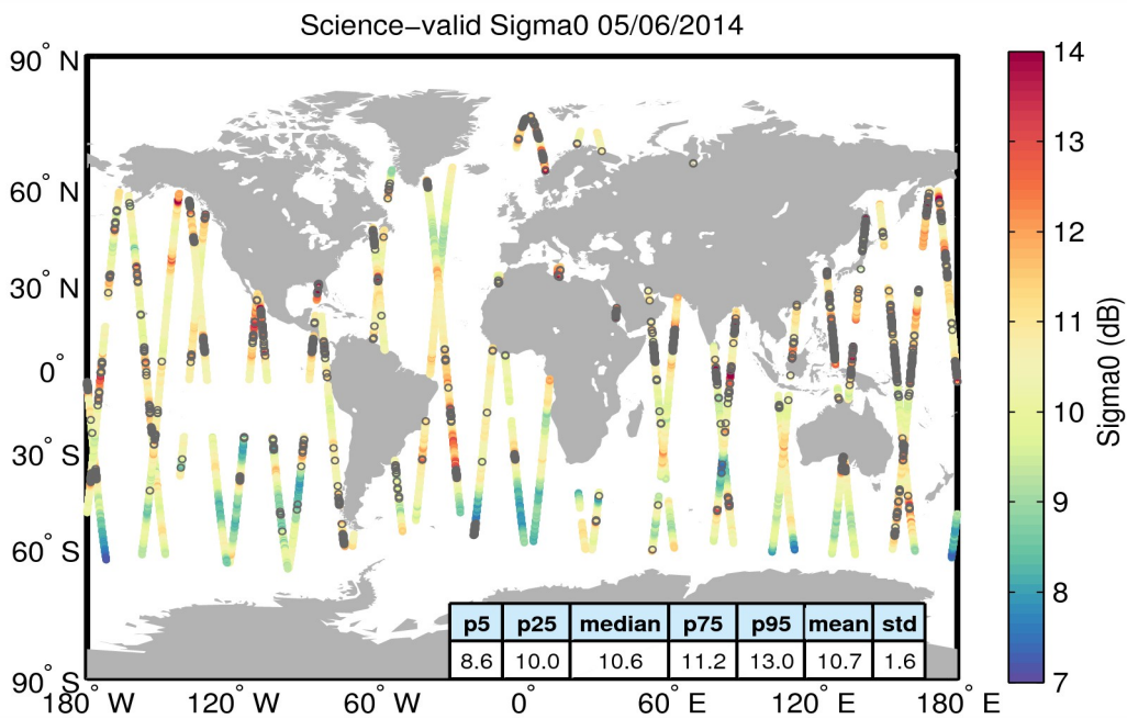
Figure 27. Geographical distribution of science-valid sigma0 data over oceans and lakes for 05/06/2014. The statistical values shown in the table refer to the sigma0 in dB and are calculated over all measurements shown in the figure. Gray circles denote records that have been rejected based on the editing criteria described in Table 4.
