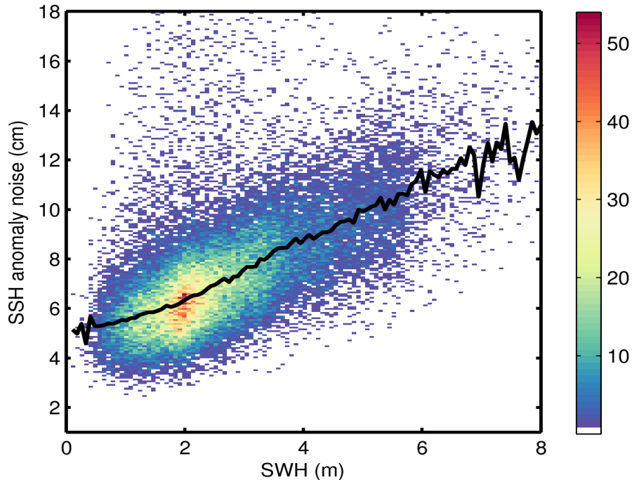
Figure 9. 2D histogram showing flag-valid SSH anomaly noise as a function of SWH for 05/06/2014. The black line denotes the median SSH anomaly as a function of SWH.
