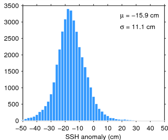
Figure 11. Histogram of science-valid SSH anomaly over oceans and lakes for 05/06/2014. The mean ( \mu ) and standard deviation ( \sigma ) are also shown. Note that values outside [-50 50] cm are excluded from the histogram for the sake of readability but not from the computation of \mu and \sigma .
