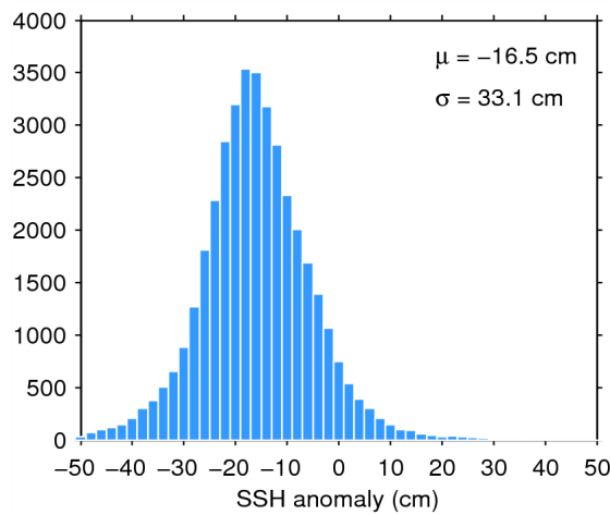
Figure 7. Histogram of flag-valid SSH anomaly over oceans and lakes for 05/06/2014. The mean ( \mu ) and standard deviation ( \sigma ) are also shown. Note that values outside [-50\ 50] cm are excluded from the histogram for the sake of readability but not from the computation of \mu and \sigma .
