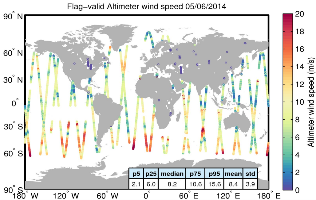
Figure 31. Geographical distribution of flag-valid wind data over oceans and lakes for 05/06/2014. The statistical values shown in the table refer to the wind in m/s and are calculated over all measurements shown in the figure.
