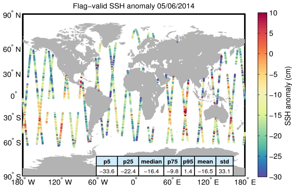
Figure 5. Geographical distribution of flag-valid 1-Hz SSH anomaly data over oceans and lakes for 05/06/2014. The statistical values shown in the table refer to the SSH anomaly in cm and are calculated over all measurements shown in the figure.
