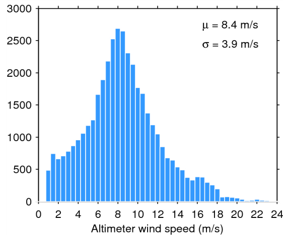
Figure 33. Histogram of flag-valid wind over oceans and lakes for 05/06/2014. The mean ( \mu ) and standard deviation ( \sigma ) are also shown. Note that values larger than 24 m/s are excluded from the histogram for the sake of readability but not from the computation of \mu and \sigma .
