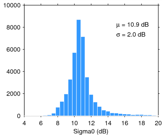
Figure 25. Histogram of flag-valid sigma0 over oceans and lakes for 05/06/2014. The mean ( \mu ) and standard deviation ( \sigma ) are also shown. Note that values outside [4 20] dB are excluded from the histogram for the sake of readability but not from the computation of \mu and \sigma .
