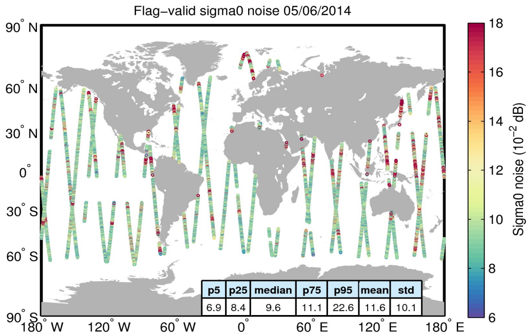
Figure 26. Geographical distribution of flag-valid 20-Hz sigma0 measurement noise over oceans and lakes for 05/06/2014. The statistical values shown in the table refer to the sigma0 noise and are calculated over all measurements shown in the figure.
