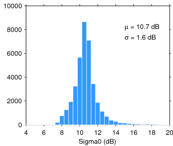
Figure 28. Histogram of science-valid sigma0 over oceans and lakes for 05/06/2014. The mean ( \mu ) and standard deviation ( \sigma ) are also shown. Note that values outside [4 20] dB are excluded from the histogram for the sake of readability but not from the computation of \mu and \sigma .
