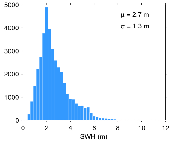
Figure 17. Histogram of flag-valid SWH over oceans and lakes for 05/06/2014. The mean ( \mu ) and standard deviation ( \sigma ) are also shown. Note that values larger than 12 m are excluded from the histogram for the sake of readability but not from the computation of \mu and \sigma .
