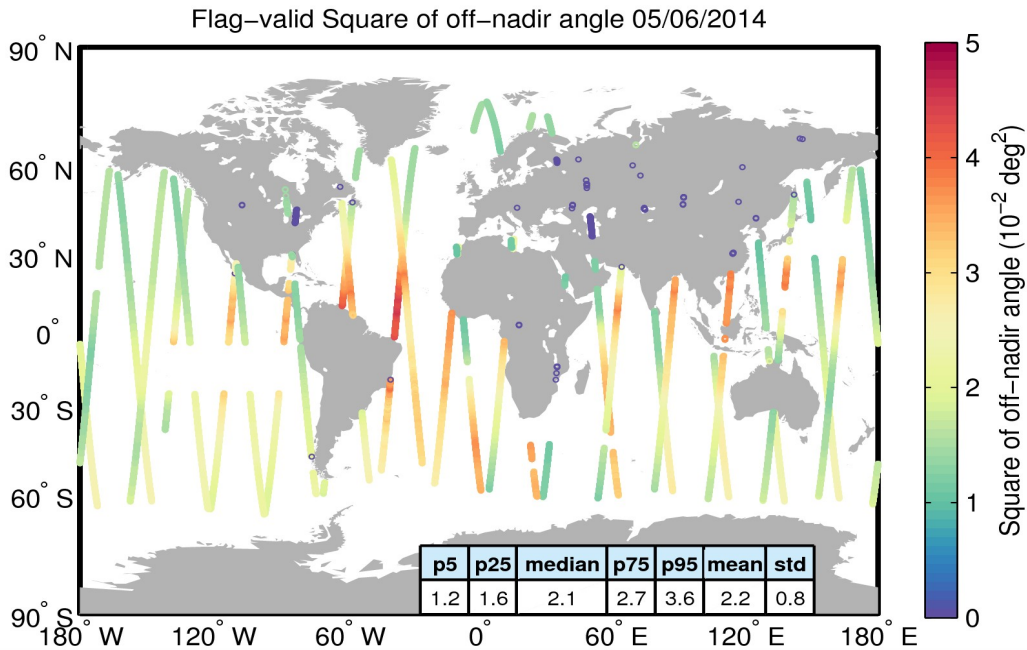
Figure 37. Geographical distribution of flag-valid mispointing data over oceans and lakes for 05/06/2014. The statistical values shown in the table refer to the mispointing in 10^{-2} \text{ deg}^2 and are calculated over all measurements shown in the figure.
