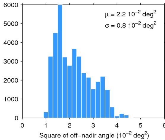
Figure 39. Histogram of flag-valid mispointing over oceans and lakes for 05/06/2014. The mean ( \mu ) and standard deviation ( \sigma ) are also shown. Note that values than 6 \cdot 10^{-2} \text{ deg}^2 are excluded from the histogram for the sake of readability but not from the computation of \mu and \sigma .
