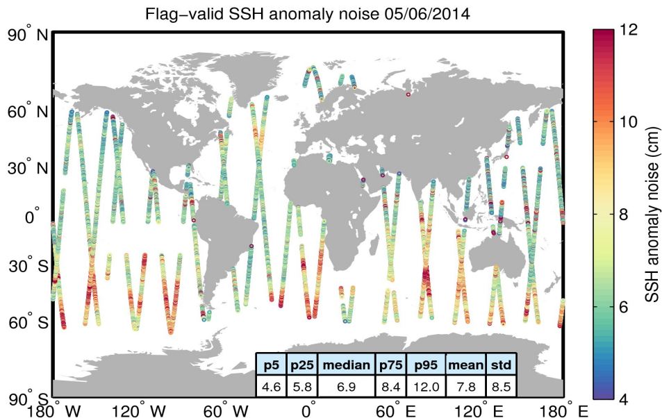
Figure 8. Geographical distribution of flag-valid 20-Hz SSH anomaly measurement noise over oceans and lakes for 05/06/2014. The statistical values shown in the table refer to the SSH anomaly noise and are calculated over all measurements shown in the figure.
