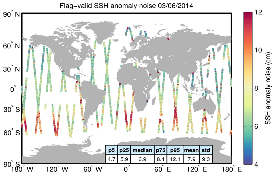
Figure 8. Geographical distribution of flag-valid 20-Hz SSH anomaly measurement noise over oceans and lakes for 03/06/2014. The statistical values shown in the table refer to the SSH anomaly noise and are calculated over all measurements shown in the figure.
