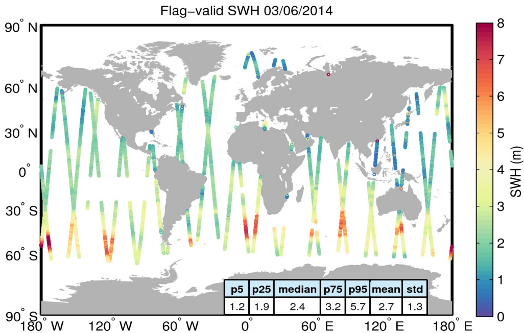
Figure 15. Geographical distribution of flag-valid SWH data over oceans and lakes for 03/06/2014. The statistical values shown in the figure refer to the SWH in m and are calculated over all measurements shown in the figure.
