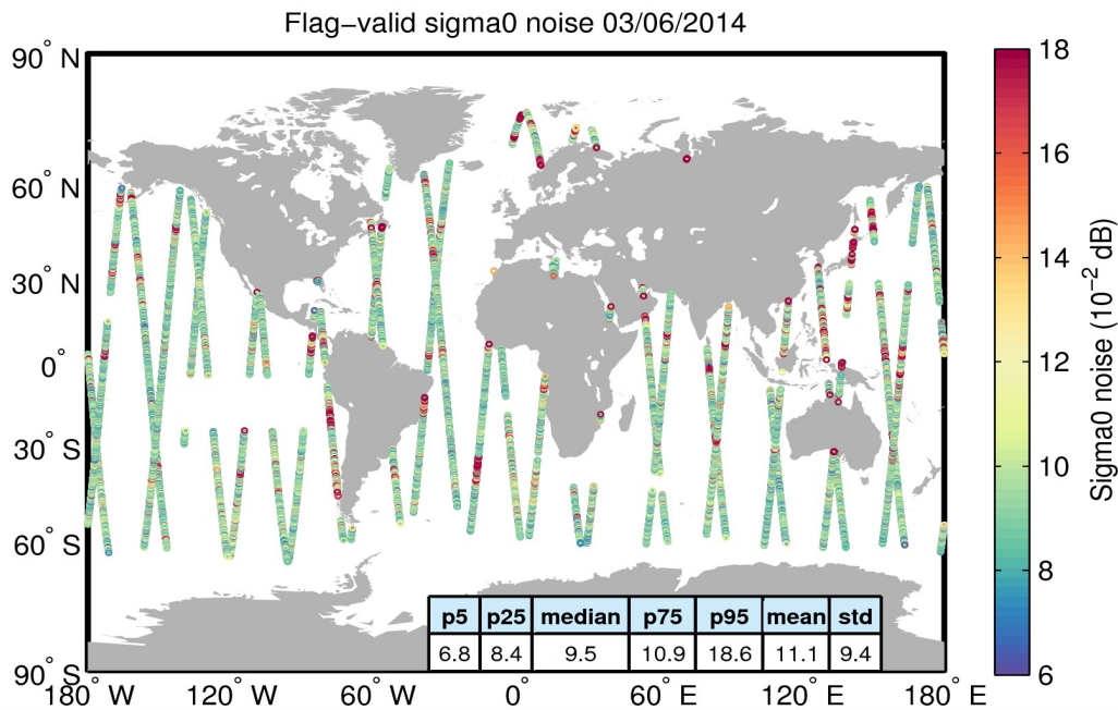
Figure 26. Geographical distribution of flag-valid 20-Hz sigma0 measurement noise over oceans and lakes for 03/06/2014. The statistical values shown in the table refer to the sigma0 noise and are calculated over all measurements shown in the figure.
