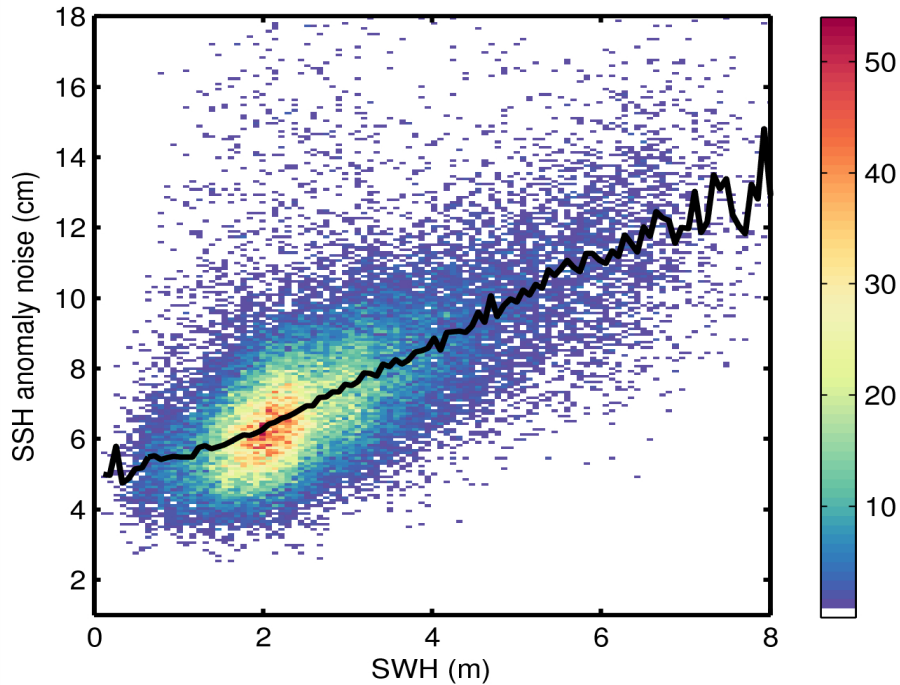
Figure 9. 2D histogram showing flag-valid SSH anomaly noise as a function of SWH for 03/06/2014. The black line denotes the median SSH anomaly as a function of SWH.
