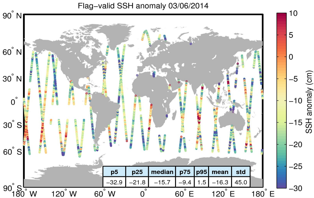
Figure 5. Geographical distribution of flag-valid 1-Hz SSH anomaly data over oceans and lakes for 03/06/2014. The statistical values shown in the table refer to the SSH anomaly in cm and are calculated over all measurements shown in the figure.
