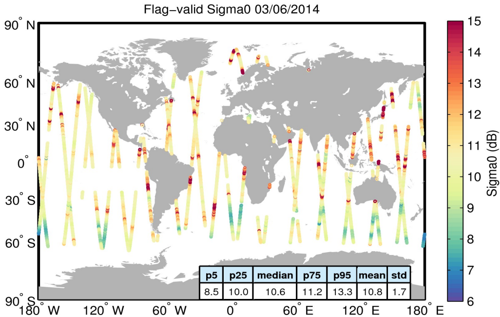
Figure 23. Geographical distribution of flag-valid sigma0 data over oceans and lakes for 03/06/2014. The statistical values shown in the table refer to the sigma0 in dB and are calculated over all measurements shown in the figure.
