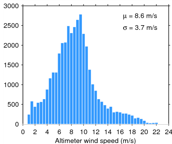
Figure 35. Histogram of science-valid wind over oceans and lakes for 03/06/2014. The mean ( \mu ) and standard deviation ( \sigma ) are also shown. Note that values larger than 24 m/s are excluded from the histogram for the sake of readability but not from the computation of \mu and \sigma .
