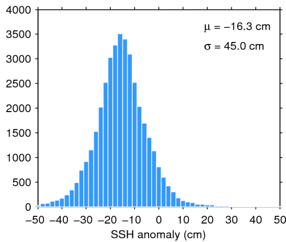
Figure 7. Histogram of flag-valid SSH anomaly over oceans and lakes for 03/06/2014. The mean ( \mu ) and standard deviation ( \sigma ) are also shown. Note that values outside [-50\ 50] cm are excluded from the histogram for the sake of readability but not from the computation of \mu and \sigma .
