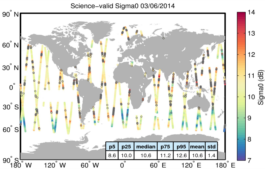
Figure 27. Geographical distribution of science-valid sigma0 data over oceans and lakes for 03/06/2014. The statistical values shown in the table refer to the sigma0 in dB and are calculated over all measurements shown in the figure. Gray circles denote records that have been rejected based on the editing criteria described in Table 4.
