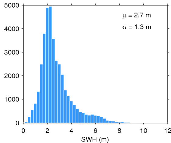
Figure 20. Histogram of science-valid SWH over oceans and lakes for 03/06/2014. The mean ( \mu ) and standard deviation ( \sigma ) are also shown. Note that values larger than 12 m are excluded from the histogram for the sake of readability but not from the computation of \mu and \sigma .
