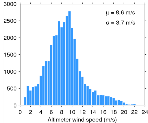
Figure 33. Histogram of flag-valid wind over oceans and lakes for 03/06/2014. The mean ( \mu ) and standard deviation ( \sigma ) are also shown. Note that values larger than 24 m/s are excluded from the histogram for the sake of readability but not from the computation of \mu and \sigma .
