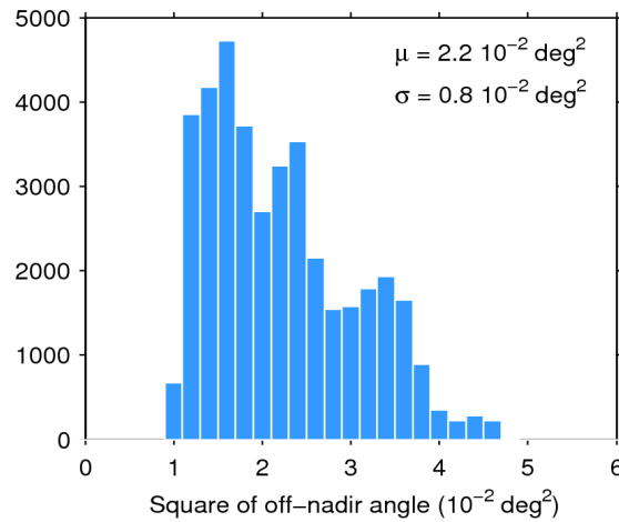
Figure 39. Histogram of flag-valid mispointing over oceans and lakes for 03/06/2014. The mean ( \mu ) and standard deviation ( \sigma ) are also shown. Note that values than 6 \cdot 10^{-2} \text{ deg}^2 are excluded from the histogram for the sake of readability but not from the computation of \mu and \sigma .
