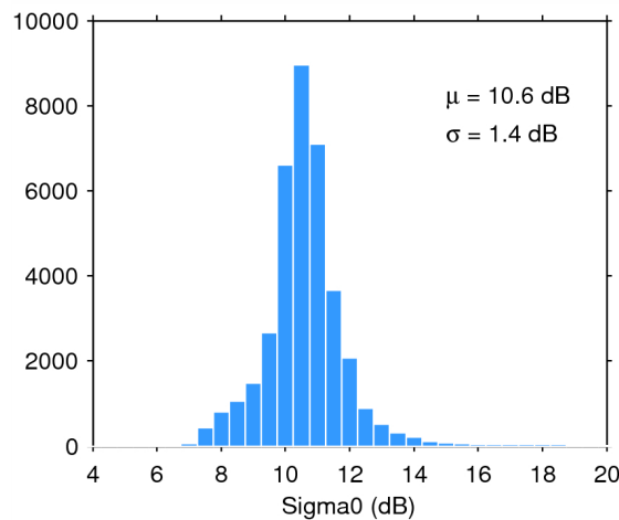
Figure 28. Histogram of science-valid sigma0 over oceans and lakes for 03/06/2014. The mean ( \mu ) and standard deviation ( \sigma ) are also shown. Note that values outside [4 20] dB are excluded from the histogram for the sake of readability but not from the computation of \mu and \sigma .
