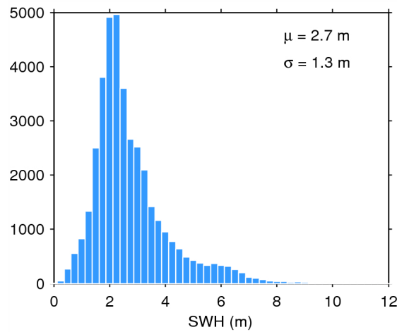
Figure 17. Histogram of flag-valid SWH over oceans and lakes for 03/06/2014. The mean ( \mu ) and standard deviation ( \sigma ) are also shown. Note that values larger than 12 m are excluded from the histogram for the sake of readability but not from the computation of \mu and \sigma .
