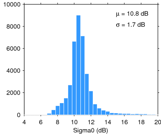
Figure 25. Histogram of flag-valid sigma0 over oceans and lakes for 03/06/2014. The mean ( \mu ) and standard deviation ( \sigma ) are also shown. Note that values outside [4 20] dB are excluded from the histogram for the sake of readability but not from the computation of \mu and \sigma .
