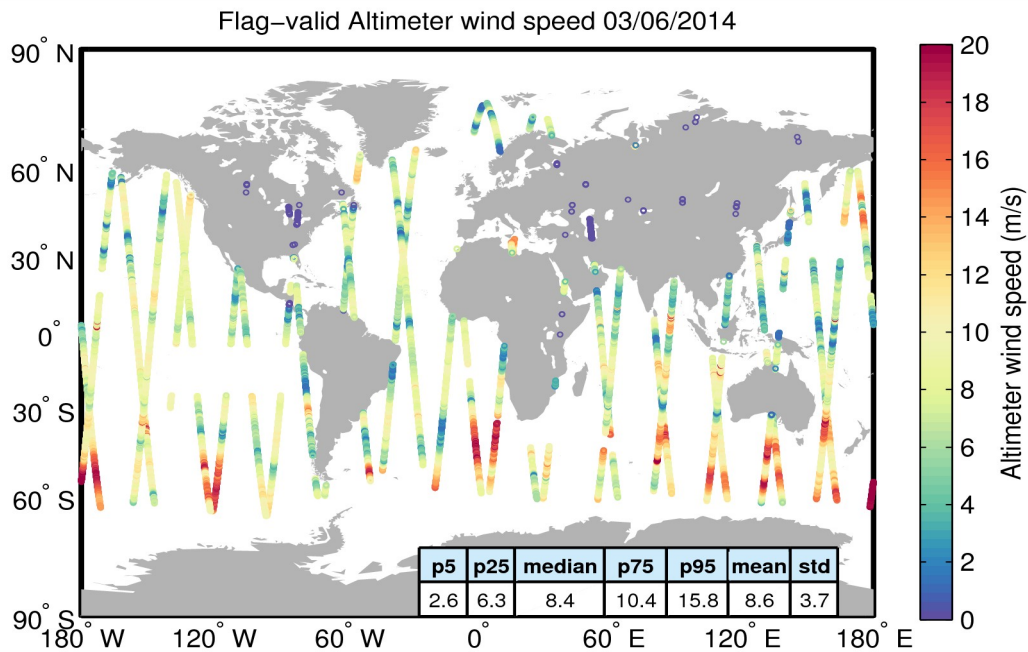
Figure 31. Geographical distribution of flag-valid wind data over oceans and lakes for 03/06/2014. The statistical values shown in the table refer to the wind in m/s and are calculated over all measurements shown in the figure.
