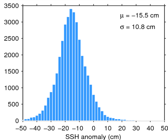
Figure 11. Histogram of science-valid SSH anomaly over oceans and lakes for 03/06/2014. The mean ( \mu ) and standard deviation ( \sigma ) are also shown. Note that values outside [-50 50] cm are excluded from the histogram for the sake of readability but not from the computation of \mu and \sigma .
