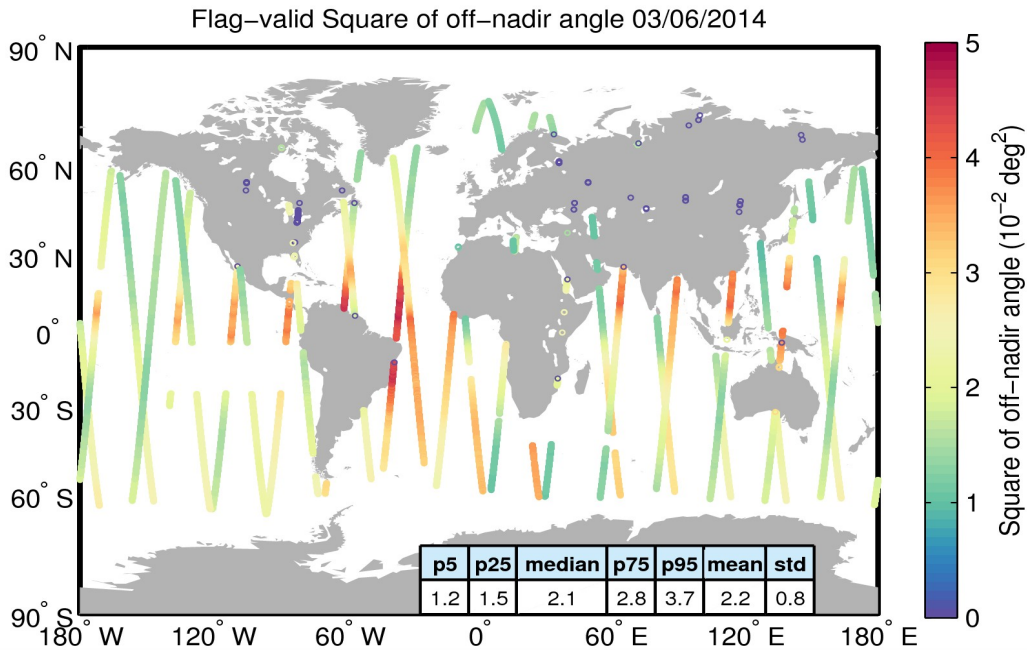
Figure 37. Geographical distribution of flag-valid mispointing data over oceans and lakes for 03/06/2014. The statistical values shown in the table refer to the mispointing in 10^{-2} \text{ deg}^2 and are calculated over all measurements shown in the figure.
