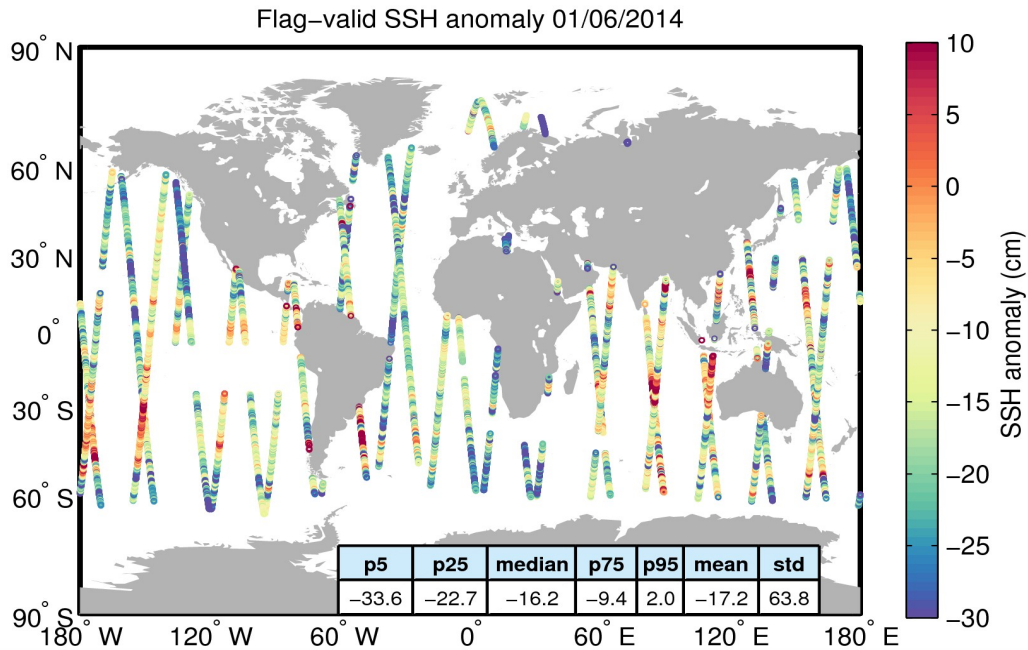
Figure 5. Geographical distribution of flag-valid 1-Hz SSH anomaly data over oceans and lakes for 01/06/2014. The statistical values shown in the table refer to the SSH anomaly in cm and are calculated over all measurements shown in the figure.
