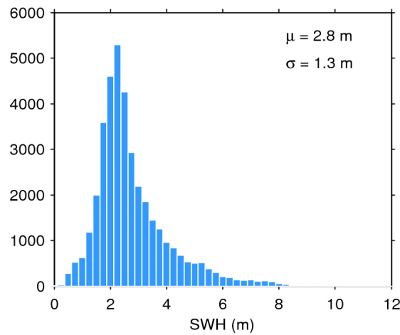
Figure 17. Histogram of flag-valid SWH over oceans and lakes for 01/06/2014. The mean ( \mu ) and standard deviation ( \sigma ) are also shown. Note that values larger than 12 m are excluded from the histogram for the sake of readability but not from the computation of \mu and \sigma .
