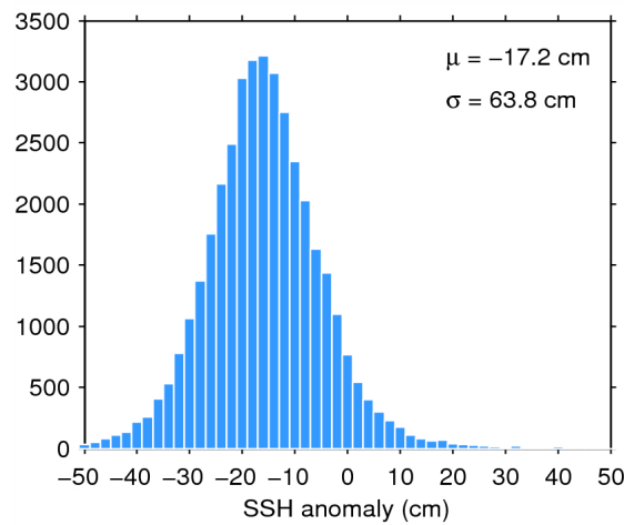
Figure 7. Histogram of flag-valid SSH anomaly over oceans and lakes for 01/06/2014. The mean ( \mu ) and standard deviation ( \sigma ) are also shown. Note that values outside [-50\ 50] cm are excluded from the histogram for the sake of readability but not from the computation of \mu and \sigma .
