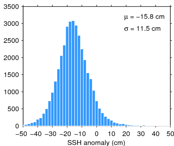
Figure 11. Histogram of science-valid SSH anomaly over oceans and lakes for 01/06/2014. The mean ( \mu ) and standard deviation ( \sigma ) are also shown. Note that values outside [-50 50] cm are excluded from the histogram for the sake of readability but not from the computation of \mu and \sigma .
