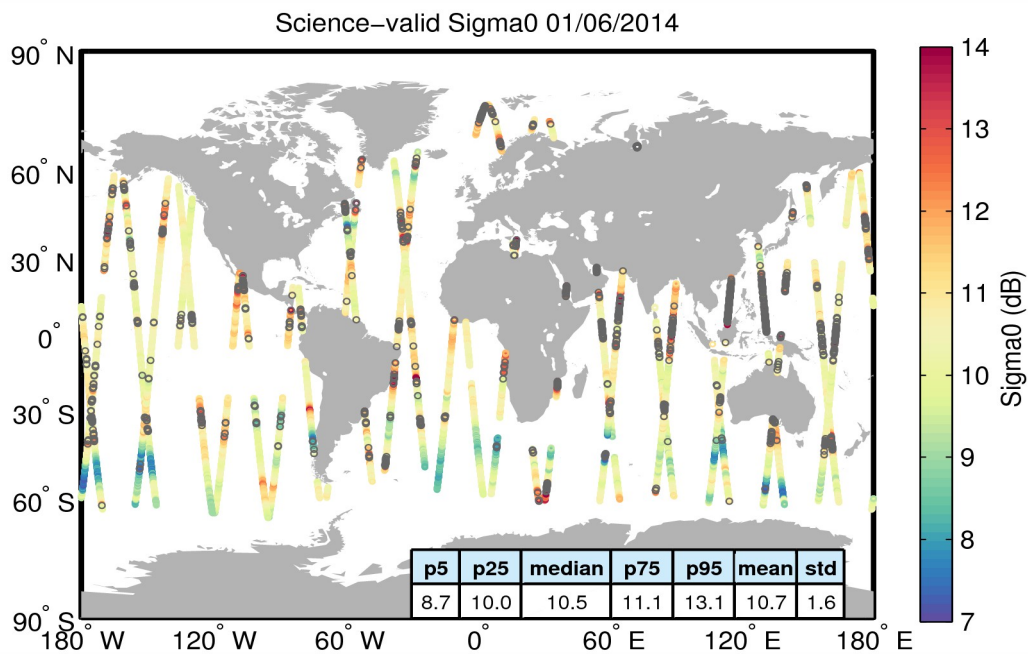
Figure 27. Geographical distribution of science-valid sigma0 data over oceans and lakes for 01/06/2014. The statistical values shown in the table refer to the sigma0 in dB and are calculated over all measurements shown in the figure. Gray circles denote records that have been rejected based on the editing criteria described in Table 4.
