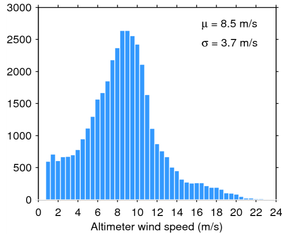
Figure 33. Histogram of flag-valid wind over oceans and lakes for 01/06/2014. The mean ( \mu ) and standard deviation ( \sigma ) are also shown. Note that values larger than 24 m/s are excluded from the histogram for the sake of readability but not from the computation of \mu and \sigma .
