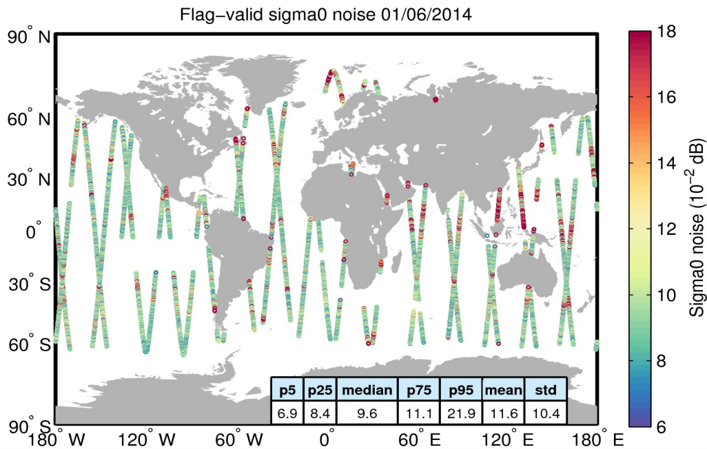
Figure 26. Geographical distribution of flag-valid 20-Hz sigma0 measurement noise over oceans and lakes for 01/06/2014. The statistical values shown in the table refer to the sigma0 noise and are calculated over all measurements shown in the figure.
