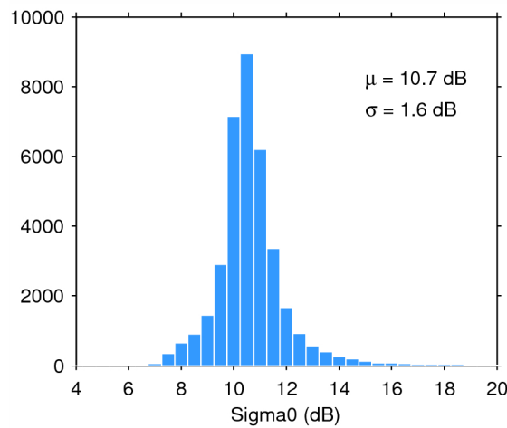
Figure 28. Histogram of science-valid sigma0 over oceans and lakes for 01/06/2014. The mean ( \mu ) and standard deviation ( \sigma ) are also shown. Note that values outside [4 20] dB are excluded from the histogram for the sake of readability but not from the computation of \mu and \sigma .
