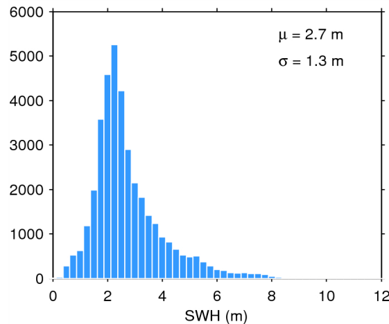
Figure 20. Histogram of science-valid SWH over oceans and lakes for 01/06/2014. The mean ( \mu ) and standard deviation ( \sigma ) are also shown. Note that values larger than 12 m are excluded from the histogram for the sake of readability but not from the computation of \mu and \sigma .
