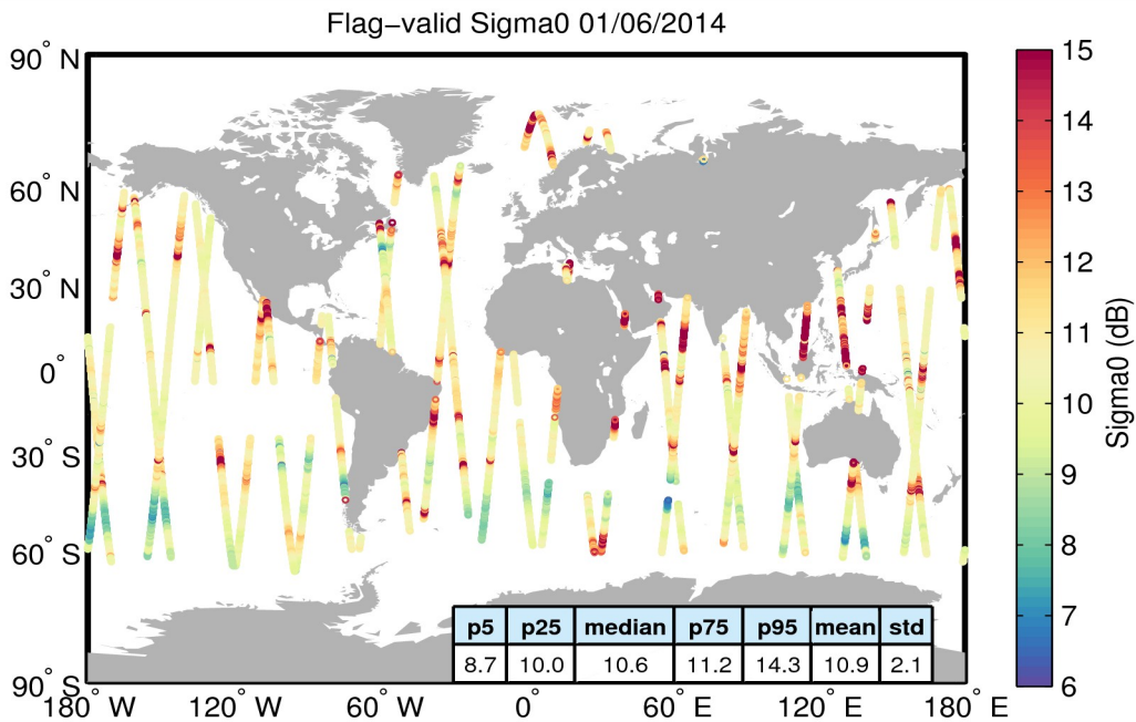
Figure 23. Geographical distribution of flag-valid sigma0 data over oceans and lakes for 01/06/2014. The statistical values shown in the table refer to the sigma0 in dB and are calculated over all measurements shown in the figure.
