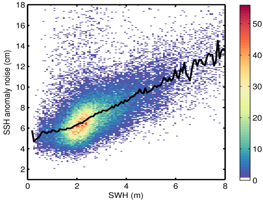
Figure 9. 2D histogram showing flag-valid SSH anomaly noise as a function of SWH for 01/06/2014. The black line denotes the median SSH anomaly as a function of SWH.
