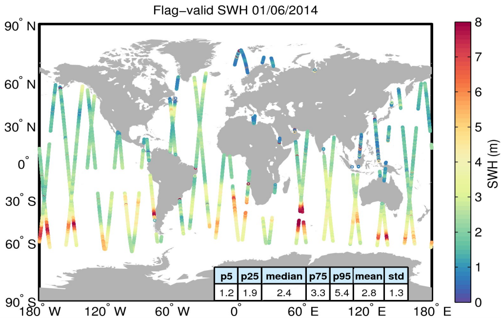
Figure 15. Geographical distribution of flag-valid SWH data over oceans and lakes for 01/06/2014. The statistical values shown in the figure refer to the SWH in m and are calculated over all measurements shown in the figure.
