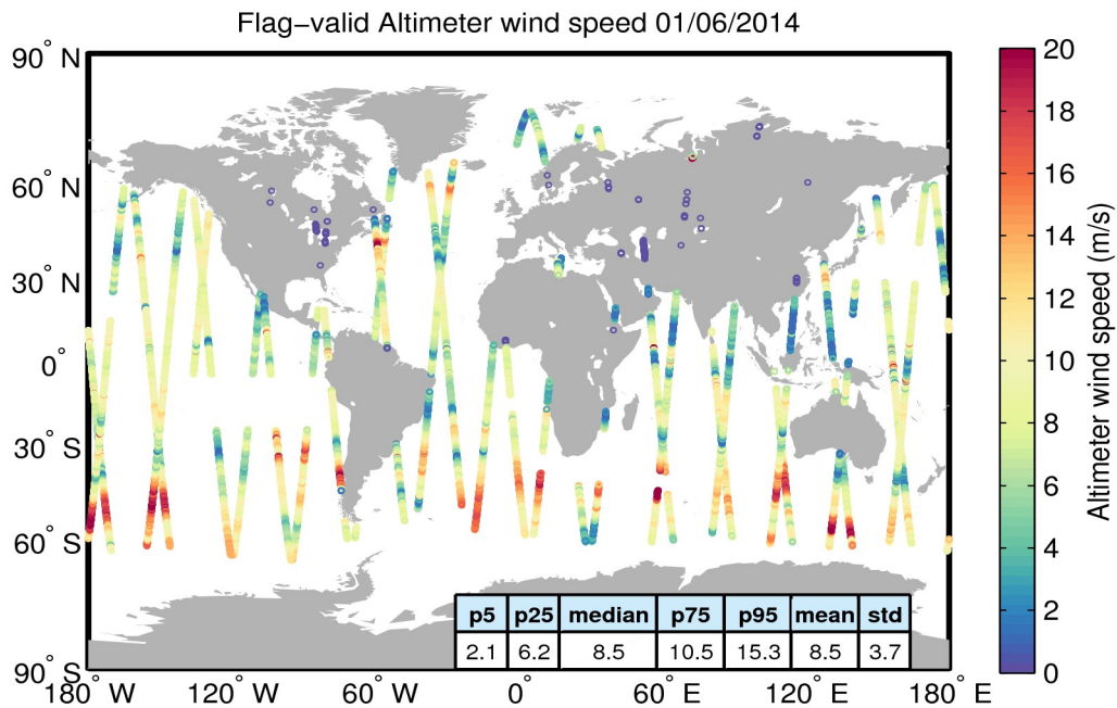
Figure 31. Geographical distribution of flag-valid wind data over oceans and lakes for 01/06/2014. The statistical values shown in the table refer to the wind in m/s and are calculated over all measurements shown in the figure.
