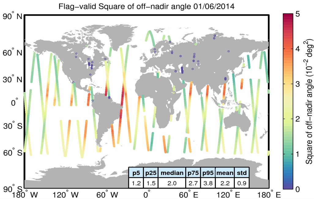
Figure 37. Geographical distribution of flag-valid mispointing data over oceans and lakes for 01/06/2014. The statistical values shown in the table refer to the mispointing in 10^{-2} \text{deg}^2 and are calculated over all measurements shown in the figure.
