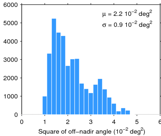
Figure 39. Histogram of flag-valid mispointing over oceans and lakes for 01/06/2014. The mean ( \mu ) and standard deviation ( \sigma ) are also shown. Note that values than 6 \cdot 10^{-2} \text{ deg}^2 are excluded from the histogram for the sake of readability but not from the computation of \mu and \sigma .
