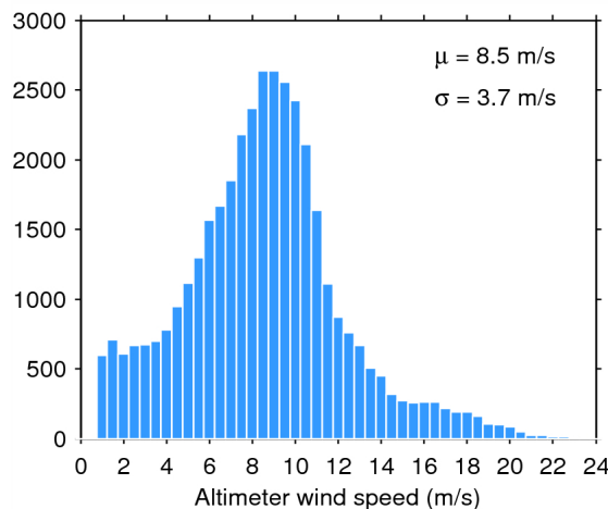
Figure 35. Histogram of science-valid wind over oceans and lakes for 01/06/2014. The mean ( \mu ) and standard deviation ( \sigma ) are also shown. Note that values larger than 24 m/s are excluded from the histogram for the sake of readability but not from the computation of \mu and \sigma .
