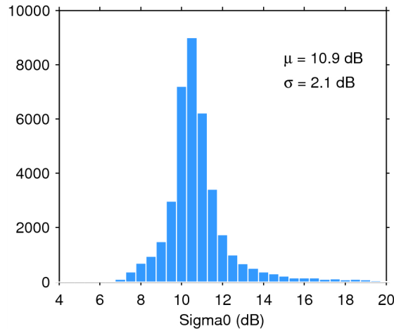
Figure 25. Histogram of flag-valid sigma0 over oceans and lakes for 01/06/2014. The mean ( \mu ) and standard deviation ( \sigma ) are also shown. Note that values outside [4 20] dB are excluded from the histogram for the sake of readability but not from the computation of \mu and \sigma .
