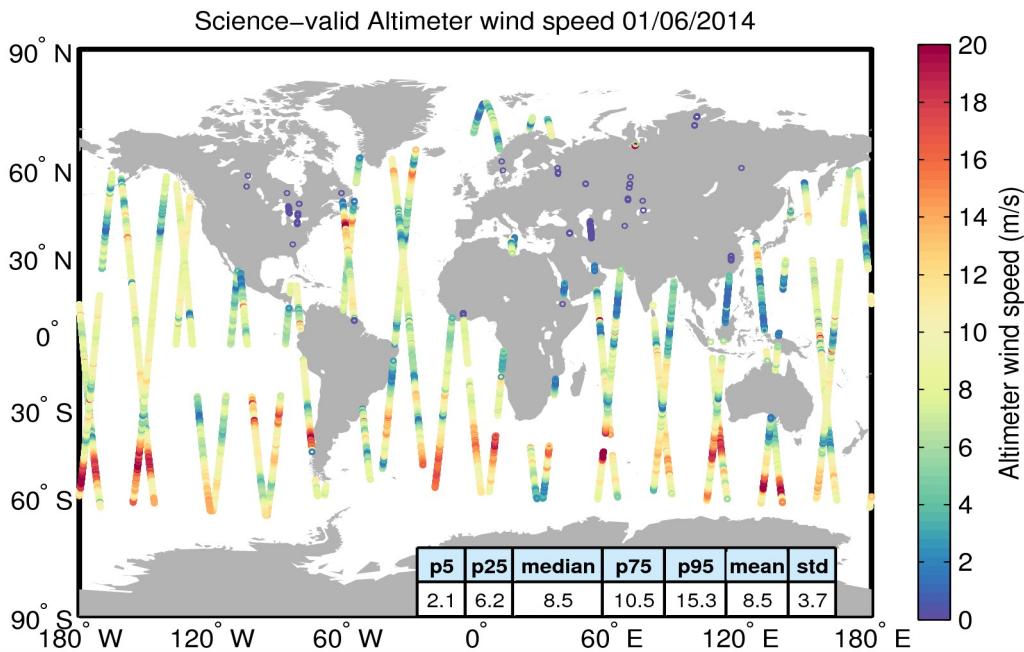
Figure 34. Geographical distribution of science-valid wind data over oceans and lakes for 01/06/2014. The statistical values shown in the table refer to the wind in m/s and are calculated over all measurements shown in the figure. Gray circles denote records that have been rejected based on the editing criteria described in Table 5.
