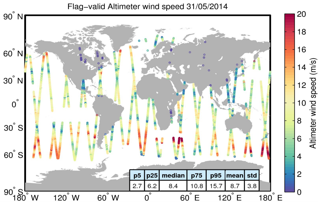
Figure 31. Geographical distribution of flag-valid wind data over oceans and lakes for 31/05/2014. The statistical values shown in the table refer to the wind in m/s and are calculated over all measurements shown in the figure.
