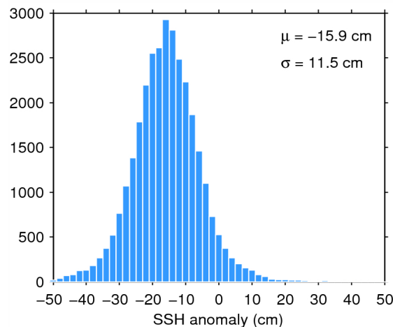
Figure 11. Histogram of science-valid SSH anomaly over oceans and lakes for 31/05/2014. The mean ( \mu ) and standard deviation ( \sigma ) are also shown. Note that values outside [-50 50] cm are excluded from the histogram for the sake of readability but not from the computation of \mu and \sigma .
