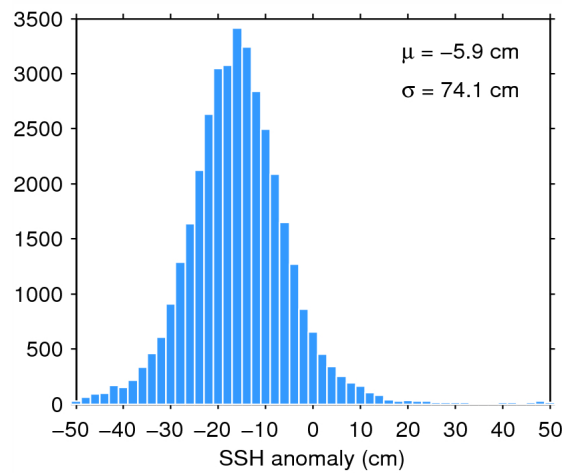
Figure 7. Histogram of flag-valid SSH anomaly over oceans and lakes for 31/05/2014. The mean ( \mu ) and standard deviation ( \sigma ) are also shown. Note that values outside [-50 50] cm are excluded from the histogram for the sake of readability but not from the computation of \mu and \sigma .
