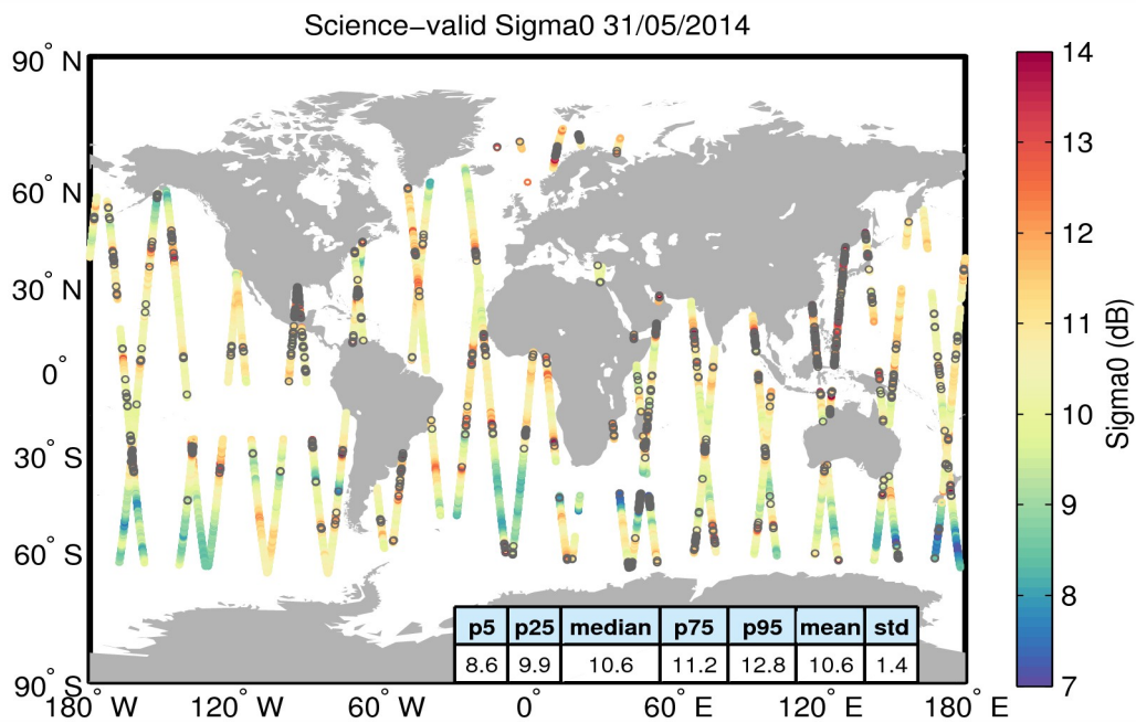
Figure 27. Geographical distribution of science-valid sigma0 data over oceans and lakes for 31/05/2014. The statistical values shown in the table refer to the sigma0 in dB and are calculated over all measurements shown in the figure. Gray circles denote records that have been rejected based on the editing criteria described in Table 4.
