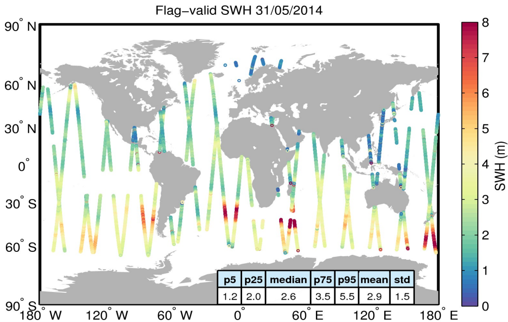
Figure 15. Geographical distribution of flag-valid SWH data over oceans and lakes for 31/05/2014. The statistical values shown in the table refer to the SWH in m and are calculated over all measurements shown in the figure.
