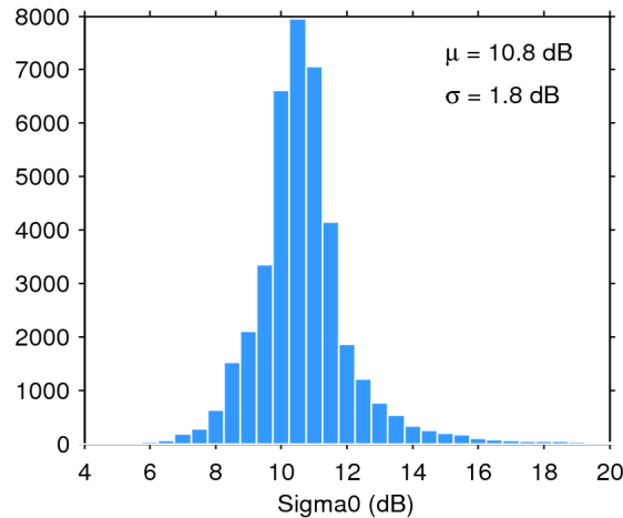
Figure 25. Histogram of flag-valid sigma0 over oceans and lakes for 31/05/2014. The mean ( \mu ) and standard deviation ( \sigma ) are also shown. Note that values outside [4 20] dB are excluded from the histogram for the sake of readability but not from the computation of \mu and \sigma .
