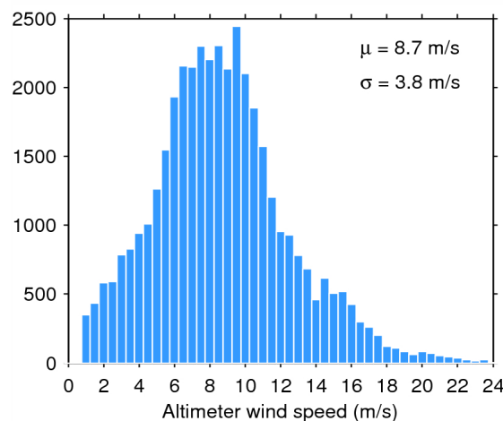
Figure 35. Histogram of science-valid wind over oceans and lakes for 31/05/2014. The mean ( \mu ) and standard deviation ( \sigma ) are also shown. Note that values larger than 24 m/s are excluded from the histogram for the sake of readability but not from the computation of \mu and \sigma .
