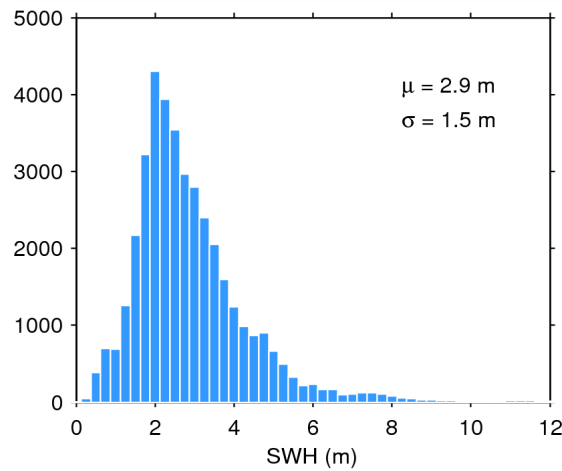
Figure 17. Histogram of flag-valid SWH over oceans and lakes for 31/05/2014. The mean ( \mu ) and standard deviation ( \sigma ) are also shown. Note that values larger than 12 m are excluded from the histogram for the sake of readability but not from the computation of \mu and \sigma .
