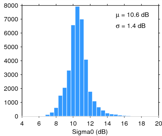
Figure 28. Histogram of science-valid sigma0 over oceans and lakes for 31/05/2014. The mean ( \mu ) and standard deviation ( \sigma ) are also shown. Note that values outside [4 20] dB are excluded from the histogram for the sake of readability but not from the computation of \mu and \sigma .
