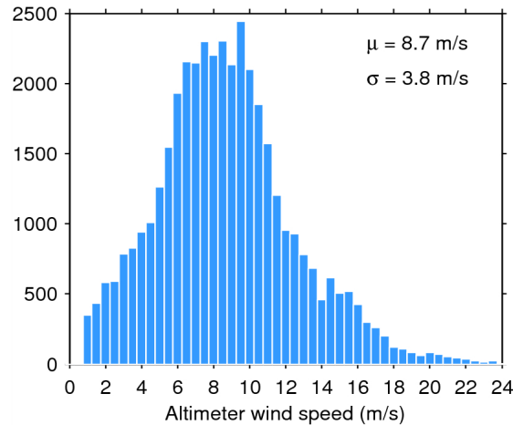
Figure 33. Histogram of flag-valid wind over oceans and lakes for 31/05/2014. The mean ( \mu ) and standard deviation ( \sigma ) are also shown. Note that values larger than 24 m/s are excluded from the histogram for the sake of readability but not from the computation of \mu and \sigma .
