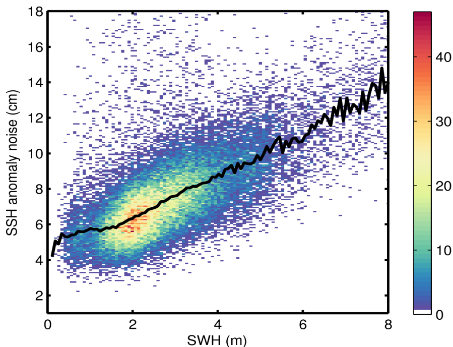
Figure 9. 2D histogram showing flag-valid SSH anomaly noise as a function of SWH for 31/05/2014. The black line denotes the median SSH anomaly as a function of SWH.
