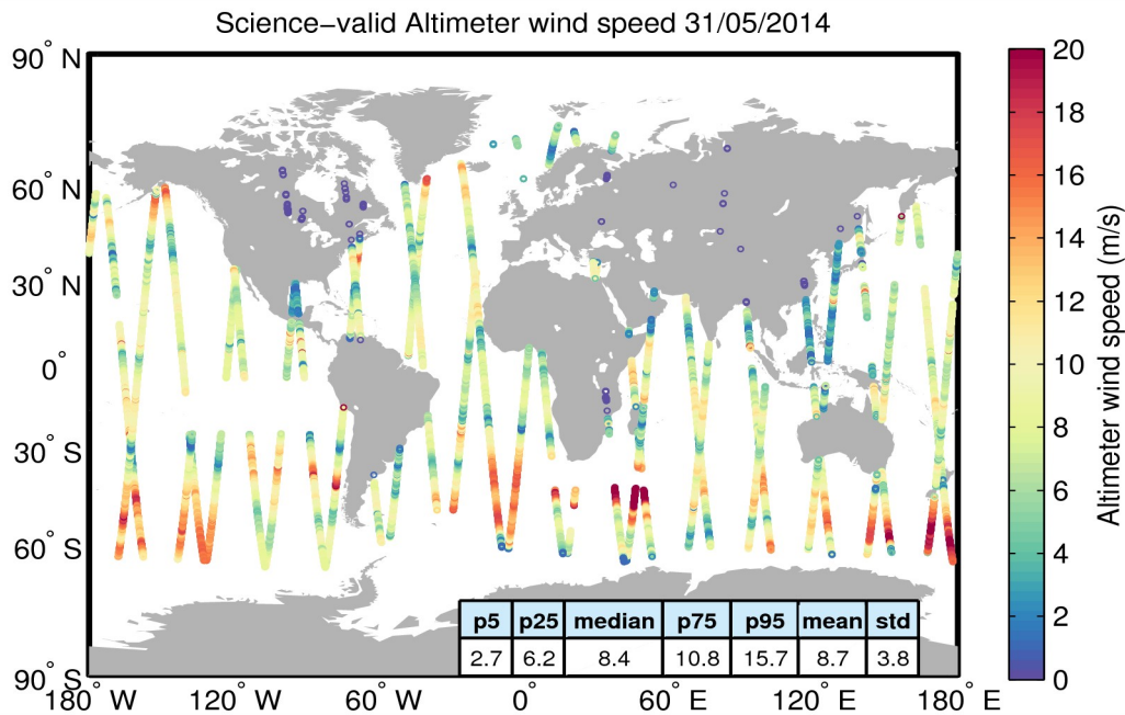
Figure 34. Geographical distribution of science-valid wind data over oceans and lakes for 31/05/2014. The statistical values shown in the table refer to the wind in m/s and are calculated over all measurements shown in the figure. Gray circles denote records that have been rejected based on the editing criteria described in Table 5.
