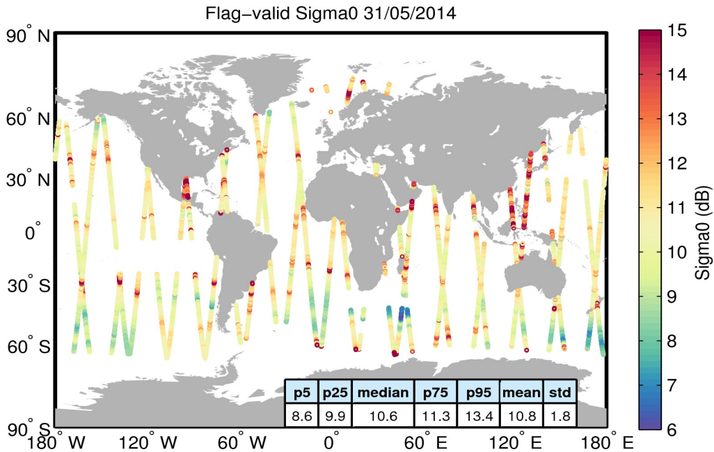
Figure 23. Geographical distribution of flag-valid sigma0 data over oceans and lakes for 31/05/2014. The statistical values shown in the table refer to the sigma0 in dB and are calculated over all measurements shown in the figure.
