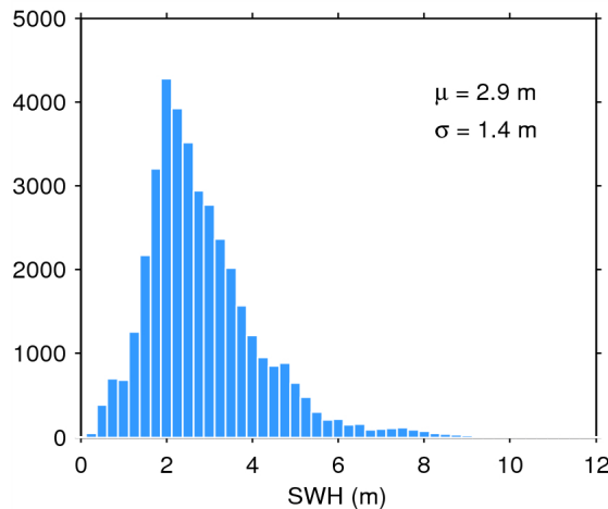
Figure 20. Histogram of science-valid SWH over oceans and lakes for 31/05/2014. The mean ( \mu ) and standard deviation ( \sigma ) are also shown. Note that values larger than 12 m are excluded from the histogram for the sake of readability but not from the computation of \mu and \sigma .
