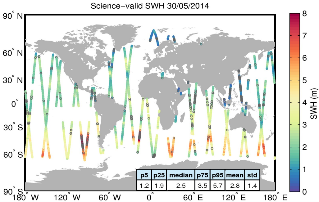
Figure 19. Geographical distribution of science-valid SWH data over oceans and lakes for 30/05/2014. The statistical values shown in the table refer to the SWH in m and are calculated over all measurements shown in the figure. Gray circles denote records that have been rejected based on the editing criteria described in Table 3.
