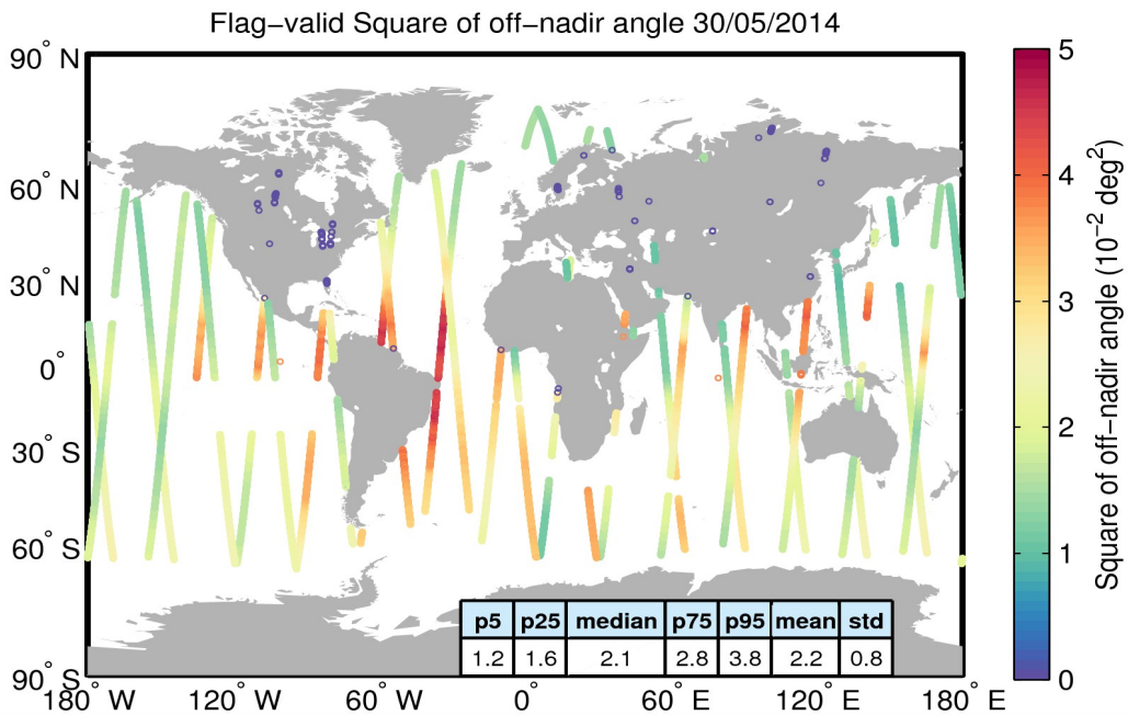
Figure 37. Geographical distribution of flag-valid mispointing data over oceans and lakes for 30/05/2014. The statistical values shown in the table refer to the mispointing in 10^{-2} \text{ deg}^2 and are calculated over all measurements shown in the figure.
