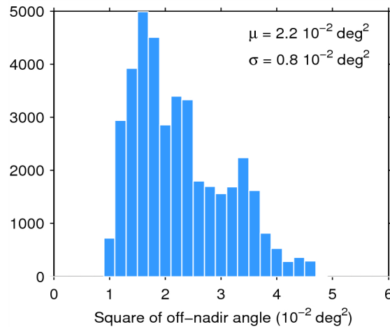
Figure 39. Histogram of flag-valid mispointing over oceans and lakes for 30/05/2014. The mean ( \mu ) and standard deviation ( \sigma ) are also shown. Note that values than 6 \cdot 10^{-2} \text{ deg}^2 are excluded from the histogram for the sake of readability but not from the computation of \mu and \sigma .
