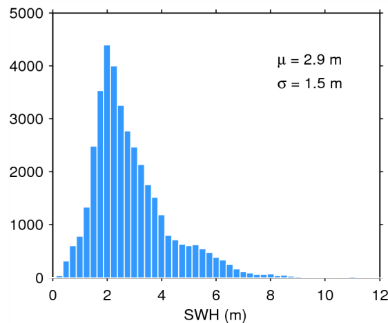
Figure 17. Histogram of flag-valid SWH over oceans and lakes for 30/05/2014. The mean ( \mu ) and standard deviation ( \sigma ) are also shown. Note that values larger than 12 m are excluded from the histogram for the sake of readability but not from the computation of \mu and \sigma .
