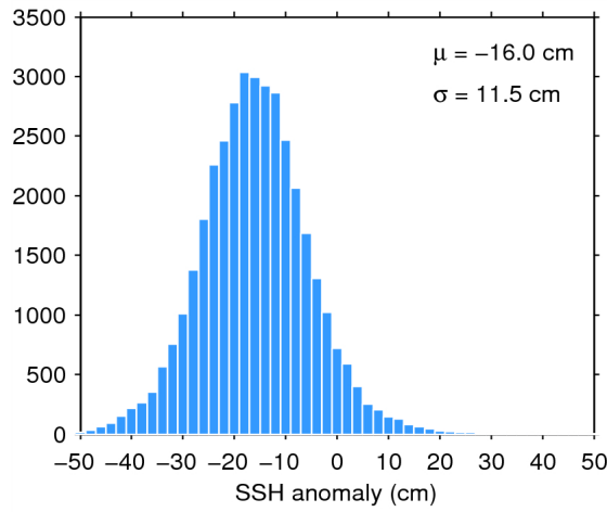
Figure 11. Histogram of science-valid SSH anomaly over oceans and lakes for 30/05/2014. The mean ( \mu ) and standard deviation ( \sigma ) are also shown. Note that values outside [-50 50] cm are excluded from the histogram for the sake of readability but not from the computation of \mu and \sigma .
