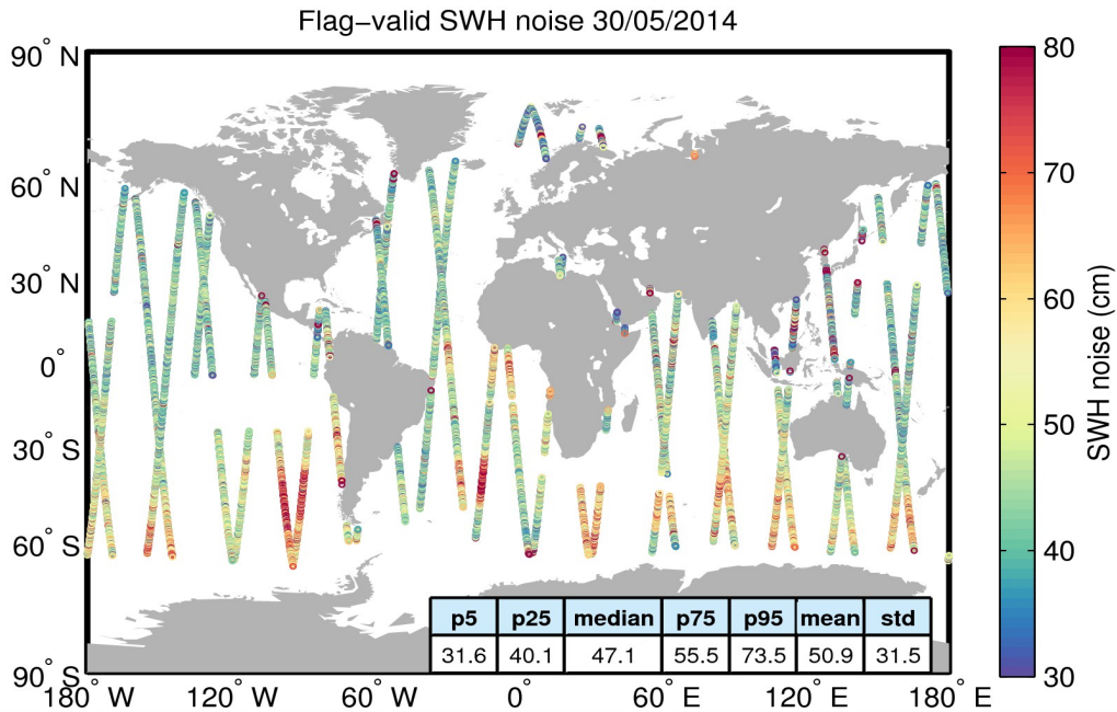
Figure 18. Geographical distribution of flag-valid 20-Hz SWH measurement noise over oceans and lakes for 30/05/2014. The statistical values shown in the figure refer to the SWH noise and are calculated over all measurements shown in the figure.
