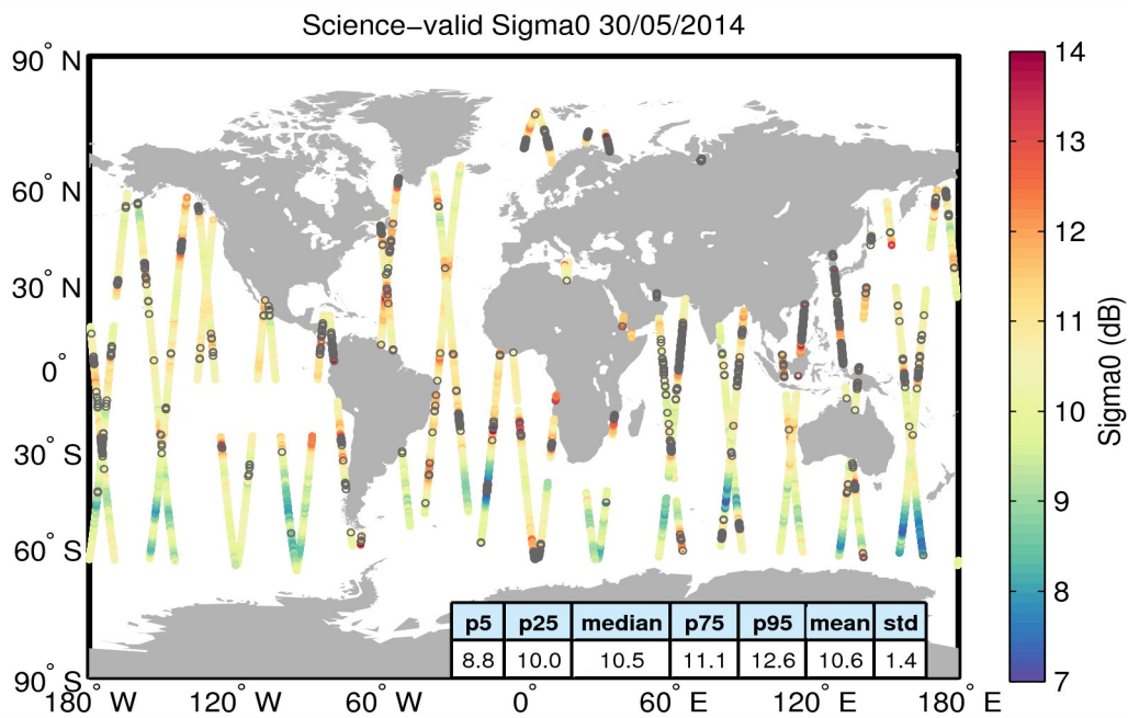
Figure 27. Geographical distribution of science-valid sigma0 data over oceans and lakes for 30/05/2014. The statistical values shown in the table refer to the sigma0 in dB and are calculated over all measurements shown in the figure. Gray circles denote records that have been rejected based on the editing criteria described in Table 4.
