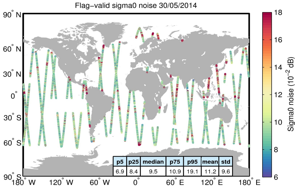
Figure 26. Geographical distribution of flag-valid 20-Hz sigma0 measurement noise over oceans and lakes for 30/05/2014. The statistical values shown in the table refer to the sigma0 noise and are calculated over all measurements shown in the figure.
