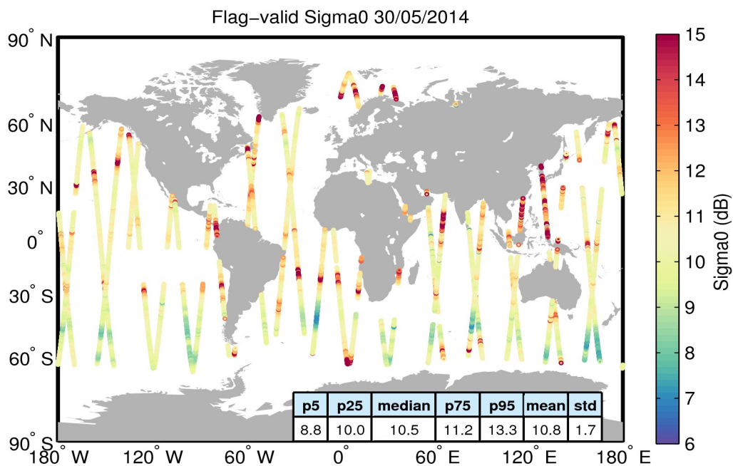
Figure 23. Geographical distribution of flag-valid sigma0 data over oceans and lakes for 30/05/2014. The statistical values shown in the table refer to the sigma0 in dB and are calculated over all measurements shown in the figure.
