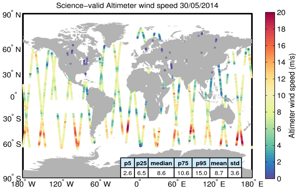
Figure 34. Geographical distribution of science-valid wind data over oceans and lakes for 30/05/2014. The statistical values shown in the table refer to the wind in m/s and are calculated over all measurements shown in the figure. Gray circles denote records that have been rejected based on the editing criteria described in Table 5.
