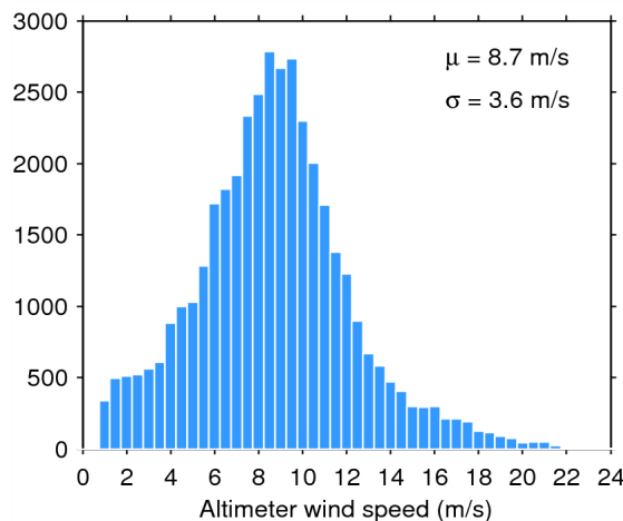
Figure 35. Histogram of science-valid wind over oceans and lakes for 30/05/2014. The mean ( \mu ) and standard deviation ( \sigma ) are also shown. Note that values larger than 24 m/s are excluded from the histogram for the sake of readability but not from the computation of \mu and \sigma .
