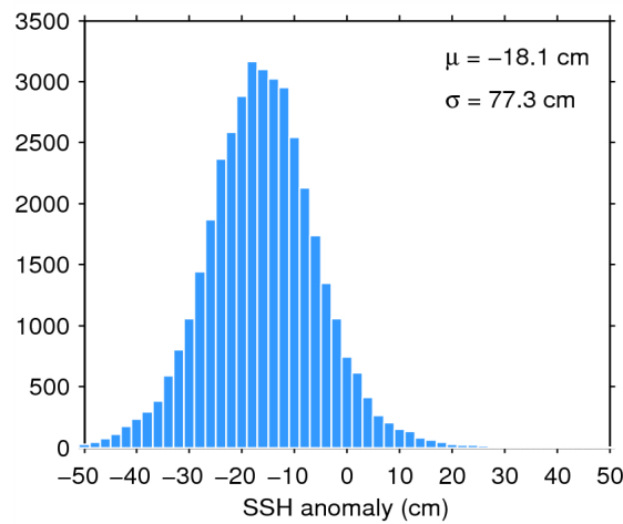
Figure 7. Histogram of flag-valid SSH anomaly over oceans and lakes for 30/05/2014. The mean ( \mu ) and standard deviation ( \sigma ) are also shown. Note that values outside [-50\ 50] cm are excluded from the histogram for the sake of readability but not from the computation of \mu and \sigma .
