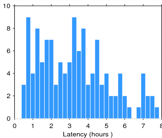
Figure 2. Histogram of the data latency for 30/05/2014. The y-axis denotes the number of files that are made available with a delay of x-hours with respect to the mean time of the records stored in the file.
