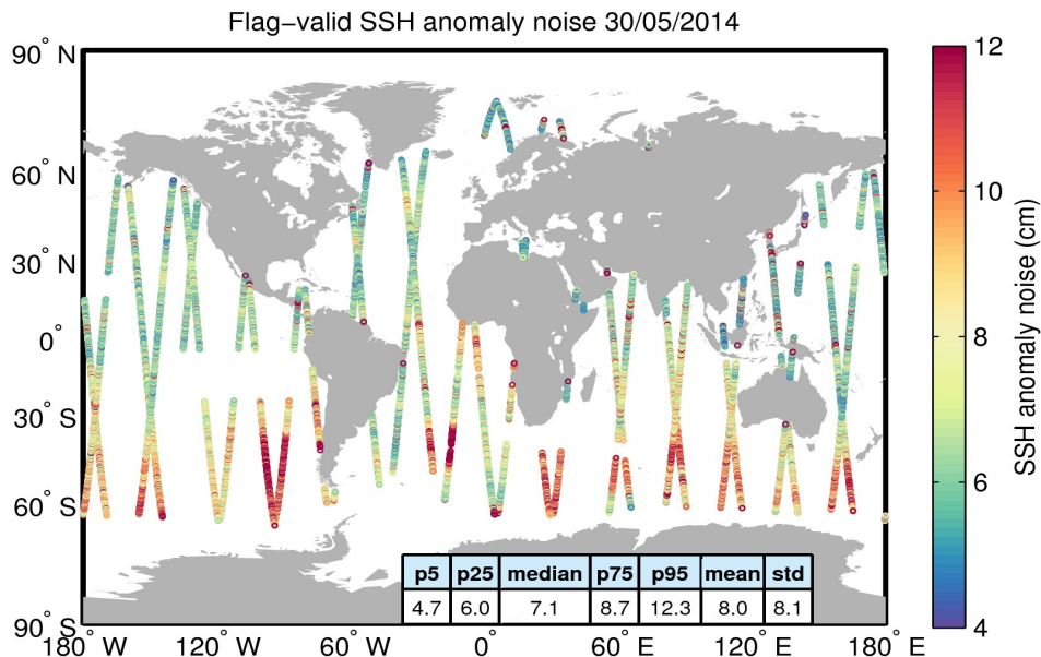
Figure 8. Geographical distribution of flag-valid 20-Hz SSH anomaly measurement noise over oceans and lakes for 30/05/2014. The statistical values shown in the table refer to the SSH anomaly noise and are calculated over all measurements shown in the figure.
