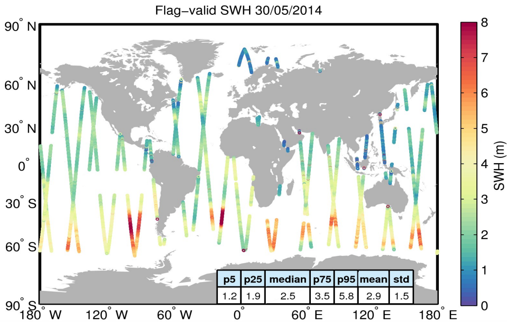
Figure 15. Geographical distribution of flag-valid SWH data over oceans and lakes for 30/05/2014. The statistical values shown in the table refer to the SWH in m and are calculated over all measurements shown in the figure.
