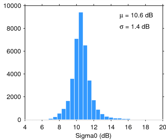
Figure 28. Histogram of science-valid sigma0 over oceans and lakes for 30/05/2014. The mean ( \mu ) and standard deviation ( \sigma ) are also shown. Note that values outside [4 20] dB are excluded from the histogram for the sake of readability but not from the computation of \mu and \sigma .
