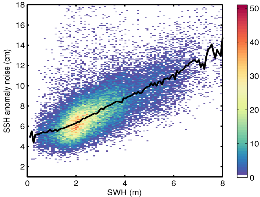
Figure 9. 2D histogram showing flag-valid SSH anomaly noise as a function of SWH for 30/05/2014. The black line denotes the median SSH anomaly as a function of SWH.
