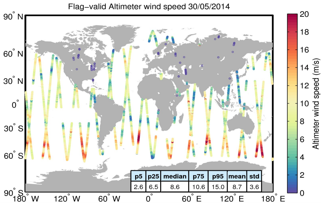
Figure 31. Geographical distribution of flag-valid wind data over oceans and lakes for 30/05/2014. The statistical values shown in the table refer to the wind in m/s and are calculated over all measurements shown in the figure.
