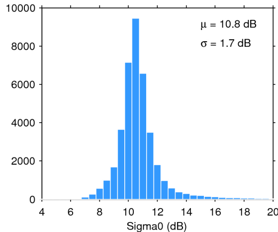
Figure 25. Histogram of flag-valid sigma0 over oceans and lakes for 30/05/2014. The mean ( \mu ) and standard deviation ( \sigma ) are also shown. Note that values outside [4 20] dB are excluded from the histogram for the sake of readability but not from the computation of \mu and \sigma .
