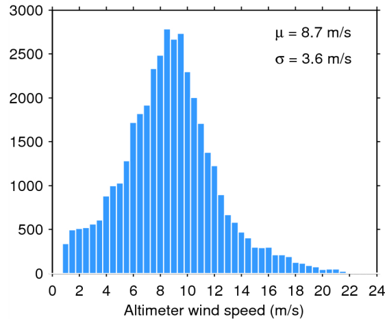
Figure 33. Histogram of flag-valid wind over oceans and lakes for 30/05/2014. The mean ( \mu ) and standard deviation ( \sigma ) are also shown. Note that values larger than 24 m/s are excluded from the histogram for the sake of readability but not from the computation of \mu and \sigma .
