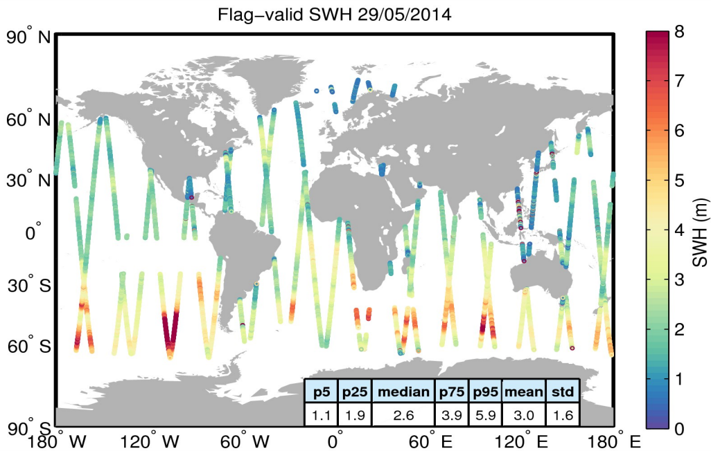
Figure 15. Geographical distribution of flag-valid SWH data over oceans and lakes for 29/05/2014. The statistical values shown in the figure refer to the SWH in m and are calculated over all measurements shown in the figure.
