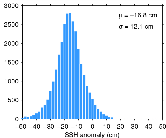
Figure 11. Histogram of science-valid SSH anomaly over oceans and lakes for 29/05/2014. The mean ( \mu ) and standard deviation ( \sigma ) are also shown. Note that values outside [-50 50] cm are excluded from the histogram for the sake of readability but not from the computation of \mu and \sigma .
