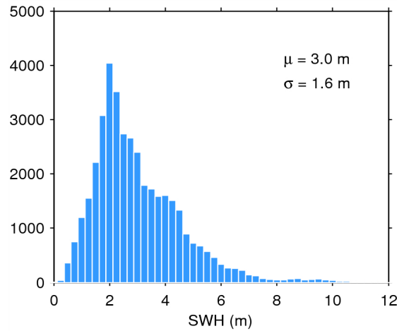
Figure 17. Histogram of flag-valid SWH over oceans and lakes for 29/05/2014. The mean ( \mu ) and standard deviation ( \sigma ) are also shown. Note that values larger than 12 m are excluded from the histogram for the sake of readability but not from the computation of \mu and \sigma .
