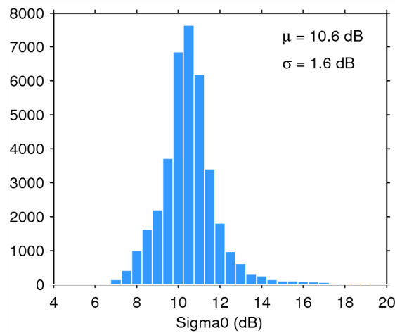
Figure 28. Histogram of science-valid sigma0 over oceans and lakes for 29/05/2014. The mean ( \mu ) and standard deviation ( \sigma ) are also shown. Note that values outside [4 20] dB are excluded from the histogram for the sake of readability but not from the computation of \mu and \sigma .
