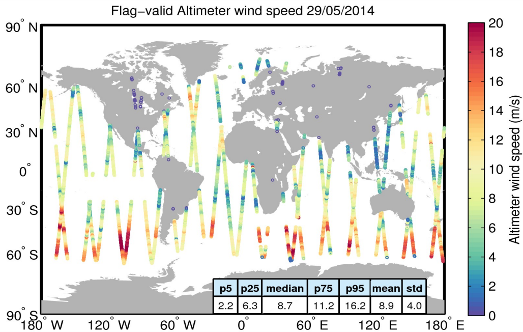
Figure 31. Geographical distribution of flag-valid wind data over oceans and lakes for 29/05/2014. The statistical values shown in the table refer to the wind in m/s and are calculated over all measurements shown in the figure.
