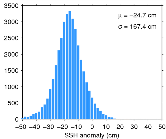
Figure 7. Histogram of flag-valid SSH anomaly over oceans and lakes for 29/05/2014. The mean ( \mu ) and standard deviation ( \sigma ) are also shown. Note that values outside [-50 50] cm are excluded from the histogram for the sake of readability but not from the computation of \mu and \sigma .
