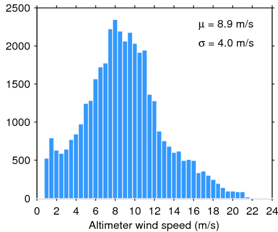
Figure 35. Histogram of science-valid wind over oceans and lakes for 29/05/2014. The mean ( \mu ) and standard deviation ( \sigma ) are also shown. Note that values larger than 24 m/s are excluded from the histogram for the sake of readability but not from the computation of \mu and \sigma .
