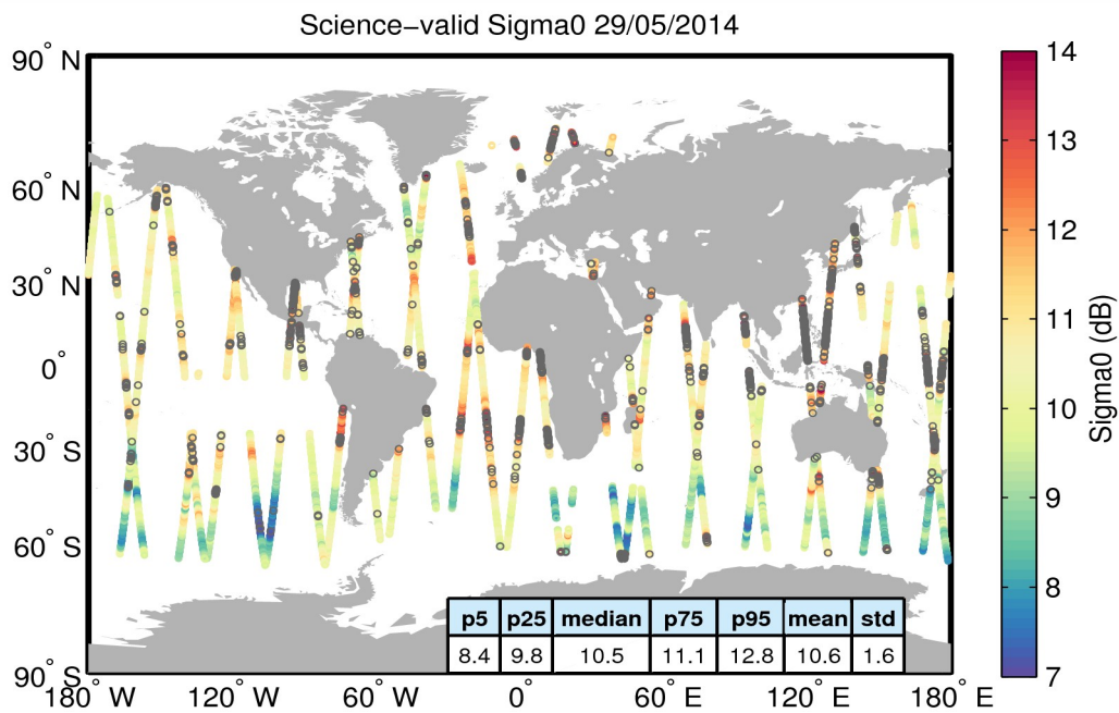
Figure 27. Geographical distribution of science-valid sigma0 data over oceans and lakes for 29/05/2014. The statistical values shown in the table refer to the sigma0 in dB and are calculated over all measurements shown in the figure. Gray circles denote records that have been rejected based on the editing criteria described in Table 4.
