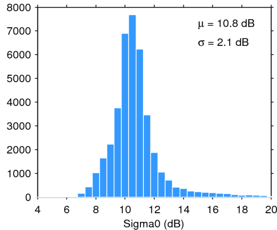
Figure 25. Histogram of flag-valid sigma0 over oceans and lakes for 29/05/2014. The mean ( \mu ) and standard deviation ( \sigma ) are also shown. Note that values outside [4 20] dB are excluded from the histogram for the sake of readability but not from the computation of \mu and \sigma .
