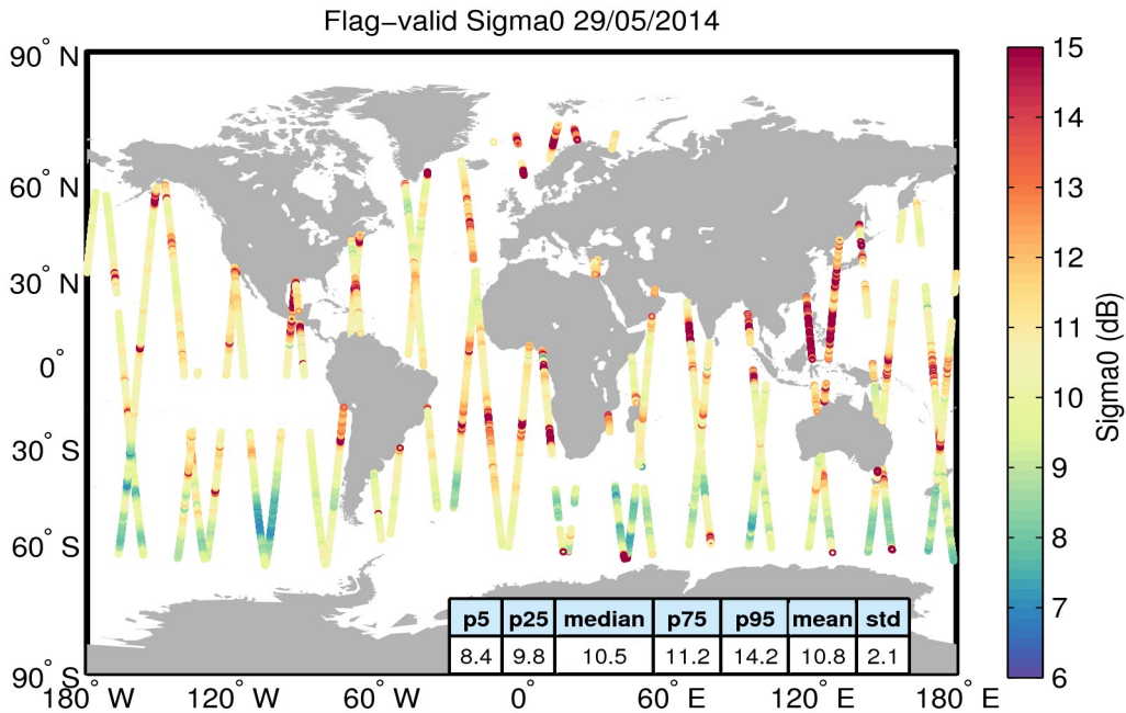
Figure 23. Geographical distribution of flag-valid sigma0 data over oceans and lakes for 29/05/2014. The statistical values shown in the table refer to the sigma0 in dB and are calculated over all measurements shown in the figure.
