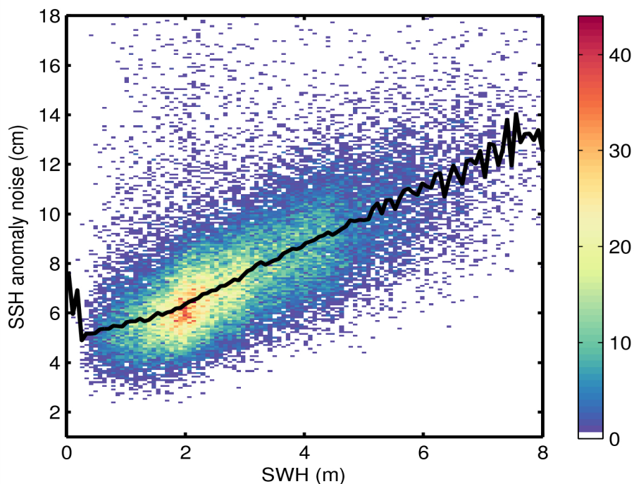
Figure 9. 2D histogram showing flag-valid SSH anomaly noise as a function of SWH for 29/05/2014. The black line denotes the median SSH anomaly as a function of SWH.
