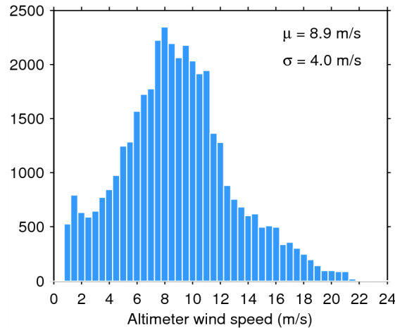
Figure 33. Histogram of flag-valid wind over oceans and lakes for 29/05/2014. The mean ( \mu ) and standard deviation ( \sigma ) are also shown. Note that values larger than 24 m/s are excluded from the histogram for the sake of readability but not from the computation of \mu and \sigma .
