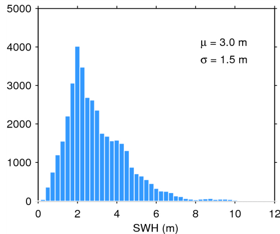
Figure 20. Histogram of science-valid SWH over oceans and lakes for 29/05/2014. The mean ( \mu ) and standard deviation ( \sigma ) are also shown. Note that values larger than 12 m are excluded from the histogram for the sake of readability but not from the computation of \mu and \sigma .
