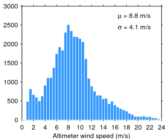
Figure 35. Histogram of science-valid wind over oceans and lakes for 28/05/2014. The mean ( \mu ) and standard deviation ( \sigma ) are also shown. Note that values larger than 24 m/s are excluded from the histogram for the sake of readability but not from the computation of \mu and \sigma .
