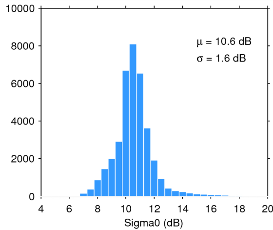
Figure 28. Histogram of science-valid sigma0 over oceans and lakes for 28/05/2014. The mean ( \mu ) and standard deviation ( \sigma ) are also shown. Note that values outside [4 20] dB are excluded from the histogram for the sake of readability but not from the computation of \mu and \sigma .
