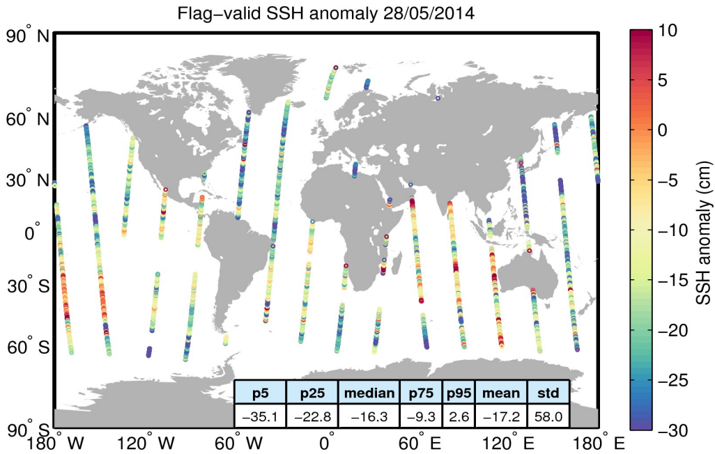
Figure 5. Geographical distribution of flag-valid 1-Hz SSH anomaly data over oceans and lakes for 28/05/2014. The statistical values shown in the table refer to the SSH anomaly in cm and are calculated over all measurements shown in the figure.
