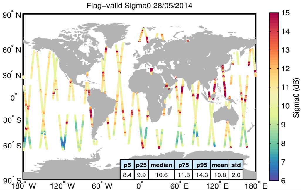
Figure 23. Geographical distribution of flag-valid sigma0 data over oceans and lakes for 28/05/2014. The statistical values shown in the table refer to the sigma0 in dB and are calculated over all measurements shown in the figure.
