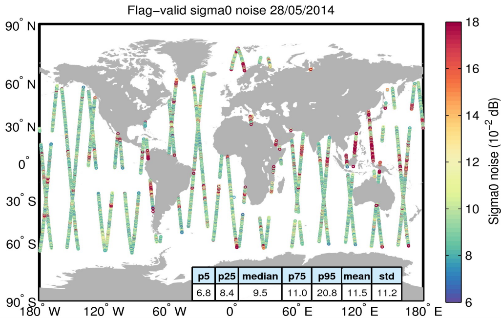
Figure 26. Geographical distribution of flag-valid 20-Hz sigma0 measurement noise over oceans and lakes for 28/05/2014. The statistical values shown in the table refer to the sigma0 noise and are calculated over all measurements shown in the figure.
