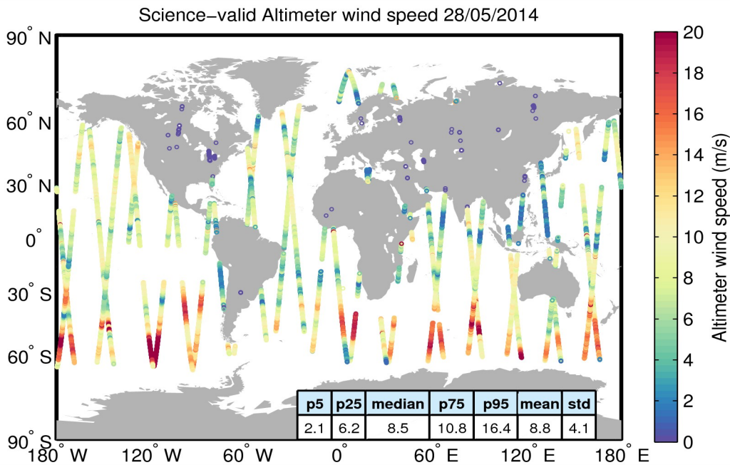
Figure 34. Geographical distribution of science-valid wind data over oceans and lakes for 28/05/2014. The statistical values shown in the table refer to the wind in m/s and are calculated over all measurements shown in the figure. Gray circles denote records that have been rejected based on the editing criteria described in Table 5.
