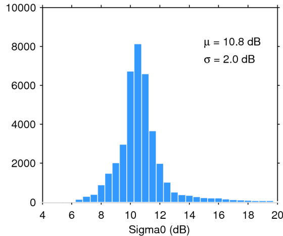
Figure 25. Histogram of flag-valid sigma0 over oceans and lakes for 28/05/2014. The mean ( \mu ) and standard deviation ( \sigma ) are also shown. Note that values outside [4 20] dB are excluded from the histogram for the sake of readability but not from the computation of \mu and \sigma .
