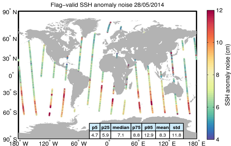
Figure 8. Geographical distribution of flag-valid 20-Hz SSH anomaly measurement noise over oceans and lakes for 28/05/2014. The statistical values shown in the table refer to the SSH anomaly noise and are calculated over all measurements shown in the figure.
