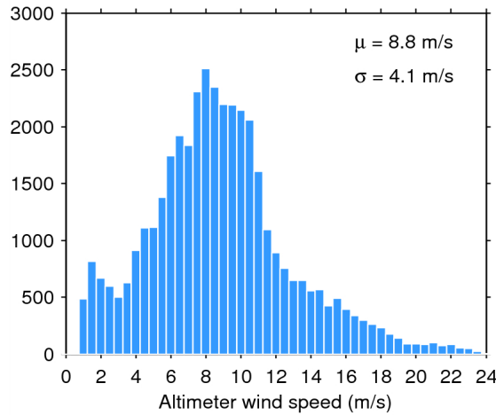
Figure 33. Histogram of flag-valid wind over oceans and lakes for 28/05/2014. The mean ( \mu ) and standard deviation ( \sigma ) are also shown. Note that values larger than 24 m/s are excluded from the histogram for the sake of readability but not from the computation of \mu and \sigma .
