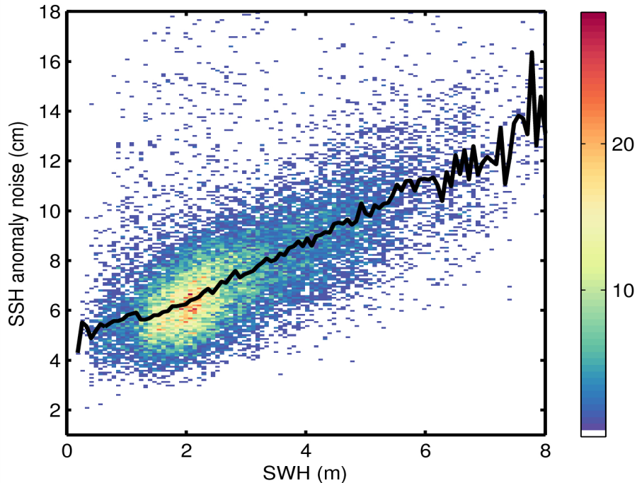
Figure 9. 2D histogram showing flag-valid SSH anomaly noise as a function of SWH for 28/05/2014. The black line denotes the median SSH anomaly as a function of SWH.
