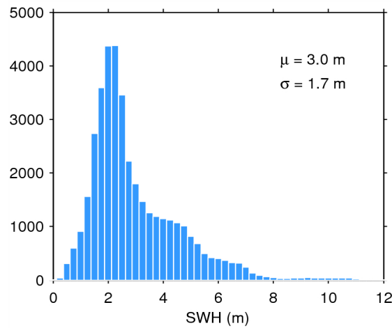
Figure 17. Histogram of flag-valid SWH over oceans and lakes for 28/05/2014. The mean ( \mu ) and standard deviation ( \sigma ) are also shown. Note that values larger than 12 m are excluded from the histogram for the sake of readability but not from the computation of \mu and \sigma .
