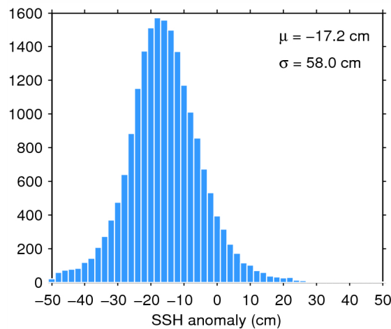
Figure 7. Histogram of flag-valid SSH anomaly over oceans and lakes for 28/05/2014. The mean ( \mu ) and standard deviation ( \sigma ) are also shown. Note that values outside [-50\ 50] cm are excluded from the histogram for the sake of readability but not from the computation of \mu and \sigma .
