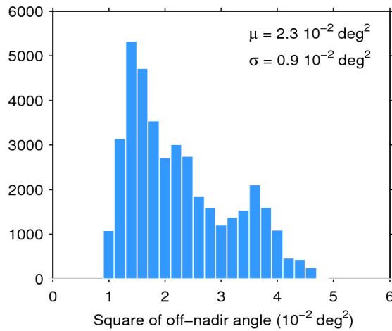
Figure 39. Histogram of flag-valid mispointing over oceans and lakes for 28/05/2014. The mean ( \mu ) and standard deviation ( \sigma ) are also shown. Note that values than 6 \cdot 10^{-2} \text{ deg}^2 are excluded from the histogram for the sake of readability but not from the computation of \mu and \sigma .
