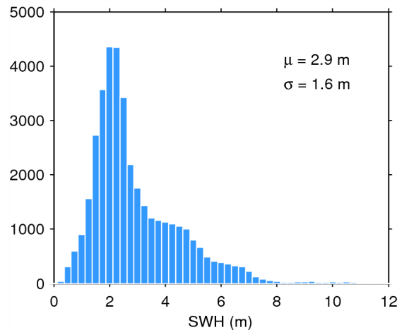
Figure 20. Histogram of science-valid SWH over oceans and lakes for 28/05/2014. The mean ( \mu ) and standard deviation ( \sigma ) are also shown. Note that values larger than 12 m are excluded from the histogram for the sake of readability but not from the computation of \mu and \sigma .
