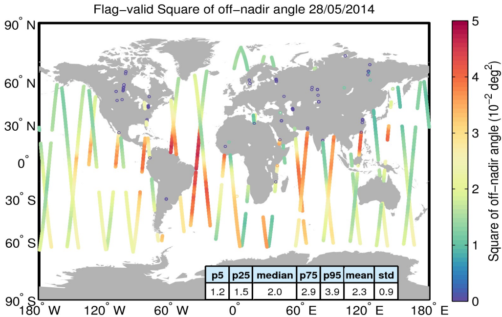
Figure 37. Geographical distribution of flag-valid mispointing data over oceans and lakes for 28/05/2014. The statistical values shown in the table refer to the mispointing in 10^{-2} \text{ deg}^2 and are calculated over all measurements shown in the figure.
