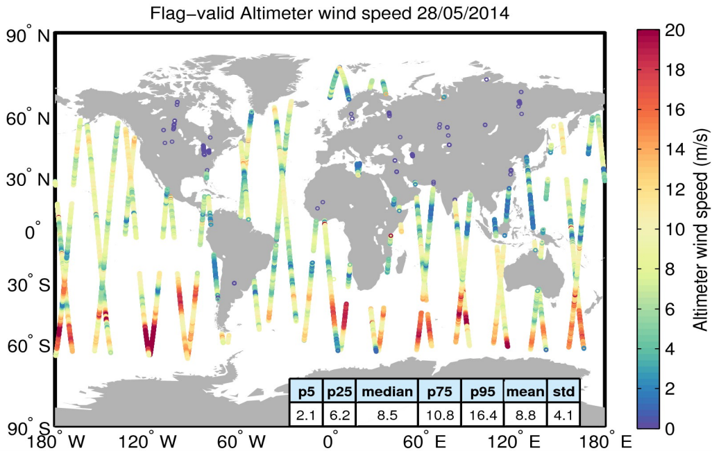
Figure 31. Geographical distribution of flag-valid wind data over oceans and lakes for 28/05/2014. The statistical values shown in the table refer to the wind in m/s and are calculated over all measurements shown in the figure.
