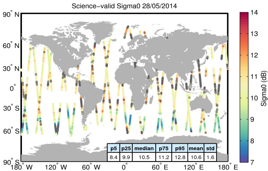
Figure 27. Geographical distribution of science-valid sigma0 data over oceans and lakes for 28/05/2014. The statistical values shown in the table refer to the sigma0 in dB and are calculated over all measurements shown in the figure. Gray circles denote records that have been rejected based on the editing criteria described in Table 4.
