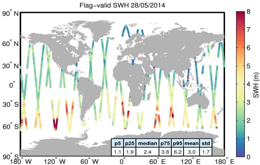
Figure 15. Geographical distribution of flag-valid SWH data over oceans and lakes for 28/05/2014. The statistical values shown in the figure refer to the SWH in m and are calculated over all measurements shown in the figure.
