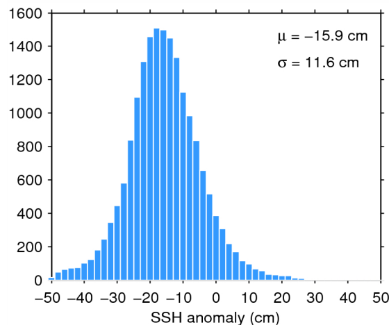
Figure 11. Histogram of science-valid SSH anomaly over oceans and lakes for 28/05/2014. The mean ( \mu ) and standard deviation ( \sigma ) are also shown. Note that values outside [-50 50] cm are excluded from the histogram for the sake of readability but not from the computation of \mu and \sigma .
