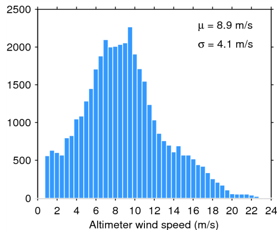
Figure 35. Histogram of science-valid wind over oceans and lakes for 27/05/2014. The mean ( \mu ) and standard deviation ( \sigma ) are also shown. Note that values larger than 24 m/s are excluded from the histogram for the sake of readability but not from the computation of \mu and \sigma .
