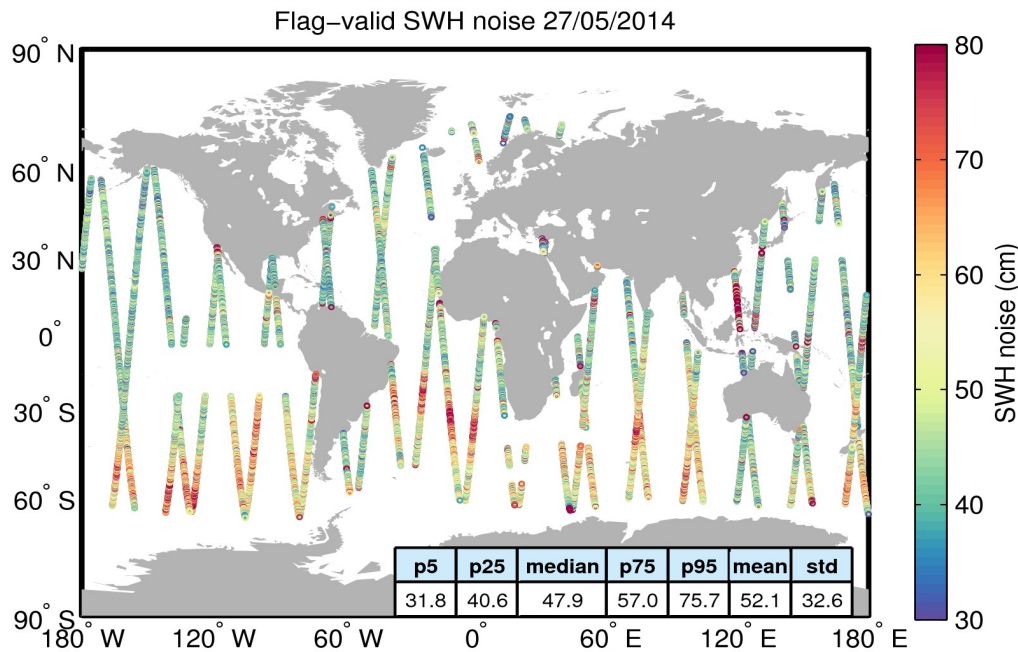
Figure 18. Geographical distribution of flag-valid 20-Hz SWH measurement noise over oceans and lakes for 27/05/2014. The statistical values shown in the figure refer to the SWH noise and are calculated over all measurements shown in the figure.
