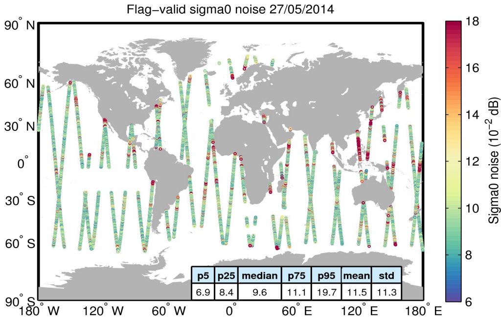
Figure 26. Geographical distribution of flag-valid 20-Hz sigma0 measurement noise over oceans and lakes for 27/05/2014. The statistical values shown in the table refer to the sigma0 noise and are calculated over all measurements shown in the figure.
