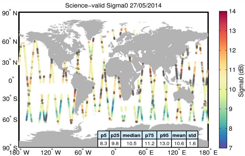
Figure 27. Geographical distribution of science-valid sigma0 data over oceans and lakes for 27/05/2014. The statistical values shown in the table refer to the sigma0 in dB and are calculated over all measurements shown in the figure. Gray circles denote records that have been rejected based on the editing criteria described in Table 4.
