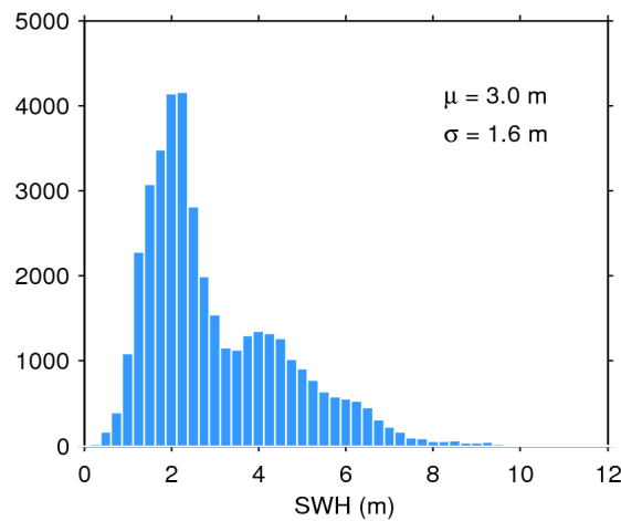
Figure 17. Histogram of flag-valid SWH over oceans and lakes for 27/05/2014. The mean ( \mu ) and standard deviation ( \sigma ) are also shown. Note that values larger than 12 m are excluded from the histogram for the sake of readability but not from the computation of \mu and \sigma .
