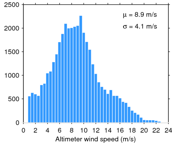
Figure 33. Histogram of flag-valid wind over oceans and lakes for 27/05/2014. The mean ( \mu ) and standard deviation ( \sigma ) are also shown. Note that values larger than 24 m/s are excluded from the histogram for the sake of readability but not from the computation of \mu and \sigma .
