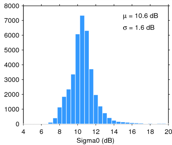
Figure 28. Histogram of science-valid sigma0 over oceans and lakes for 27/05/2014. The mean ( \mu ) and standard deviation ( \sigma ) are also shown. Note that values outside [4 20] dB are excluded from the histogram for the sake of readability but not from the computation of \mu and \sigma .
