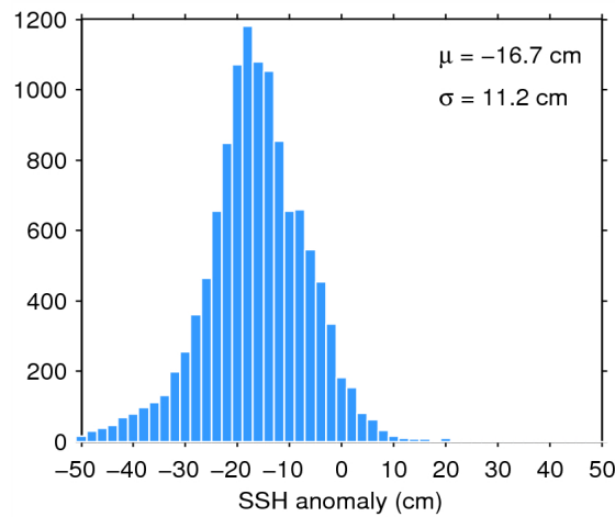
Figure 11. Histogram of science-valid SSH anomaly over oceans and lakes for 27/05/2014. The mean ( \mu ) and standard deviation ( \sigma ) are also shown. Note that values outside [-50 50] cm are excluded from the histogram for the sake of readability but not from the computation of \mu and \sigma .
