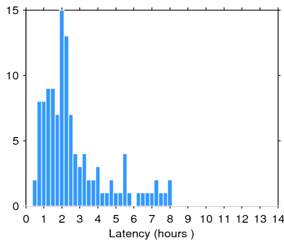
Figure 2. Histogram of the data latency for 27/05/2014. The y-axis denotes the number of files that are made available with a delay of x-hours with respect to the mean time of the records stored in the file.
