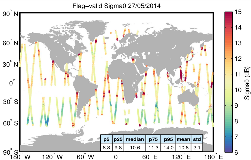
Figure 23. Geographical distribution of flag-valid sigma0 data over oceans and lakes for 27/05/2014. The statistical values shown in the table refer to the sigma0 in dB and are calculated over all measurements shown in the figure.
