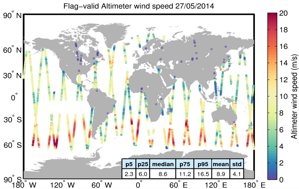
Figure 31. Geographical distribution of flag-valid wind data over oceans and lakes for 27/05/2014. The statistical values shown in the table refer to the wind in m/s and are calculated over all measurements shown in the figure.
