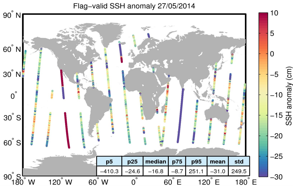
Figure 5. Geographical distribution of flag-valid 1-Hz SSH anomaly data over oceans and lakes for 27/05/2014. The statistical values shown in the table refer to the SSH anomaly in cm and are calculated over all measurements shown in the figure.
