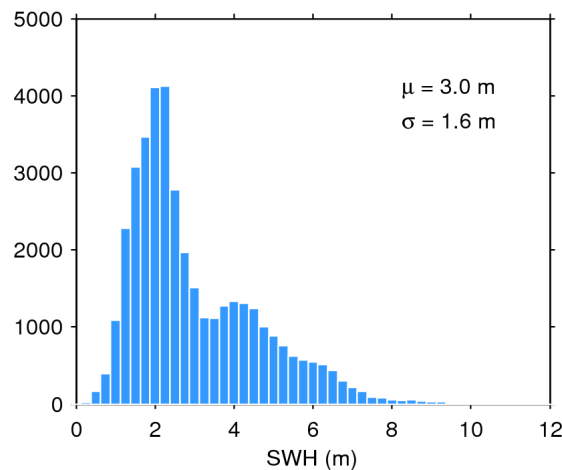
Figure 20. Histogram of science-valid SWH over oceans and lakes for 27/05/2014. The mean ( \mu ) and standard deviation ( \sigma ) are also shown. Note that values larger than 12 m are excluded from the histogram for the sake of readability but not from the computation of \mu and \sigma .
