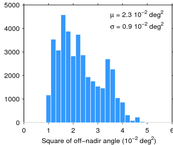
Figure 39. Histogram of flag-valid mispointing over oceans and lakes for 27/05/2014. The mean ( \mu ) and standard deviation ( \sigma ) are also shown. Note that values than 6 \cdot 10^{-2} \text{ deg}^2 are excluded from the histogram for the sake of readability but not from the computation of \mu and \sigma .
