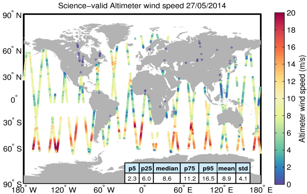
Figure 34. Geographical distribution of science-valid wind data over oceans and lakes for 27/05/2014. The statistical values shown in the table refer to the wind in m/s and are calculated over all measurements shown in the figure. Gray circles denote records that have been rejected based on the editing criteria described in Table 5.
