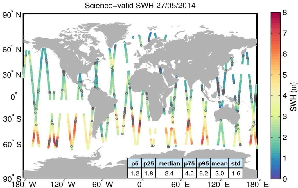
Figure 19. Geographical distribution of science-valid SWH data over oceans and lakes for 27/05/2014. The statistical values shown in the table refer to the SWH in m and are calculated over all measurements shown in the figure. Gray circles denote records that have been rejected based on the editing criteria described in Table 3.
