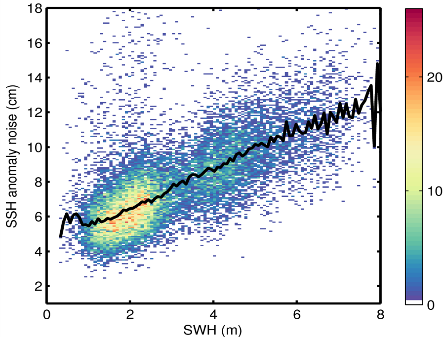
Figure 9. 2D histogram showing flag-valid SSH anomaly noise as a function of SWH for 27/05/2014. The black line denotes the median SSH anomaly as a function of SWH.
