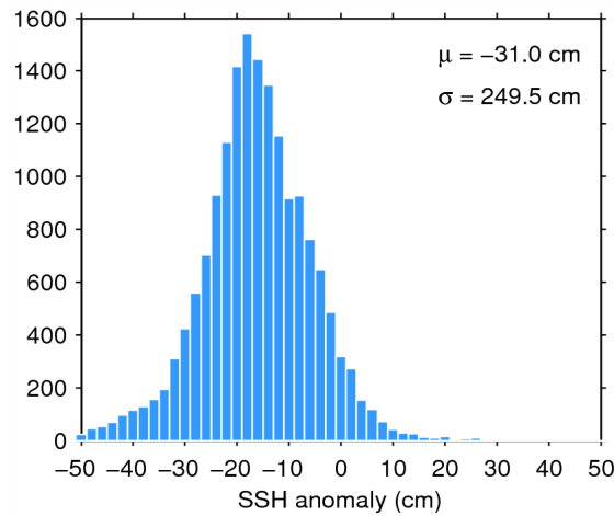
Figure 7. Histogram of flag-valid SSH anomaly over oceans and lakes for 27/05/2014. The mean ( \mu ) and standard deviation ( \sigma ) are also shown. Note that values outside [-50 50] cm are excluded from the histogram for the sake of readability but not from the computation of \mu and \sigma .
