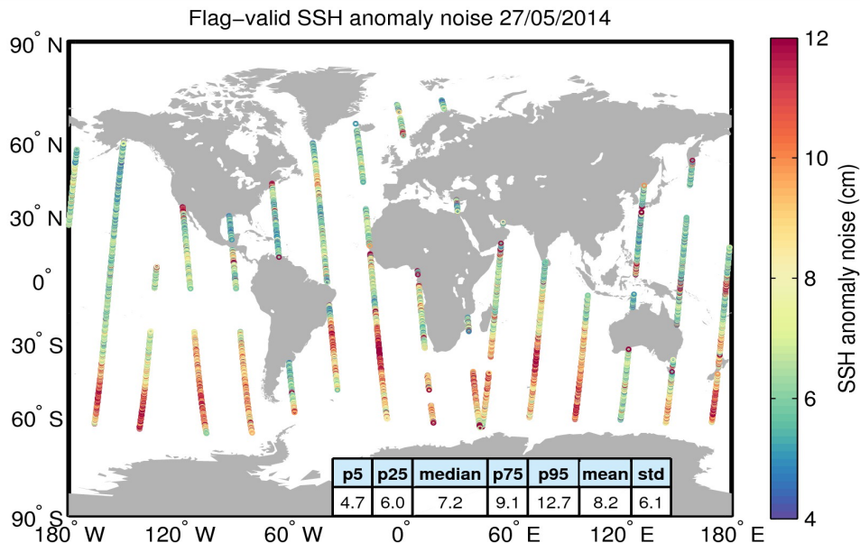
Figure 8. Geographical distribution of flag-valid 20-Hz SSH anomaly measurement noise over oceans and lakes for 27/05/2014. The statistical values shown in the table refer to the SSH anomaly noise and are calculated over all measurements shown in the figure.
