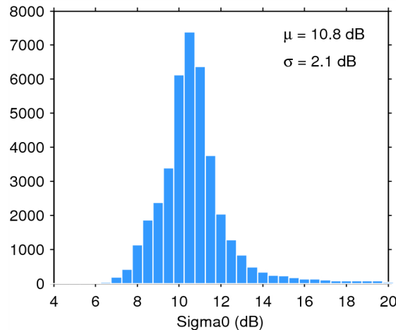
Figure 25. Histogram of flag-valid sigma0 over oceans and lakes for 27/05/2014. The mean ( \mu ) and standard deviation ( \sigma ) are also shown. Note that values outside [4 20] dB are excluded from the histogram for the sake of readability but not from the computation of \mu and \sigma .
