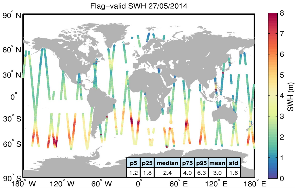
Figure 15. Geographical distribution of flag-valid SWH data over oceans and lakes for 27/05/2014. The statistical values shown in the table refer to the SWH in m and are calculated over all measurements shown in the figure.
