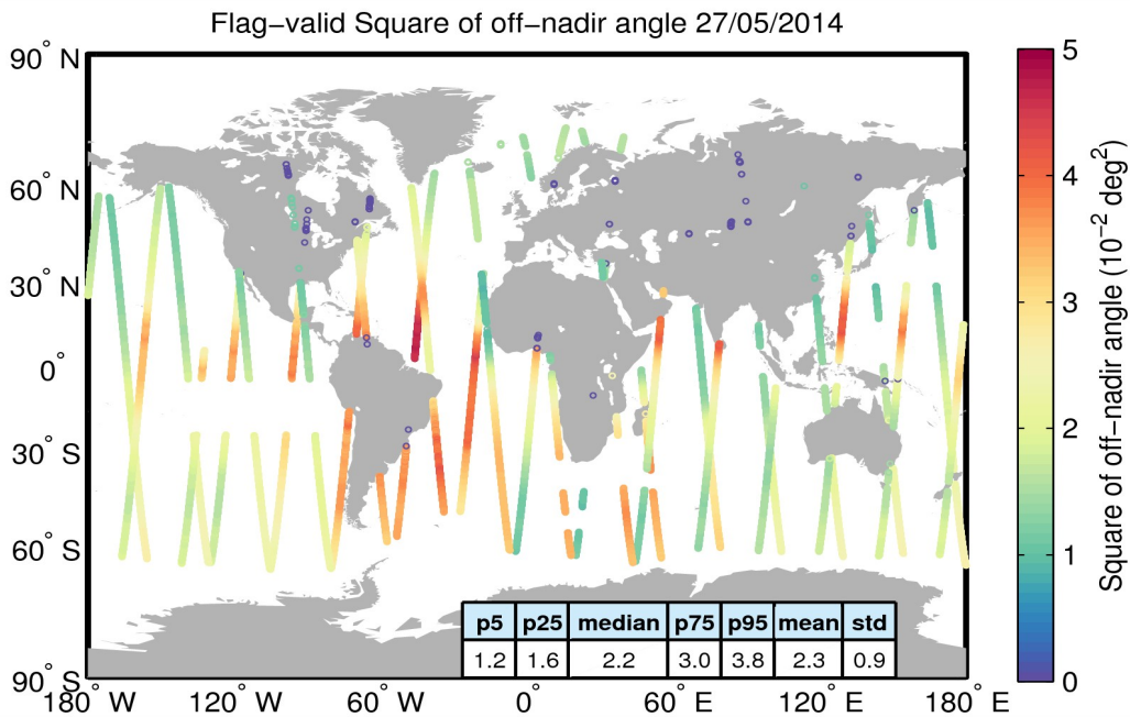
Figure 37. Geographical distribution of flag-valid mispointing data over oceans and lakes for 27/05/2014. The statistical values shown in the table refer to the mispointing in 10^{-2} \text{ deg}^2 and are calculated over all measurements shown in the figure.
