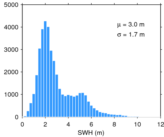
Figure 17. Histogram of flag-valid SWH over oceans and lakes for 26/05/2014. The mean ( \mu ) and standard deviation ( \sigma ) are also shown. Note that values larger than 12 m are excluded from the histogram for the sake of readability but not from the computation of \mu and \sigma .
