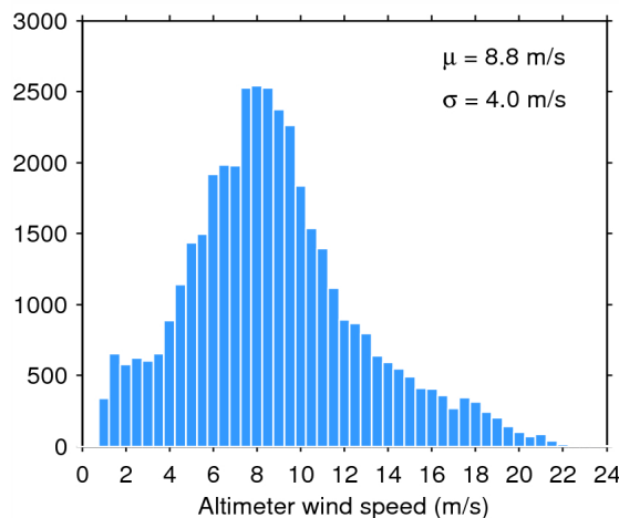
Figure 35. Histogram of science-valid wind over oceans and lakes for 26/05/2014. The mean ( \mu ) and standard deviation ( \sigma ) are also shown. Note that values larger than 24 m/s are excluded from the histogram for the sake of readability but not from the computation of \mu and \sigma .
