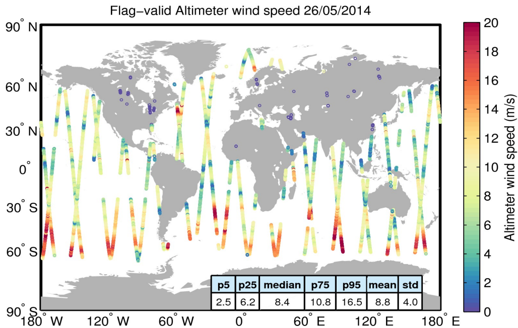
Figure 31. Geographical distribution of flag-valid wind data over oceans and lakes for 26/05/2014. The statistical values shown in the table refer to the wind in m/s and are calculated over all measurements shown in the figure.
