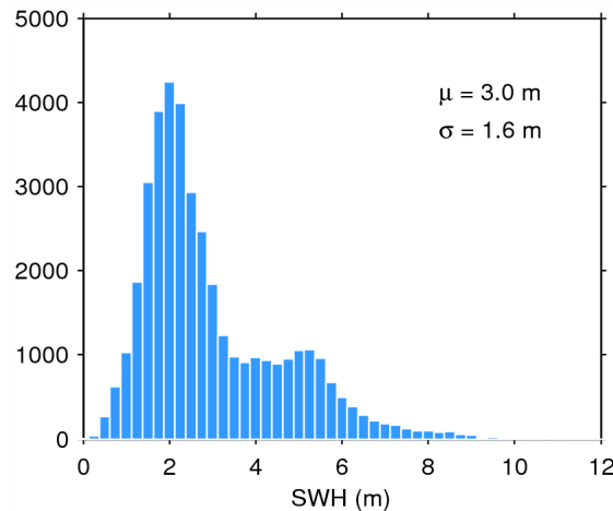
Figure 20. Histogram of science-valid SWH over oceans and lakes for 26/05/2014. The mean ( \mu ) and standard deviation ( \sigma ) are also shown. Note that values larger than 12 m are excluded from the histogram for the sake of readability but not from the computation of \mu and \sigma .
