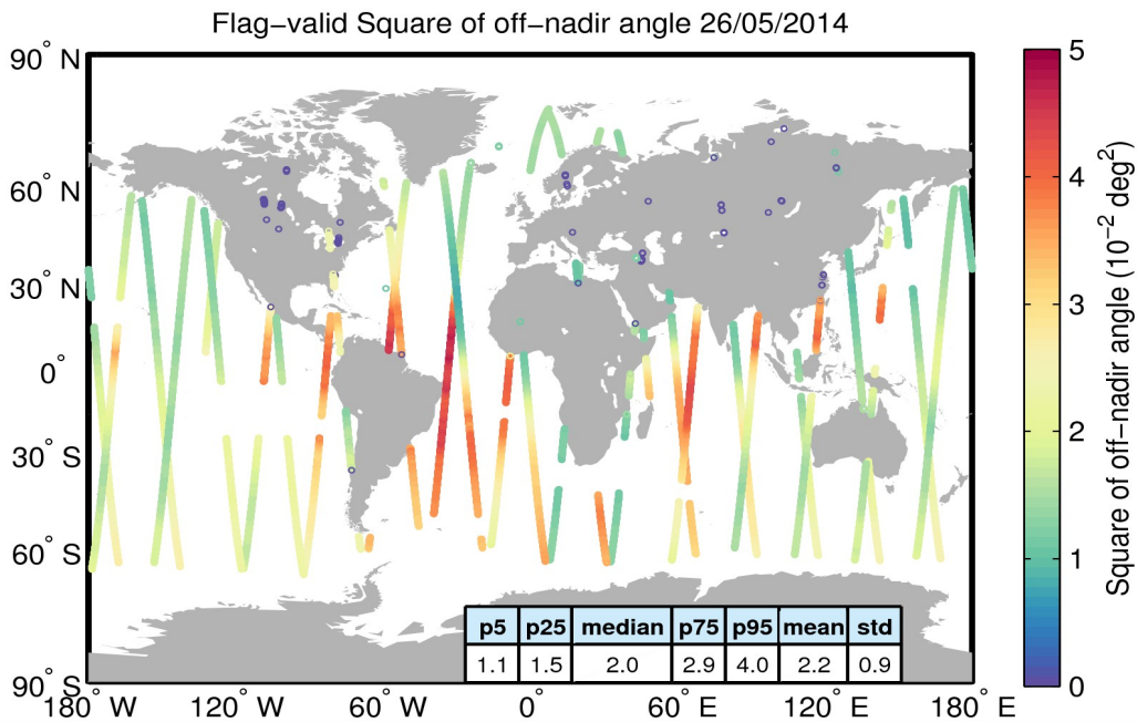
Figure 37. Geographical distribution of flag-valid mispointing data over oceans and lakes for 26/05/2014. The statistical values shown in the table refer to the mispointing in 10^{-2} \text{ deg}^2 and are calculated over all measurements shown in the figure.
