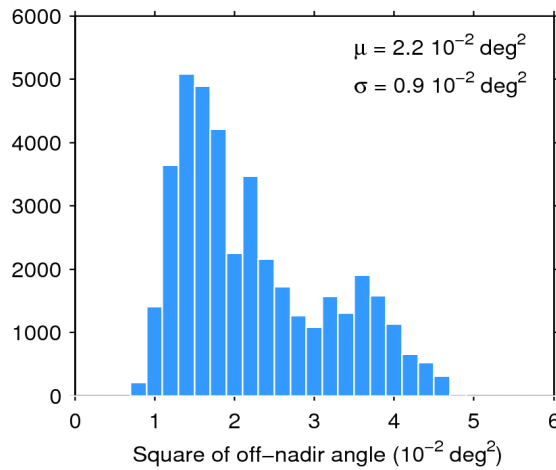
Figure 39. Histogram of flag-valid mispointing over oceans and lakes for 26/05/2014. The mean ( \mu ) and standard deviation ( \sigma ) are also shown. Note that values than 6 \cdot 10^{-2} \text{ deg}^2 are excluded from the histogram for the sake of readability but not from the computation of \mu and \sigma .
