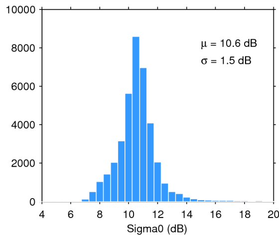
Figure 28. Histogram of science-valid sigma0 over oceans and lakes for 26/05/2014. The mean ( \mu ) and standard deviation ( \sigma ) are also shown. Note that values outside [4 20] dB are excluded from the histogram for the sake of readability but not from the computation of \mu and \sigma .
