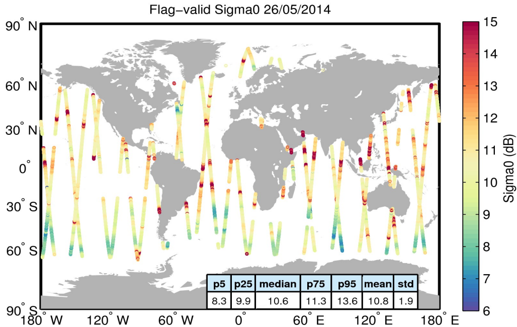
Figure 23. Geographical distribution of flag-valid sigma0 data over oceans and lakes for 26/05/2014. The statistical values shown in the table refer to the sigma0 in dB and are calculated over all measurements shown in the figure.
