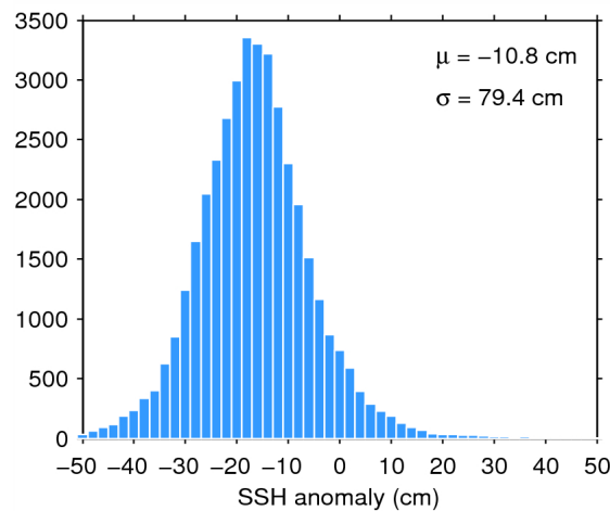
Figure 7. Histogram of flag-valid SSH anomaly over oceans and lakes for 26/05/2014. The mean ( \mu ) and standard deviation ( \sigma ) are also shown. Note that values outside [-50 50] cm are excluded from the histogram for the sake of readability but not from the computation of \mu and \sigma .
