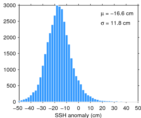
Figure 11. Histogram of science-valid SSH anomaly over oceans and lakes for 26/05/2014. The mean ( \mu ) and standard deviation ( \sigma ) are also shown. Note that values outside [-50 50] cm are excluded from the histogram for the sake of readability but not from the computation of \mu and \sigma .
