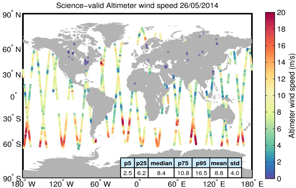
Figure 34. Geographical distribution of science-valid wind data over oceans and lakes for 26/05/2014. The statistical values shown in the table refer to the wind in m/s and are calculated over all measurements shown in the figure. Gray circles denote records that have been rejected based on the editing criteria described in Table 5.
