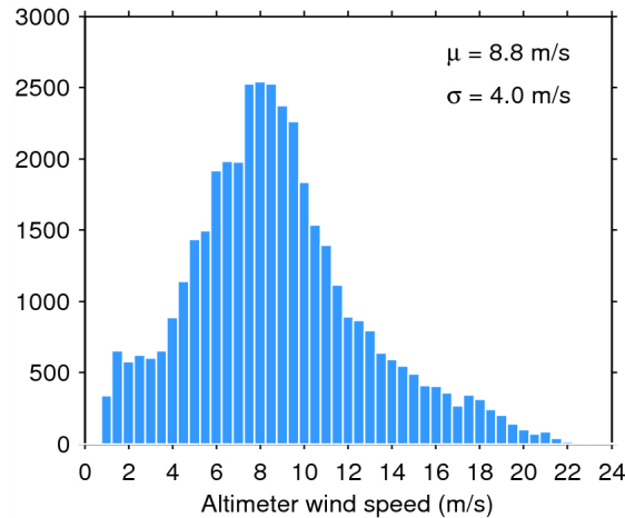
Figure 33. Histogram of flag-valid wind over oceans and lakes for 26/05/2014. The mean ( \mu ) and standard deviation ( \sigma ) are also shown. Note that values larger than 24 m/s are excluded from the histogram for the sake of readability but not from the computation of \mu and \sigma .
