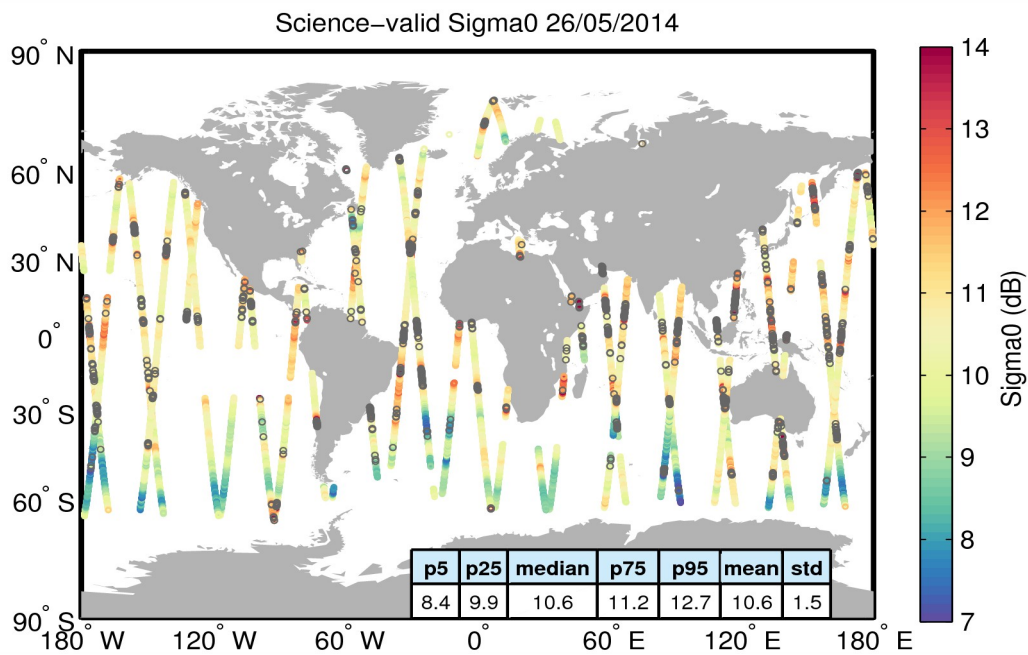
Figure 27. Geographical distribution of science-valid sigma0 data over oceans and lakes for 26/05/2014. The statistical values shown in the table refer to the sigma0 in dB and are calculated over all measurements shown in the figure. Gray circles denote records that have been rejected based on the editing criteria described in Table 4.
