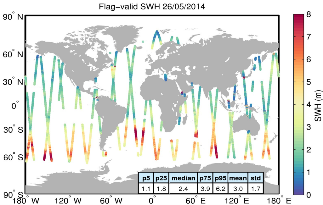
Figure 15. Geographical distribution of flag-valid SWH data over oceans and lakes for 26/05/2014. The statistical values shown in the table refer to the SWH in m and are calculated over all measurements shown in the figure.
