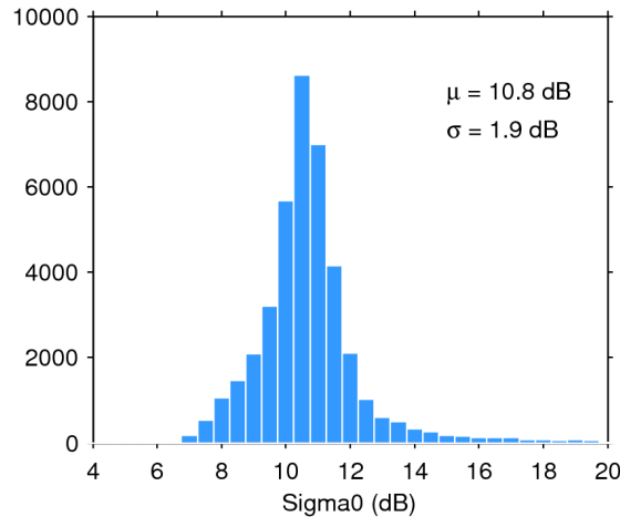
Figure 25. Histogram of flag-valid sigma0 over oceans and lakes for 26/05/2014. The mean ( \mu ) and standard deviation ( \sigma ) are also shown. Note that values outside [4 20] dB are excluded from the histogram for the sake of readability but not from the computation of \mu and \sigma .
