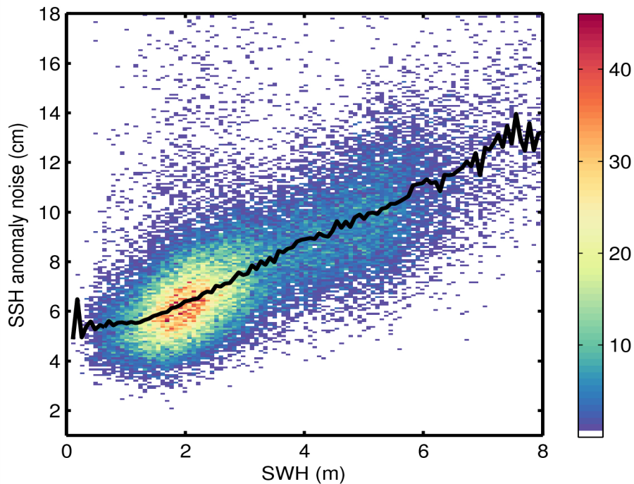
Figure 9. 2D histogram showing flag-valid SSH anomaly noise as a function of SWH for 26/05/2014. The black line denotes the median SSH anomaly as a function of SWH.
