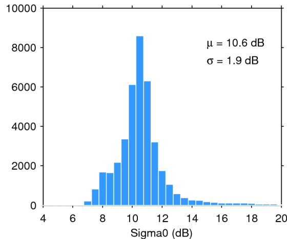
Figure 25. Histogram of flag-valid sigma0 over oceans and lakes for 25/05/2014. The mean ( \mu ) and standard deviation ( \sigma ) are also shown. Note that values outside [4 20] dB are excluded from the histogram for the sake of readability but not from the computation of \mu and \sigma .
