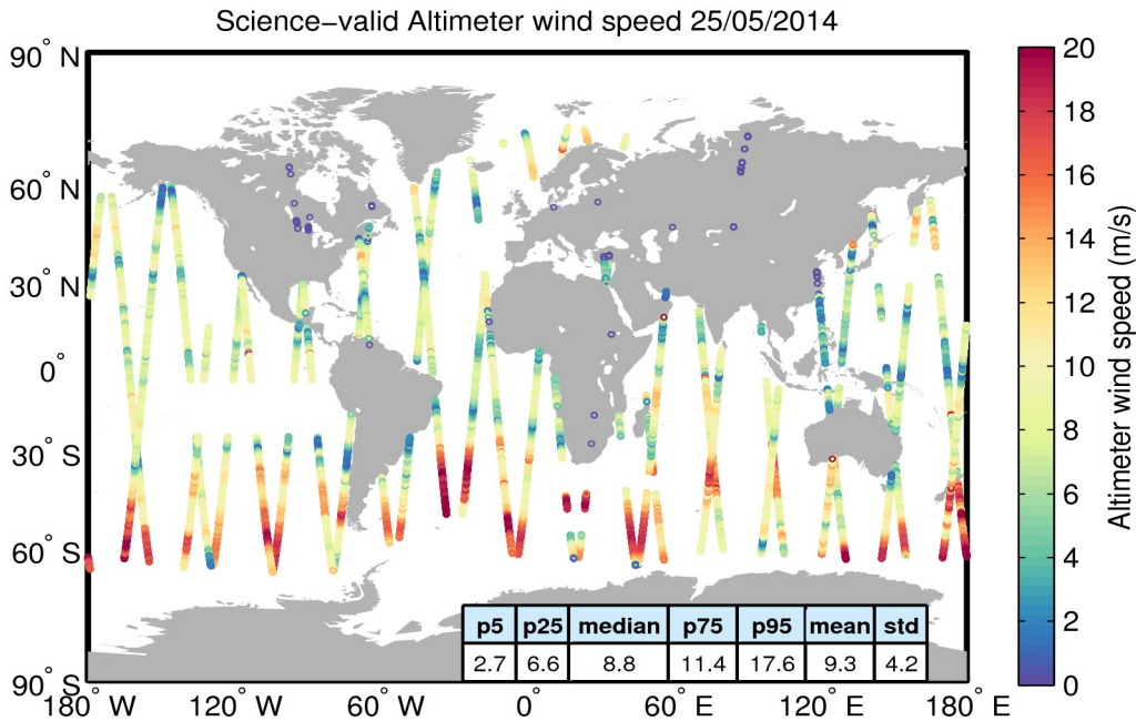
Figure 34. Geographical distribution of science-valid wind data over oceans and lakes for 25/05/2014. The statistical values shown in the table refer to the wind in m/s and are calculated over all measurements shown in the figure. Gray circles denote records that have been rejected based on the editing criteria described in Table 5.
