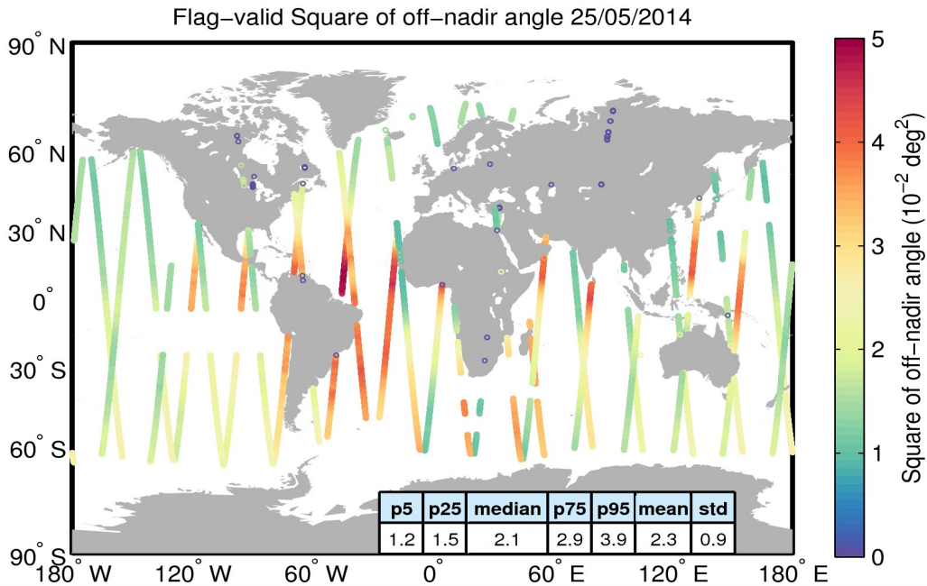
Figure 37. Geographical distribution of flag-valid mispointing data over oceans and lakes for 25/05/2014. The statistical values shown in the table refer to the mispointing in 10^{-2} \text{ deg}^2 and are calculated over all measurements shown in the figure.
