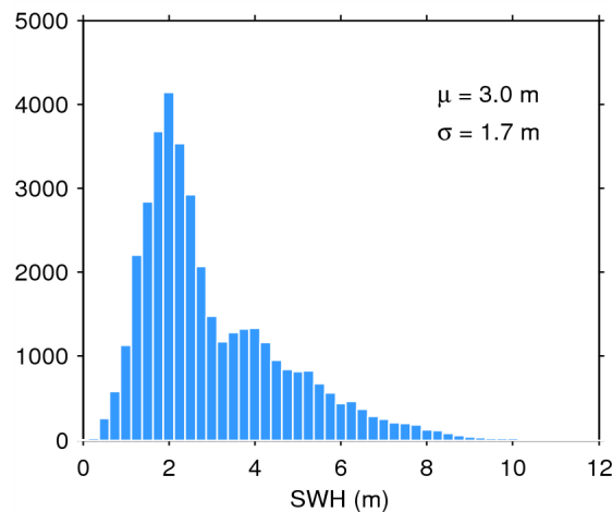
Figure 20. Histogram of science-valid SWH over oceans and lakes for 25/05/2014. The mean ( \mu ) and standard deviation ( \sigma ) are also shown. Note that values larger than 12 m are excluded from the histogram for the sake of readability but not from the computation of \mu and \sigma .
