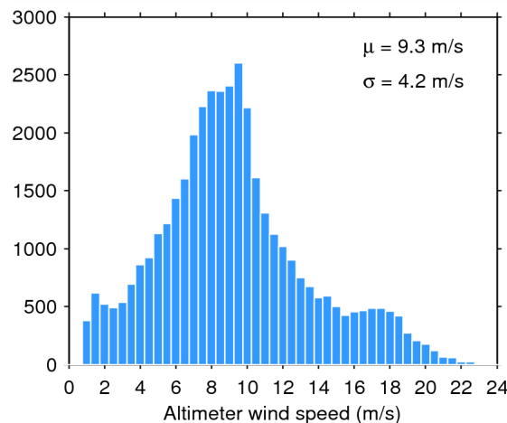
Figure 35. Histogram of science-valid wind over oceans and lakes for 25/05/2014. The mean ( \mu ) and standard deviation ( \sigma ) are also shown. Note that values larger than 24 m/s are excluded from the histogram for the sake of readability but not from the computation of \mu and \sigma .
