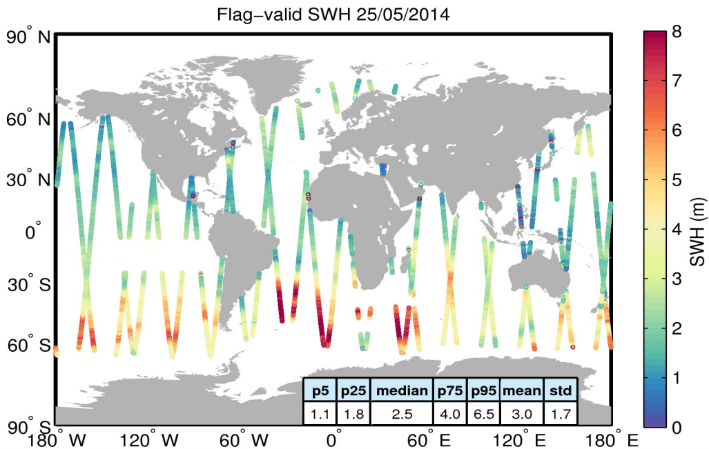
Figure 15. Geographical distribution of flag-valid SWH data over oceans and lakes for 25/05/2014. The statistical values shown in the table refer to the SWH in m and are calculated over all measurements shown in the figure.
