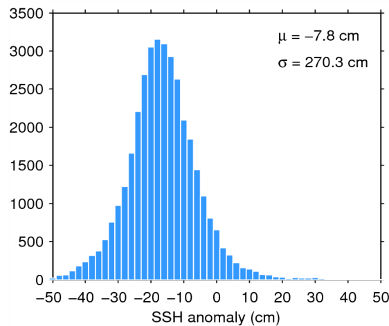
Figure 7. Histogram of flag-valid SSH anomaly over oceans and lakes for 25/05/2014. The mean ( \mu ) and standard deviation ( \sigma ) are also shown. Note that values outside [-50\ 50] cm are excluded from the histogram for the sake of readability but not from the computation of \mu and \sigma .
