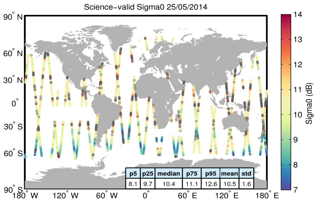
Figure 27. Geographical distribution of science-valid sigma0 data over oceans and lakes for 25/05/2014. The statistical values shown in the table refer to the sigma0 in dB and are calculated over all measurements shown in the figure. Gray circles denote records that have been rejected based on the editing criteria described in Table 4.
