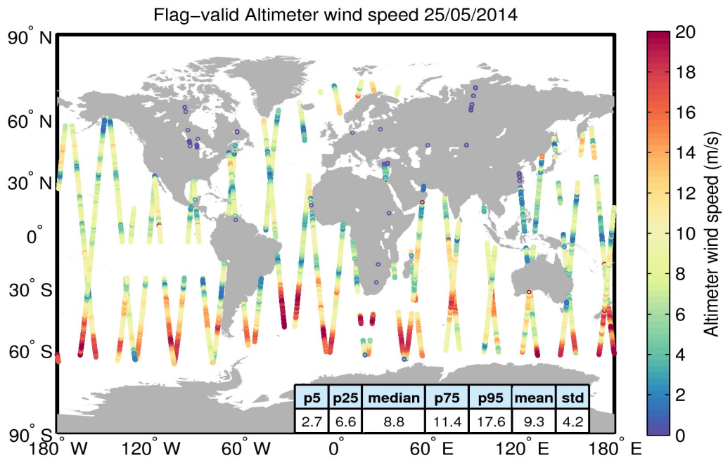
Figure 31. Geographical distribution of flag-valid wind data over oceans and lakes for 25/05/2014. The statistical values shown in the table refer to the wind in m/s and are calculated over all measurements shown in the figure.
