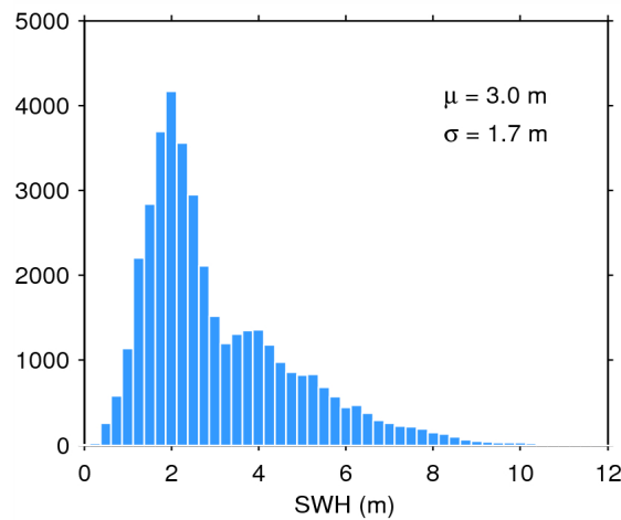
Figure 17. Histogram of flag-valid SWH over oceans and lakes for 25/05/2014. The mean ( \mu ) and standard deviation ( \sigma ) are also shown. Note that values larger than 12 m are excluded from the histogram for the sake of readability but not from the computation of \mu and \sigma .
