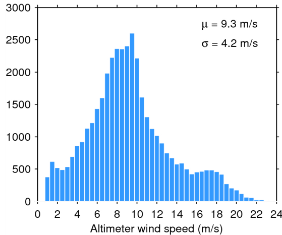
Figure 33. Histogram of flag-valid wind over oceans and lakes for 25/05/2014. The mean ( \mu ) and standard deviation ( \sigma ) are also shown. Note that values larger than 24 m/s are excluded from the histogram for the sake of readability but not from the computation of \mu and \sigma .
