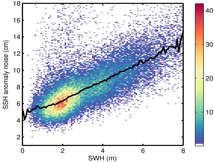
Figure 9. 2D histogram showing flag-valid SSH anomaly noise as a function of SWH for 25/05/2014. The black line denotes the median SSH anomaly as a function of SWH.
