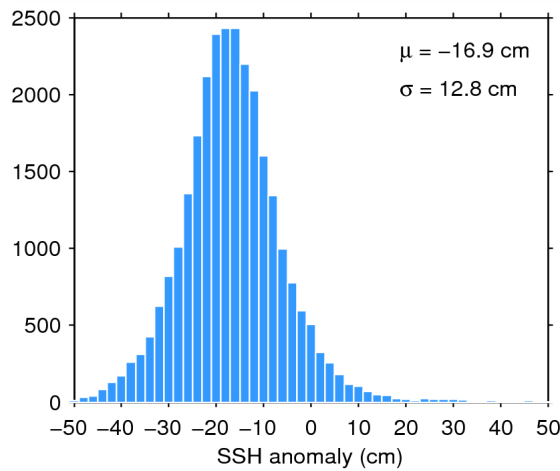
Figure 11. Histogram of science-valid SSH anomaly over oceans and lakes for 25/05/2014. The mean ( \mu ) and standard deviation ( \sigma ) are also shown. Note that values outside [-50 50] cm are excluded from the histogram for the sake of readability but not from the computation of \mu and \sigma .
