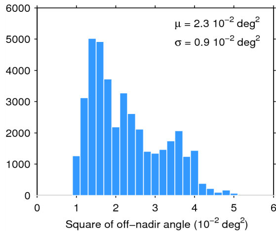
Figure 39. Histogram of flag-valid mispointing over oceans and lakes for 25/05/2014. The mean ( \mu ) and standard deviation ( \sigma ) are also shown. Note that values than 6 \cdot 10^{-2} \text{ deg}^2 are excluded from the histogram for the sake of readability but not from the computation of \mu and \sigma .
