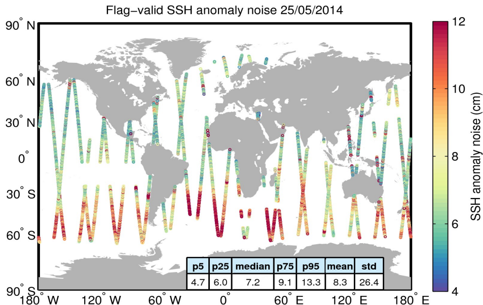
Figure 8. Geographical distribution of flag-valid 20-Hz SSH anomaly measurement noise over oceans and lakes for 25/05/2014. The statistical values shown in the table refer to the SSH anomaly noise and are calculated over all measurements shown in the figure.
