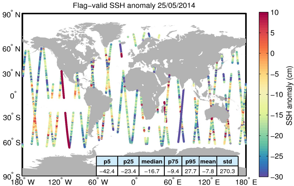
Figure 5. Geographical distribution of flag-valid 1-Hz SSH anomaly data over oceans and lakes for 25/05/2014. The statistical values shown in the table refer to the SSH anomaly in cm and are calculated over all measurements shown in the figure.
