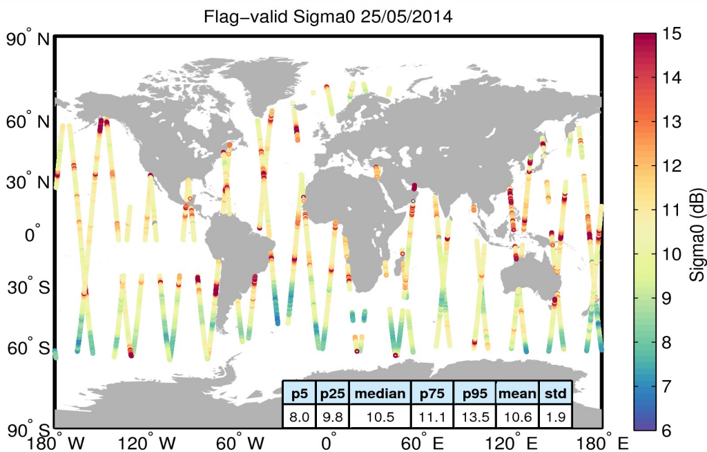
Figure 23. Geographical distribution of flag-valid sigma0 data over oceans and lakes for 25/05/2014. The statistical values shown in the table refer to the sigma0 in dB and are calculated over all measurements shown in the figure.
