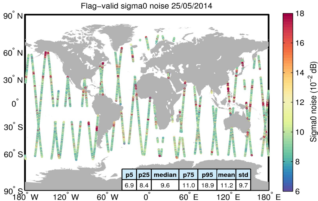
Figure 26. Geographical distribution of flag-valid 20-Hz sigma0 measurement noise over oceans and lakes for 25/05/2014. The statistical values shown in the table refer to the sigma0 noise and are calculated over all measurements shown in the figure.
