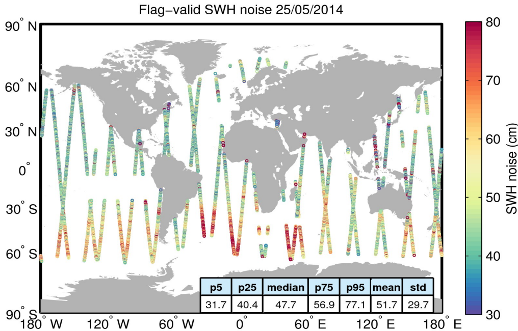
Figure 18. Geographical distribution of flag-valid 20-Hz SWH measurement noise over oceans and lakes for 25/05/2014. The statistical values shown in the figure refer to the SWH noise and are calculated over all measurements shown in the figure.
