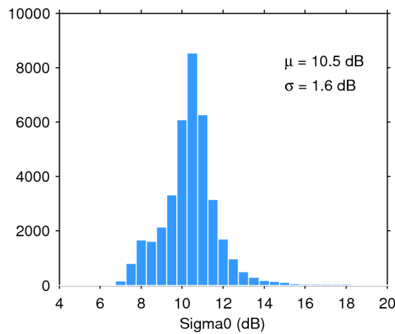
Figure 28. Histogram of science-valid sigma0 over oceans and lakes for 25/05/2014. The mean ( \mu ) and standard deviation ( \sigma ) are also shown. Note that values outside [4 20] dB are excluded from the histogram for the sake of readability but not from the computation of \mu and \sigma .
