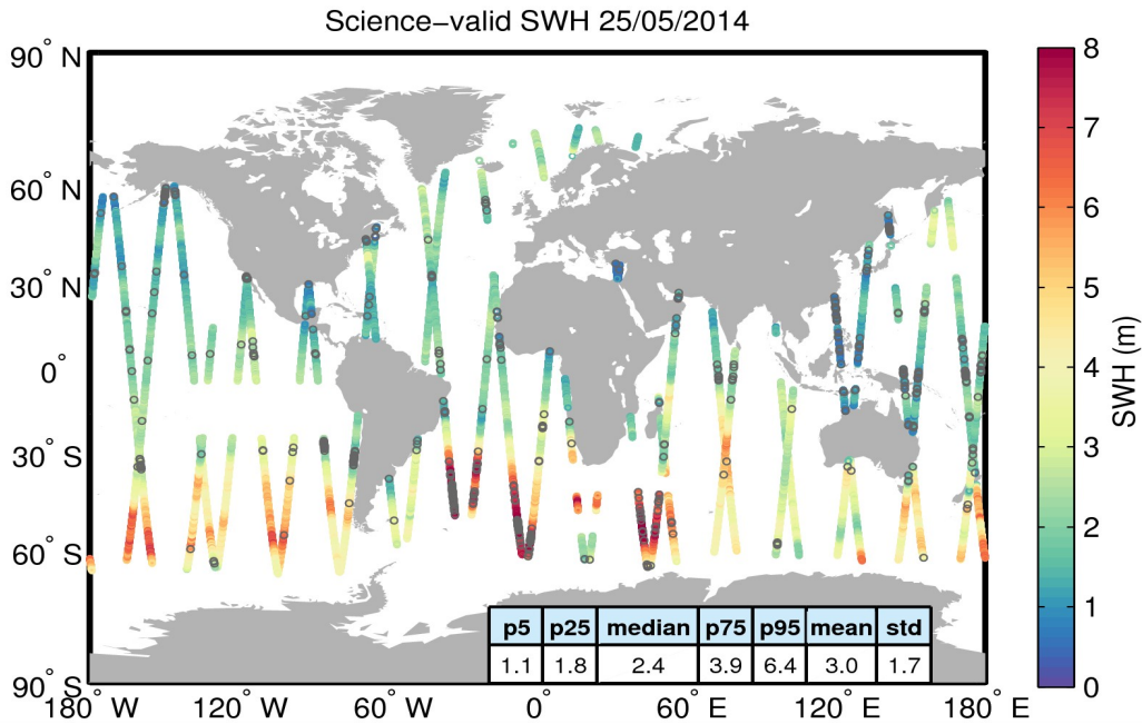
Figure 19. Geographical distribution of science-valid SWH data over oceans and lakes for 25/05/2014. The statistical values shown in the table refer to the SWH in m and are calculated over all measurements shown in the figure. Gray circles denote records that have been rejected based on the editing criteria described in Table 3.
