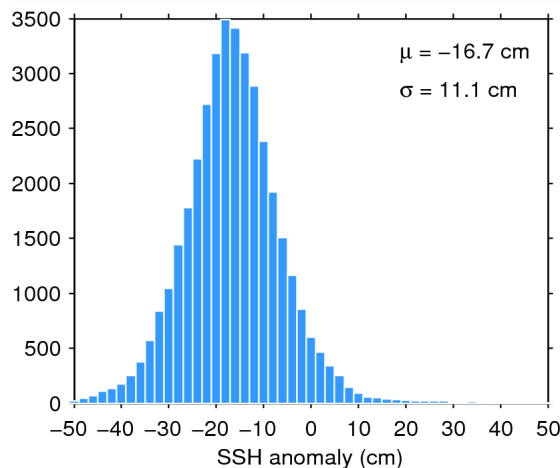
Figure 11. Histogram of science-valid SSH anomaly over oceans and lakes for 24/05/2014. The mean ( \mu ) and standard deviation ( \sigma ) are also shown. Note that values outside [-50 50] cm are excluded from the histogram for the sake of readability but not from the computation of \mu and \sigma .
