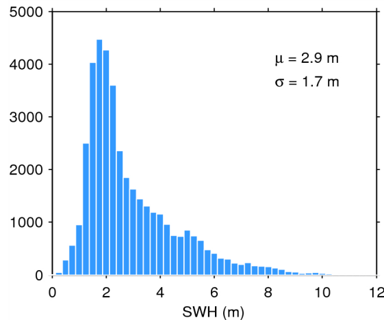
Figure 20. Histogram of science-valid SWH over oceans and lakes for 24/05/2014. The mean ( \mu ) and standard deviation ( \sigma ) are also shown. Note that values larger than 12 m are excluded from the histogram for the sake of readability but not from the computation of \mu and \sigma .
