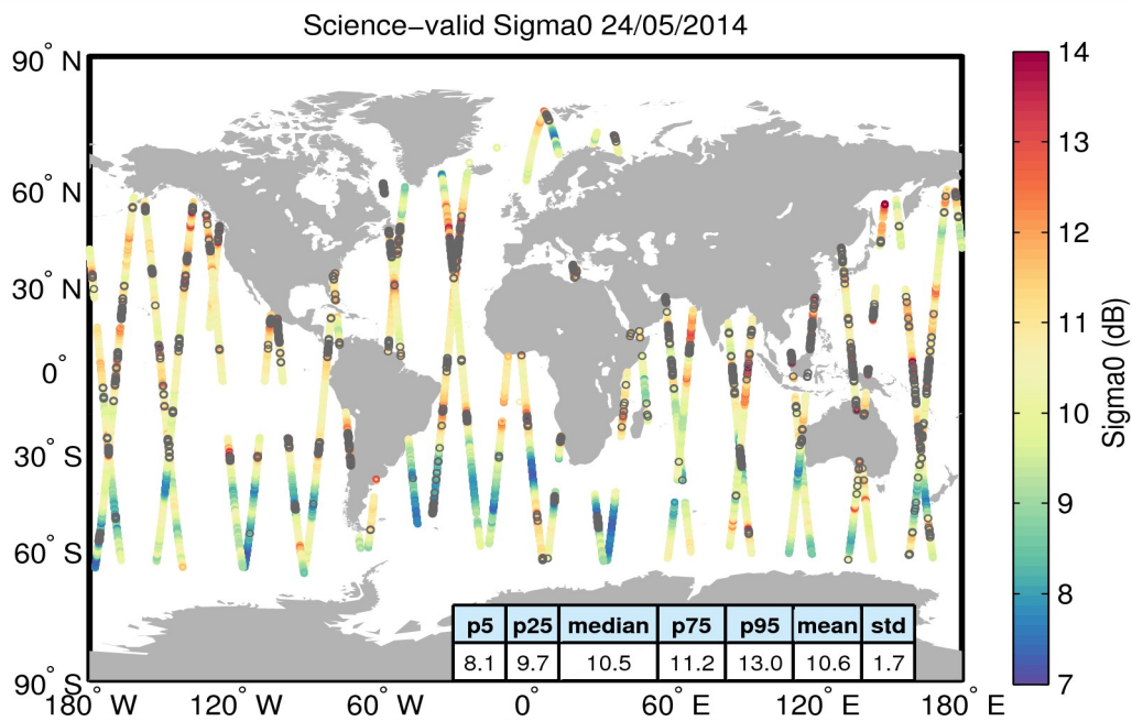
Figure 27. Geographical distribution of science-valid sigma0 data over oceans and lakes for 24/05/2014. The statistical values shown in the table refer to the sigma0 in dB and are calculated over all measurements shown in the figure. Gray circles denote records that have been rejected based on the editing criteria described in Table 4.
