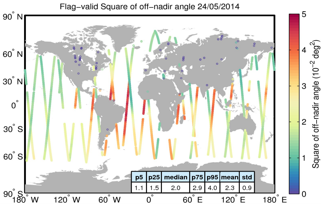
Figure 37. Geographical distribution of flag-valid mispointing data over oceans and lakes for 24/05/2014. The statistical values shown in the table refer to the mispointing in 10^{-2} \text{ deg}^2 and are calculated over all measurements shown in the figure.
