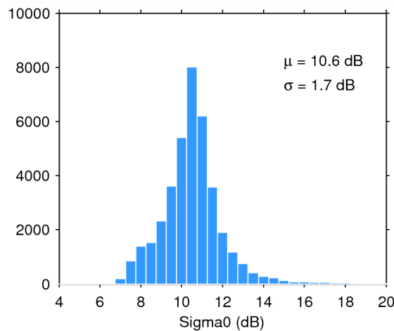
Figure 28. Histogram of science-valid sigma0 over oceans and lakes for 24/05/2014. The mean ( \mu ) and standard deviation ( \sigma ) are also shown. Note that values outside [4 20] dB are excluded from the histogram for the sake of readability but not from the computation of \mu and \sigma .
