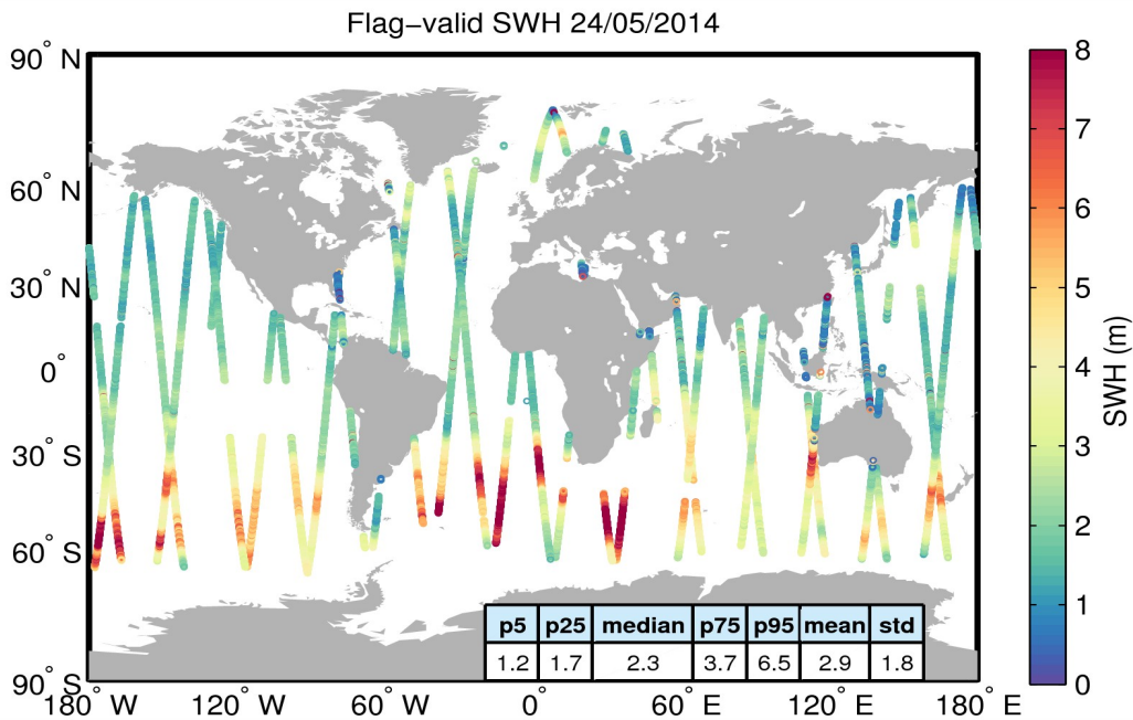
Figure 15. Geographical distribution of flag-valid SWH data over oceans and lakes for 24/05/2014. The statistical values shown in the table refer to the SWH in m and are calculated over all measurements shown in the figure.
