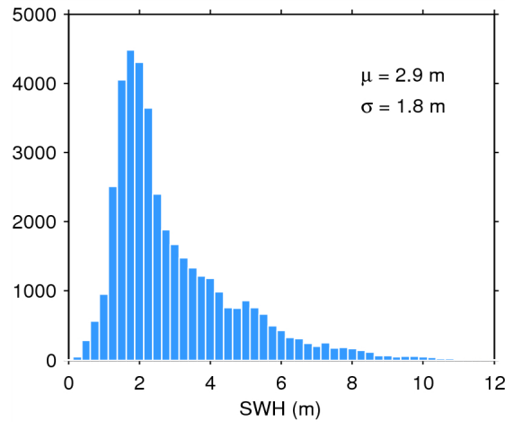
Figure 17. Histogram of flag-valid SWH over oceans and lakes for 24/05/2014. The mean ( \mu ) and standard deviation ( \sigma ) are also shown. Note that values larger than 12 m are excluded from the histogram for the sake of readability but not from the computation of \mu and \sigma .
