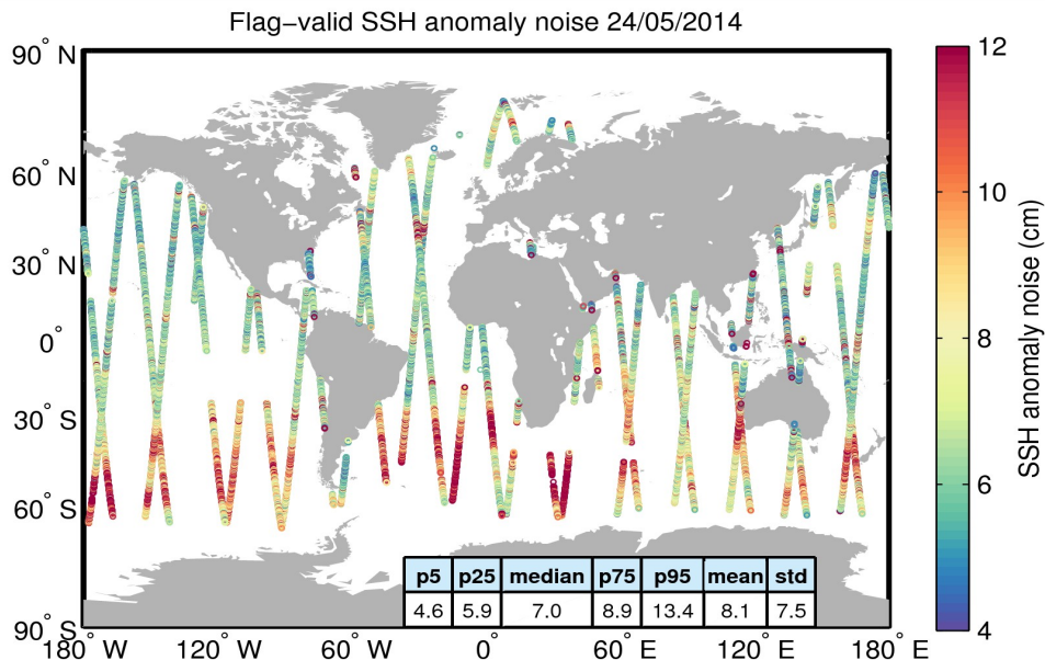
Figure 8. Geographical distribution of flag-valid 20-Hz SSH anomaly measurement noise over oceans and lakes for 24/05/2014. The statistical values shown in the table refer to the SSH anomaly noise and are calculated over all measurements shown in the figure.
