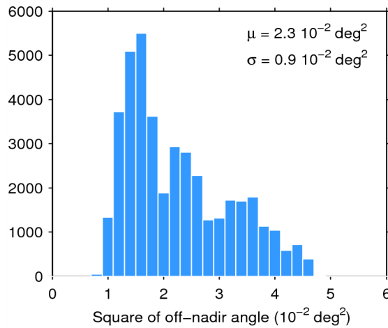
Figure 39. Histogram of flag-valid mispointing over oceans and lakes for 24/05/2014. The mean ( \mu ) and standard deviation ( \sigma ) are also shown. Note that values than 6 \cdot 10^{-2} \text{ deg}^2 are excluded from the histogram for the sake of readability but not from the computation of \mu and \sigma .
