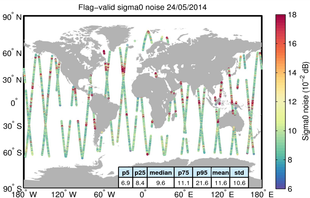
Figure 26. Geographical distribution of flag-valid 20-Hz sigma0 measurement noise over oceans and lakes for 24/05/2014. The statistical values shown in the table refer to the sigma0 noise and are calculated over all measurements shown in the figure.
