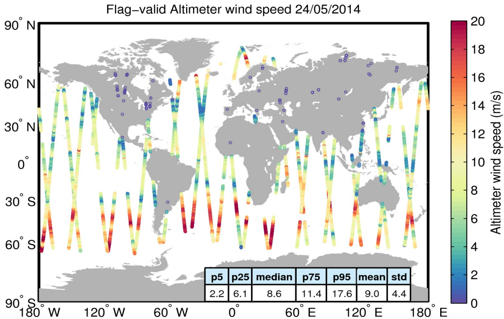
Figure 31. Geographical distribution of flag-valid wind data over oceans and lakes for 24/05/2014. The statistical values shown in the table refer to the wind in m/s and are calculated over all measurements shown in the figure.
