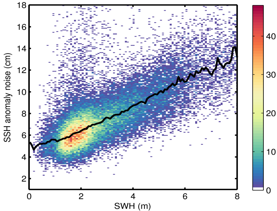
Figure 9. 2D histogram showing flag-valid SSH anomaly noise as a function of SWH for 24/05/2014. The black line denotes the median SSH anomaly as a function of SWH.
