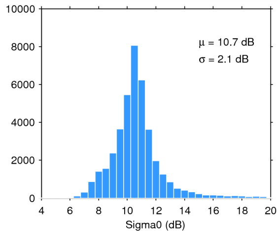
Figure 25. Histogram of flag-valid sigma0 over oceans and lakes for 24/05/2014. The mean ( \mu ) and standard deviation ( \sigma ) are also shown. Note that values outside [4 20] dB are excluded from the histogram for the sake of readability but not from the computation of \mu and \sigma .
