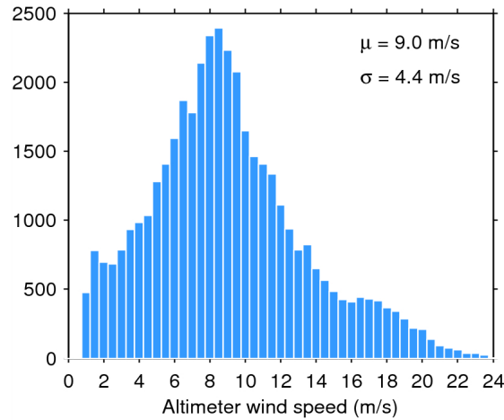
Figure 33. Histogram of flag-valid wind over oceans and lakes for 24/05/2014. The mean ( \mu ) and standard deviation ( \sigma ) are also shown. Note that values larger than 24 m/s are excluded from the histogram for the sake of readability but not from the computation of \mu and \sigma .
