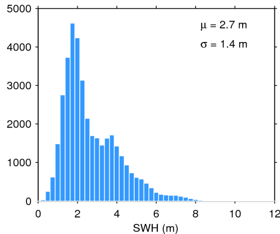
Figure 20. Histogram of science-valid SWH over oceans and lakes for 23/05/2014. The mean ( \mu ) and standard deviation ( \sigma ) are also shown. Note that values larger than 12 m are excluded from the histogram for the sake of readability but not from the computation of \mu and \sigma .
