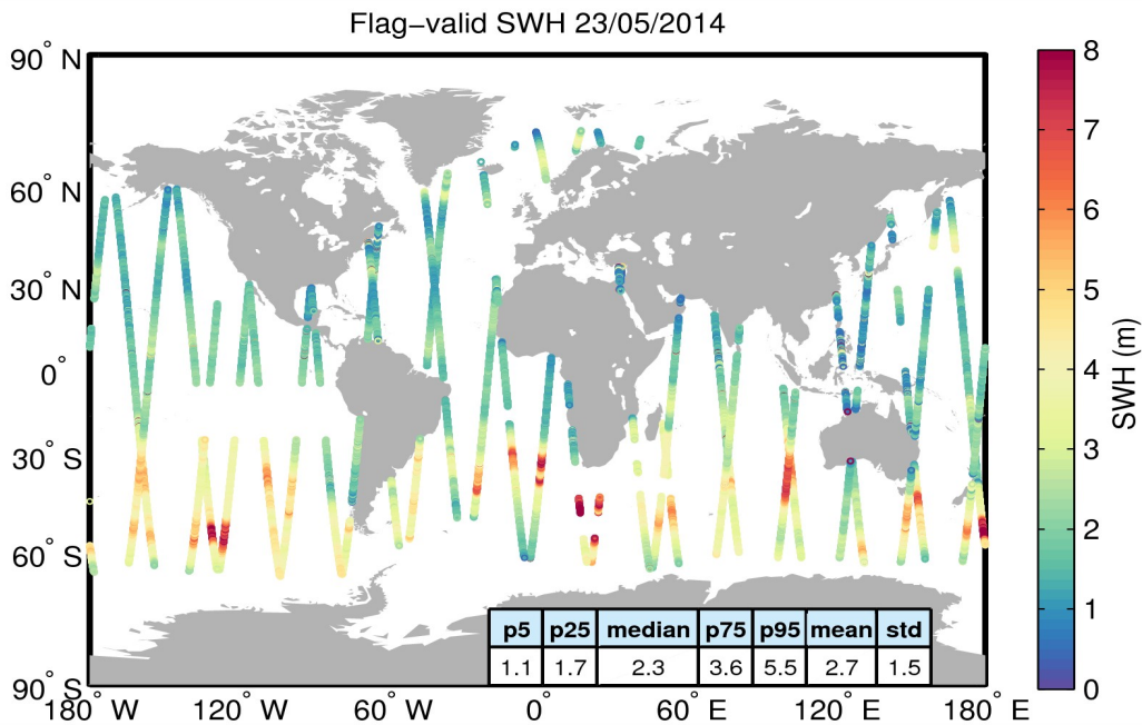
Figure 15. Geographical distribution of flag-valid SWH data over oceans and lakes for 23/05/2014. The statistical values shown in the table refer to the SWH in m and are calculated over all measurements shown in the figure.
