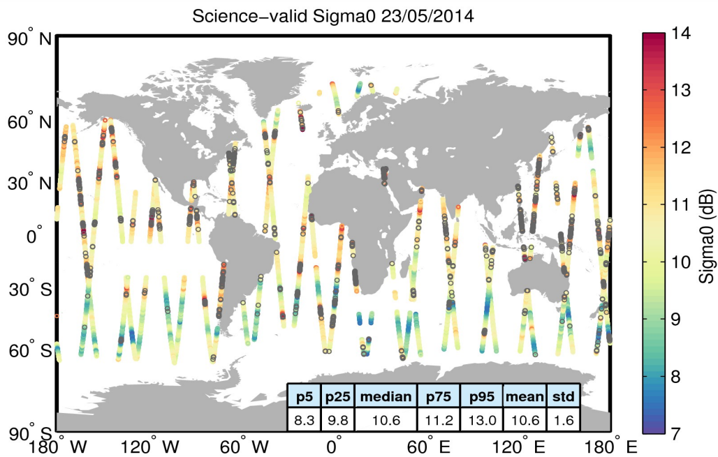
Figure 27. Geographical distribution of science-valid sigma0 data over oceans and lakes for 23/05/2014. The statistical values shown in the table refer to the sigma0 in dB and are calculated over all measurements shown in the figure. Gray circles denote records that have been rejected based on the editing criteria described in Table 4.
