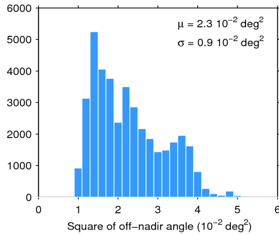
Figure 39. Histogram of flag-valid mispointing over oceans and lakes for 23/05/2014. The mean ( \mu ) and standard deviation ( \sigma ) are also shown. Note that values than 6 \cdot 10^{-2} \text{ deg}^2 are excluded from the histogram for the sake of readability but not from the computation of \mu and \sigma .
