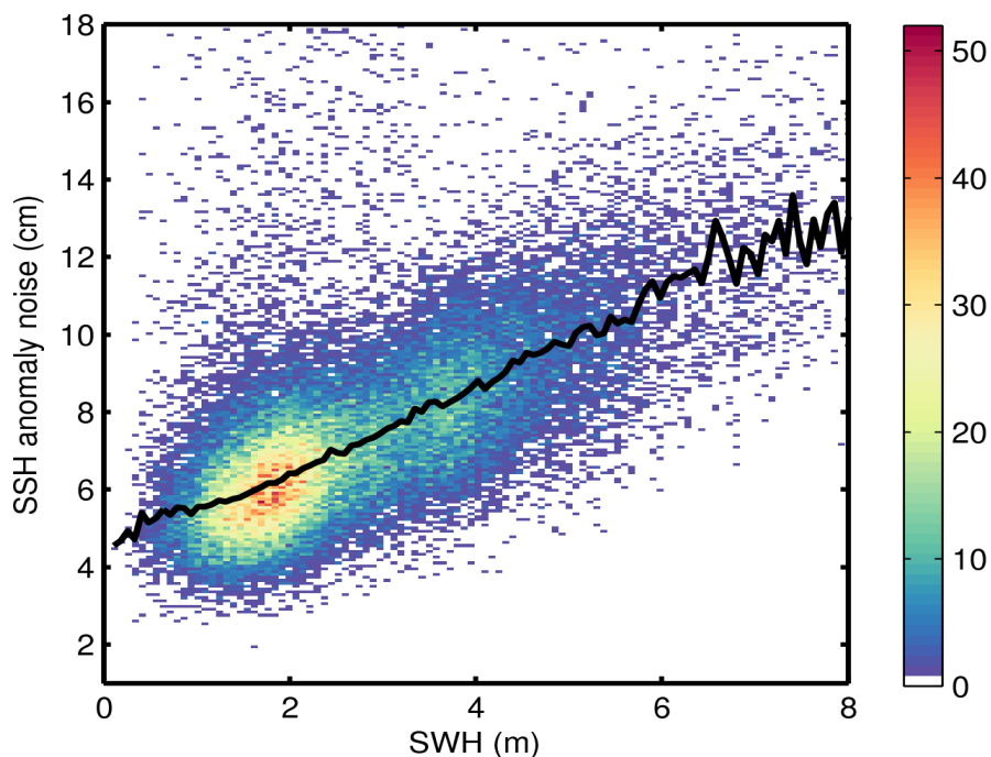
Figure 9. 2D histogram showing flag-valid SSH anomaly noise as a function of SWH for 23/05/2014. The black line denotes the median SSH anomaly as a function of SWH.
