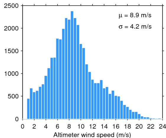
Figure 35. Histogram of science-valid wind over oceans and lakes for 23/05/2014. The mean ( \mu ) and standard deviation ( \sigma ) are also shown. Note that values larger than 24 m/s are excluded from the histogram for the sake of readability but not from the computation of \mu and \sigma .
