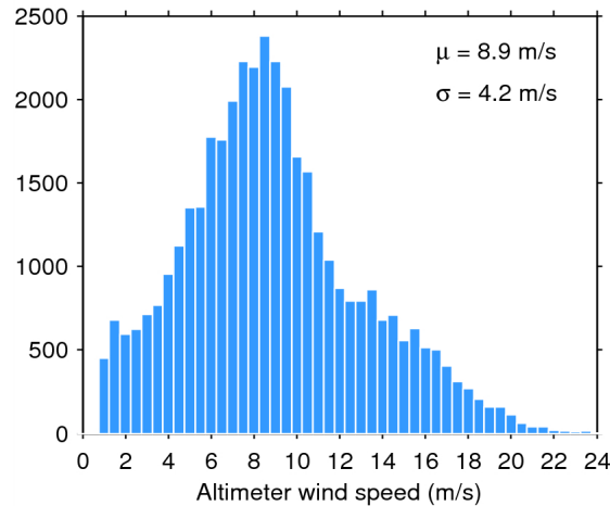
Figure 33. Histogram of flag-valid wind over oceans and lakes for 23/05/2014. The mean ( \mu ) and standard deviation ( \sigma ) are also shown. Note that values larger than 24 m/s are excluded from the histogram for the sake of readability but not from the computation of \mu and \sigma .
