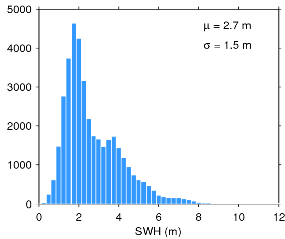
Figure 17. Histogram of flag-valid SWH over oceans and lakes for 23/05/2014. The mean ( \mu ) and standard deviation ( \sigma ) are also shown. Note that values larger than 12 m are excluded from the histogram for the sake of readability but not from the computation of \mu and \sigma .
