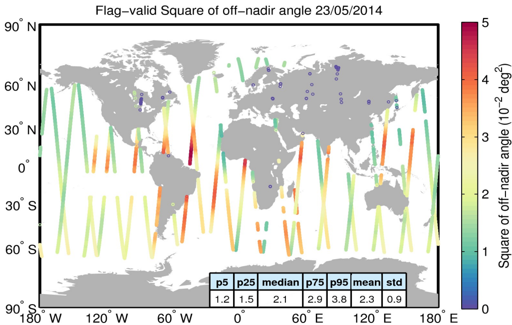
Figure 37. Geographical distribution of flag-valid mispointing data over oceans and lakes for 23/05/2014. The statistical values shown in the table refer to the mispointing in 10^{-2} deg 2 and are calculated over all measurements shown in the figure.
