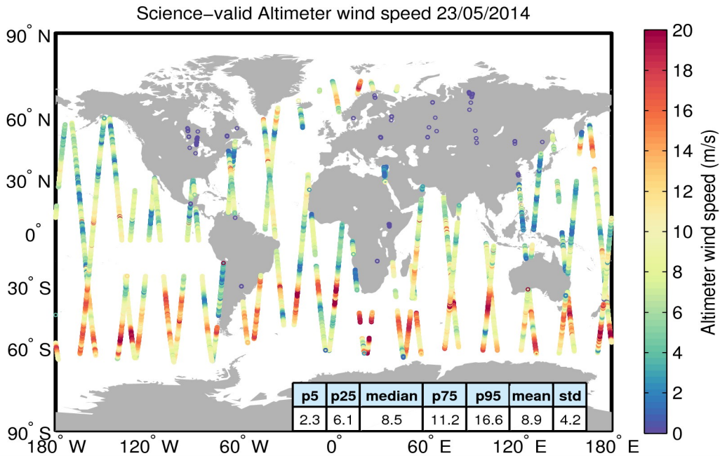
Figure 34. Geographical distribution of science-valid wind data over oceans and lakes for 23/05/2014. The statistical values shown in the table refer to the wind in m/s and are calculated over all measurements shown in the figure. Gray circles denote records that have been rejected based on the editing criteria described in Table 5.
