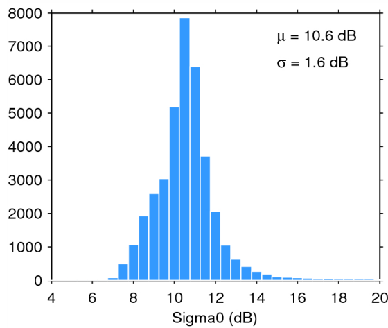
Figure 28. Histogram of science-valid sigma0 over oceans and lakes for 23/05/2014. The mean ( \mu ) and standard deviation ( \sigma ) are also shown. Note that values outside [4 20] dB are excluded from the histogram for the sake of readability but not from the computation of \mu and \sigma .
