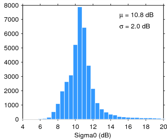
Figure 25. Histogram of flag-valid sigma0 over oceans and lakes for 23/05/2014. The mean ( \mu ) and standard deviation ( \sigma ) are also shown. Note that values outside [4 20] dB are excluded from the histogram for the sake of readability but not from the computation of \mu and \sigma .
