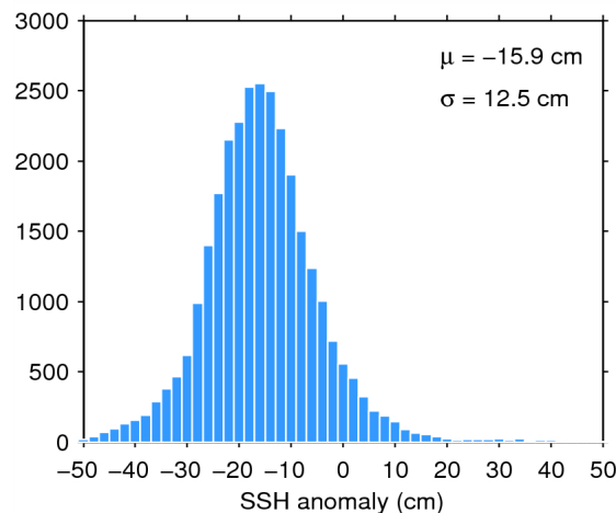
Figure 11. Histogram of science-valid SSH anomaly over oceans and lakes for 23/05/2014. The mean ( \mu ) and standard deviation ( \sigma ) are also shown. Note that values outside [-50 50] cm are excluded from the histogram for the sake of readability but not from the computation of \mu and \sigma .
