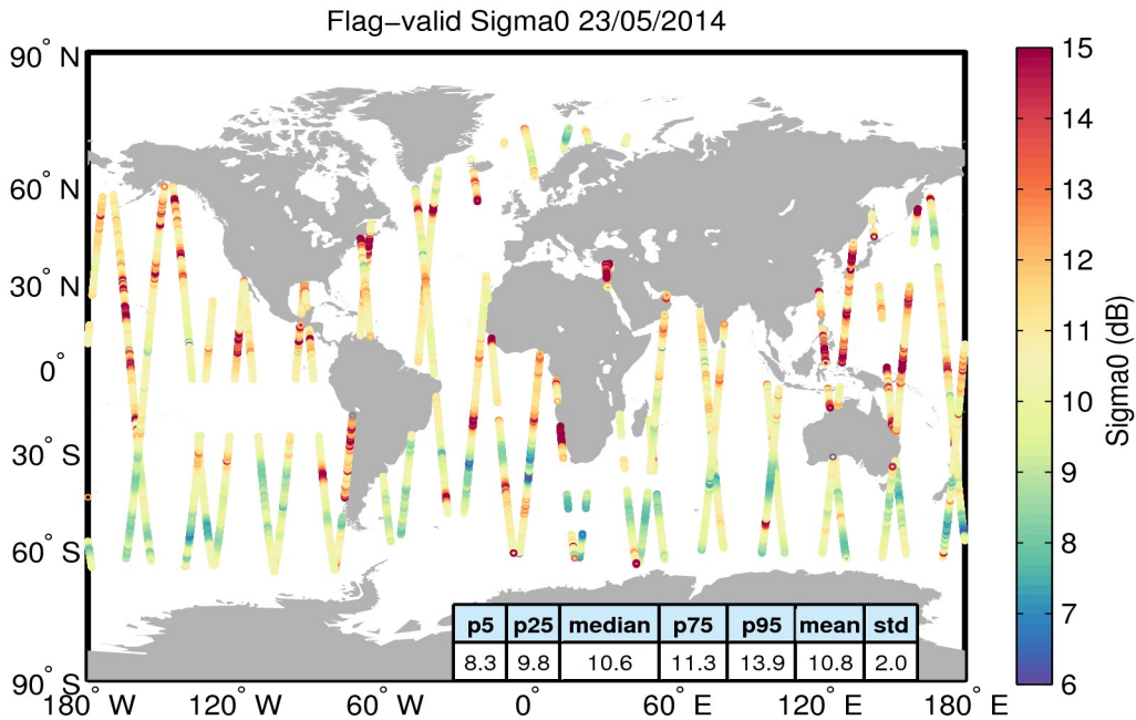
Figure 23. Geographical distribution of flag-valid sigma0 data over oceans and lakes for 23/05/2014. The statistical values shown in the table refer to the sigma0 in dB and are calculated over all measurements shown in the figure.
