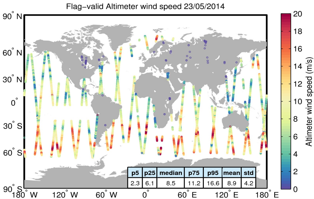
Figure 31. Geographical distribution of flag-valid wind data over oceans and lakes for 23/05/2014. The statistical values shown in the table refer to the wind in m/s and are calculated over all measurements shown in the figure.
