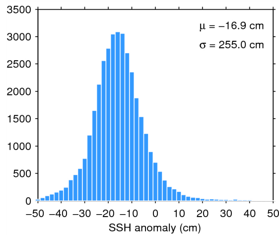
Figure 7. Histogram of flag-valid SSH anomaly over oceans and lakes for 23/05/2014. The mean ( \mu ) and standard deviation ( \sigma ) are also shown. Note that values outside [-50 50] cm are excluded from the histogram for the sake of readability but not from the computation of \mu and \sigma .
