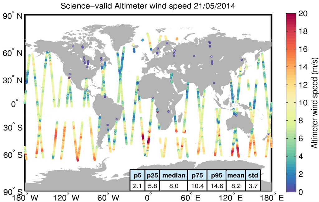
Figure 34. Geographical distribution of science-valid wind data over oceans and lakes for 21/05/2014. The statistical values shown in the table refer to the wind in m/s and are calculated over all measurements shown in the figure. Gray circles denote records that have been rejected based on the editing criteria described in Table 5.
