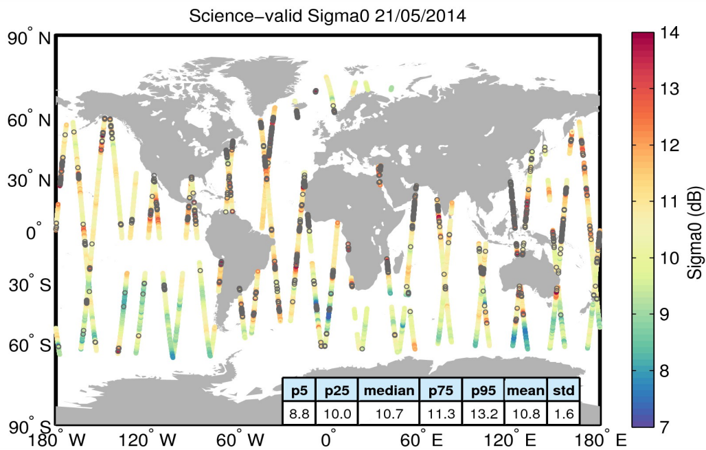
Figure 27. Geographical distribution of science-valid sigma0 data over oceans and lakes for 21/05/2014. The statistical values shown in the table refer to the sigma0 in dB and are calculated over all measurements shown in the figure. Gray circles denote records that have been rejected based on the editing criteria described in Table 4.
