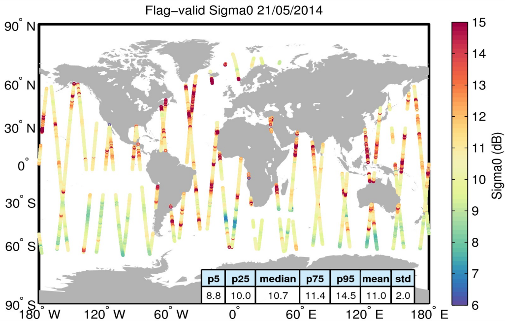
Figure 23. Geographical distribution of flag-valid sigma0 data over oceans and lakes for 21/05/2014. The statistical values shown in the table refer to the sigma0 in dB and are calculated over all measurements shown in the figure.
