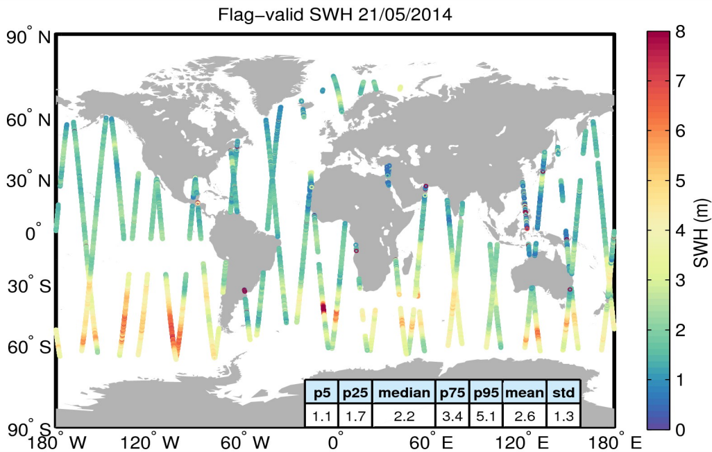
Figure 15. Geographical distribution of flag-valid SWH data over oceans and lakes for 21/05/2014. The statistical values shown in the table refer to the SWH in m and are calculated over all measurements shown in the figure.
