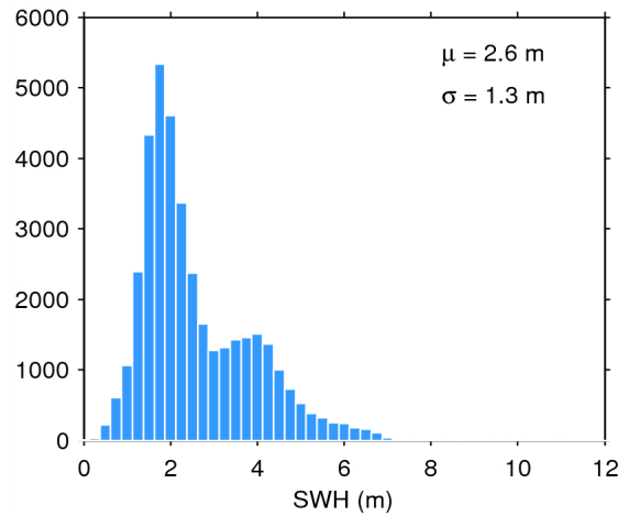
Figure 17. Histogram of flag-valid SWH over oceans and lakes for 21/05/2014. The mean ( \mu ) and standard deviation ( \sigma ) are also shown. Note that values larger than 12 m are excluded from the histogram for the sake of readability but not from the computation of \mu and \sigma .
