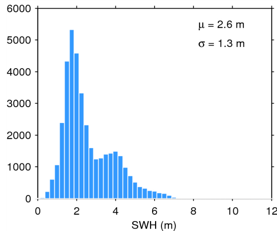
Figure 20. Histogram of science-valid SWH over oceans and lakes for 21/05/2014. The mean ( \mu ) and standard deviation ( \sigma ) are also shown. Note that values larger than 12 m are excluded from the histogram for the sake of readability but not from the computation of \mu and \sigma .
