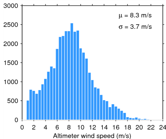
Figure 35. Histogram of science-valid wind over oceans and lakes for 20/05/2014. The mean ( \mu ) and standard deviation ( \sigma ) are also shown. Note that values larger than 24 m/s are excluded from the histogram for the sake of readability but not from the computation of \mu and \sigma .
