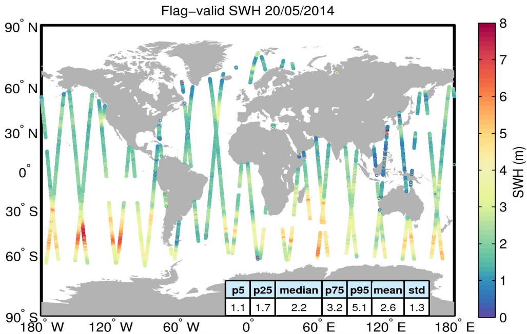
Figure 15. Geographical distribution of flag-valid SWH data over oceans and lakes for 20/05/2014. The statistical values shown in the table refer to the SWH in m and are calculated over all measurements shown in the figure.
