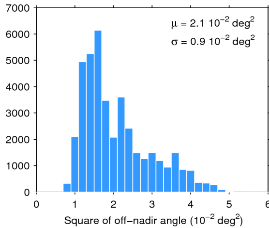
Figure 39. Histogram of flag-valid mispointing over oceans and lakes for 20/05/2014. The mean ( \mu ) and standard deviation ( \sigma ) are also shown. Note that values than 6 \cdot 10^{-2} \text{ deg}^2 are excluded from the histogram for the sake of readability but not from the computation of \mu and \sigma .
