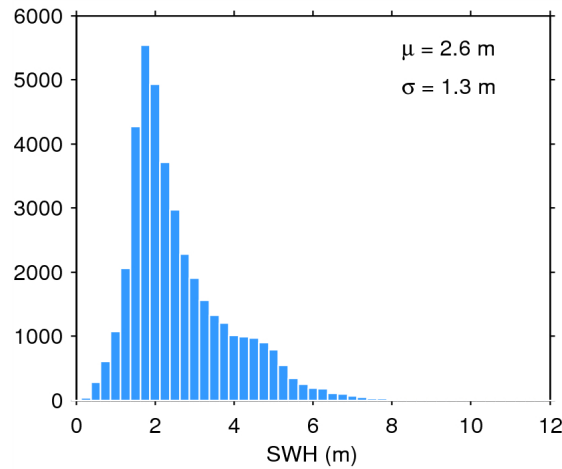
Figure 17. Histogram of flag-valid SWH over oceans and lakes for 20/05/2014. The mean ( \mu ) and standard deviation ( \sigma ) are also shown. Note that values larger than 12 m are excluded from the histogram for the sake of readability but not from the computation of \mu and \sigma .
