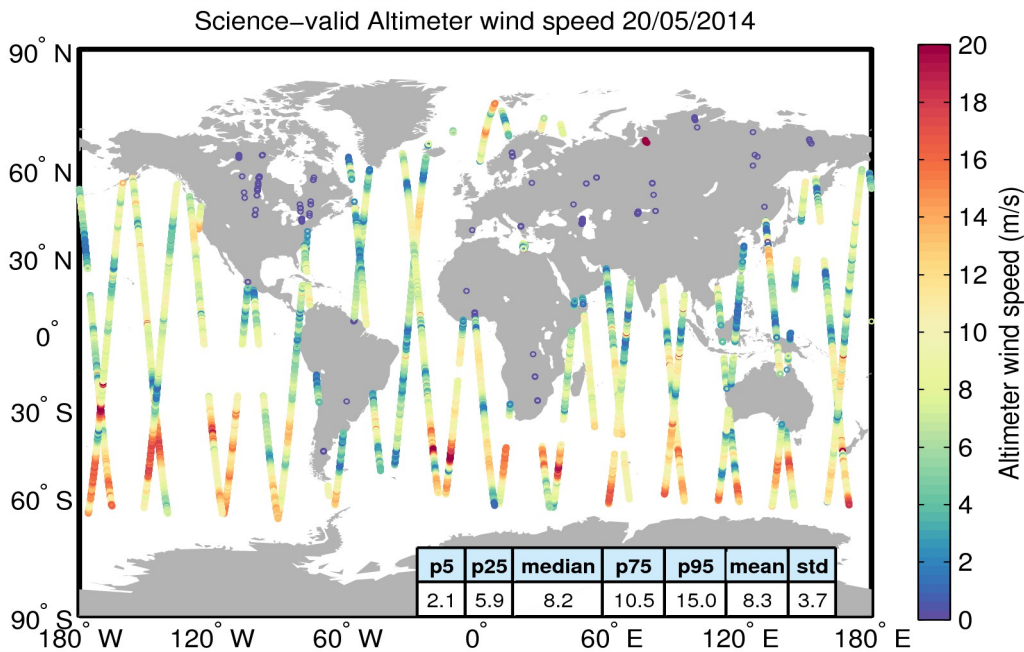
Figure 34. Geographical distribution of science-valid wind data over oceans and lakes for 20/05/2014. The statistical values shown in the table refer to the wind in m/s and are calculated over all measurements shown in the figure. Gray circles denote records that have been rejected based on the editing criteria described in Table 5.
