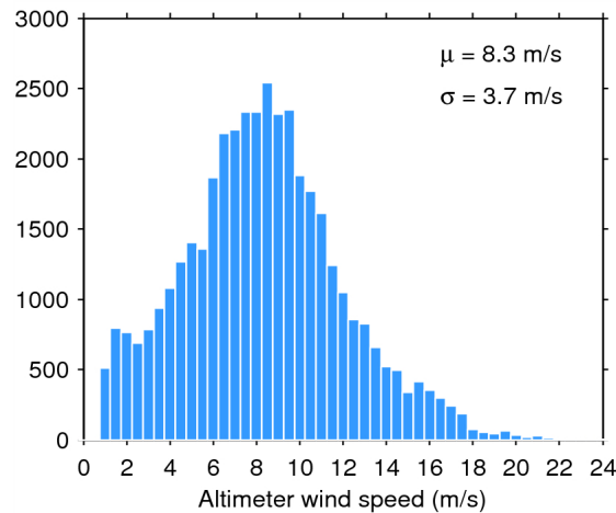
Figure 33. Histogram of flag-valid wind over oceans and lakes for 20/05/2014. The mean ( \mu ) and standard deviation ( \sigma ) are also shown. Note that values larger than 24 m/s are excluded from the histogram for the sake of readability but not from the computation of \mu and \sigma .
