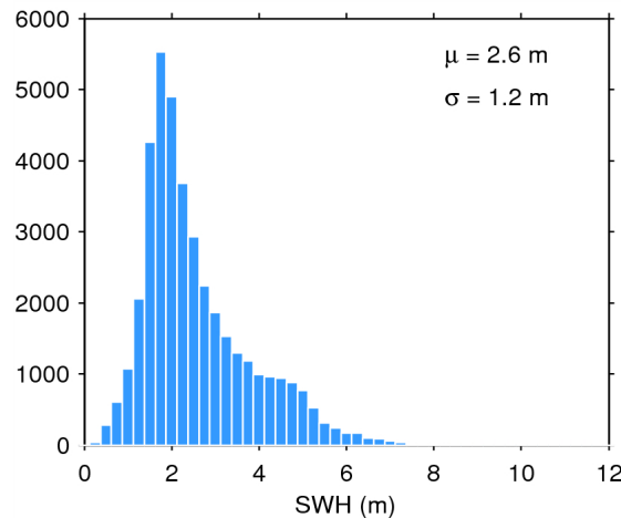
Figure 20. Histogram of science-valid SWH over oceans and lakes for 20/05/2014. The mean ( \mu ) and standard deviation ( \sigma ) are also shown. Note that values larger than 12 m are excluded from the histogram for the sake of readability but not from the computation of \mu and \sigma .
