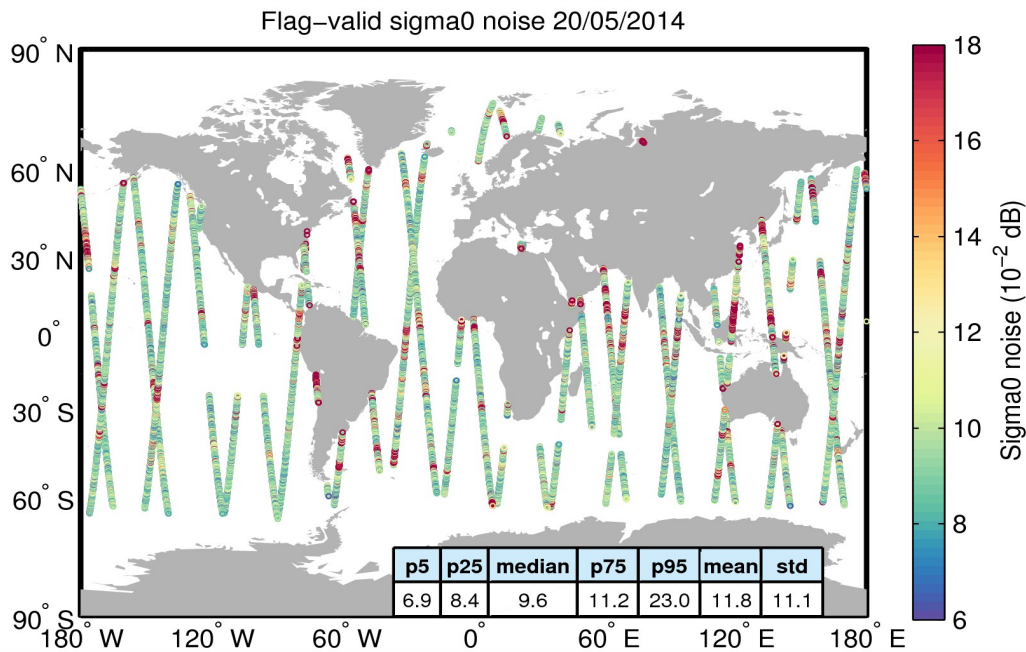
Figure 26. Geographical distribution of flag-valid 20-Hz sigma0 measurement noise over oceans and lakes for 20/05/2014. The statistical values shown in the table refer to the sigma0 noise and are calculated over all measurements shown in the figure.
