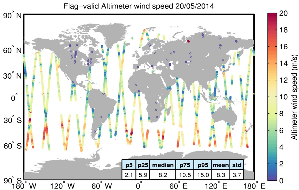
Figure 31. Geographical distribution of flag-valid wind data over oceans and lakes for 20/05/2014. The statistical values shown in the table refer to the wind in m/s and are calculated over all measurements shown in the figure.
