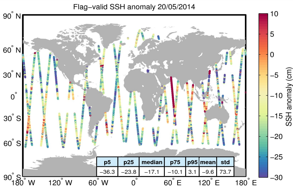
Figure 5. Geographical distribution of flag-valid 1-Hz SSH anomaly data over oceans and lakes for 20/05/2014. The statistical values shown in the table refer to the SSH anomaly in cm and are calculated over all measurements shown in the figure.
