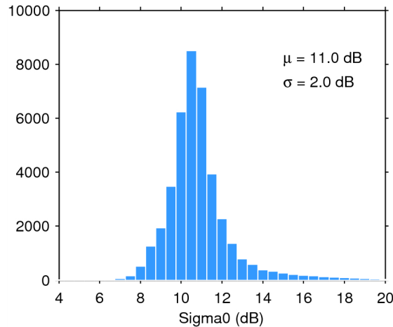
Figure 25. Histogram of flag-valid sigma0 over oceans and lakes for 20/05/2014. The mean ( \mu ) and standard deviation ( \sigma ) are also shown. Note that values outside [4 20] dB are excluded from the histogram for the sake of readability but not from the computation of \mu and \sigma .
