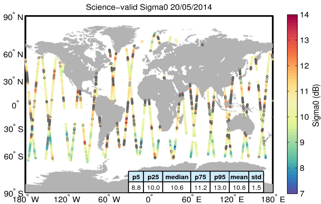
Figure 27. Geographical distribution of science-valid sigma0 data over oceans and lakes for 20/05/2014. The statistical values shown in the table refer to the sigma0 in dB and are calculated over all measurements shown in the figure. Gray circles denote records that have been rejected based on the editing criteria described in Table 4.
