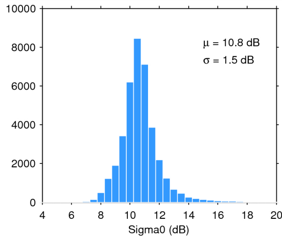
Figure 28. Histogram of science-valid sigma0 over oceans and lakes for 20/05/2014. The mean ( \mu ) and standard deviation ( \sigma ) are also shown. Note that values outside [4 20] dB are excluded from the histogram for the sake of readability but not from the computation of \mu and \sigma .
