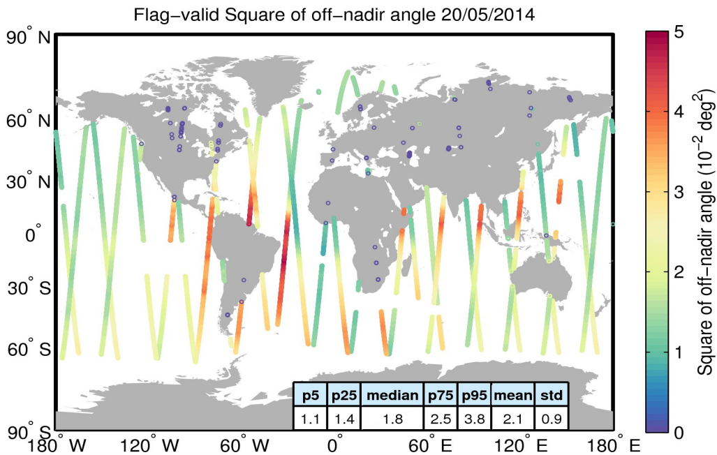
Figure 37. Geographical distribution of flag-valid mispointing data over oceans and lakes for 20/05/2014. The statistical values shown in the table refer to the mispointing in 10^{-2} \text{ deg}^2 and are calculated over all measurements shown in the figure.
