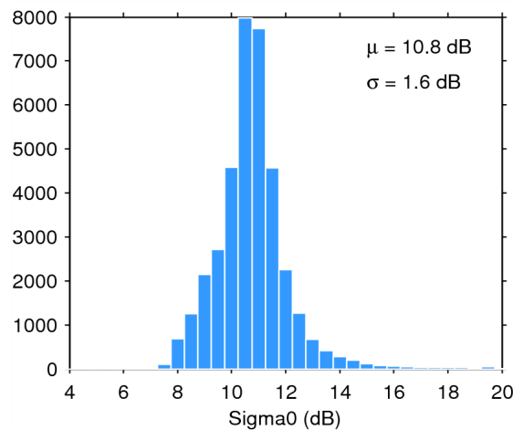
Figure 28. Histogram of science-valid sigma0 over oceans and lakes for 19/05/2014. The mean ( \mu ) and standard deviation ( \sigma ) are also shown. Note that values outside [4 20] dB are excluded from the histogram for the sake of readability but not from the computation of \mu and \sigma .
