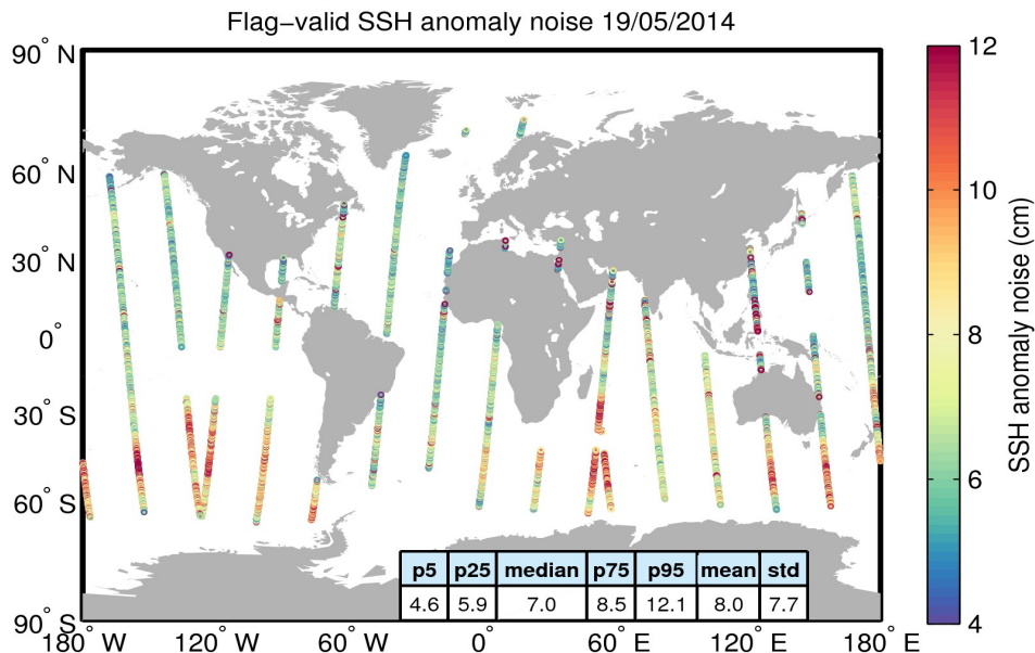
Figure 8. Geographical distribution of flag-valid 20-Hz SSH anomaly measurement noise over oceans and lakes for 19/05/2014. The statistical values shown in the table refer to the SSH anomaly noise and are calculated over all measurements shown in the figure.
