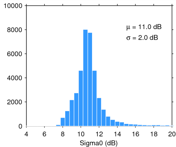
Figure 25. Histogram of flag-valid sigma0 over oceans and lakes for 19/05/2014. The mean ( \mu ) and standard deviation ( \sigma ) are also shown. Note that values outside [4 20] dB are excluded from the histogram for the sake of readability but not from the computation of \mu and \sigma .
