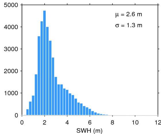
Figure 20. Histogram of science-valid SWH over oceans and lakes for 19/05/2014. The mean ( \mu ) and standard deviation ( \sigma ) are also shown. Note that values larger than 12 m are excluded from the histogram for the sake of readability but not from the computation of \mu and \sigma .
