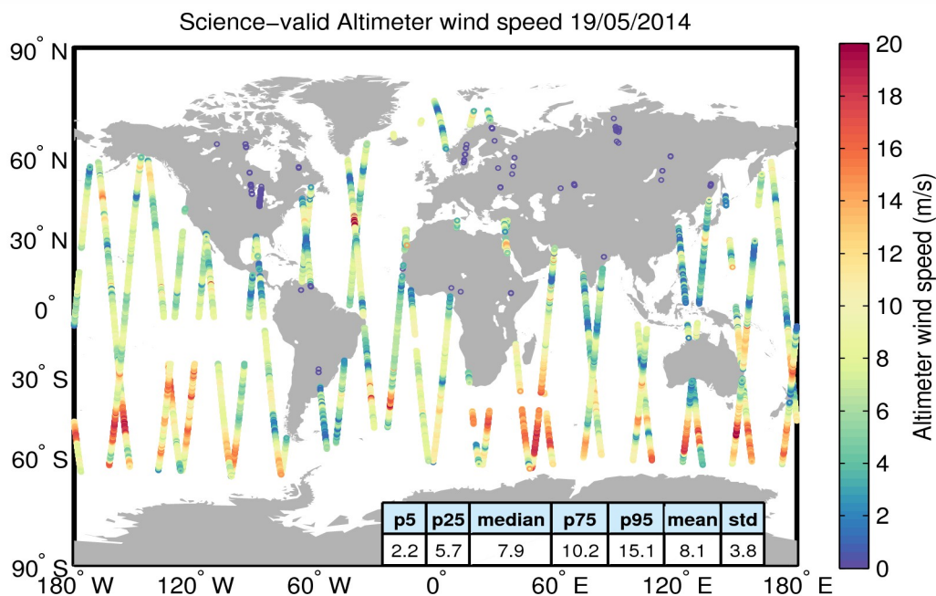
Figure 34. Geographical distribution of science-valid wind data over oceans and lakes for 19/05/2014. The statistical values shown in the table refer to the wind in m/s and are calculated over all measurements shown in the figure. Gray circles denote records that have been rejected based on the editing criteria described in Table 5.
