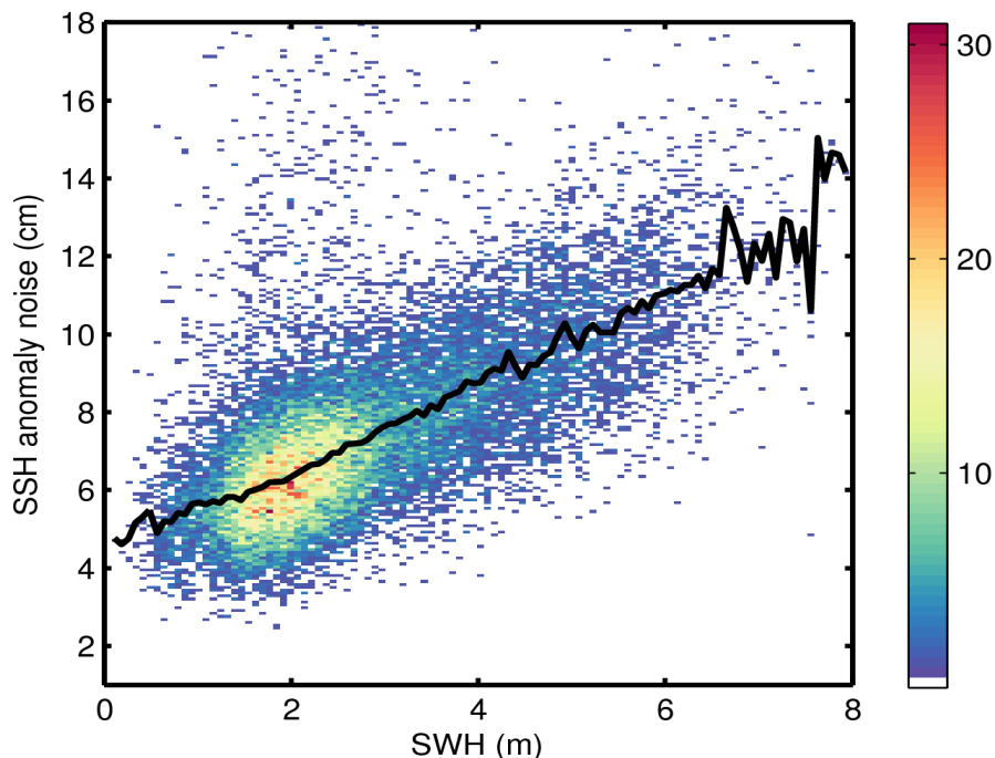
Figure 9. 2D histogram showing flag-valid SSH anomaly noise as a function of SWH for 19/05/2014. The black line denotes the median SSH anomaly as a function of SWH.
