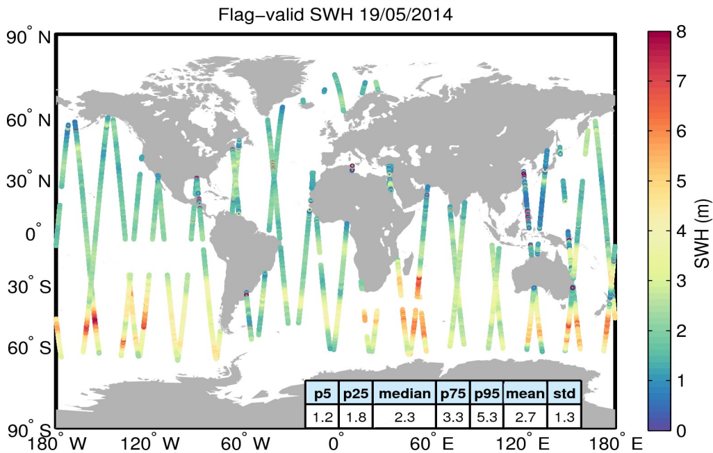
Figure 15. Geographical distribution of flag-valid SWH data over oceans and lakes for 19/05/2014. The statistical values shown in the table refer to the SWH in m and are calculated over all measurements shown in the figure.
