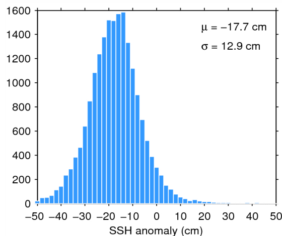
Figure 11. Histogram of science-valid SSH anomaly over oceans and lakes for 19/05/2014. The mean ( \mu ) and standard deviation ( \sigma ) are also shown. Note that values outside [-50 50] cm are excluded from the histogram for the sake of readability but not from the computation of \mu and \sigma .
