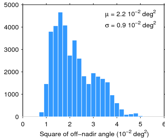
Figure 39. Histogram of flag-valid mispointing over oceans and lakes for 19/05/2014. The mean ( \mu ) and standard deviation ( \sigma ) are also shown. Note that values than 6 \cdot 10^{-2} \text{ deg}^2 are excluded from the histogram for the sake of readability but not from the computation of \mu and \sigma .
