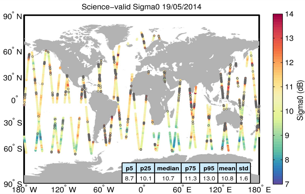
Figure 27. Geographical distribution of science-valid sigma0 data over oceans and lakes for 19/05/2014. The statistical values shown in the table refer to the sigma0 in dB and are calculated over all measurements shown in the figure. Gray circles denote records that have been rejected based on the editing criteria described in Table 4.
