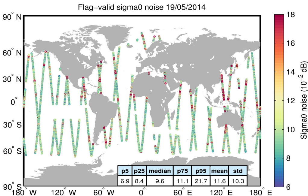
Figure 26. Geographical distribution of flag-valid 20-Hz sigma0 measurement noise over oceans and lakes for 19/05/2014. The statistical values shown in the table refer to the sigma0 noise and are calculated over all measurements shown in the figure.
