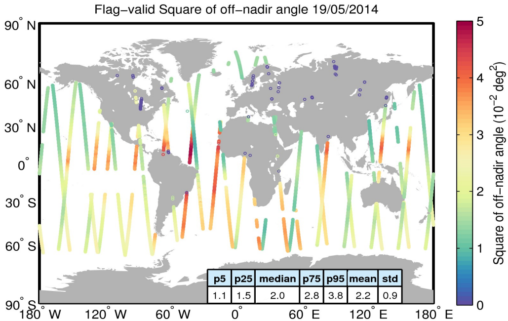
Figure 37. Geographical distribution of flag-valid mispointing data over oceans and lakes for 19/05/2014. The statistical values shown in the table refer to the mispointing in 10^{-2} \text{deg}^2 and are calculated over all measurements shown in the figure.
