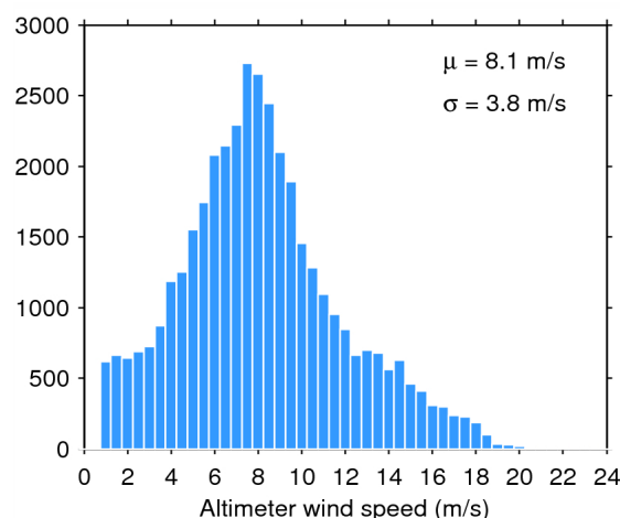
Figure 35. Histogram of science-valid wind over oceans and lakes for 19/05/2014. The mean ( \mu ) and standard deviation ( \sigma ) are also shown. Note that values larger than 24 m/s are excluded from the histogram for the sake of readability but not from the computation of \mu and \sigma .
