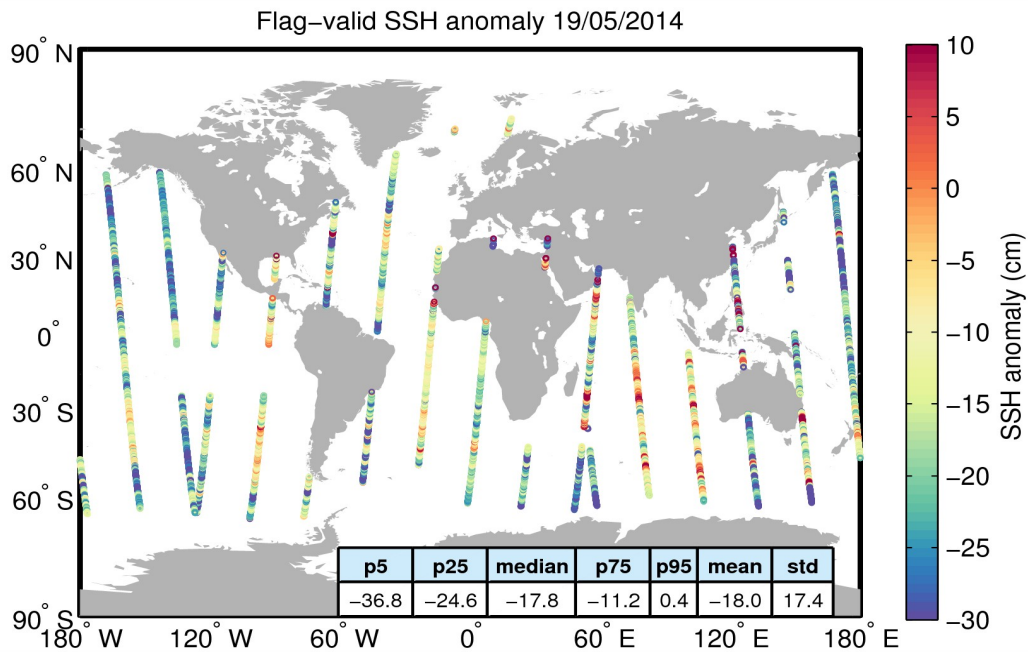
Figure 5. Geographical distribution of flag-valid 1-Hz SSH anomaly data over oceans and lakes for 19/05/2014. The statistical values shown in the table refer to the SSH anomaly in cm and are calculated over all measurements shown in the figure.
