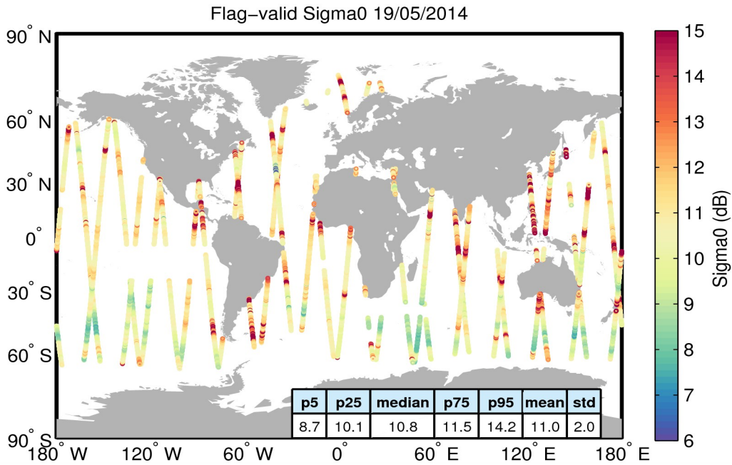
Figure 23. Geographical distribution of flag-valid sigma0 data over oceans and lakes for 19/05/2014. The statistical values shown in the table refer to the sigma0 in dB and are calculated over all measurements shown in the figure.
