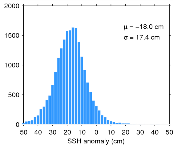
Figure 7. Histogram of flag-valid SSH anomaly over oceans and lakes for 19/05/2014. The mean ( \mu ) and standard deviation ( \sigma ) are also shown. Note that values outside [-50\ 50] cm are excluded from the histogram for the sake of readability but not from the computation of \mu and \sigma .
