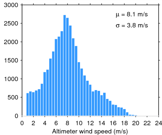
Figure 33. Histogram of flag-valid wind over oceans and lakes for 19/05/2014. The mean ( \mu ) and standard deviation ( \sigma ) are also shown. Note that values larger than 24 m/s are excluded from the histogram for the sake of readability but not from the computation of \mu and \sigma .
