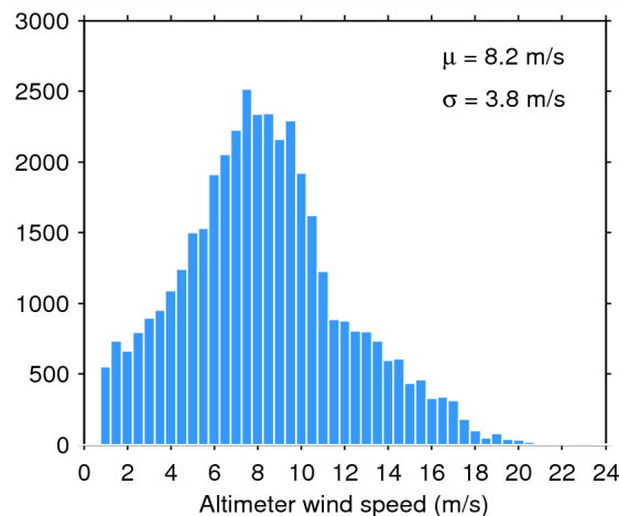
Figure 35. Histogram of science-valid wind over oceans and lakes for 18/05/2014. The mean ( \mu ) and standard deviation ( \sigma ) are also shown. Note that values larger than 24 m/s are excluded from the histogram for the sake of readability but not from the computation of \mu and \sigma .
