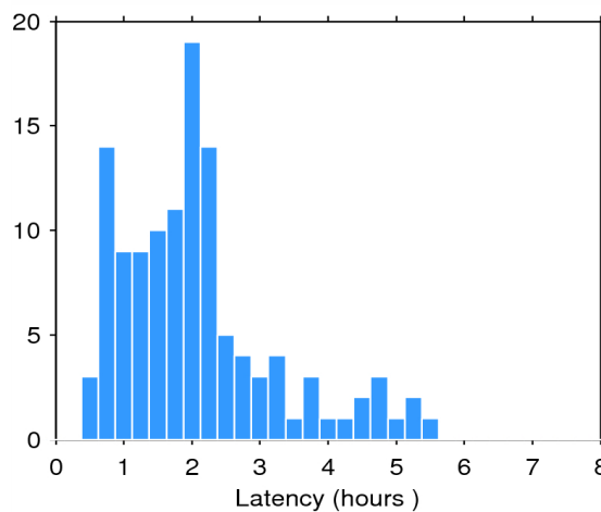
Figure 2. Histogram of the data latency for 18/05/2014. The y-axis denotes the number of files that are made available with a delay of x-hours with respect to the mean time of the records stored in the file.
