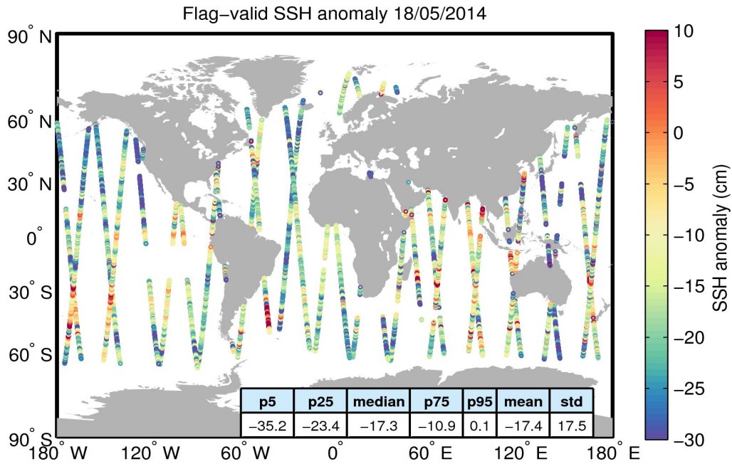
Figure 5. Geographical distribution of flag-valid 1-Hz SSH anomaly data over oceans and lakes for 18/05/2014. The statistical values shown in the table refer to the SSH anomaly in cm and are calculated over all measurements shown in the figure.
