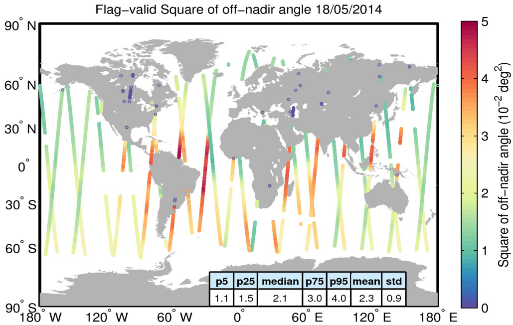
Figure 37. Geographical distribution of flag-valid mispointing data over oceans and lakes for 18/05/2014. The statistical values shown in the table refer to the mispointing in 10^{-2} \text{ deg}^2 and are calculated over all measurements shown in the figure.
