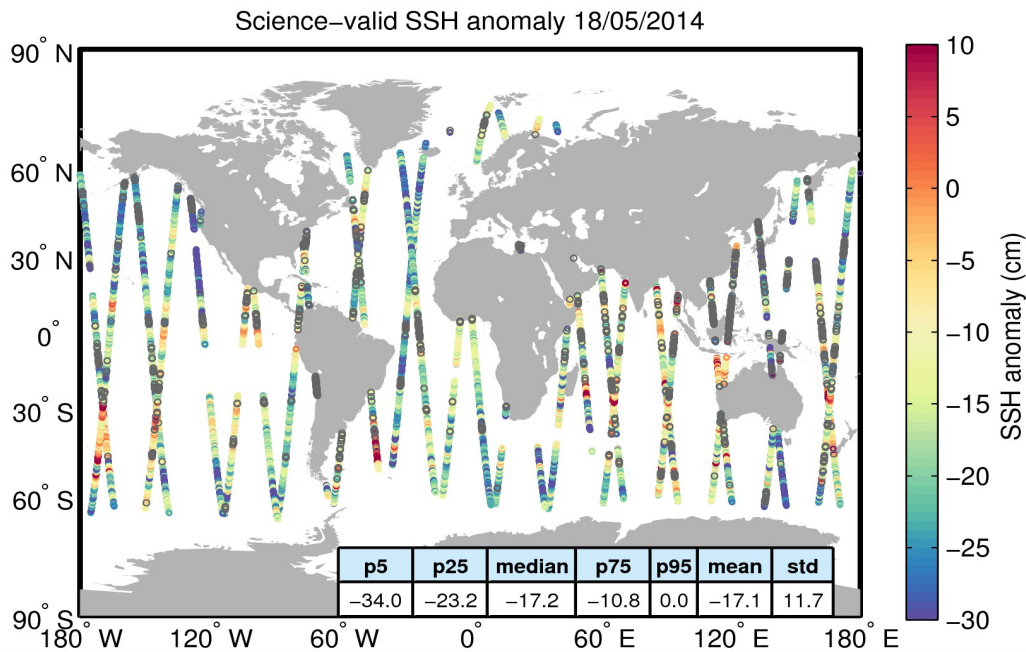
Figure 10. Geographical distribution of science-valid SSH anomaly data over oceans and lakes for 18/05/2014. The statistical values shown in the table refer to the SSH anomaly in cm and are calculated over all measurements shown in the figure. Gray circles denote records that have been rejected based on the editing criteria described in Table 2.
