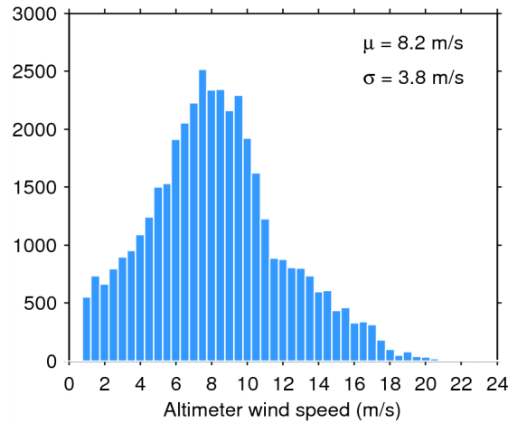
Figure 33. Histogram of flag-valid wind over oceans and lakes for 18/05/2014. The mean ( \mu ) and standard deviation ( \sigma ) are also shown. Note that values larger than 24 m/s are excluded from the histogram for the sake of readability but not from the computation of \mu and \sigma .
