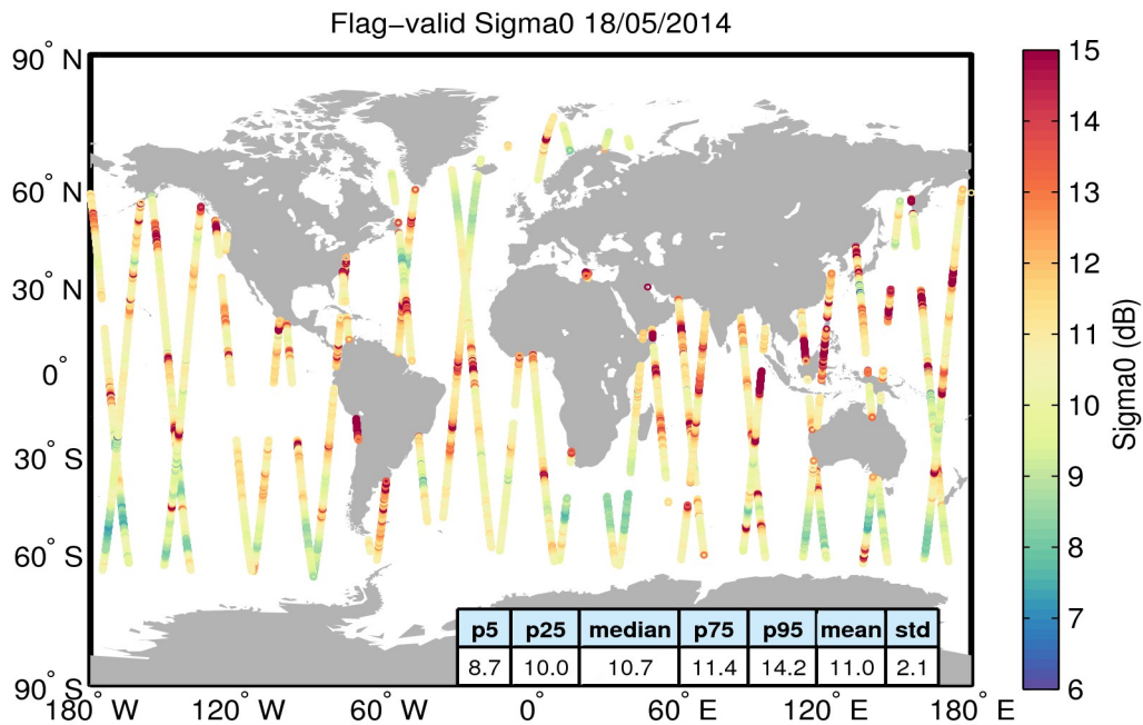
Figure 23. Geographical distribution of flag-valid sigma0 data over oceans and lakes for 18/05/2014. The statistical values shown in the table refer to the sigma0 in dB and are calculated over all measurements shown in the figure.
