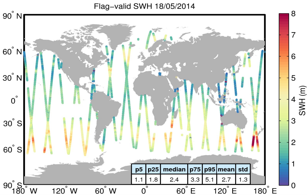
Figure 15. Geographical distribution of flag-valid SWH data over oceans and lakes for 18/05/2014. The statistical values shown in the table refer to the SWH in m and are calculated over all measurements shown in the figure.
