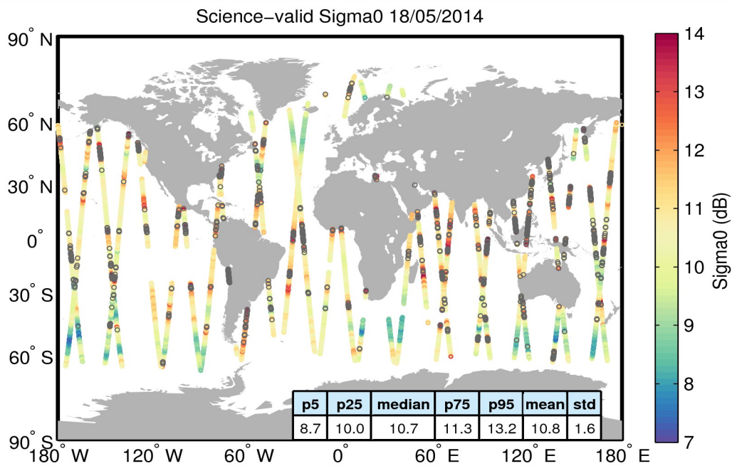
Figure 27. Geographical distribution of science-valid sigma0 data over oceans and lakes for 18/05/2014. The statistical values shown in the table refer to the sigma0 in dB and are calculated over all measurements shown in the figure. Gray circles denote records that have been rejected based on the editing criteria described in Table 4.
