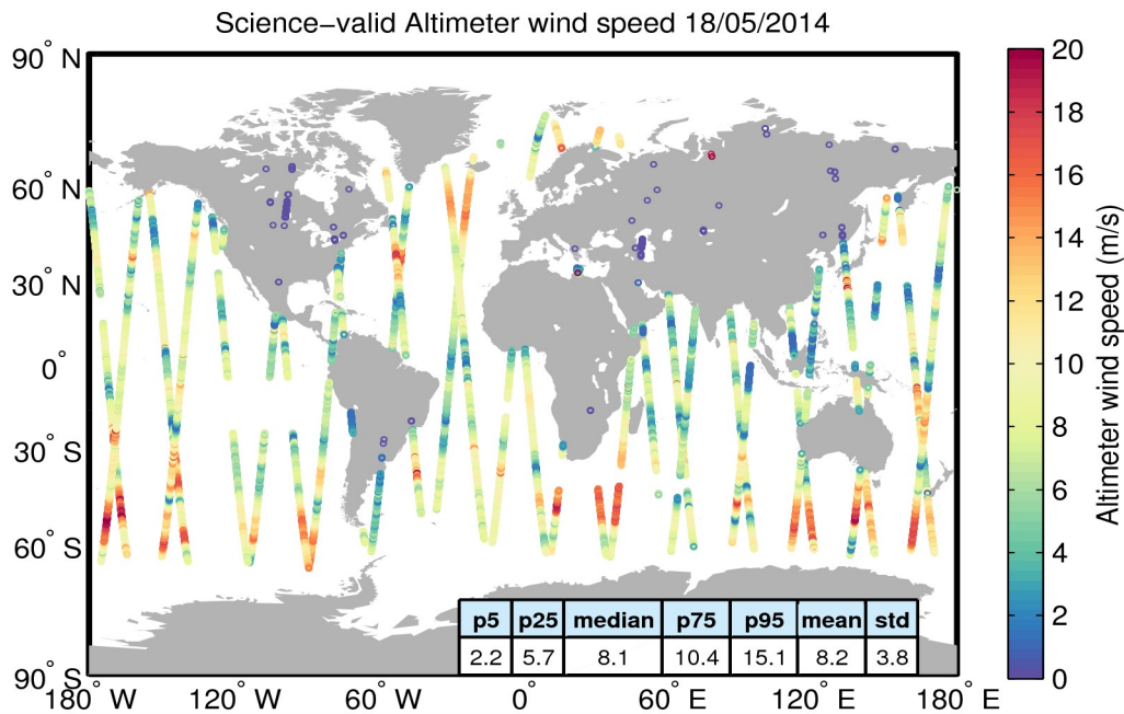
Figure 34. Geographical distribution of science-valid wind data over oceans and lakes for 18/05/2014. The statistical values shown in the table refer to the wind in m/s and are calculated over all measurements shown in the figure. Gray circles denote records that have been rejected based on the editing criteria described in Table 5.
