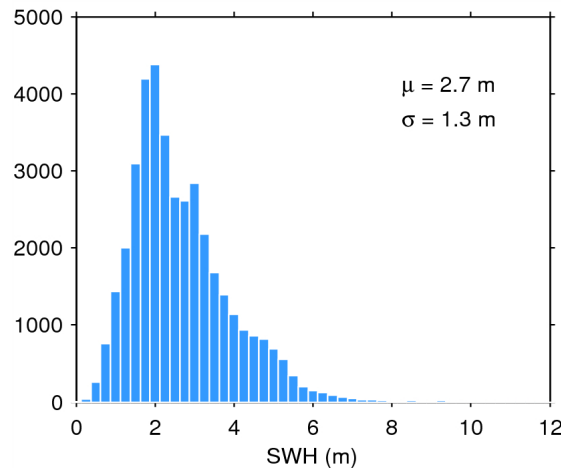
Figure 20. Histogram of science-valid SWH over oceans and lakes for 18/05/2014. The mean ( \mu ) and standard deviation ( \sigma ) are also shown. Note that values larger than 12 m are excluded from the histogram for the sake of readability but not from the computation of \mu and \sigma .
