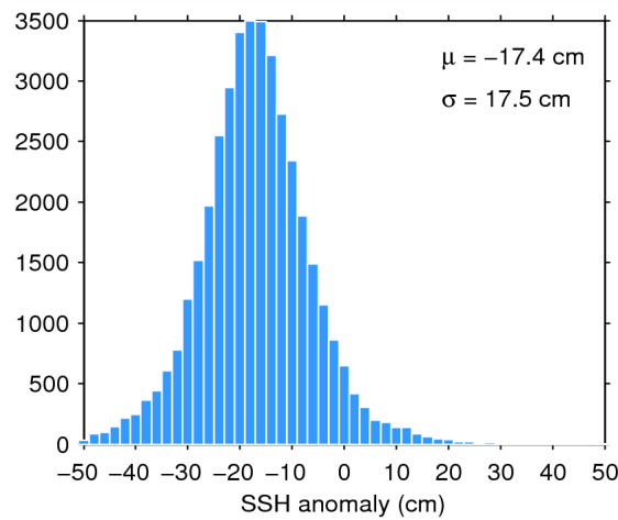
Figure 7. Histogram of flag-valid SSH anomaly over oceans and lakes for 18/05/2014. The mean ( \mu ) and standard deviation ( \sigma ) are also shown. Note that values outside [-50\ 50] cm are excluded from the histogram for the sake of readability but not from the computation of \mu and \sigma .
