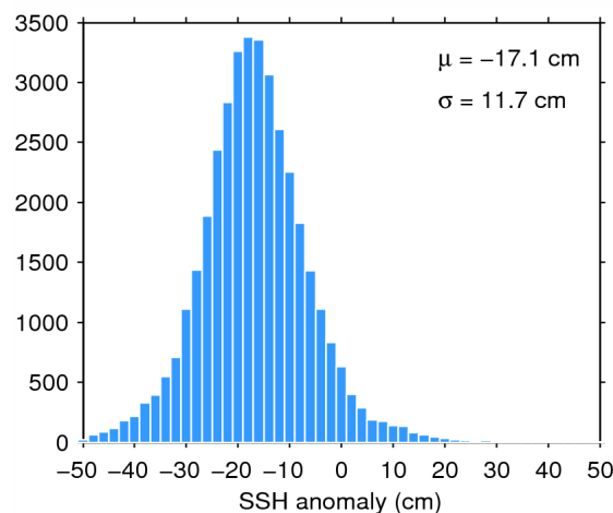
Figure 11. Histogram of science-valid SSH anomaly over oceans and lakes for 18/05/2014. The mean ( \mu ) and standard deviation ( \sigma ) are also shown. Note that values outside [-50 50] cm are excluded from the histogram for the sake of readability but not from the computation of \mu and \sigma .
