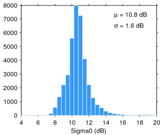
Figure 28. Histogram of science-valid sigma0 over oceans and lakes for 18/05/2014. The mean ( \mu ) and standard deviation ( \sigma ) are also shown. Note that values outside [4 20] dB are excluded from the histogram for the sake of readability but not from the computation of \mu and \sigma .
