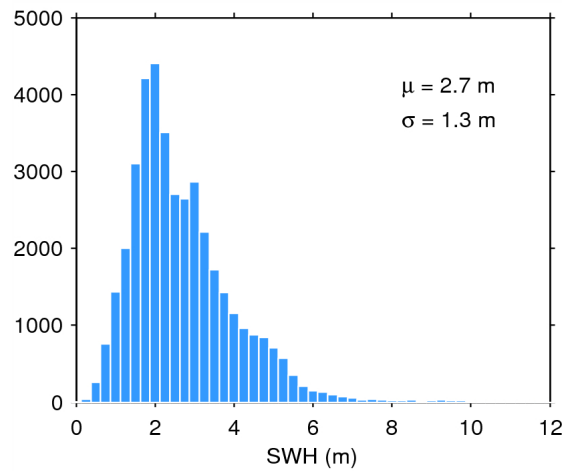
Figure 17. Histogram of flag-valid SWH over oceans and lakes for 18/05/2014. The mean ( \mu ) and standard deviation ( \sigma ) are also shown. Note that values larger than 12 m are excluded from the histogram for the sake of readability but not from the computation of \mu and \sigma .
