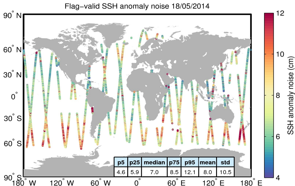
Figure 8. Geographical distribution of flag-valid 20-Hz SSH anomaly measurement noise over oceans and lakes for 18/05/2014. The statistical values shown in the table refer to the SSH anomaly noise and are calculated over all measurements shown in the figure.
