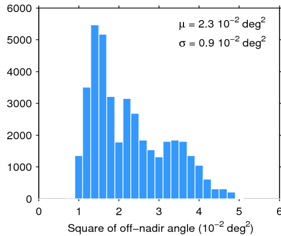
Figure 39. Histogram of flag-valid mispointing over oceans and lakes for 18/05/2014. The mean ( \mu ) and standard deviation ( \sigma ) are also shown. Note that values than 6 \cdot 10^{-2} \text{ deg}^2 are excluded from the histogram for the sake of readability but not from the computation of \mu and \sigma .
