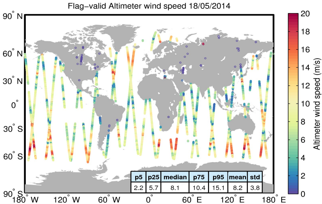
Figure 31. Geographical distribution of flag-valid wind data over oceans and lakes for 18/05/2014. The statistical values shown in the table refer to the wind in m/s and are calculated over all measurements shown in the figure.
