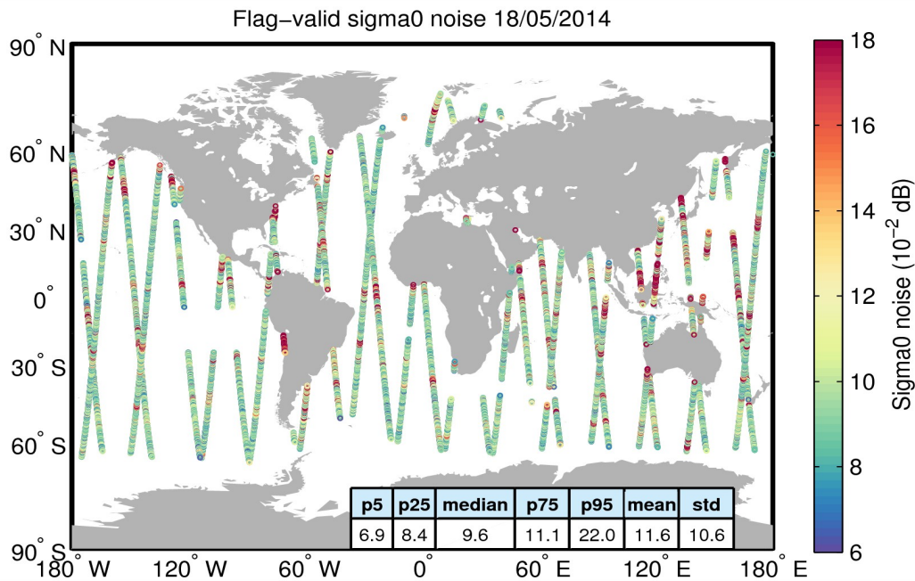
Figure 26. Geographical distribution of flag-valid 20-Hz sigma0 measurement noise over oceans and lakes for 18/05/2014. The statistical values shown in the table refer to the sigma0 noise and are calculated over all measurements shown in the figure.
