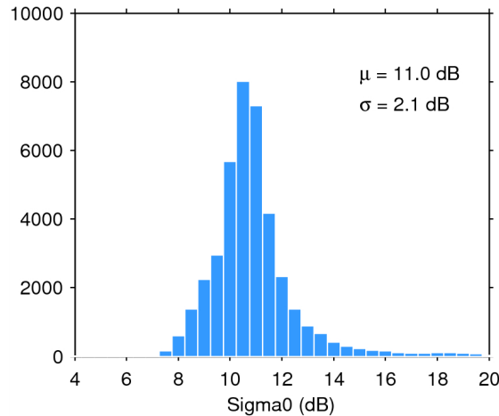
Figure 25. Histogram of flag-valid sigma0 over oceans and lakes for 18/05/2014. The mean ( \mu ) and standard deviation ( \sigma ) are also shown. Note that values outside [4 20] dB are excluded from the histogram for the sake of readability but not from the computation of \mu and \sigma .
