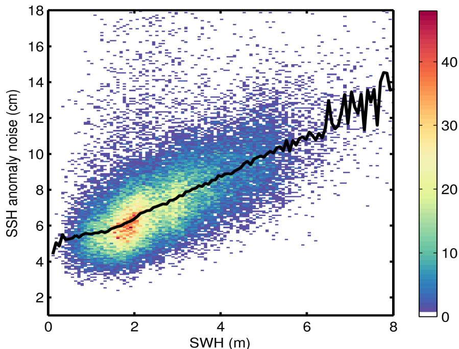
Figure 9. 2D histogram showing flag-valid SSH anomaly noise as a function of SWH for 18/05/2014. The black line denotes the median SSH anomaly as a function of SWH.
