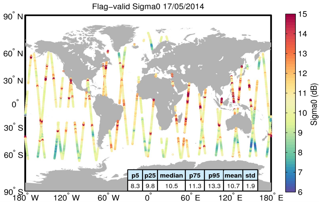
Figure 23. Geographical distribution of flag-valid sigma0 data over oceans and lakes for 17/05/2014. The statistical values shown in the table refer to the sigma0 in dB and are calculated over all measurements shown in the figure.
