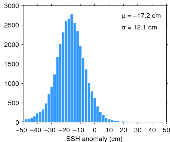
Figure 11. Histogram of science-valid SSH anomaly over oceans and lakes for 17/05/2014. The mean ( \mu ) and standard deviation ( \sigma ) are also shown. Note that values outside [-50 50] cm are excluded from the histogram for the sake of readability but not from the computation of \mu and \sigma .
