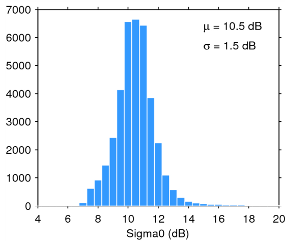
Figure 28. Histogram of science-valid sigma0 over oceans and lakes for 17/05/2014. The mean ( \mu ) and standard deviation ( \sigma ) are also shown. Note that values outside [4 20] dB are excluded from the histogram for the sake of readability but not from the computation of \mu and \sigma .
