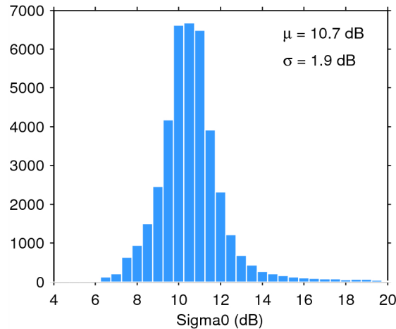
Figure 25. Histogram of flag-valid sigma0 over oceans and lakes for 17/05/2014. The mean ( \mu ) and standard deviation ( \sigma ) are also shown. Note that values outside [4 20] dB are excluded from the histogram for the sake of readability but not from the computation of \mu and \sigma .
