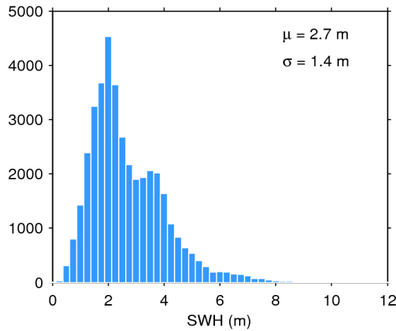
Figure 17. Histogram of flag-valid SWH over oceans and lakes for 17/05/2014. The mean ( \mu ) and standard deviation ( \sigma ) are also shown. Note that values larger than 12 m are excluded from the histogram for the sake of readability but not from the computation of \mu and \sigma .
