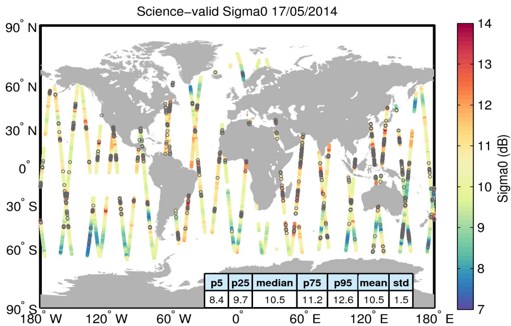
Figure 27. Geographical distribution of science-valid sigma0 data over oceans and lakes for 17/05/2014. The statistical values shown in the table refer to the sigma0 in dB and are calculated over all measurements shown in the figure. Gray circles denote records that have been rejected based on the editing criteria described in Table 4.
