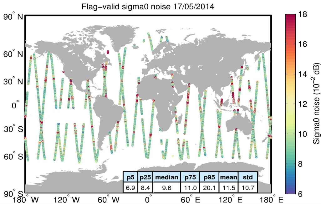
Figure 26. Geographical distribution of flag-valid 20-Hz sigma0 measurement noise over oceans and lakes for 17/05/2014. The statistical values shown in the table refer to the sigma0 noise and are calculated over all measurements shown in the figure.
