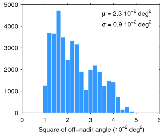
Figure 39. Histogram of flag-valid mispointing over oceans and lakes for 17/05/2014. The mean ( \mu ) and standard deviation ( \sigma ) are also shown. Note that values than 6 \cdot 10^{-2} \text{ deg}^2 are excluded from the histogram for the sake of readability but not from the computation of \mu and \sigma .
