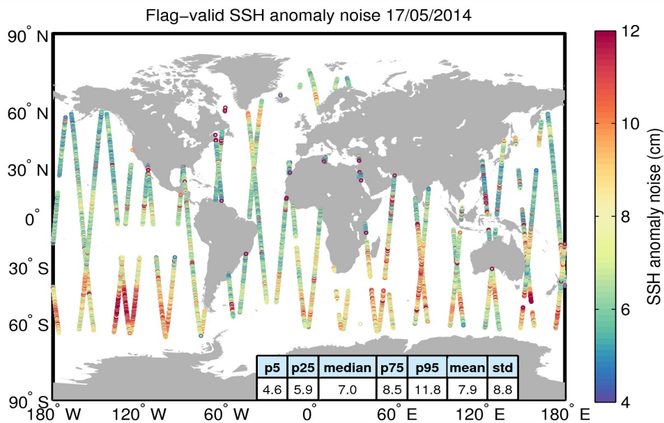
Figure 8. Geographical distribution of flag-valid 20-Hz SSH anomaly measurement noise over oceans and lakes for 17/05/2014. The statistical values shown in the table refer to the SSH anomaly noise and are calculated over all measurements shown in the figure.
