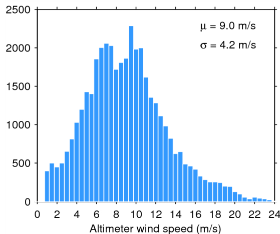
Figure 35. Histogram of science-valid wind over oceans and lakes for 17/05/2014. The mean ( \mu ) and standard deviation ( \sigma ) are also shown. Note that values larger than 24 m/s are excluded from the histogram for the sake of readability but not from the computation of \mu and \sigma .
