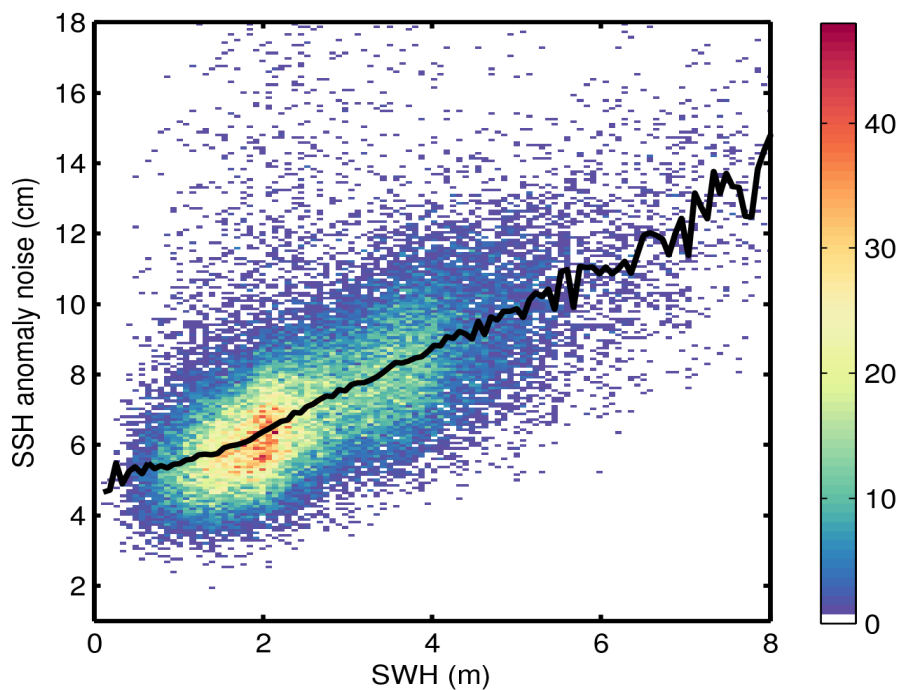
Figure 9. 2D histogram showing flag-valid SSH anomaly noise as a function of SWH for 17/05/2014. The black line denotes the median SSH anomaly as a function of SWH.
