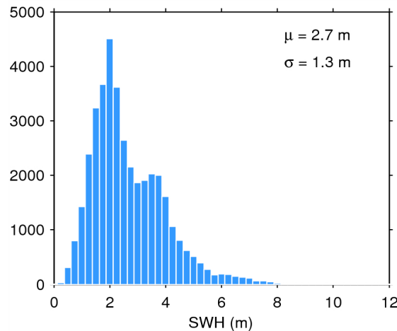
Figure 20. Histogram of science-valid SWH over oceans and lakes for 17/05/2014. The mean ( \mu ) and standard deviation ( \sigma ) are also shown. Note that values larger than 12 m are excluded from the histogram for the sake of readability but not from the computation of \mu and \sigma .
