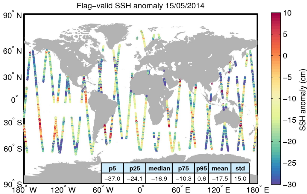
Figure 5. Geographical distribution of flag-valid 1-Hz SSH anomaly data over oceans and lakes for 15/05/2014. The statistical values shown in the table refer to the SSH anomaly in cm and are calculated over all measurements shown in the figure.
