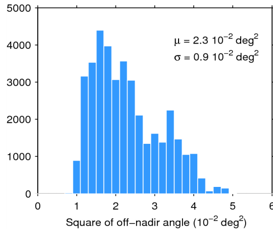
Figure 39. Histogram of flag-valid mispointing over oceans and lakes for 15/05/2014. The mean ( \mu ) and standard deviation ( \sigma ) are also shown. Note that values than 6 \cdot 10^{-2} \text{ deg}^2 are excluded from the histogram for the sake of readability but not from the computation of \mu and \sigma .
