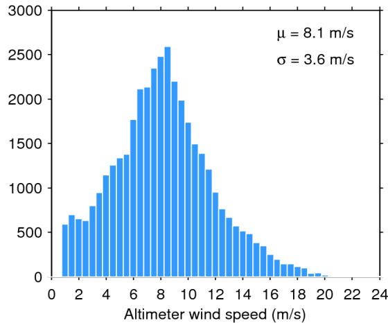
Figure 33. Histogram of flag-valid wind over oceans and lakes for 15/05/2014. The mean ( \mu ) and standard deviation ( \sigma ) are also shown. Note that values larger than 24 m/s are excluded from the histogram for the sake of readability but not from the computation of \mu and \sigma .
