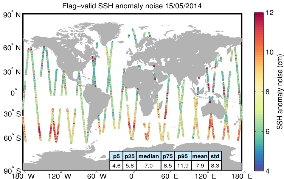
Figure 8. Geographical distribution of flag-valid 20-Hz SSH anomaly measurement noise over oceans and lakes for 15/05/2014. The statistical values shown in the table refer to the SSH anomaly noise and are calculated over all measurements shown in the figure.
