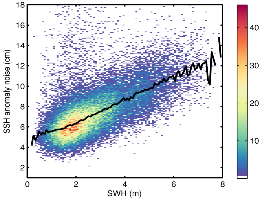
Figure 9. 2D histogram showing flag-valid SSH anomaly noise as a function of SWH for 15/05/2014. The black line denotes the median SSH anomaly as a function of SWH.
