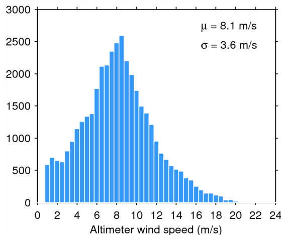
Figure 35. Histogram of science-valid wind over oceans and lakes for 15/05/2014. The mean ( \mu ) and standard deviation ( \sigma ) are also shown. Note that values larger than 24 m/s are excluded from the histogram for the sake of readability but not from the computation of \mu and \sigma .
