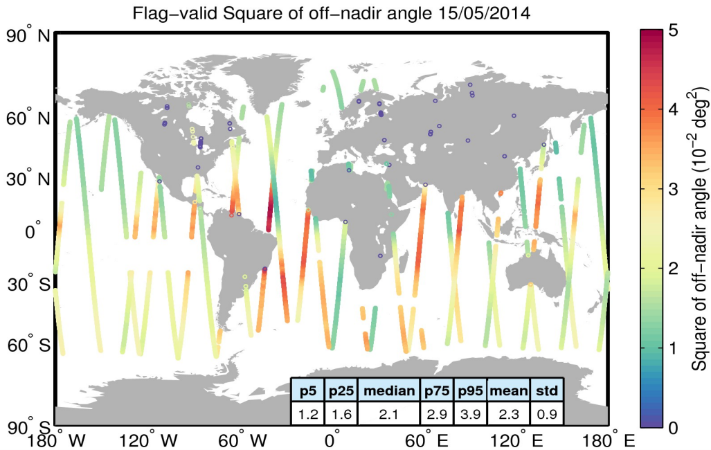
Figure 37. Geographical distribution of flag-valid mispointing data over oceans and lakes for 15/05/2014. The statistical values shown in the table refer to the mispointing in 10^{-2} \text{deg}^2 and are calculated over all measurements shown in the figure.
