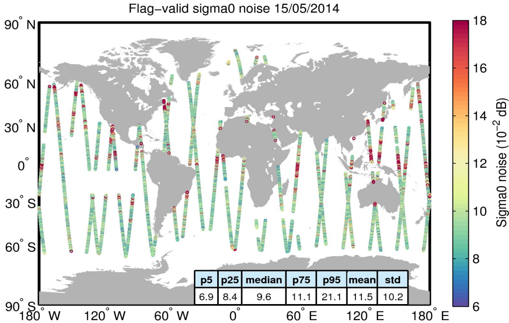
Figure 26. Geographical distribution of flag-valid 20-Hz sigma0 measurement noise over oceans and lakes for 15/05/2014. The statistical values shown in the table refer to the sigma0 noise and are calculated over all measurements shown in the figure.
