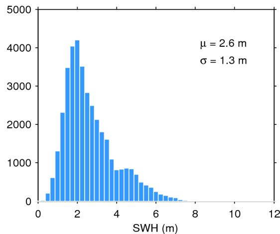
Figure 20. Histogram of science-valid SWH over oceans and lakes for 15/05/2014. The mean ( \mu ) and standard deviation ( \sigma ) are also shown. Note that values larger than 12 m are excluded from the histogram for the sake of readability but not from the computation of \mu and \sigma .
