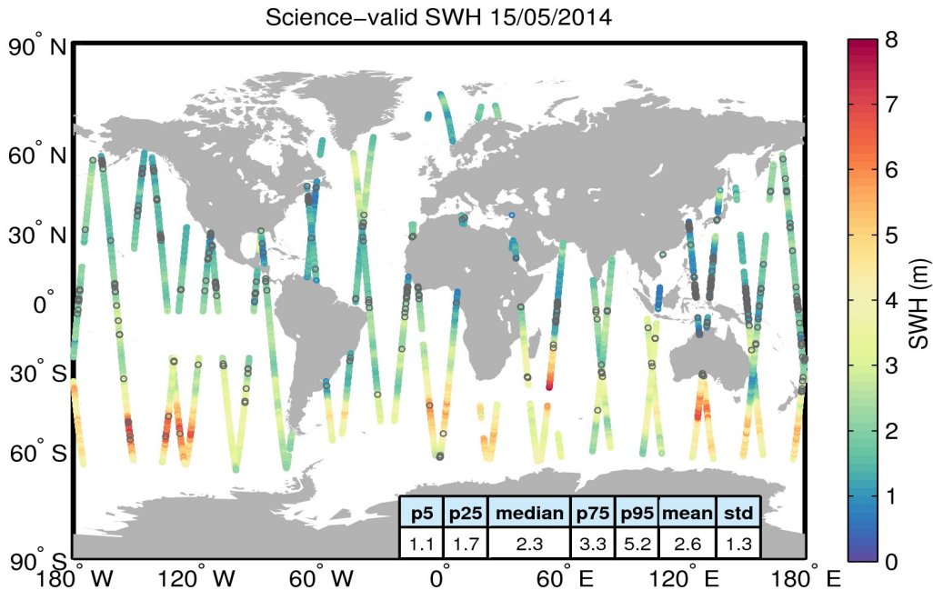
Figure 19. Geographical distribution of science-valid SWH data over oceans and lakes for 15/05/2014. The statistical values shown in the table refer to the SWH in m and are calculated over all measurements shown in the figure. Gray circles denote records that have been rejected based on the editing criteria described in Table 3.
