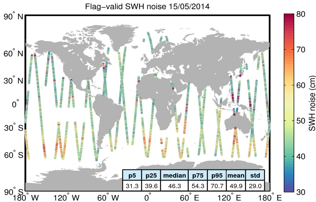
Figure 18. Geographical distribution of flag-valid 20-Hz SWH measurement noise over oceans and lakes for 15/05/2014. The statistical values shown in the figure refer to the SWH noise and are calculated over all measurements shown in the figure.
