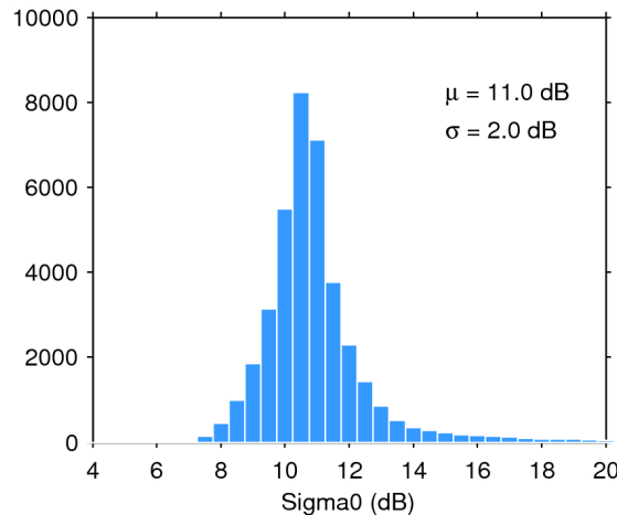
Figure 25. Histogram of flag-valid sigma0 over oceans and lakes for 15/05/2014. The mean ( \mu ) and standard deviation ( \sigma ) are also shown. Note that values outside [4 20] dB are excluded from the histogram for the sake of readability but not from the computation of \mu and \sigma .
