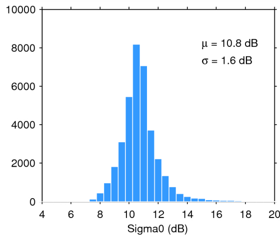
Figure 28. Histogram of science-valid sigma0 over oceans and lakes for 15/05/2014. The mean ( \mu ) and standard deviation ( \sigma ) are also shown. Note that values outside [4 20] dB are excluded from the histogram for the sake of readability but not from the computation of \mu and \sigma .
