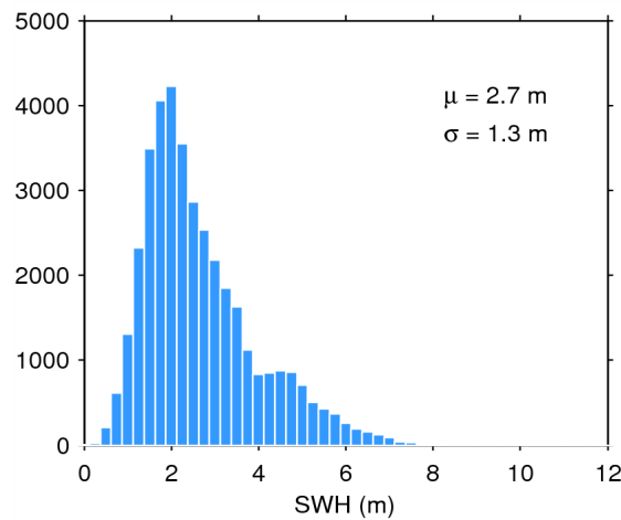
Figure 17. Histogram of flag-valid SWH over oceans and lakes for 15/05/2014. The mean ( \mu ) and standard deviation ( \sigma ) are also shown. Note that values larger than 12 m are excluded from the histogram for the sake of readability but not from the computation of \mu and \sigma .
