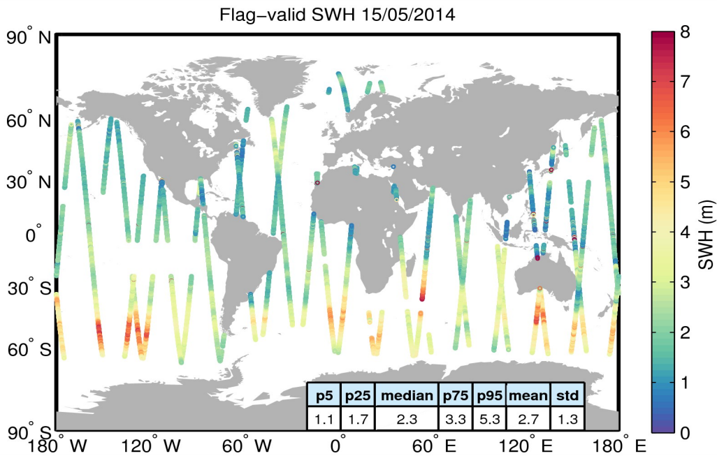
Figure 15. Geographical distribution of flag-valid SWH data over oceans and lakes for 15/05/2014. The statistical values shown in the table refer to the SWH in m and are calculated over all measurements shown in the figure.
