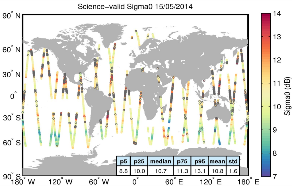
Figure 27. Geographical distribution of science-valid sigma0 data over oceans and lakes for 15/05/2014. The statistical values shown in the table refer to the sigma0 in dB and are calculated over all measurements shown in the figure. Gray circles denote records that have been rejected based on the editing criteria described in Table 4.
