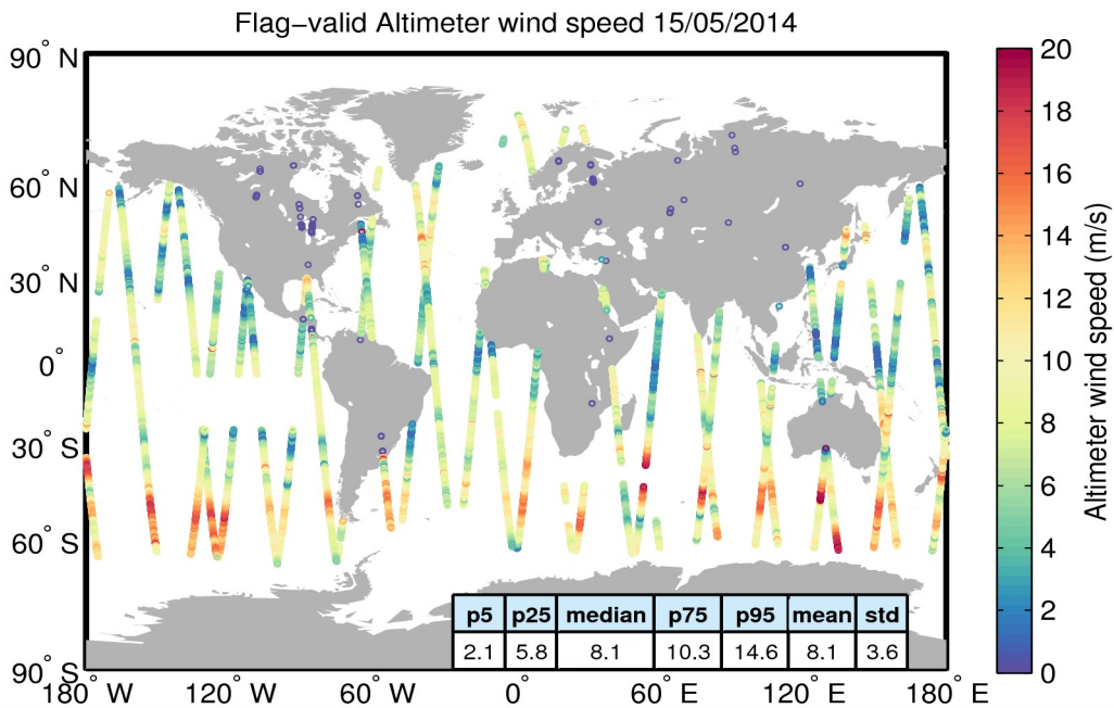
Figure 31. Geographical distribution of flag-valid wind data over oceans and lakes for 15/05/2014. The statistical values shown in the table refer to the wind in m/s and are calculated over all measurements shown in the figure.
