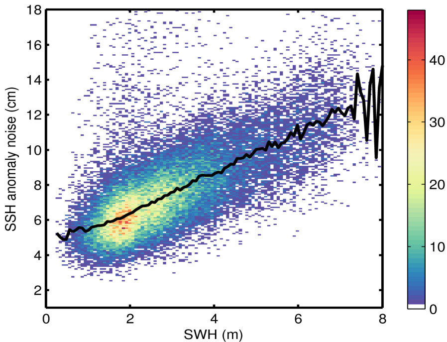
Figure 9. 2D histogram showing flag-valid SSH anomaly noise as a function of SWH for 14/05/2014. The black line denotes the median SSH anomaly as a function of SWH.
