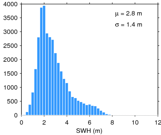
Figure 20. Histogram of science-valid SWH over oceans and lakes for 14/05/2014. The mean ( \mu ) and standard deviation ( \sigma ) are also shown. Note that values larger than 12 m are excluded from the histogram for the sake of readability but not from the computation of \mu and \sigma .
