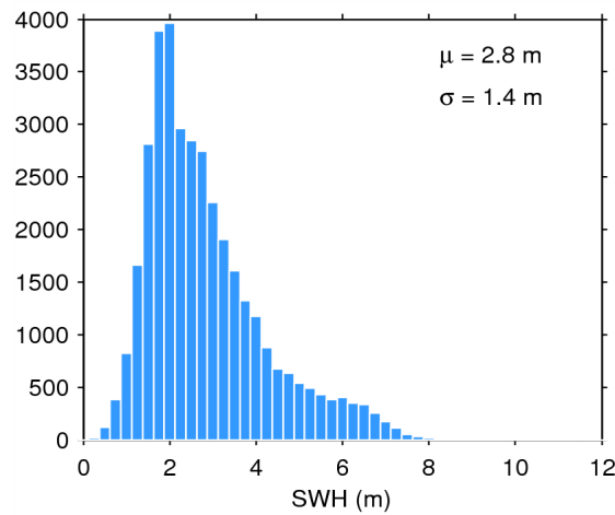
Figure 17. Histogram of flag-valid SWH over oceans and lakes for 14/05/2014. The mean ( \mu ) and standard deviation ( \sigma ) are also shown. Note that values larger than 12 m are excluded from the histogram for the sake of readability but not from the computation of \mu and \sigma .
