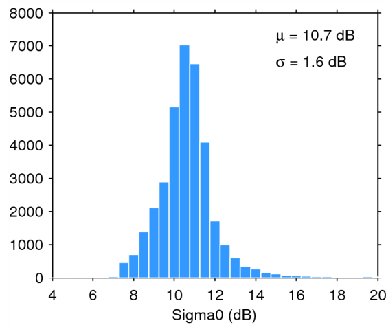
Figure 28. Histogram of science-valid sigma0 over oceans and lakes for 14/05/2014. The mean ( \mu ) and standard deviation ( \sigma ) are also shown. Note that values outside [4 20] dB are excluded from the histogram for the sake of readability but not from the computation of \mu and \sigma .
