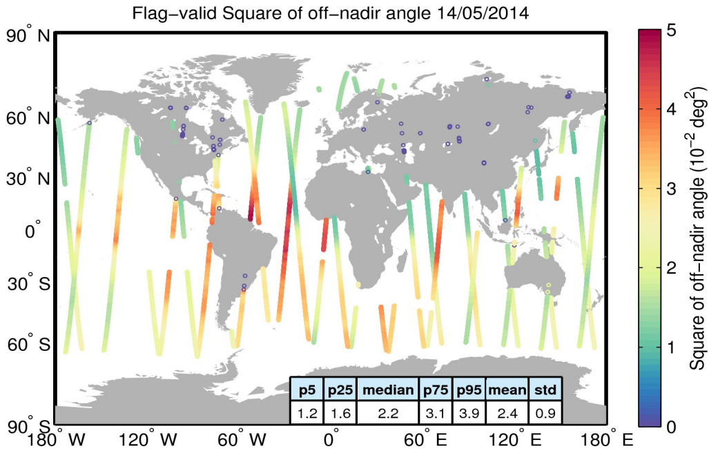
Figure 37. Geographical distribution of flag-valid mispointing data over oceans and lakes for 14/05/2014. The statistical values shown in the table refer to the mispointing in 10^{-2} \text{deg}^2 and are calculated over all measurements shown in the figure.
