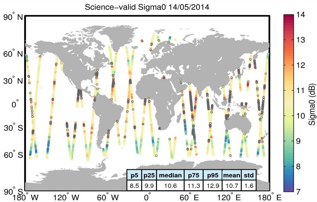
Figure 27. Geographical distribution of science-valid sigma0 data over oceans and lakes for 14/05/2014. The statistical values shown in the table refer to the sigma0 in dB and are calculated over all measurements shown in the figure. Gray circles denote records that have been rejected based on the editing criteria described in Table 4.
