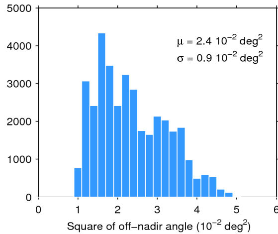
Figure 39. Histogram of flag-valid mispointing over oceans and lakes for 14/05/2014. The mean ( \mu ) and standard deviation ( \sigma ) are also shown. Note that values than 6 \cdot 10^{-2} \text{ deg}^2 are excluded from the histogram for the sake of readability but not from the computation of \mu and \sigma .
