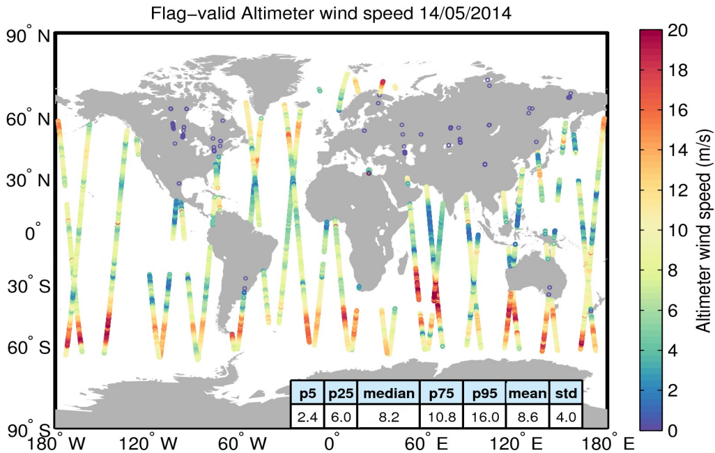
Figure 31. Geographical distribution of flag-valid wind data over oceans and lakes for 14/05/2014. The statistical values shown in the table refer to the wind in m/s and are calculated over all measurements shown in the figure.
