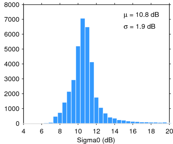
Figure 25. Histogram of flag-valid sigma0 over oceans and lakes for 14/05/2014. The mean ( \mu ) and standard deviation ( \sigma ) are also shown. Note that values outside [4 20] dB are excluded from the histogram for the sake of readability but not from the computation of \mu and \sigma .
