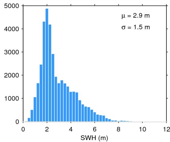
Figure 17. Histogram of flag-valid SWH over oceans and lakes for 13/05/2014. The mean ( \mu ) and standard deviation ( \sigma ) are also shown. Note that values larger than 12 m are excluded from the histogram for the sake of readability but not from the computation of \mu and \sigma .
