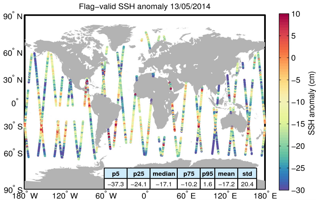
Figure 5. Geographical distribution of flag-valid 1-Hz SSH anomaly data over oceans and lakes for 13/05/2014. The statistical values shown in the table refer to the SSH anomaly in cm and are calculated over all measurements shown in the figure.
