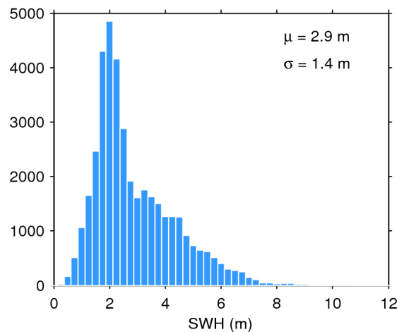
Figure 20. Histogram of science-valid SWH over oceans and lakes for 13/05/2014. The mean ( \mu ) and standard deviation ( \sigma ) are also shown. Note that values larger than 12 m are excluded from the histogram for the sake of readability but not from the computation of \mu and \sigma .
