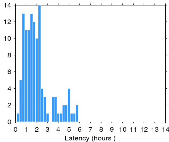
Figure 2. Histogram of the data latency for 13/05/2014. The y-axis denotes the number of files that are made available with a delay of x-hours with respect to the mean time of the records stored in the file.
