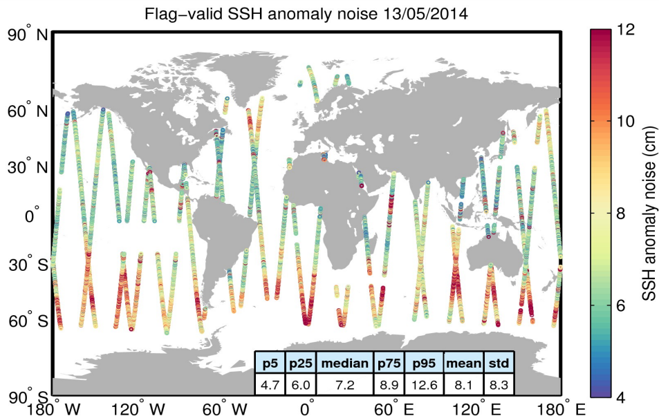
Figure 8. Geographical distribution of flag-valid 20-Hz SSH anomaly measurement noise over oceans and lakes for 13/05/2014. The statistical values shown in the table refer to the SSH anomaly noise and are calculated over all measurements shown in the figure.
