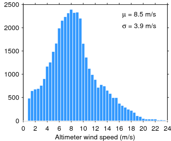
Figure 33. Histogram of flag-valid wind over oceans and lakes for 13/05/2014. The mean ( \mu ) and standard deviation ( \sigma ) are also shown. Note that values larger than 24 m/s are excluded from the histogram for the sake of readability but not from the computation of \mu and \sigma .
