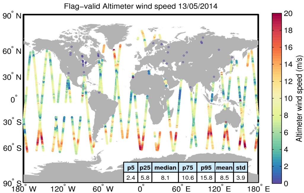
Figure 31. Geographical distribution of flag-valid wind data over oceans and lakes for 13/05/2014. The statistical values shown in the table refer to the wind in m/s and are calculated over all measurements shown in the figure.
