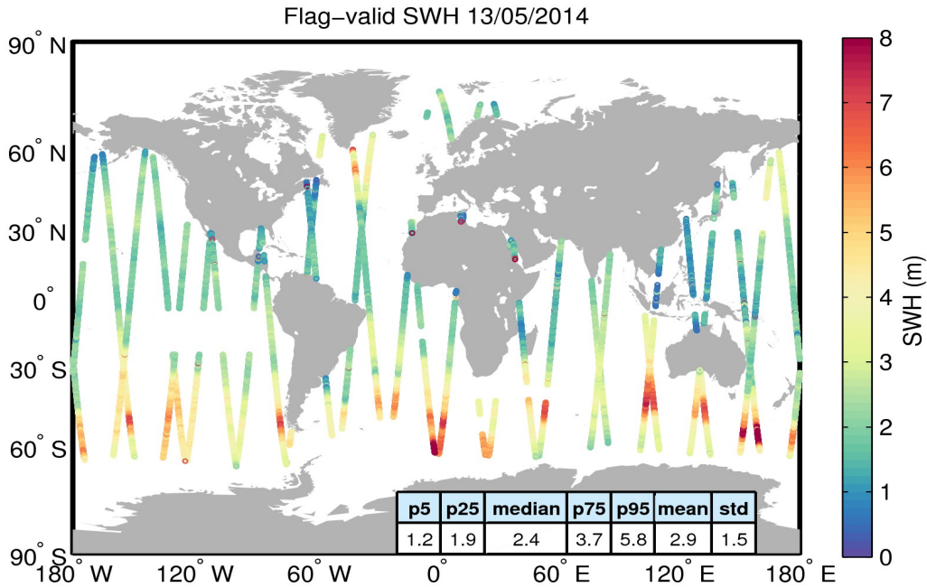
Figure 15. Geographical distribution of flag-valid SWH data over oceans and lakes for 13/05/2014. The statistical values shown in the table refer to the SWH in m and are calculated over all measurements shown in the figure.
