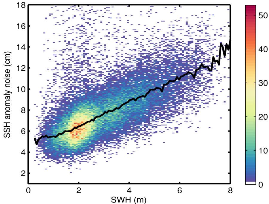
Figure 9. 2D histogram showing flag-valid SSH anomaly noise as a function of SWH for 13/05/2014. The black line denotes the median SSH anomaly as a function of SWH.
