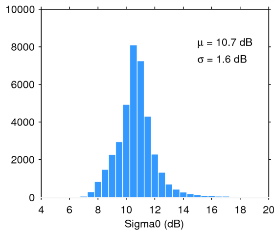
Figure 28. Histogram of science-valid sigma0 over oceans and lakes for 13/05/2014. The mean ( \mu ) and standard deviation ( \sigma ) are also shown. Note that values outside [4 20] dB are excluded from the histogram for the sake of readability but not from the computation of \mu and \sigma .
