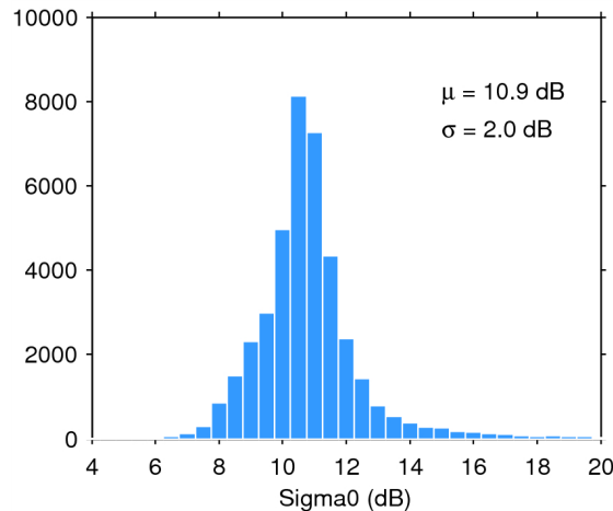
Figure 25. Histogram of flag-valid sigma0 over oceans and lakes for 13/05/2014. The mean ( \mu ) and standard deviation ( \sigma ) are also shown. Note that values outside [4 20] dB are excluded from the histogram for the sake of readability but not from the computation of \mu and \sigma .
