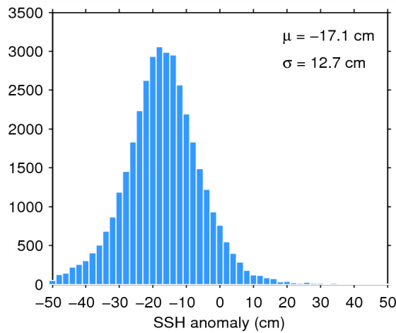
Figure 11. Histogram of science-valid SSH anomaly over oceans and lakes for 13/05/2014. The mean ( \mu ) and standard deviation ( \sigma ) are also shown. Note that values outside [-50 50] cm are excluded from the histogram for the sake of readability but not from the computation of \mu and \sigma .
