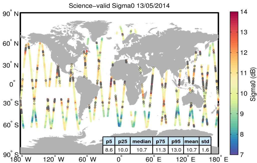
Figure 27. Geographical distribution of science-valid sigma0 data over oceans and lakes for 13/05/2014. The statistical values shown in the table refer to the sigma0 in dB and are calculated over all measurements shown in the figure. Gray circles denote records that have been rejected based on the editing criteria described in Table 4.
