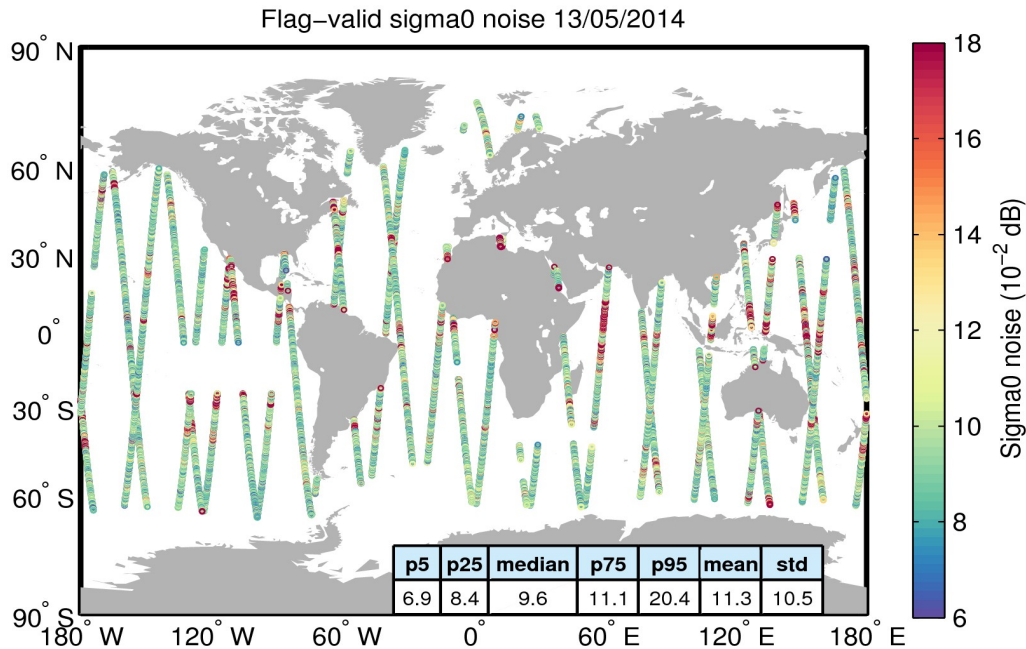
Figure 26. Geographical distribution of flag-valid 20-Hz sigma0 measurement noise over oceans and lakes for 13/05/2014. The statistical values shown in the table refer to the sigma0 noise and are calculated over all measurements shown in the figure.
