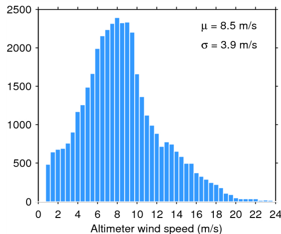
Figure 35. Histogram of science-valid wind over oceans and lakes for 13/05/2014. The mean ( \mu ) and standard deviation ( \sigma ) are also shown. Note that values larger than 24 m/s are excluded from the histogram for the sake of readability but not from the computation of \mu and \sigma .
