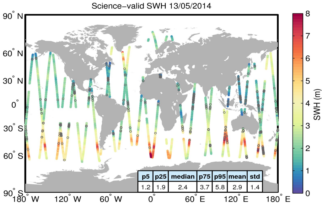
Figure 19. Geographical distribution of science-valid SWH data over oceans and lakes for 13/05/2014. The statistical values shown in the table refer to the SWH in m and are calculated over all measurements shown in the figure. Gray circles denote records that have been rejected based on the editing criteria described in Table 3.
