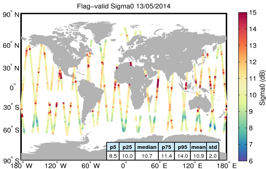
Figure 23. Geographical distribution of flag-valid sigma0 data over oceans and lakes for 13/05/2014. The statistical values shown in the table refer to the sigma0 in dB and are calculated over all measurements shown in the figure.
