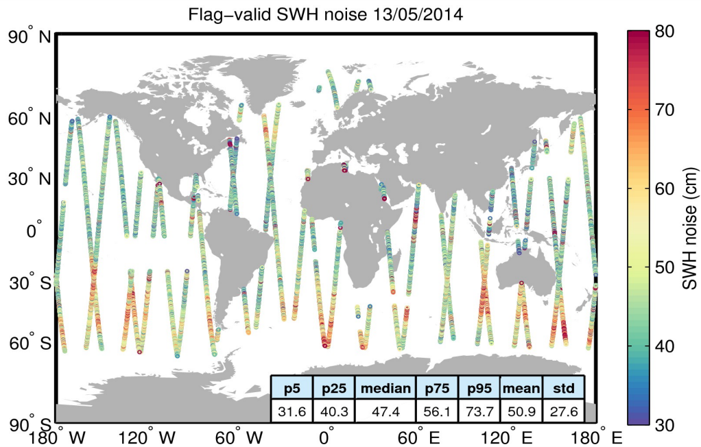
Figure 18. Geographical distribution of flag-valid 20-Hz SWH measurement noise over oceans and lakes for 13/05/2014. The statistical values shown in the figure refer to the SWH noise and are calculated over all measurements shown in the figure.
