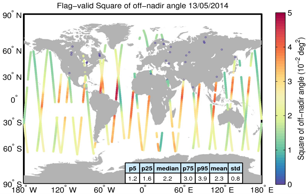
Figure 37. Geographical distribution of flag-valid mispointing data over oceans and lakes for 13/05/2014. The statistical values shown in the table refer to the mispointing in 10^{-2} \text{ deg}^2 and are calculated over all measurements shown in the figure.
