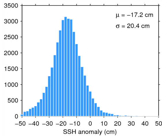
Figure 7. Histogram of flag-valid SSH anomaly over oceans and lakes for 13/05/2014. The mean ( \mu ) and standard deviation ( \sigma ) are also shown. Note that values outside [-50\ 50] cm are excluded from the histogram for the sake of readability but not from the computation of \mu and \sigma .
