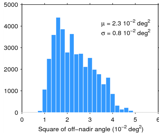
Figure 39. Histogram of flag-valid mispointing over oceans and lakes for 13/05/2014. The mean ( \mu ) and standard deviation ( \sigma ) are also shown. Note that values than 6 \cdot 10^{-2} \text{ deg}^2 are excluded from the histogram for the sake of readability but not from the computation of \mu and \sigma .
